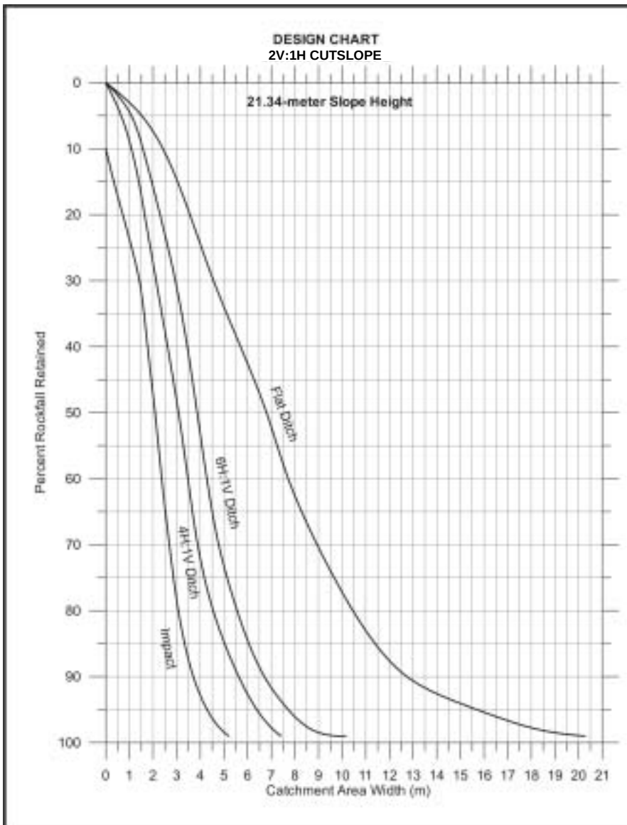
Figure 5.14: Design chart for 21.3-meter high 2V:1H cutslopes
