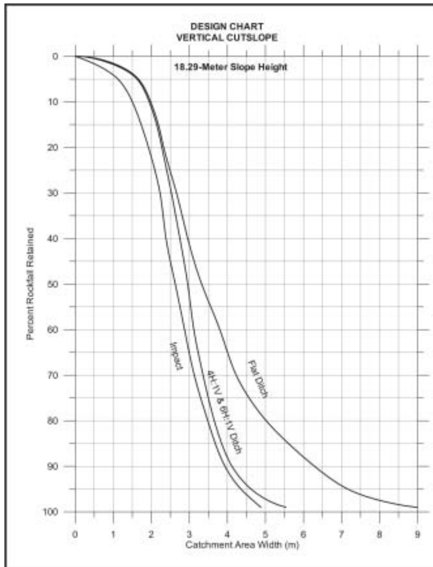
Figure 5.3: Design chart for 18.3-meter high vertical cut slopes
