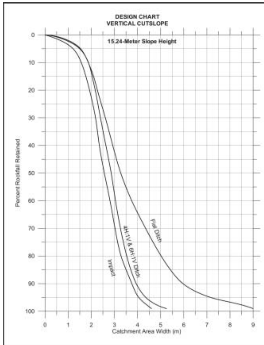
Figure 5.2: Design chart for 15.2-meter high vertical cutslopes
