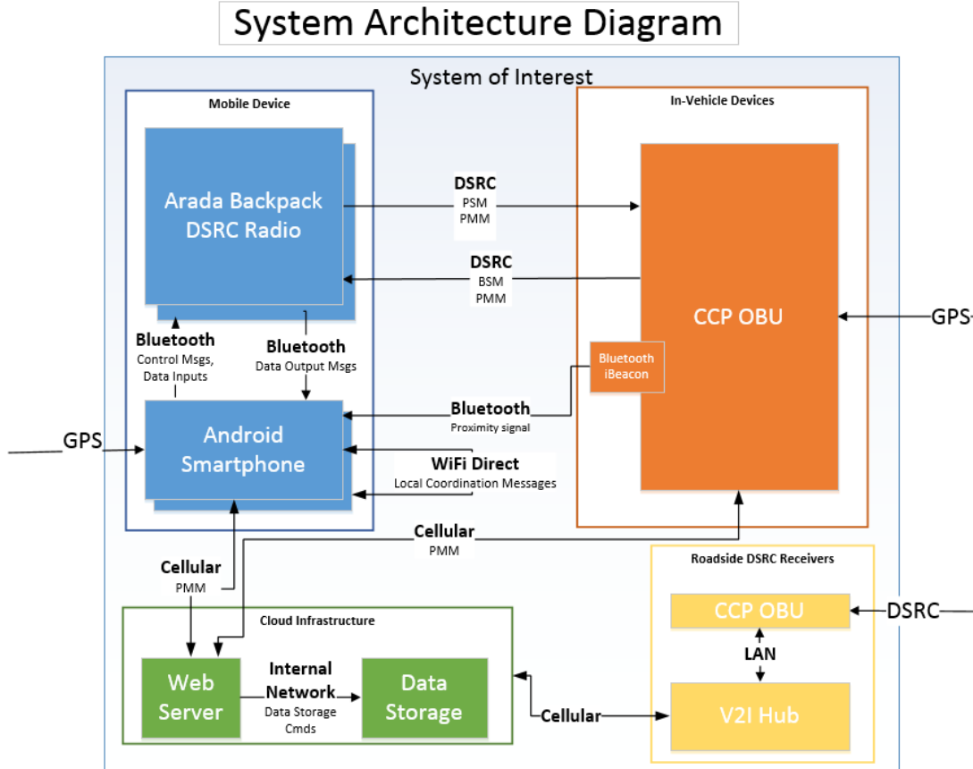
Figure 2. High Level Component Diagram
