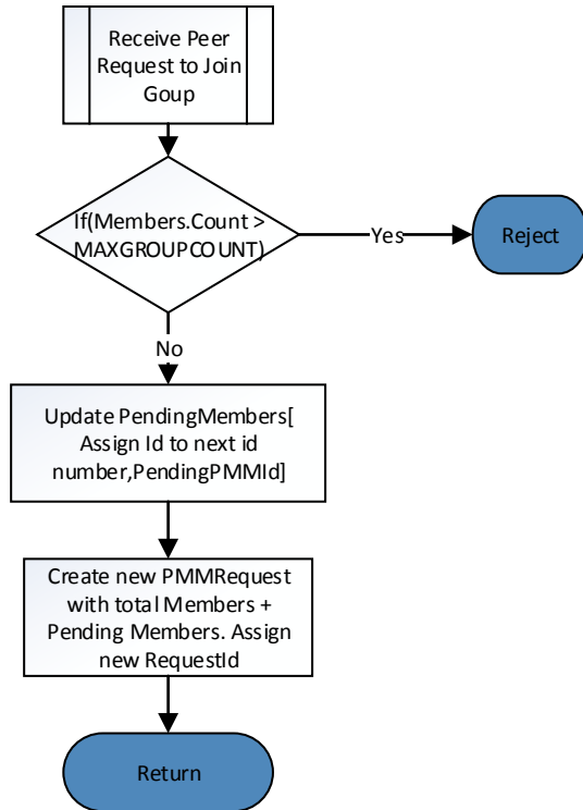
Figure 14. Monitor Receives Request to Join Group
