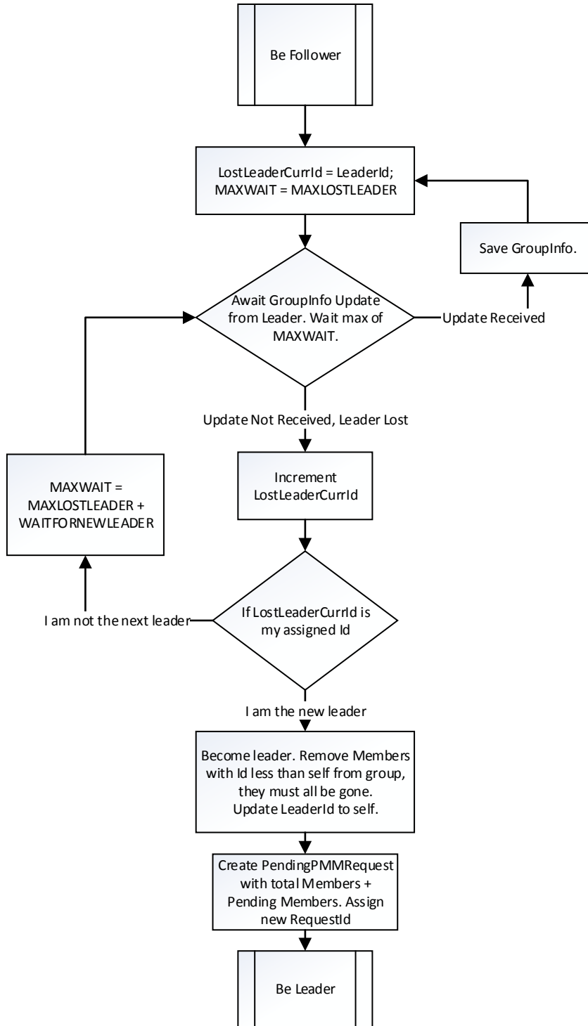
Figure 16. Follower Mode Watches for Loss of Leader
