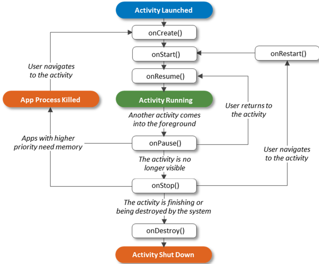
Figure 8. Mobile Device User Interface Application Lifecycle
