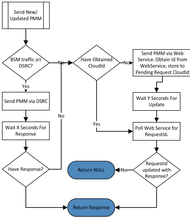
Figure 19. PMM Requests are Sent via Either DSRC or Cellular
