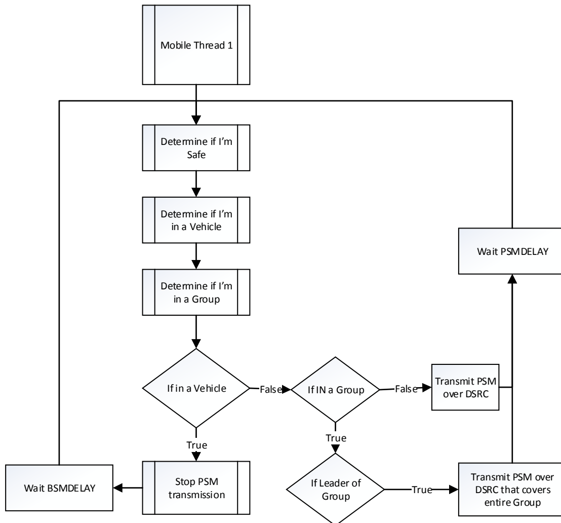
Figure 11. Process for Sending PSMs
