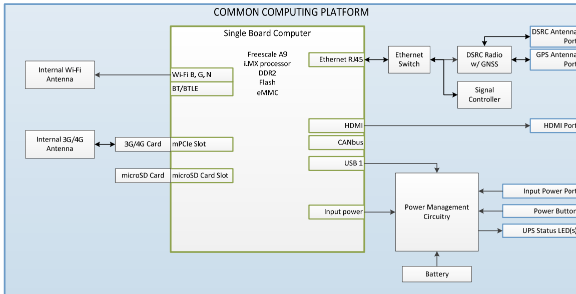
Figure 5. Conceptualized Hardware Architecture of the CCP and DSRC System Communications Ports
