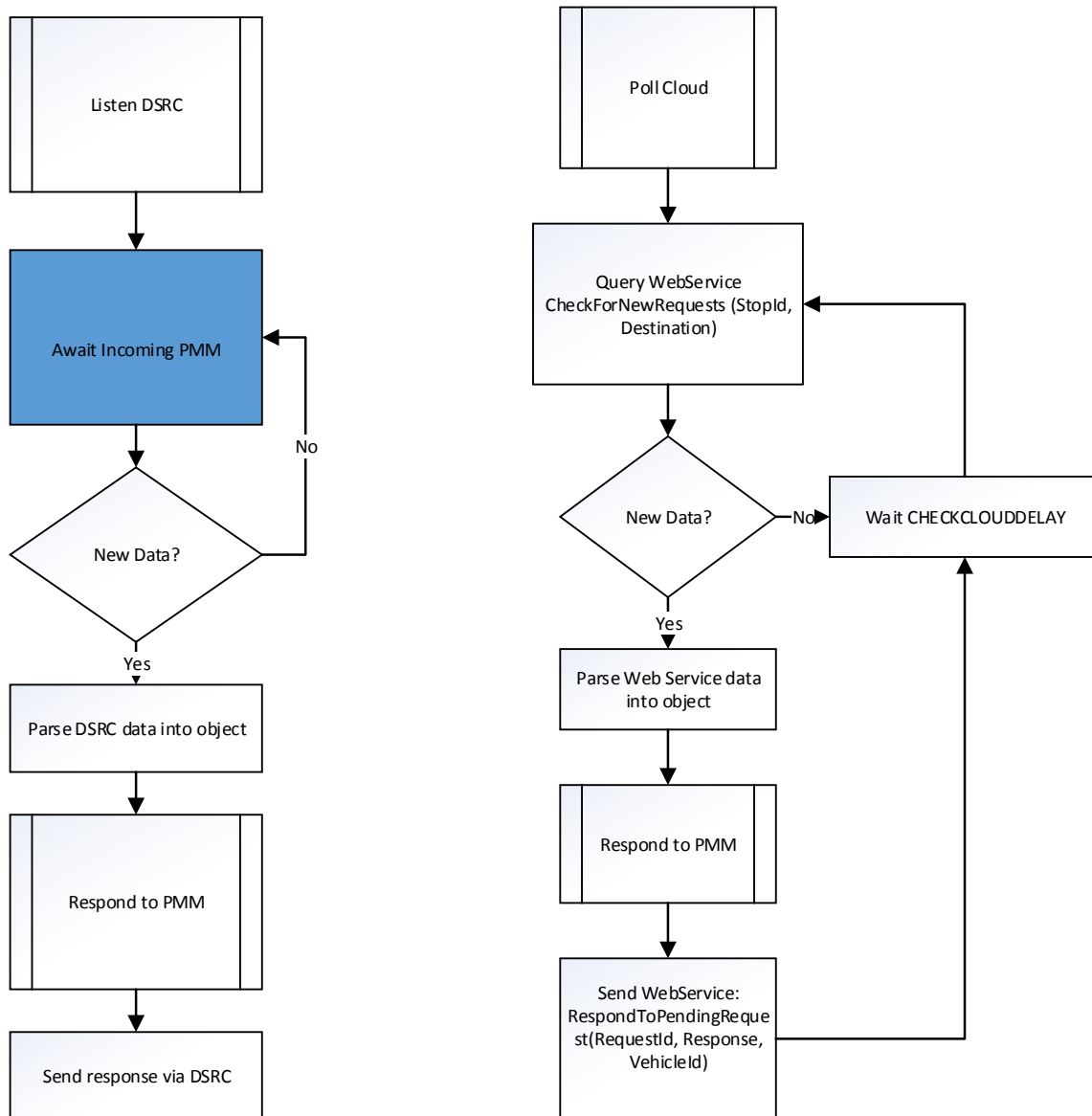
Figure 24. Two Threads for Monitoring Ride Requests
