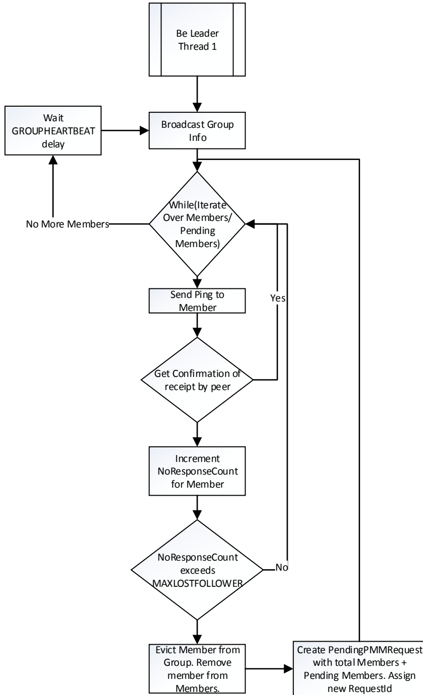
Figure 15. Flow of Leader Keeping Track of Group
