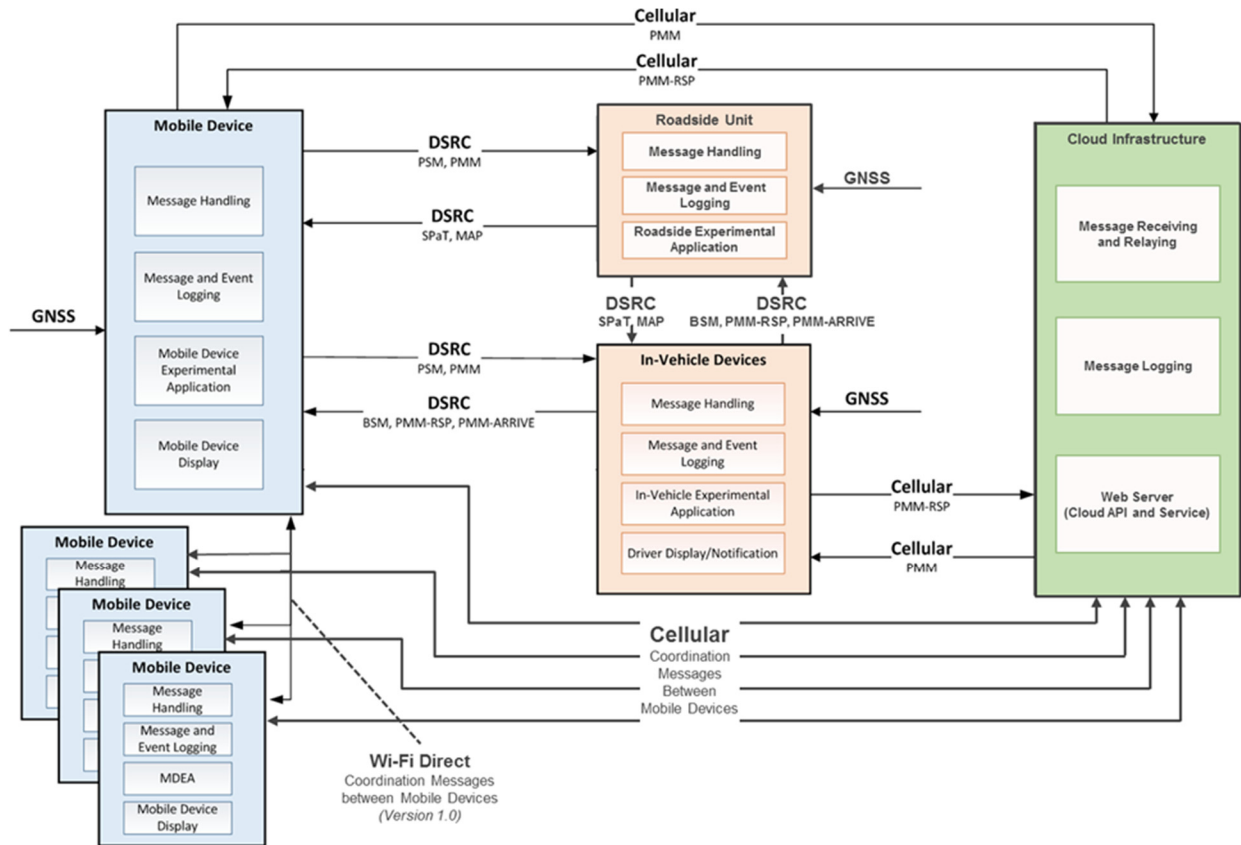
Figure 1. EPS 'System of Interest' Diagram
