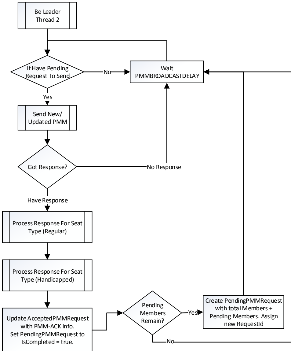
Figure 17. Leader Mode Processes Accepted Members
