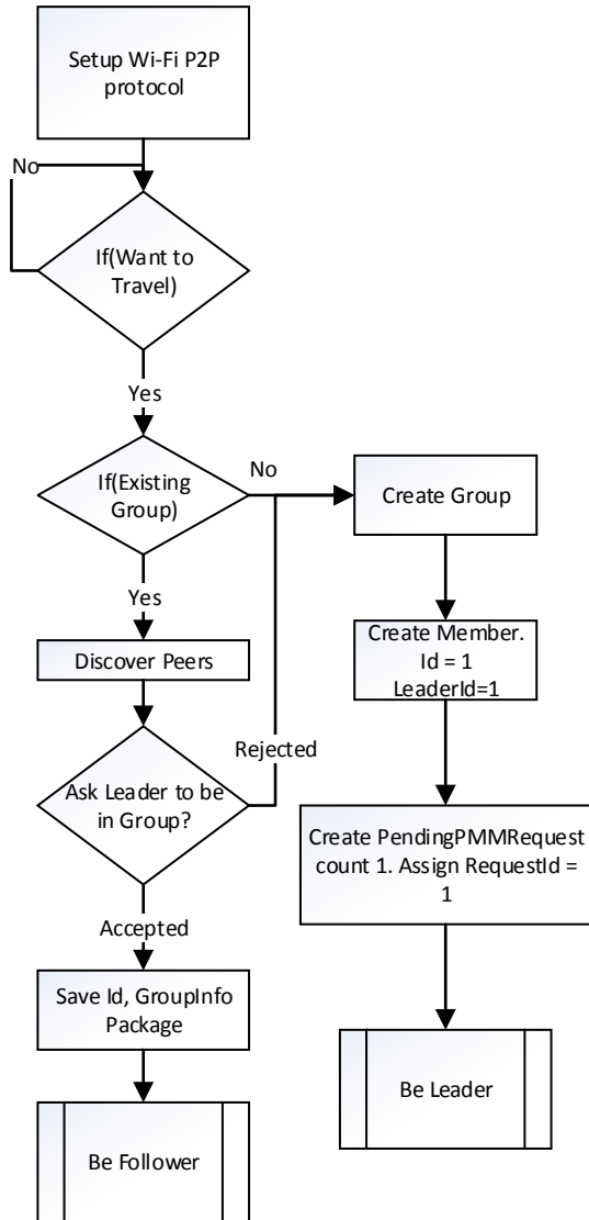
Figure 12. Monitor Decides Role to Play in Group
