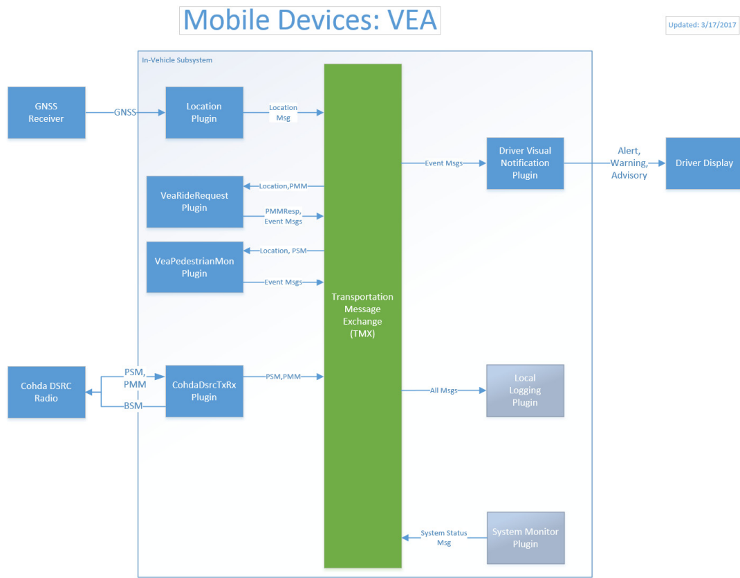
Figure 22. VEA Plugin Diagram
