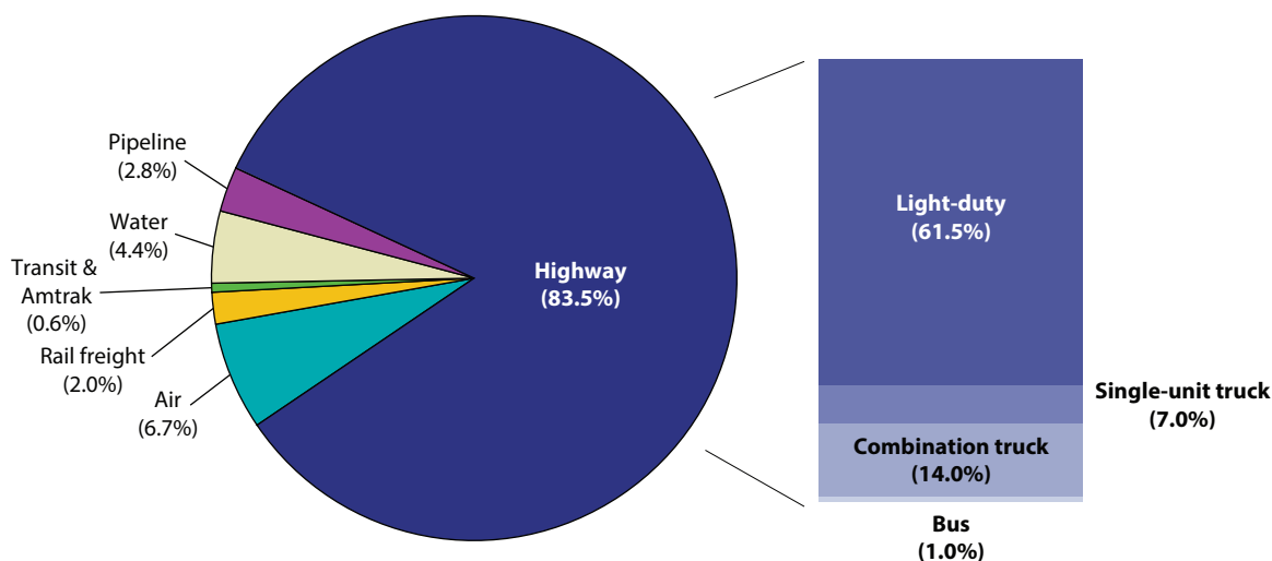
FIGURE 8-3 Energy Use by Mode of Transportation: 2011
