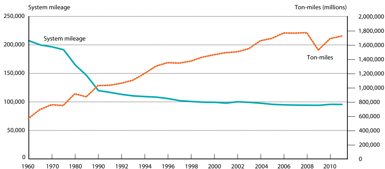
FIGURE 1-3 Class I Railroad System Mileage and Ton-miles of Freight: 1960, 1965, 1970–2011
