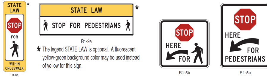
Figure 49. Uncontrolled pedestrian-crosswalk signs (FHWA, 2009).
