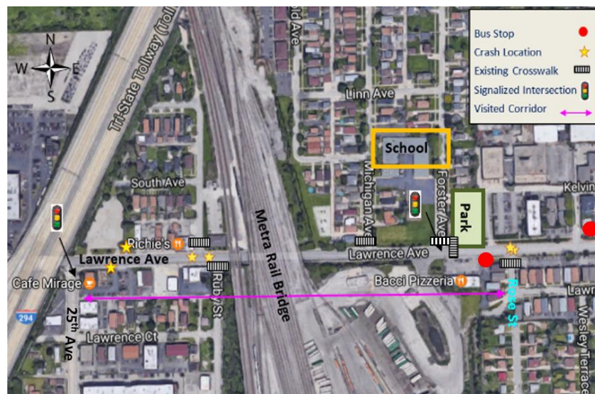
Figure E-83. Overview of Lawrence Ave. (Section One).
