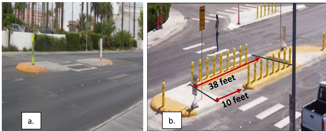
Figure A- 4. a) Raised median (Pulugurtha et al. 2012); b) Danish Offset at Maryland Parkway, Las Vegas (Pechoux et al. 2009).
