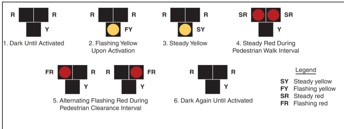
Figure 61. Sequence for a pedestrian hybrid beacon (FHWA, 2009).
