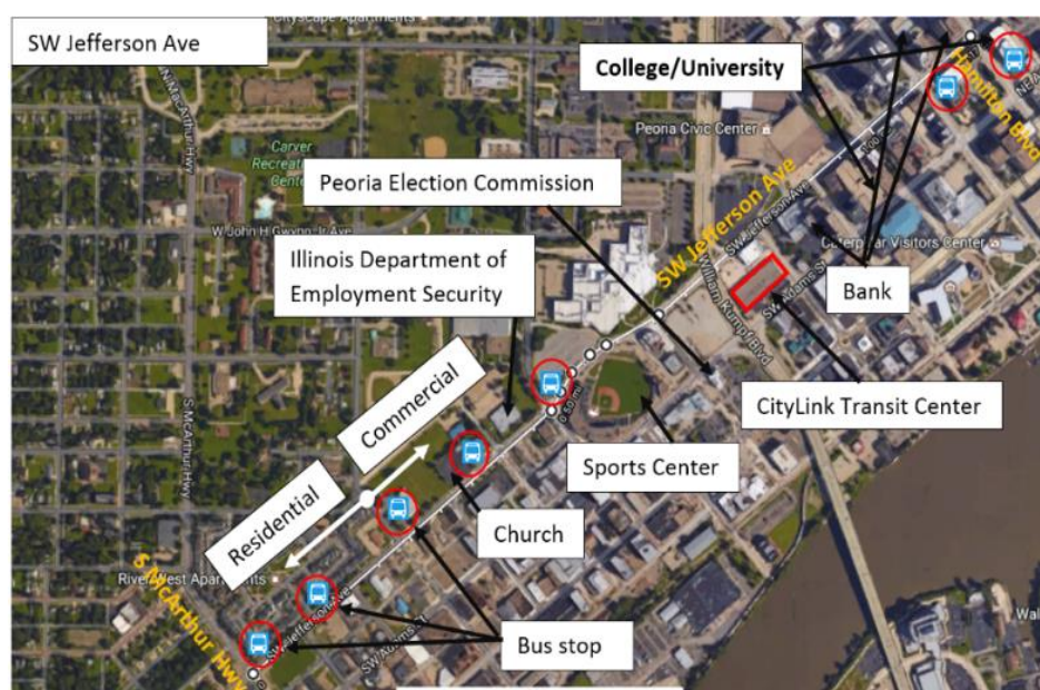
Figure E-9. Land use pattern and pedestrian attractions along SW Jefferson Ave.
