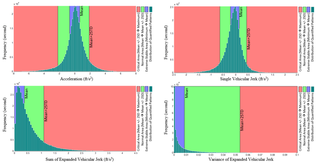
Figure 4: Defining thresholds for 40±0.25 mph speed range.
