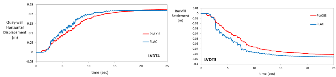
Fig. 24. Horizontal and vertical deformations of the quay-wall using both PLAXIS 2D and FLAC (after Tasiopoulou et al. 2015).
