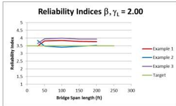
Figure 17. Reliability Indices for Live Load Factor \gamma_L = 2.00
