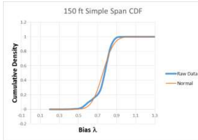
Figure 4. Cumulative Density Function Bias \lambda
