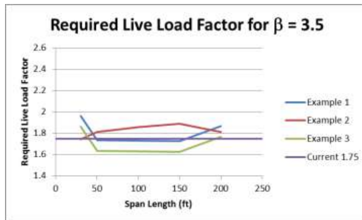
Figure 20. Required Live Load factor for Target \beta = 3.50 for NCHRP Method
