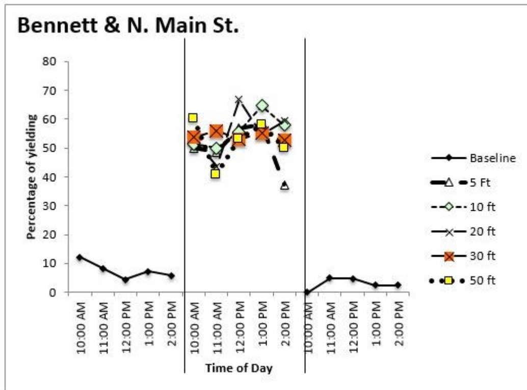
Figure 6.1 The percentage if drivers yielding right-of-way to pedestrians when the sign was placed 5 ft, 10 ft., 20 ft. 30 Ft. and 50 ft. in advance of the crosswalk.
