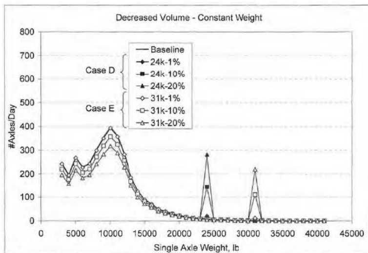
Figure D.7: Single-axle load spectra: decreased volume–constant weight (Timm et al. 2007).
