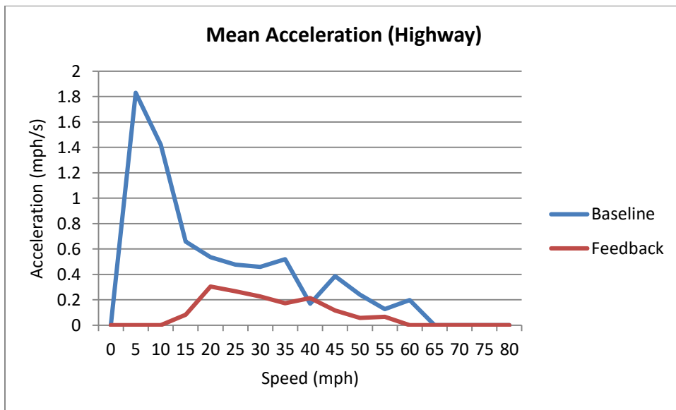
Figure 29. Mean acceleration profile on highway for Driver # 14
