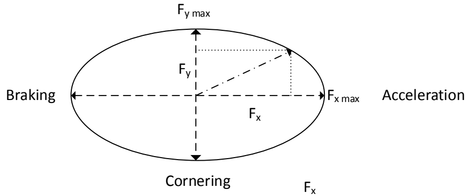
Figure 14. The Tire Friction Ellipse
