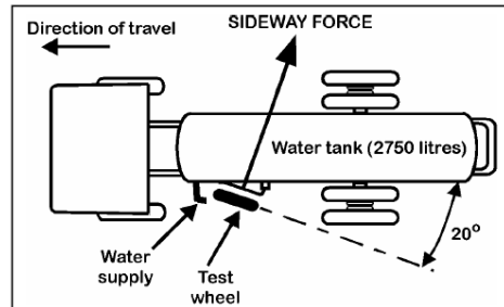
Figure 15. SCRIM Layout [20]
