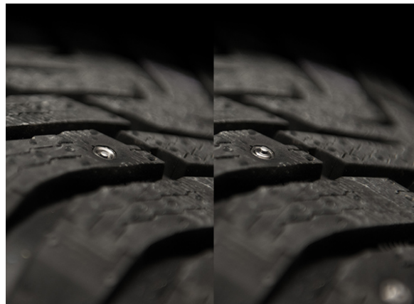
Figure 6. Nokian Hakkapeliitta 8 Concept Tire Showing Stud Retracted and Deployed [7]
