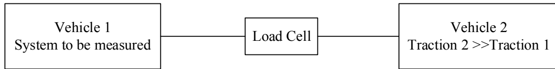
Figure 23. Generalized Pull Test Configuration
