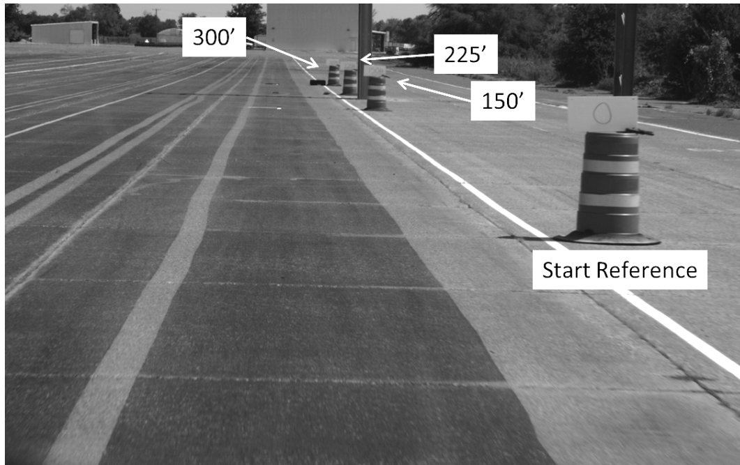
Figure 31. Testing Setup at Riverside Campus.
