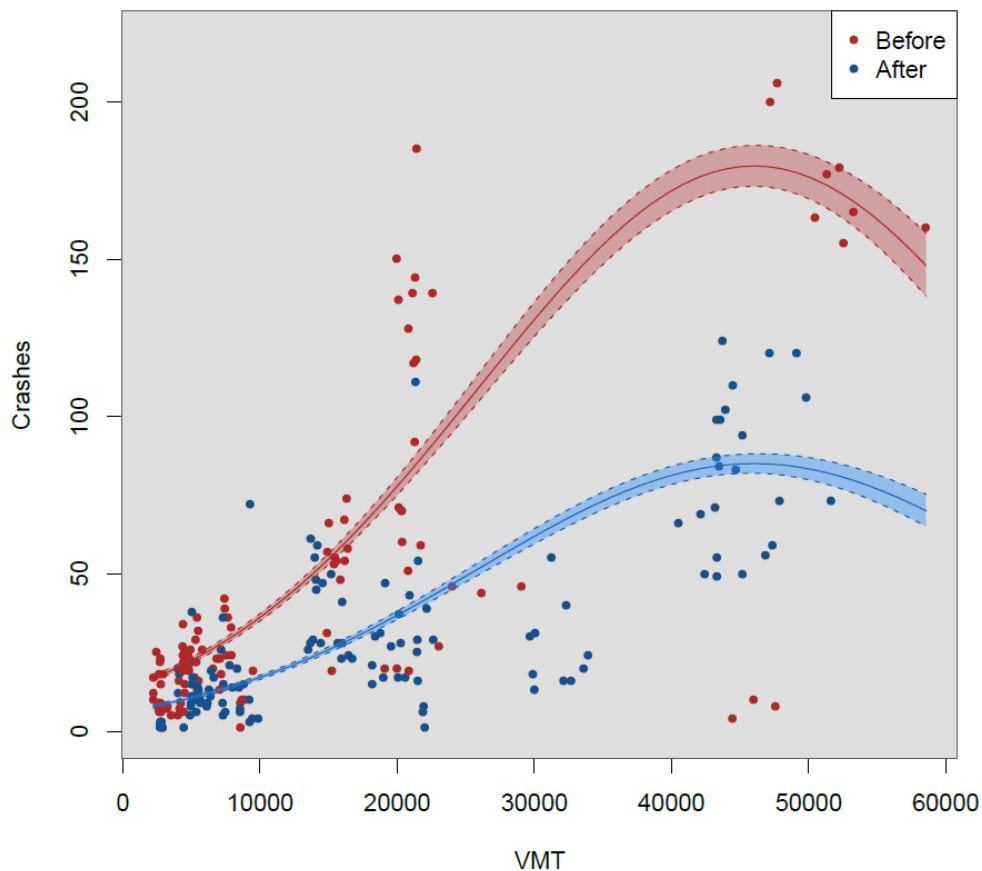
Figure C-1: Regression plot for all AC.
