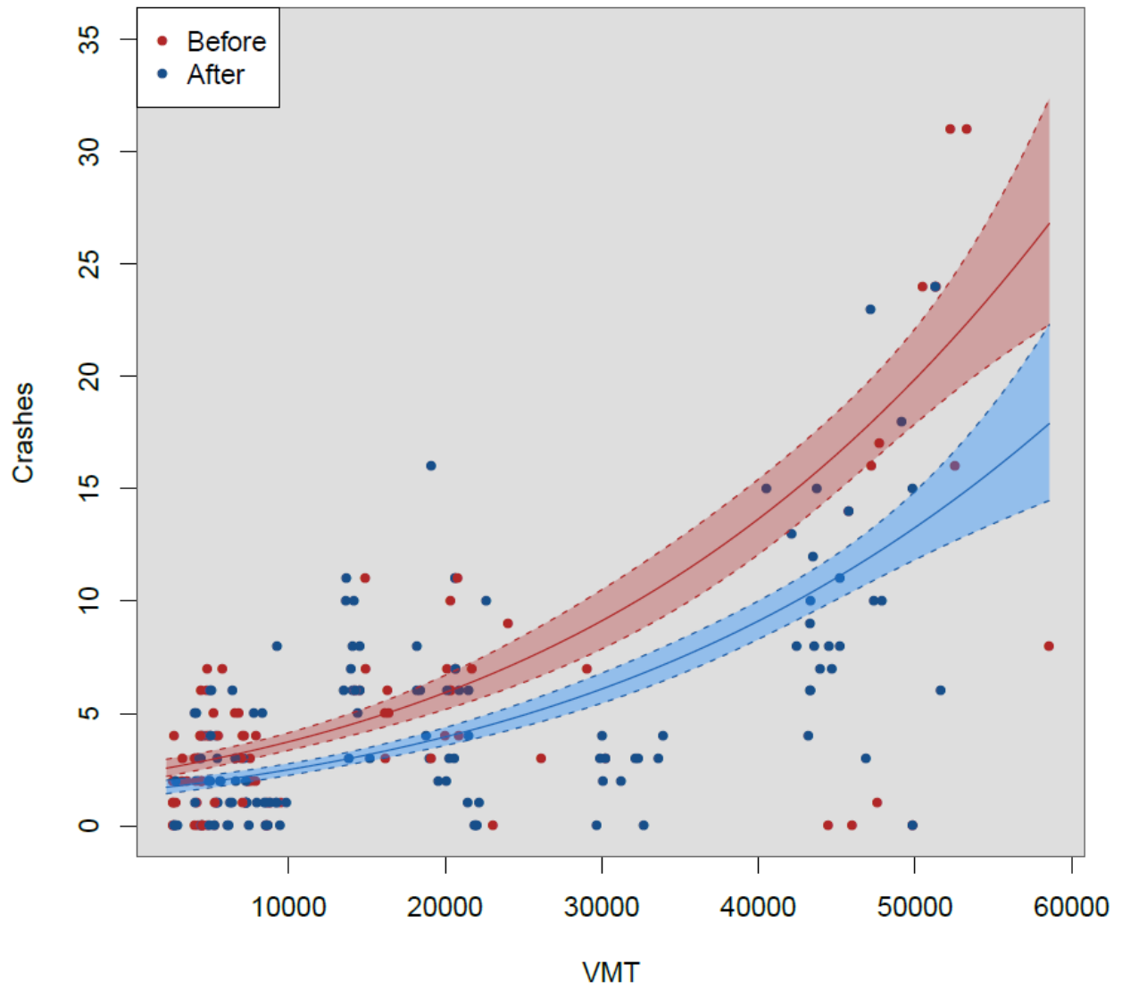
Figure C-20: Regression plot for AC 5 only including crashes with severity 3, 4, and 5.
