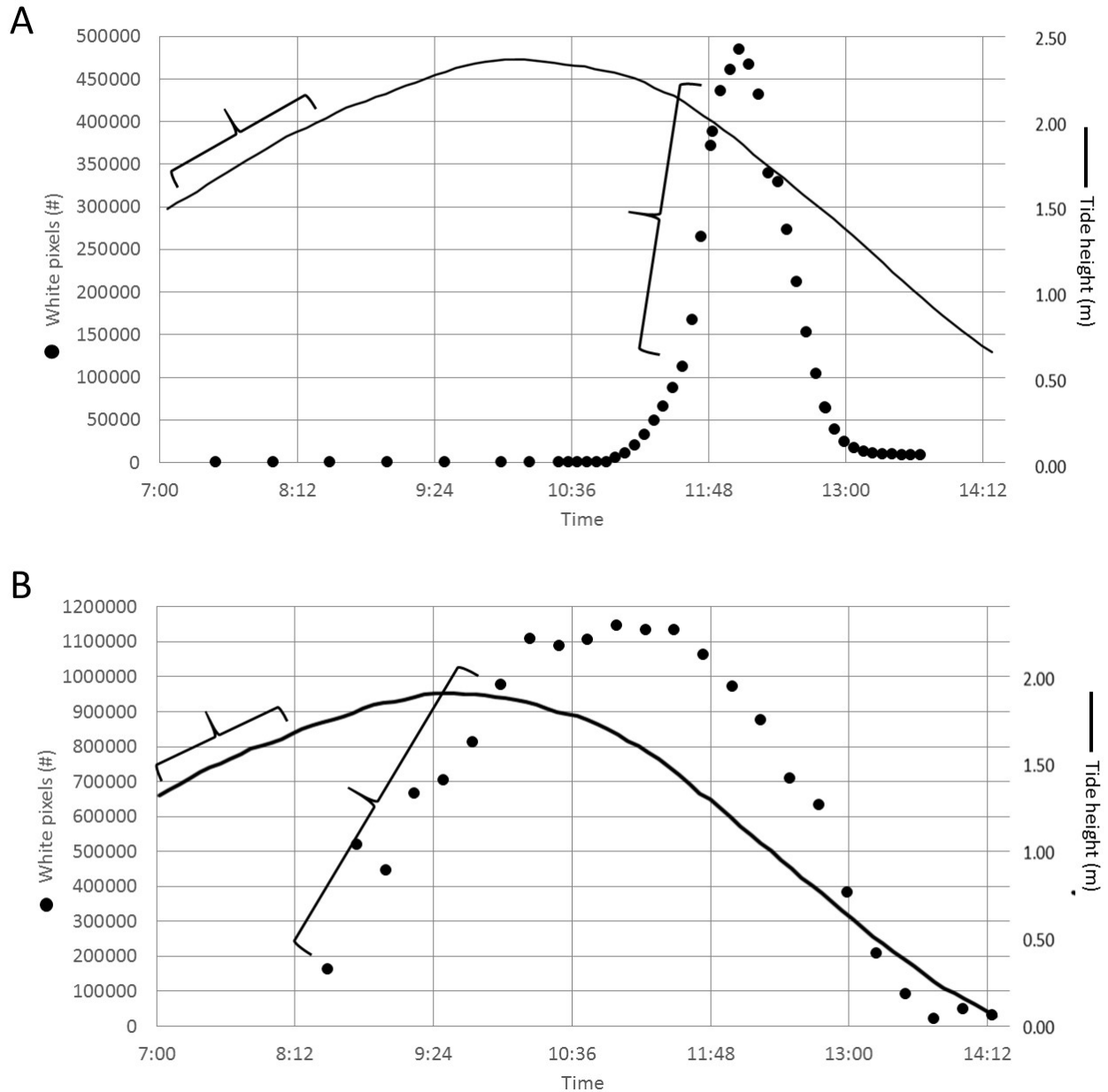
FIGURE 3. Estimated marsh inundation and tide-based change in sea elevation for one tide cycle. Change in reflected light (# white pixels) and sea elevation (tide) for: (A) a mid-high tidal, pickleweed-dominated marsh and B) a mid-tidal, bulrush-dominated marsh. Brackets indicate the range of tide heights and marsh area used to calculate rate of water elevation change and rate of inundation.
