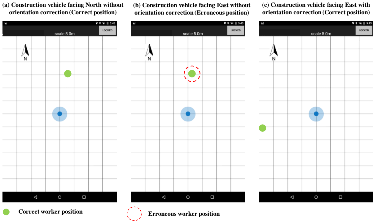
Figure 4.4 Tablet screen snapshots showing relative orientation of worker with respect to the construction vehicle.
