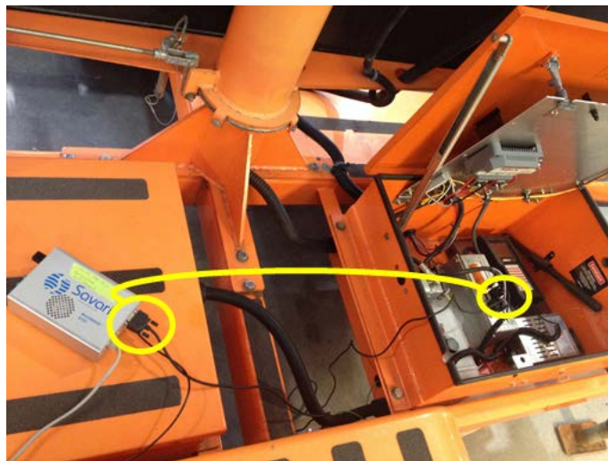
Figure 3.14 Serial connection between VMS and DSRC device.
