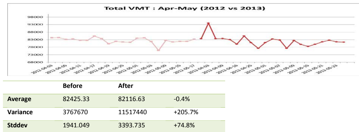
Figure 3.2.16 Before-After Comparison of Total Vehicle Miles Traveled (April-May)
