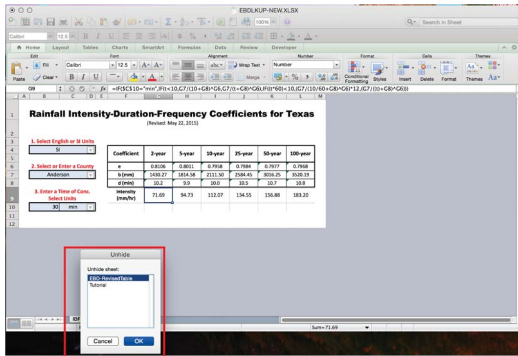
Figure 20: Interface of EBDLKUP-NEW.XLS Spreadsheet. Select a sheet name to unhide – in this example the choices are the EBD-RevisedTable database and the Tutorial sheet. In the final product, the tutorial sheet will be default unhidden – the user should not have to enter a password to follow the tutorial.
