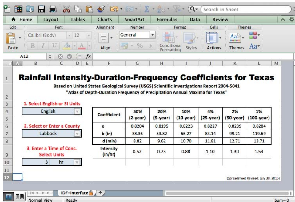
Figure 7: Screen capture of the initial display upon opening the new EBDLKUP-2015.xlsx spreadsheet. The sheet is referred to as the IDF-Interface and interacts with the user through prompts.
