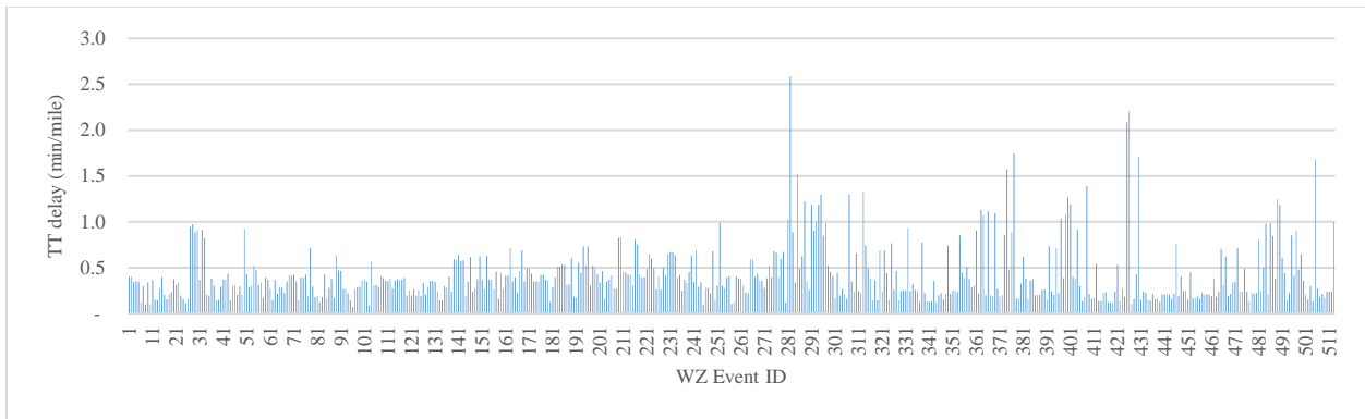
Figure A3. One-mile HATT delay by each WZ event ID of the two interstates (more than one day duration for I-270 and I-70)
