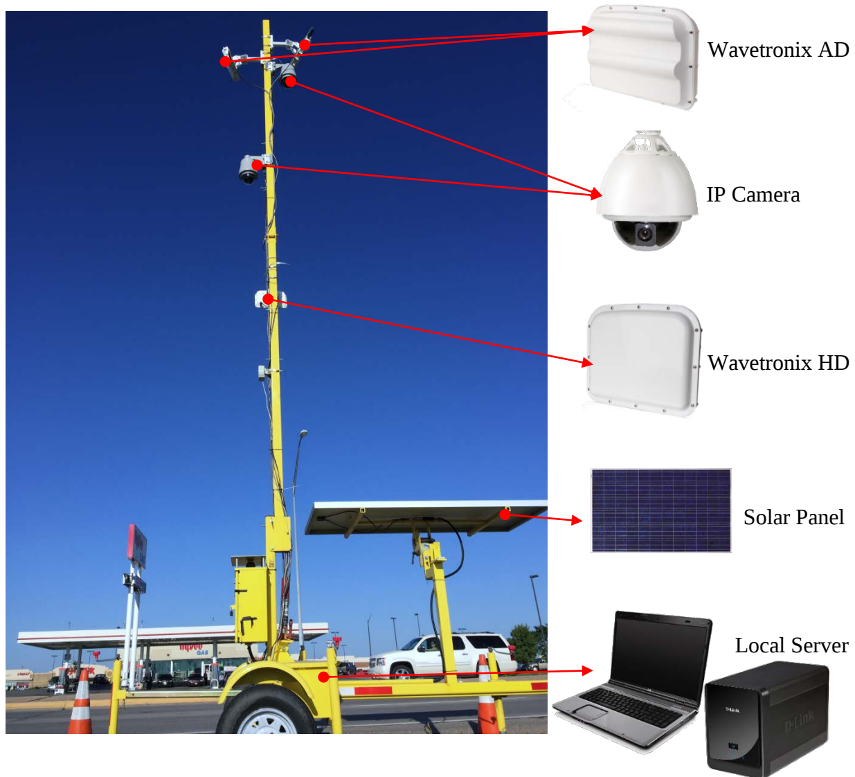
Figure 3.1 Mobile trailer data collection (MTDC) system
