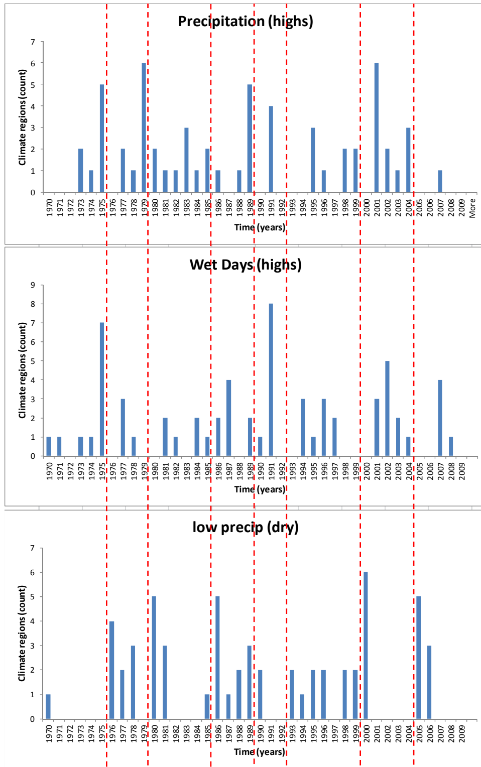
Figure 20 Selecting precipitation cycles using annual dry events
