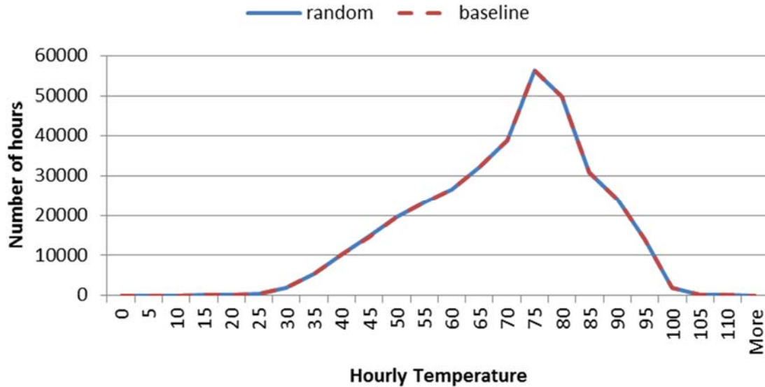
Figure 17 Comparison of historic and randomly re-sorted hourly climate data
