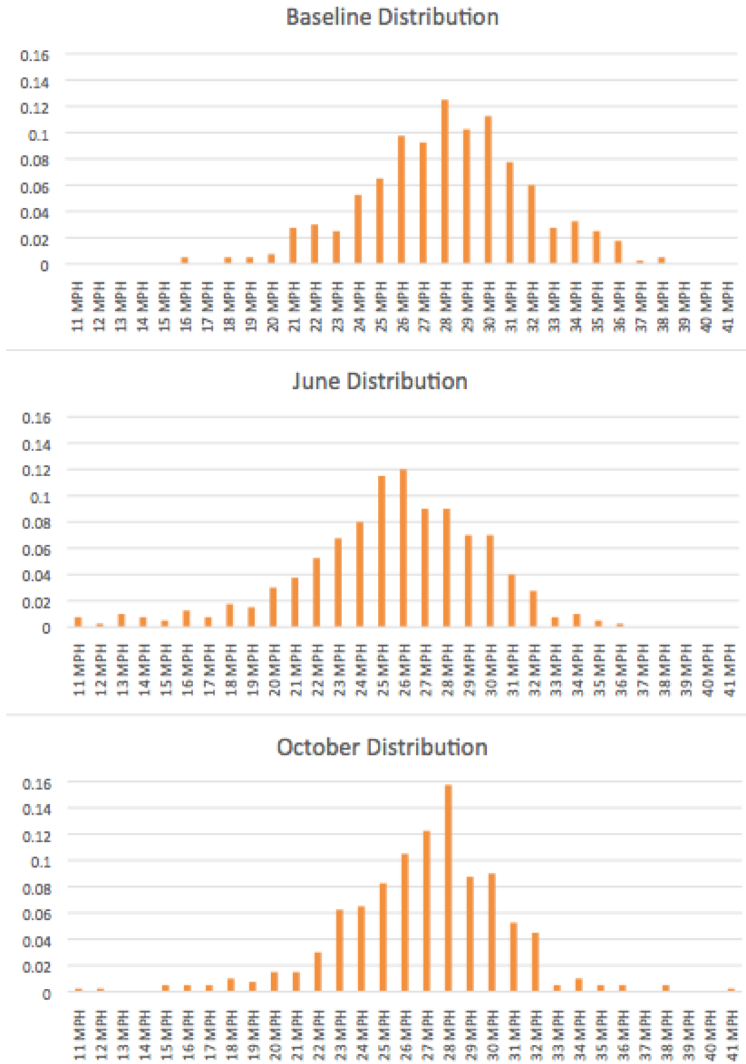
Figure 2.7. The speed distribution at the midblock crosswalk on Monroe in Allegan. The top frame shows the distribution of speeds for baseline, the middle frame shows the distribution in June and the bottom frame shows the distribution in October.
