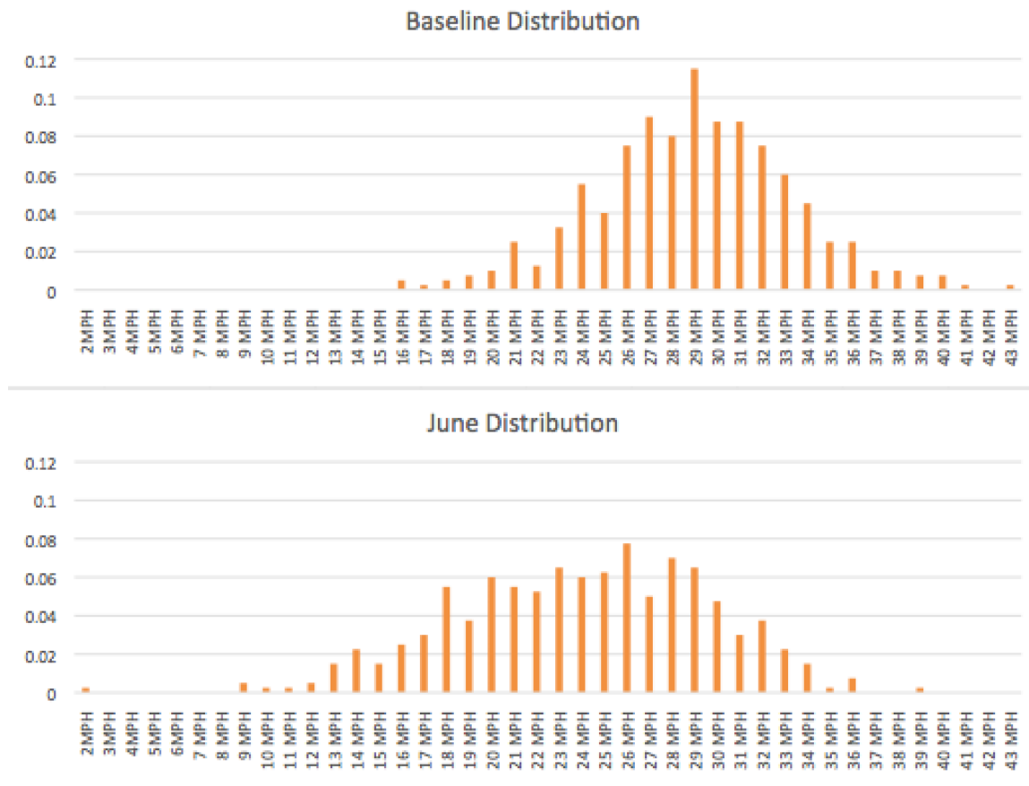
Figure 2.10. This Figure shows the speed distribution at the crosswalk on South Westnedge at Ranny. The top frame shows the distribution of speeds for baseline, the bottom frame shows the distribution in June. Two out of three gateway elements were destroyed at this site after the June speed measures. Parked cars often screened the third element.
