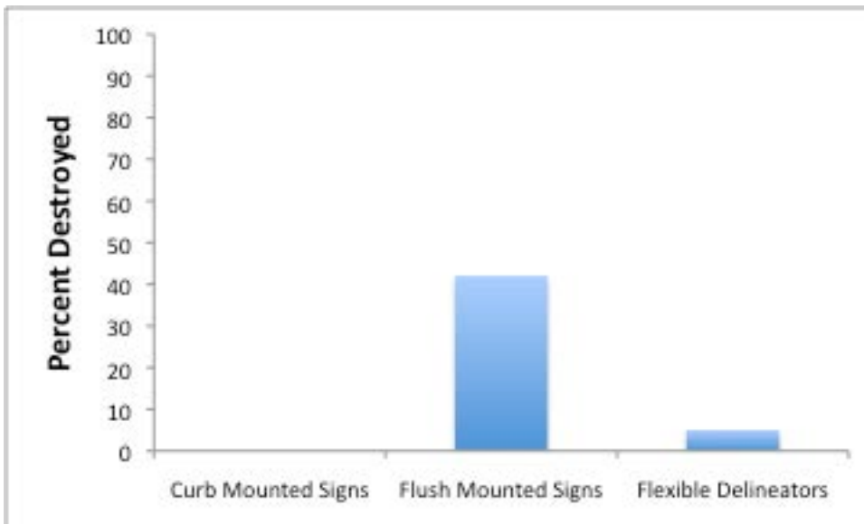
Figures 5.1. The percentage of curb type base mounted signs, flush type base mounted signs and flexible delineators destroyed in 2016 during the study period.
