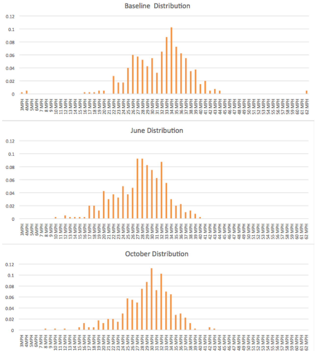
Figure 2.4. The speed distribution at the crosswalk for Stadium Drive. The top frame shows the distribution of speeds for baseline, the middle frame shows the distribution in June and the bottom frame shows the distribution in October.
