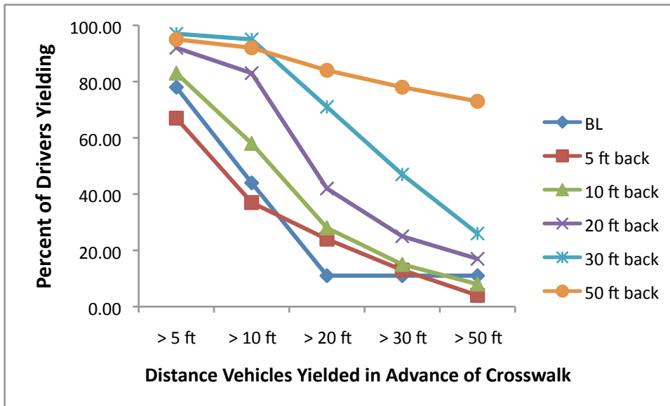
Figure 4.2. The percentage of drivers yielding greater than 5, 10, 20, 30 and 50 ft in advance of the crosswalk during Baseline, and when the gateway is placed 5, 10 20, 30 and 50 ft. in advance of the crosswalk.
