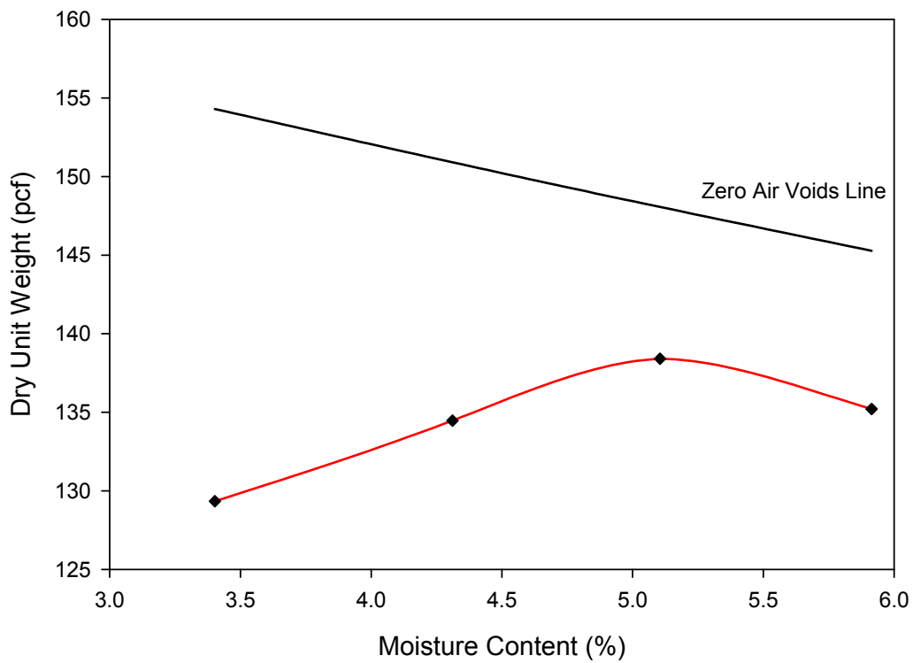
Figure C-4: Modified Proctor results for Source B Modified gradation.
