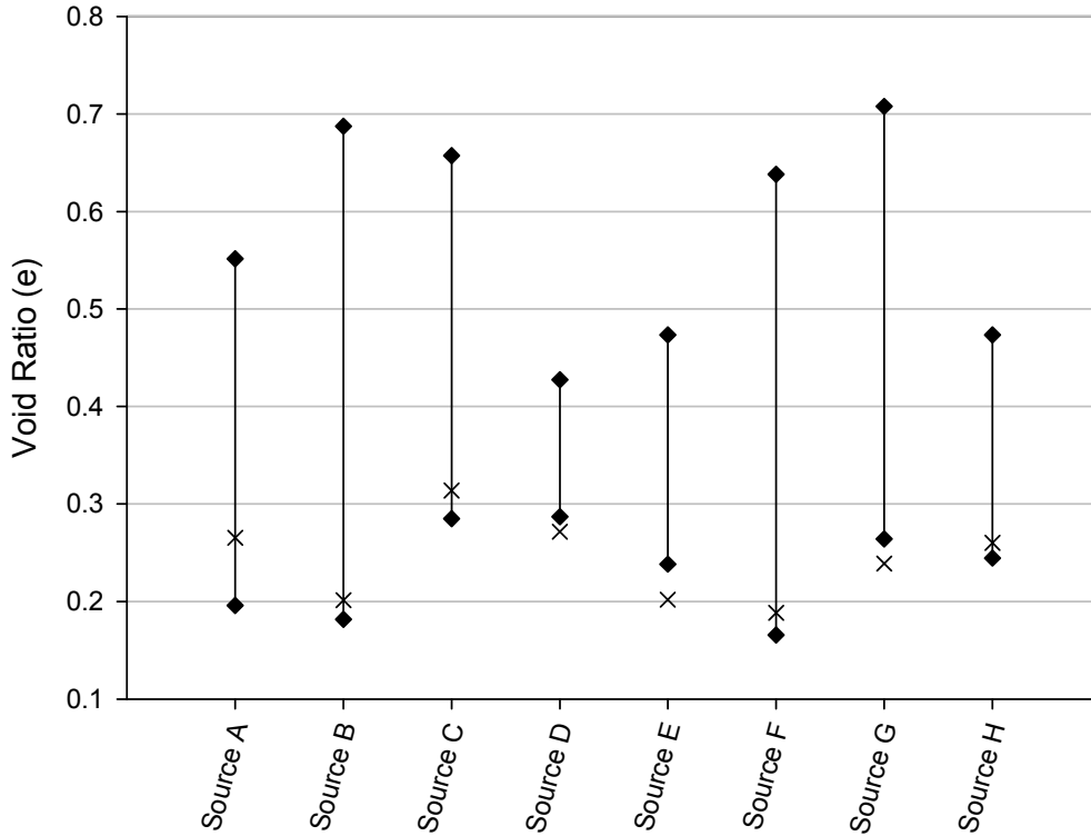
Figure 11: Proctor densities in terms of void ratio for Modified gradations.
