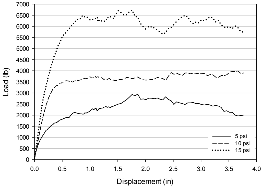
Figure E-3: Load-displacement plots from direct shear tests on Source B Prepared gradation.
