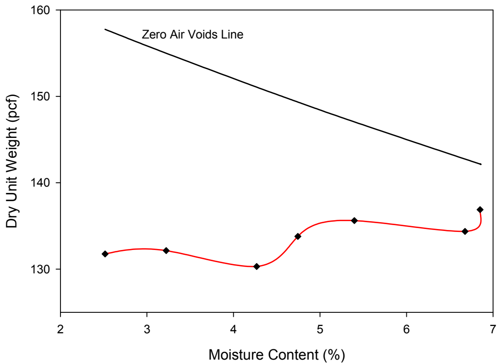
Figure C-14: Modified Proctor results for Source G Modified gradation.
