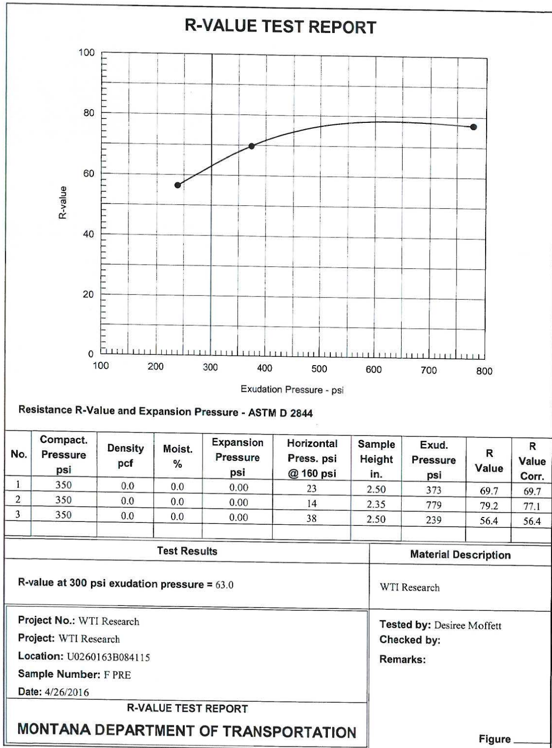
Figure D-21: R-value test report for Source F Prepared gradation.
