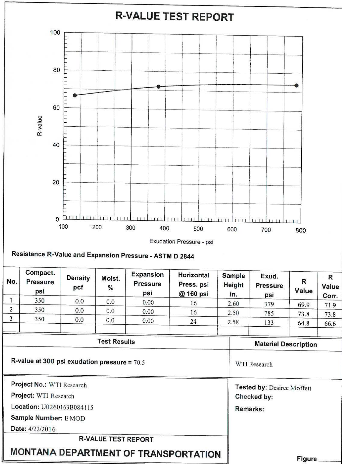
Figure D-19: R-value test report for Source E Modified gradation.
