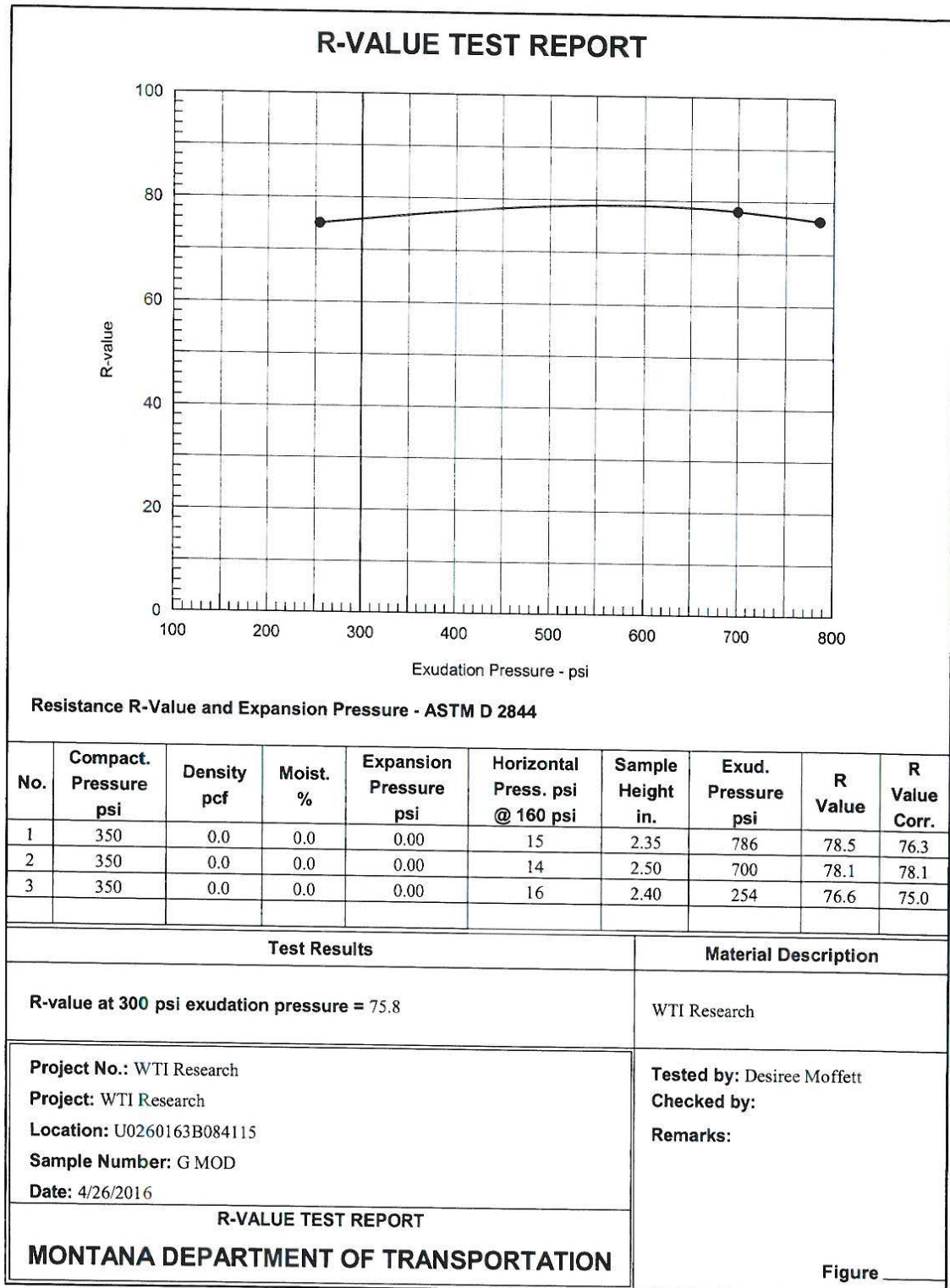
Figure D-27: R-value test report for Source G Modified gradation.
