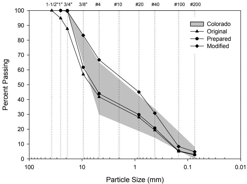
Figure B-8: Grain-size distribution of Source H gradations compared to Colorado specification.
