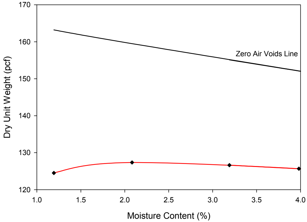
Figure C-5: Modified Proctor results for Source C Prepared gradation.
