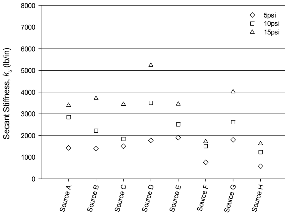
Figure 18: Ultimate secant stiffness ( k_u ) results for the Modified gradations.
