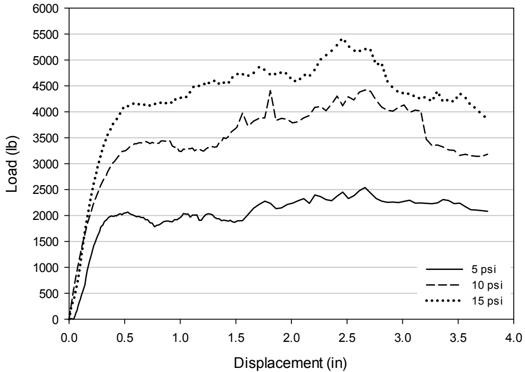
Figure E-11: Load-displacement plots from direct shear tests on Source F Prepared gradation.
