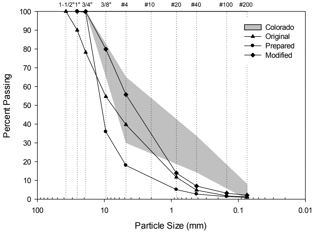
Figure B-3: Grain-size distribution of Source C gradations compared to Colorado specification.
