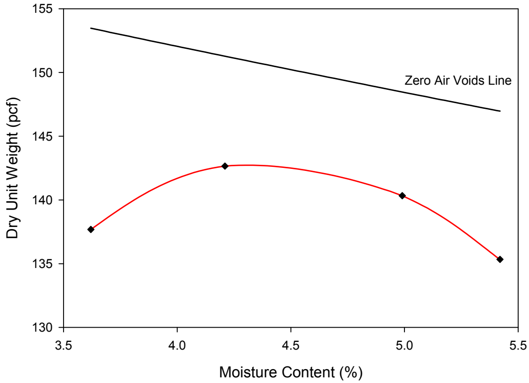
Figure C-11: Modified Proctor results for Source F Prepared gradation.
