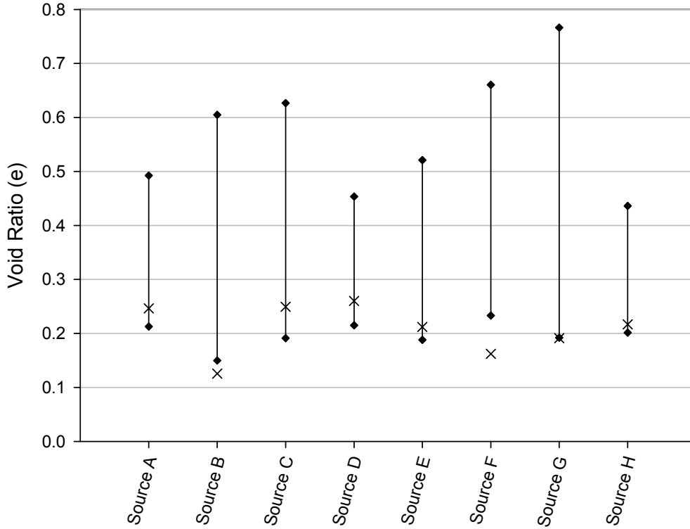
Figure 10: Proctor densities in terms of void ratio for Prepared gradations.
