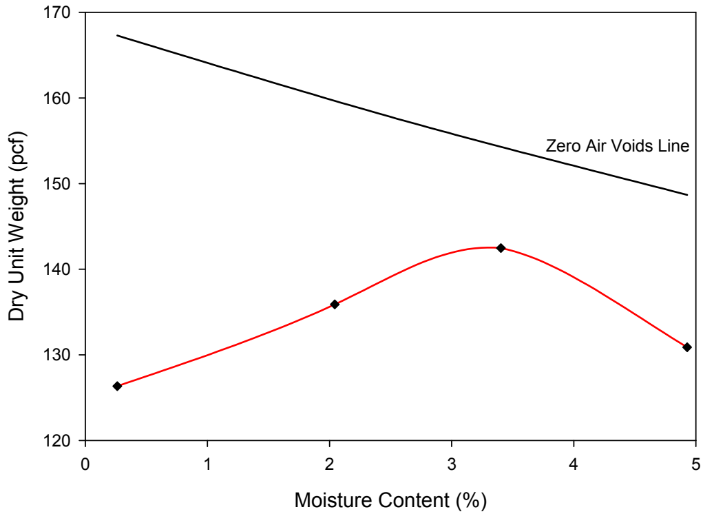
Figure C-3: Modified Proctor results for Source B Prepared gradation.
