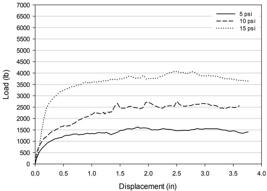
Figure E-4: Load-displacement plots from direct shear tests on Source B Modified gradation.
