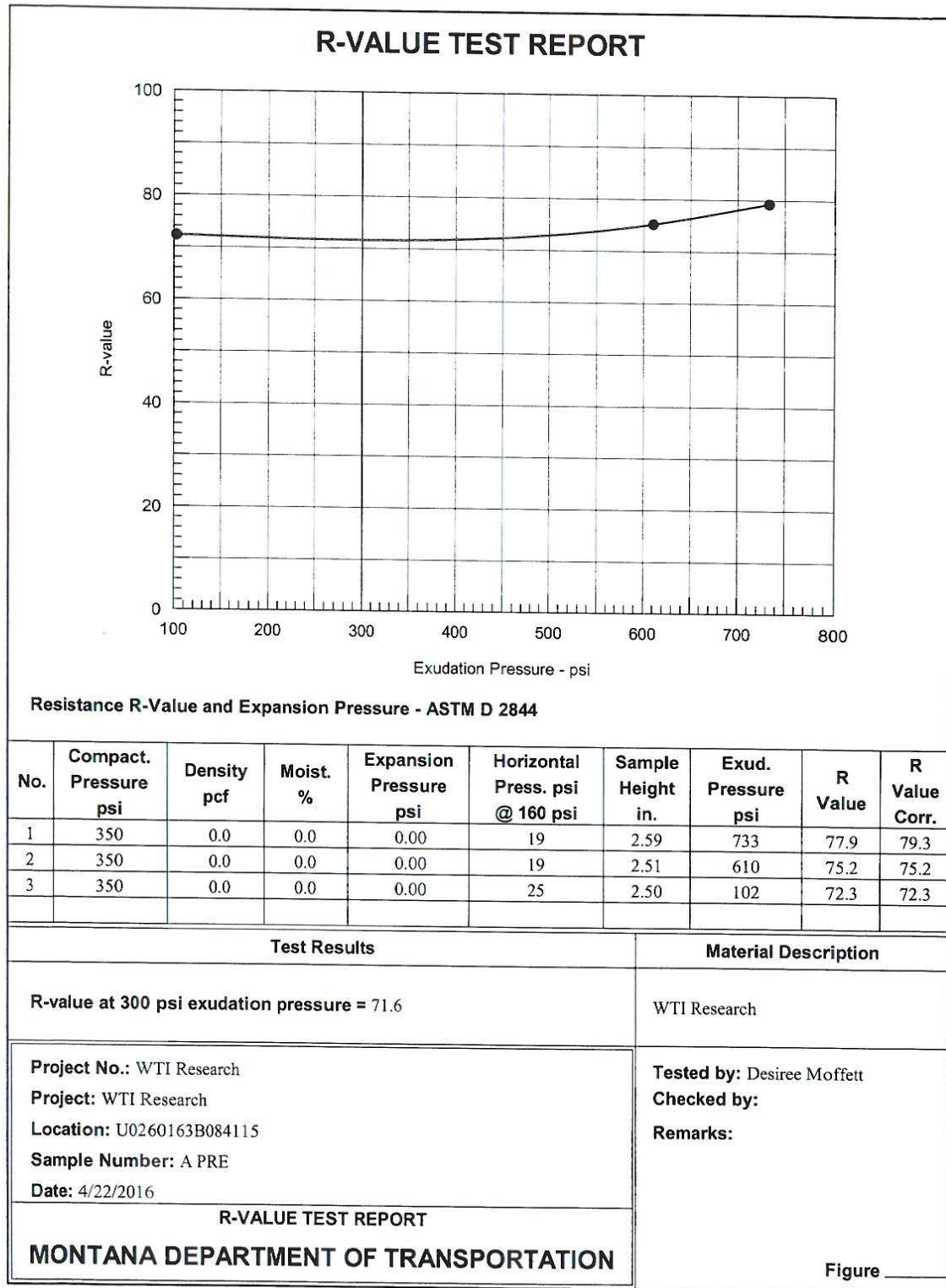
Figure D-1: R-value test report for Source A Prepared gradation.
