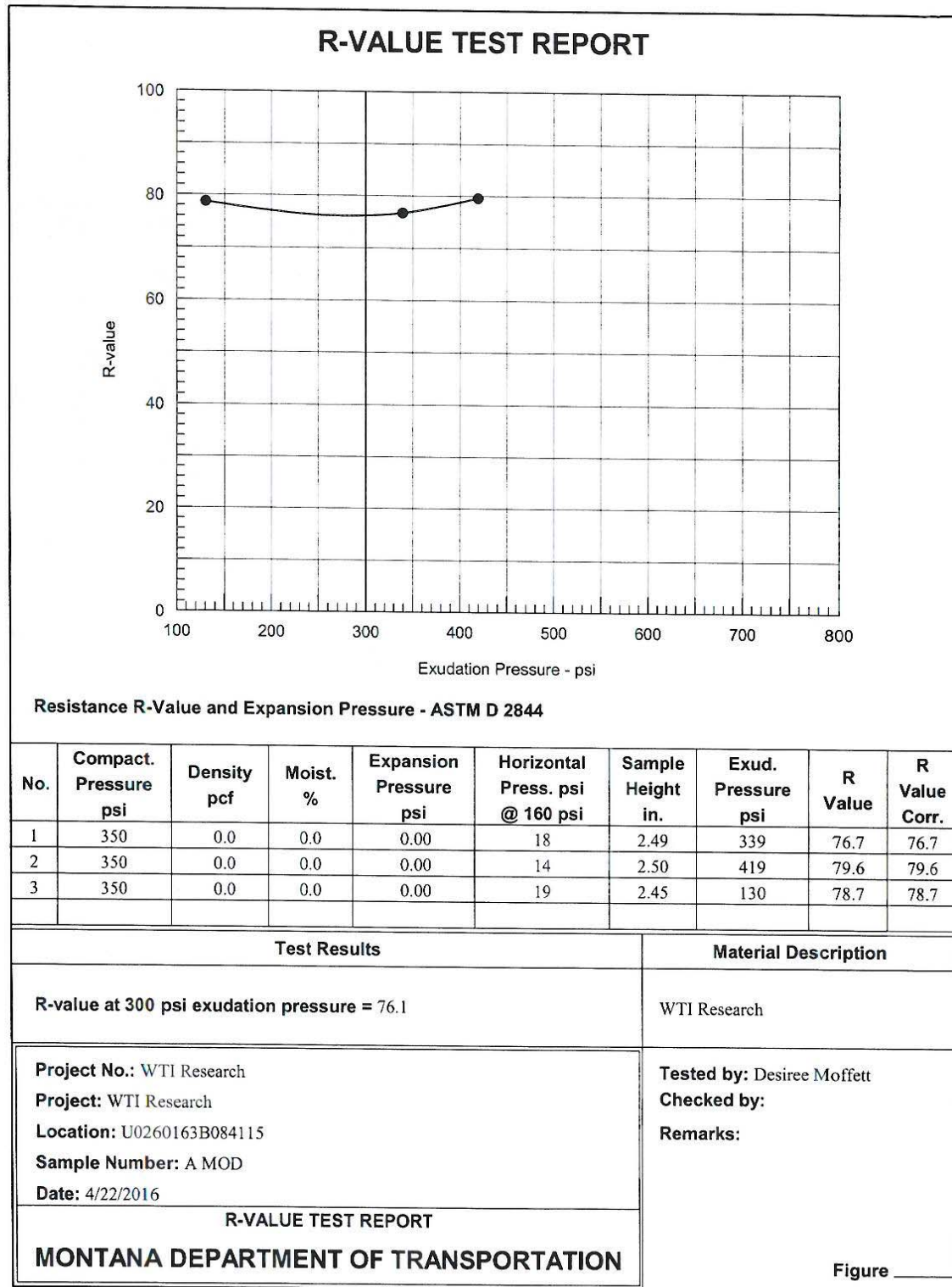
Figure D-3: R-value test report for Source A Modified gradation.
