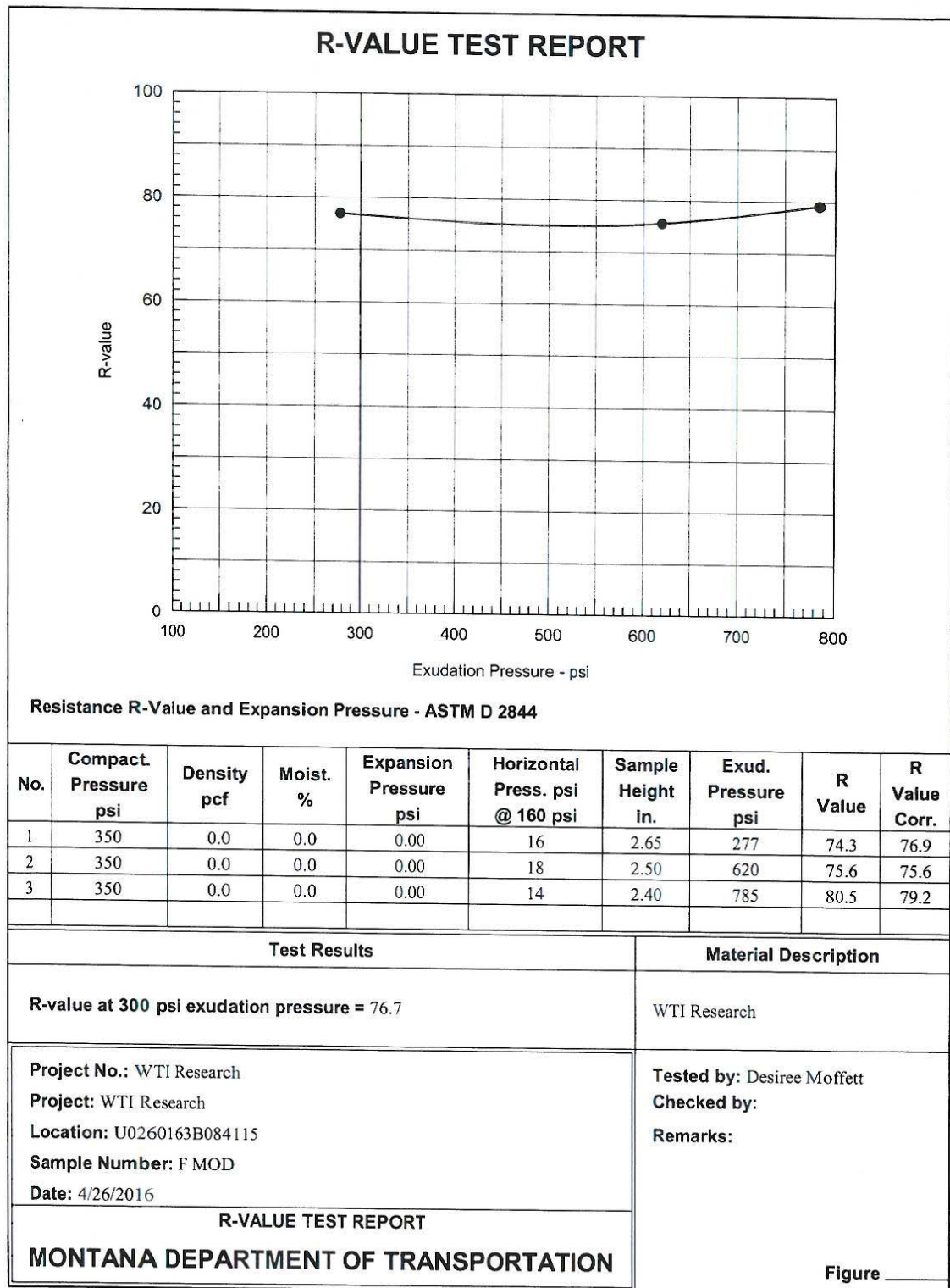
Figure D-23: R-value test report for Source F Modified gradation.
