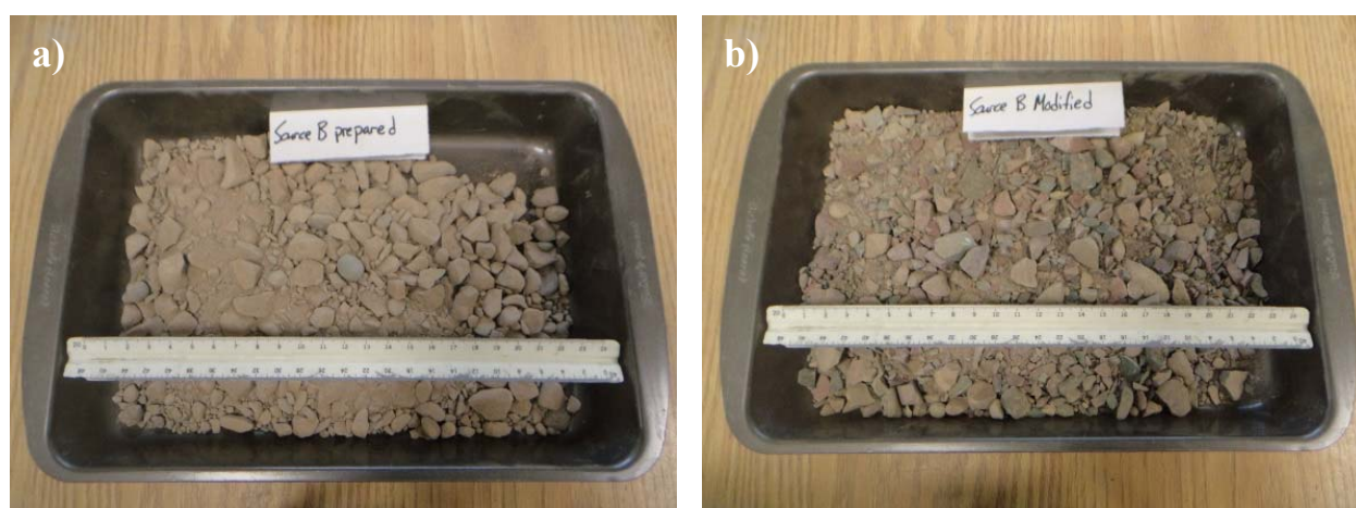
Figure A-2: Photo of Source B a) Prepared gradation and b) Modified gradation.
