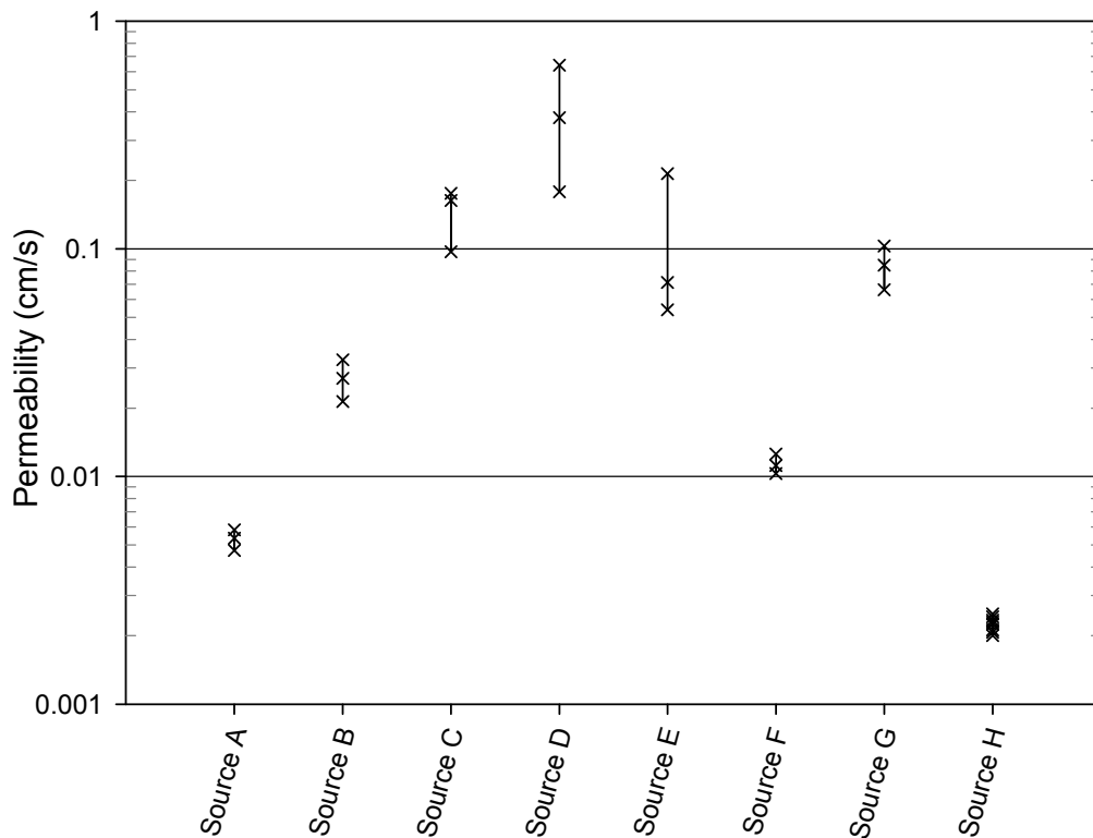
Figure 25: Permeability results of Modified gradations.
