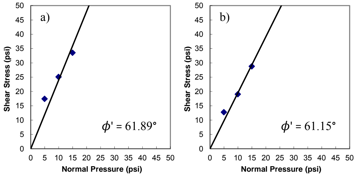
Figure F-7: Friction angle plots for Source G a) Prepared gradation and b) Modified gradation.
