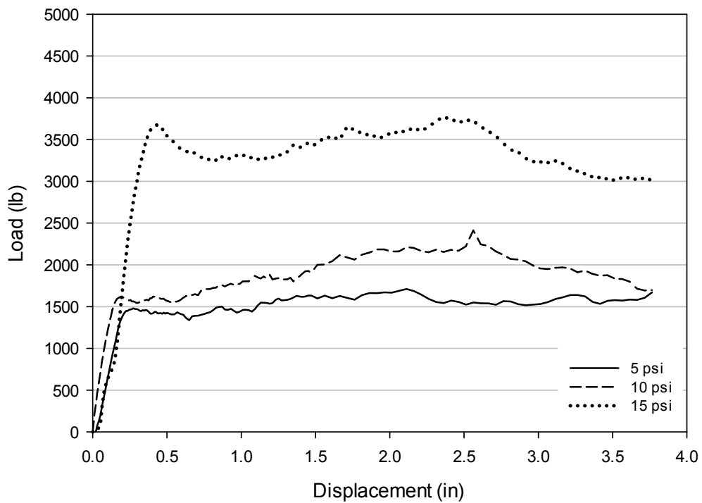
Figure E-6: Load-displacement plots from direct shear tests on Source C Modified gradation.
