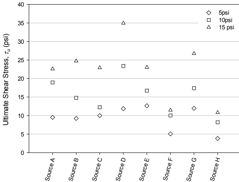
Figure 20: Ultimate shear strength ( \tau_u ) results for the Modified gradations.
