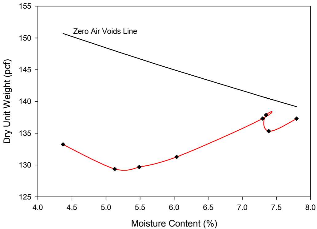
Figure C-10: Modified Proctor results for Source E Modified gradation.
