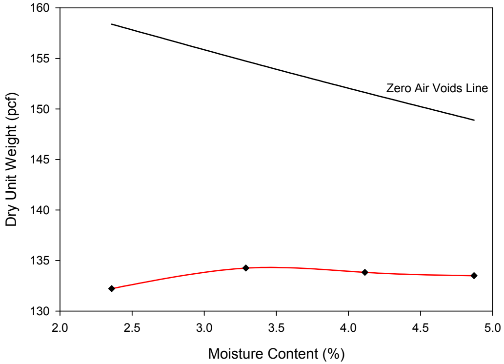
Figure C-7: Modified Proctor results for Source D Prepared gradation.
