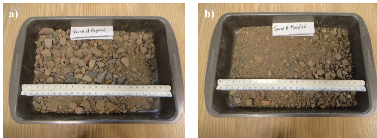
Figure A-8: Photo of Source H a) Prepared gradation and b) Modified gradation.
