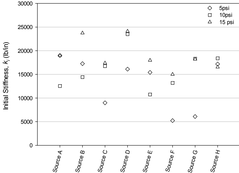
Figure 15: Initial stiffness ( k_i ) results for the Prepared gradations.
