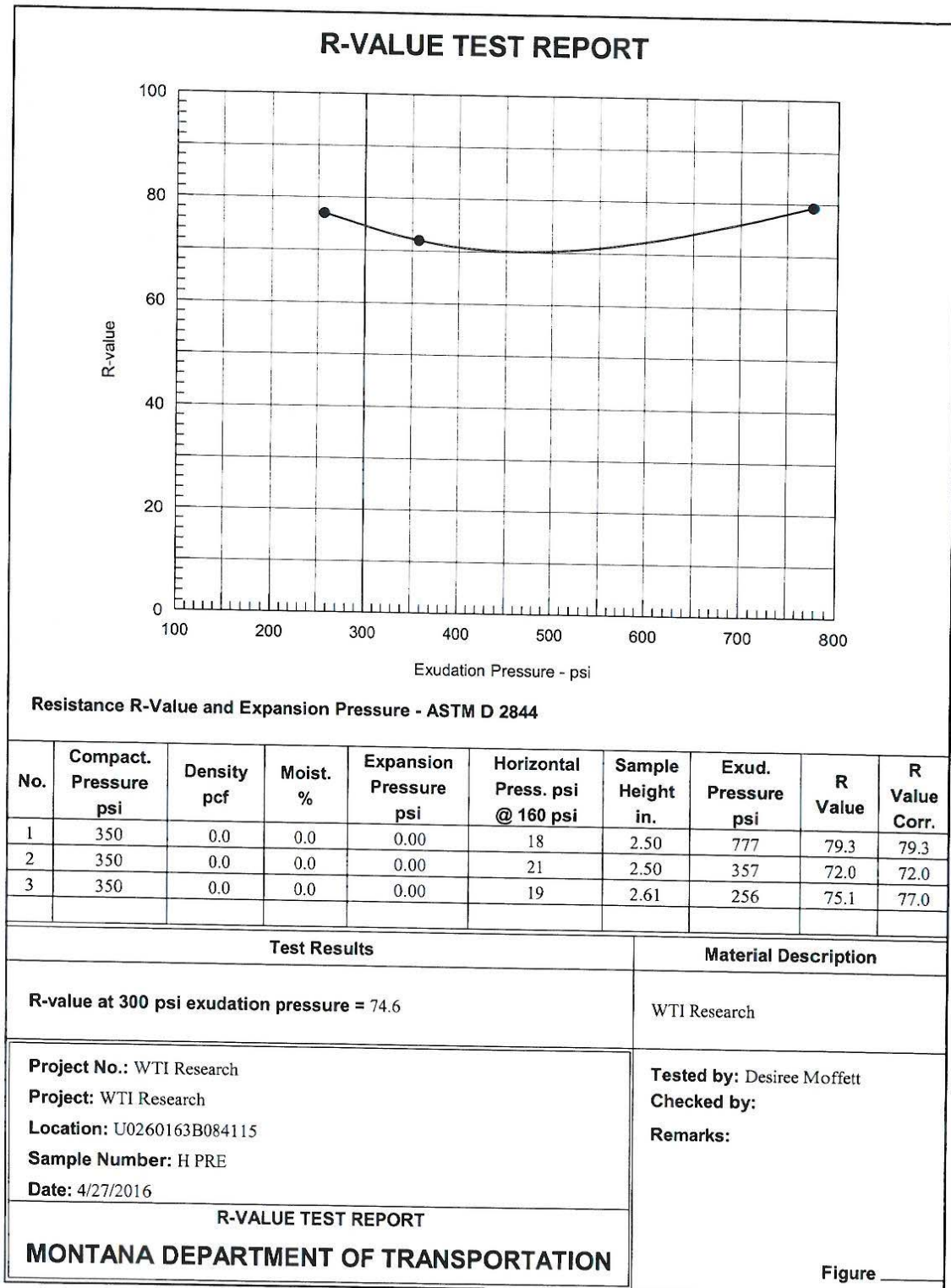
Figure D-29: R-value test report for Source H Prepared gradation.
