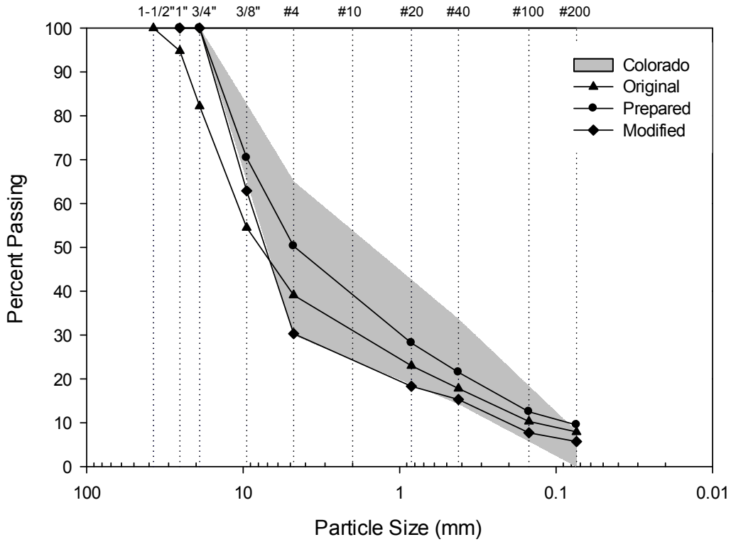
Figure B-7: Grain-size distribution of Source G gradations compared to Colorado specification.
