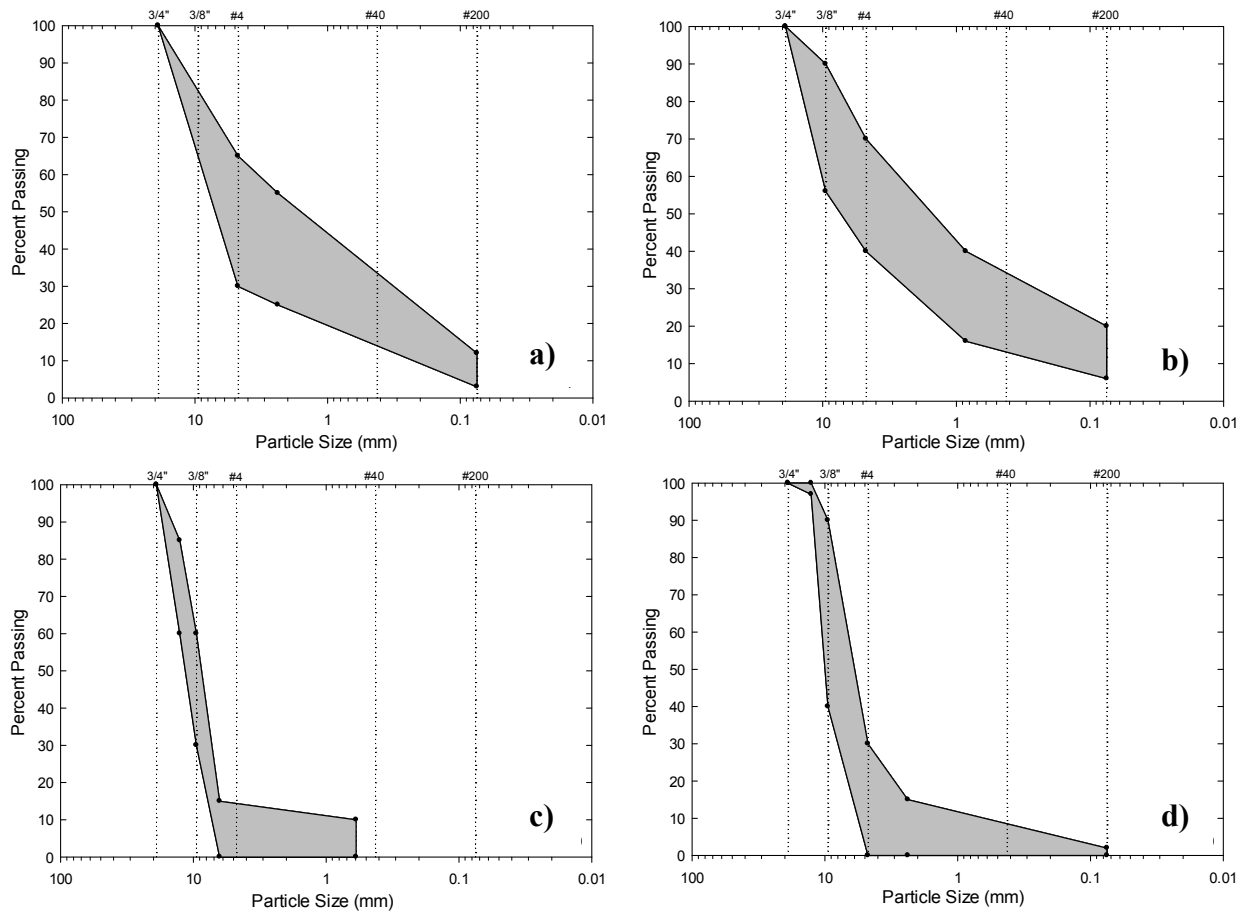
Figure 1: ¾-inch minus specification ranges for a) Colorado, b) Nebraska, c) Indiana and d) Iowa.
