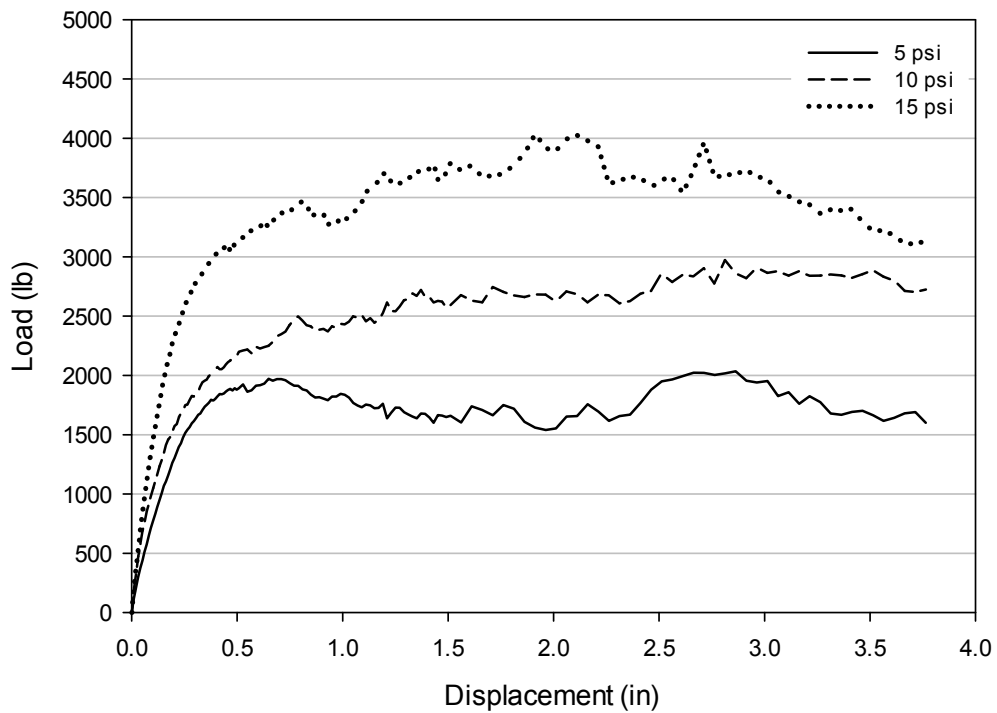
Figure E-10: Load-displacement plots from direct shear tests on Source E Modified gradation.
