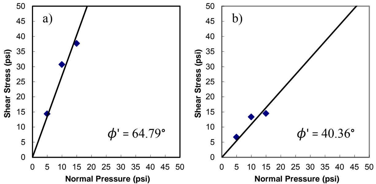
Figure F-6: Friction angle plots for Source F a) Prepared gradation and b) Modified gradation.
