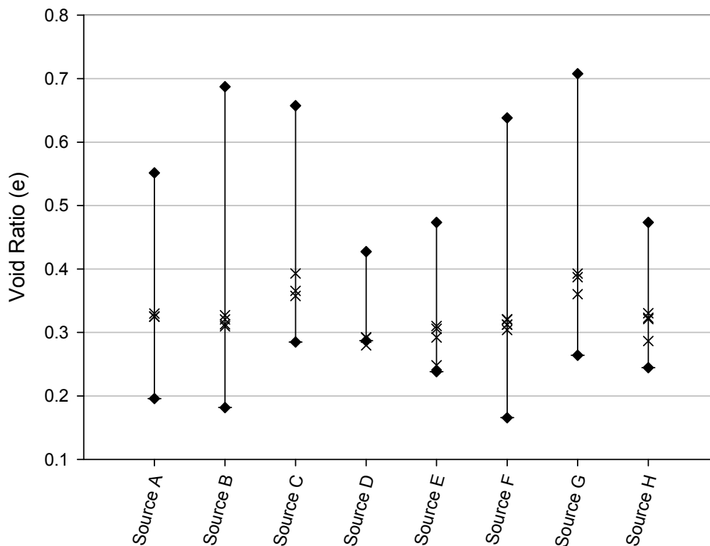
Figure 14: Direct shear densities for Modified gradations.
