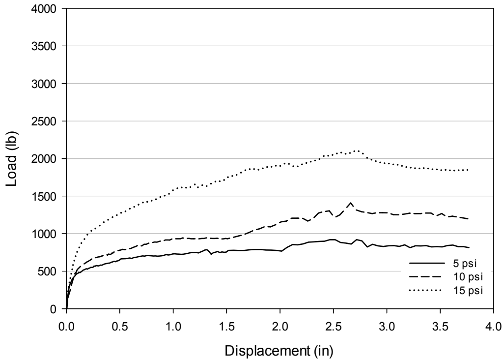
Figure E-1: Load-displacement plots from direct shear tests on Source A Prepared gradation.
