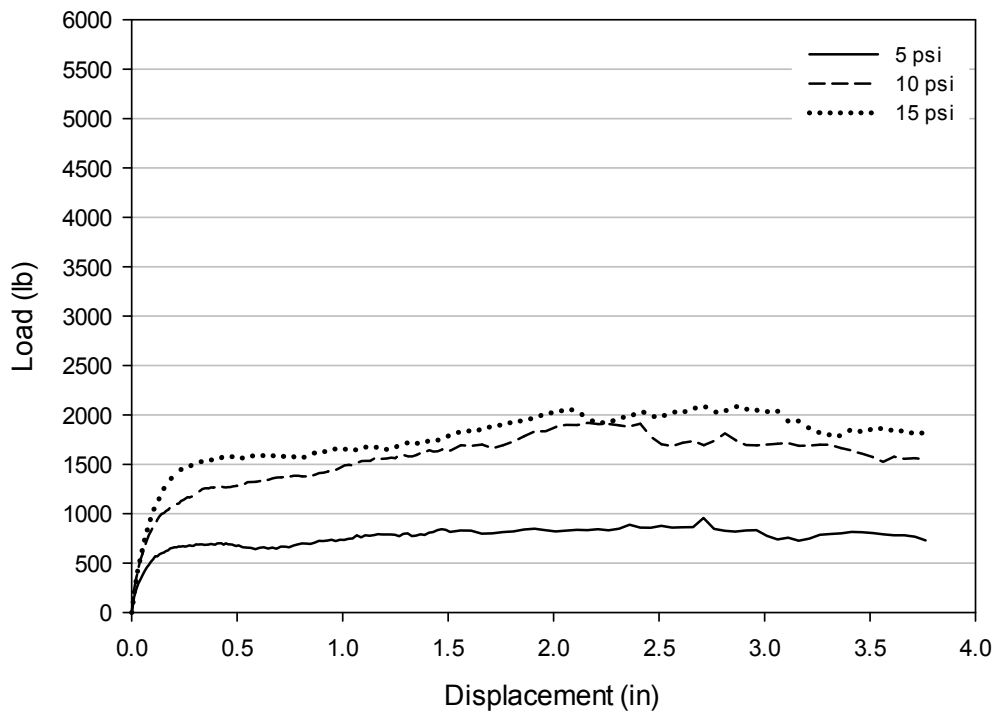
Figure E-12: Load-displacement plots from direct shear tests on Source F Modified gradation.
