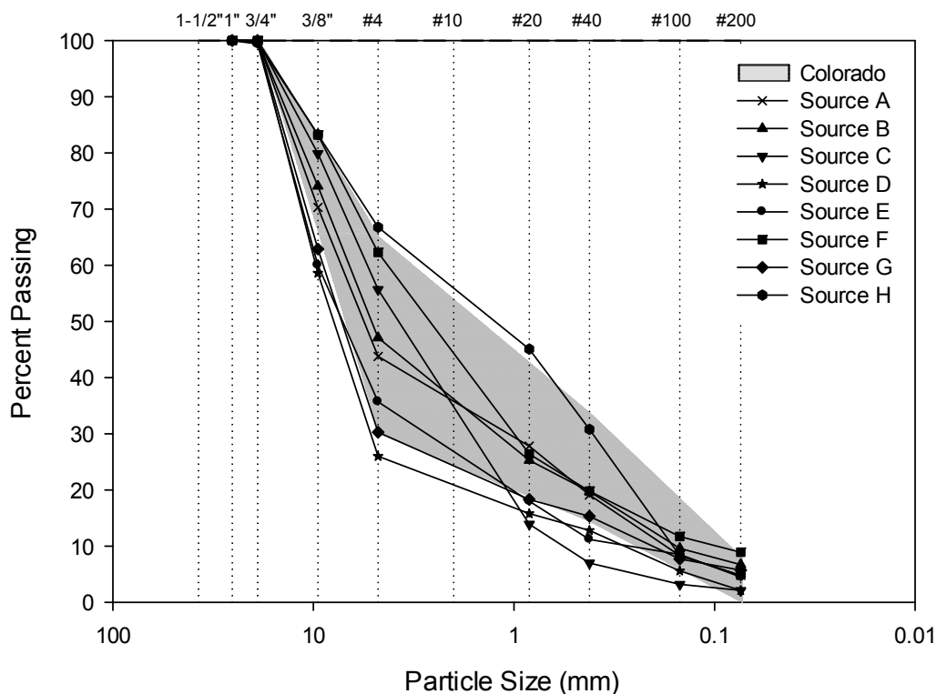
Figure 7: Sieve analysis results of Modified gradations with respect to Colorado specification limits.
