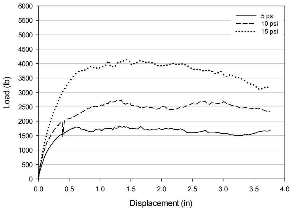
Figure E-14: Load-displacement plots from direct shear tests on Source G Modified gradation.
