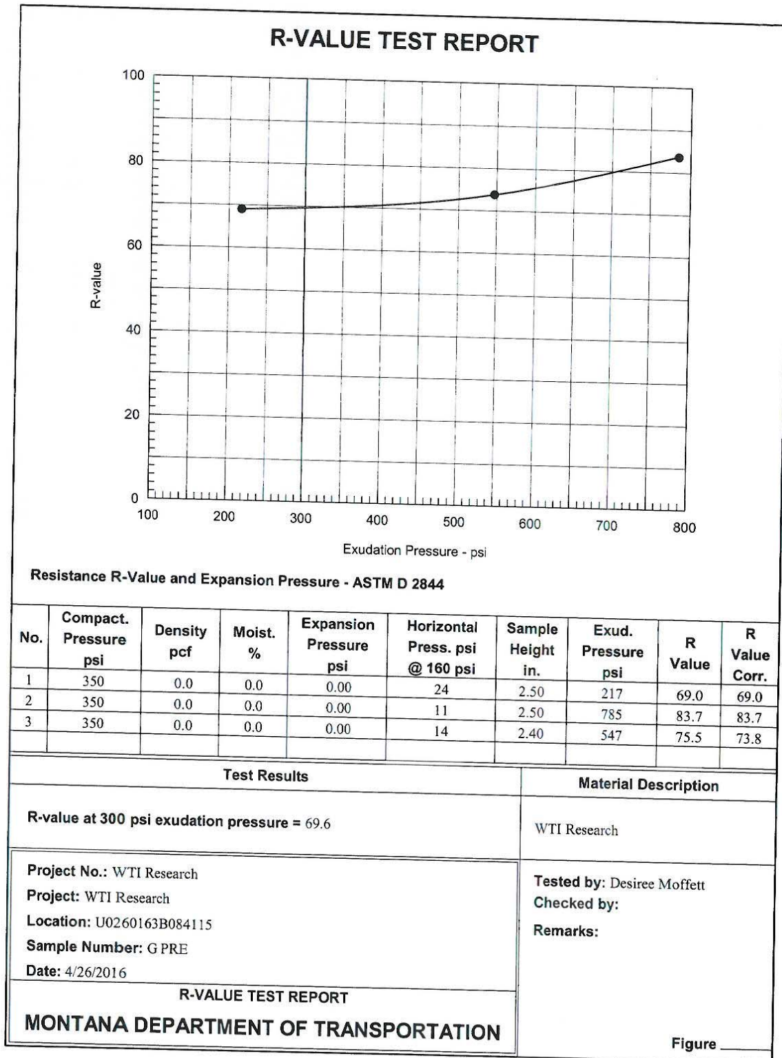
Figure D-25: R-value test report for Source G Prepared gradation.
