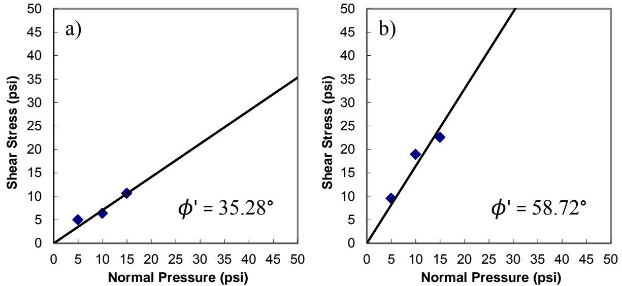
Figure F-1: Friction angle plots for Source A a) Prepared gradation and b) Modified gradation.
