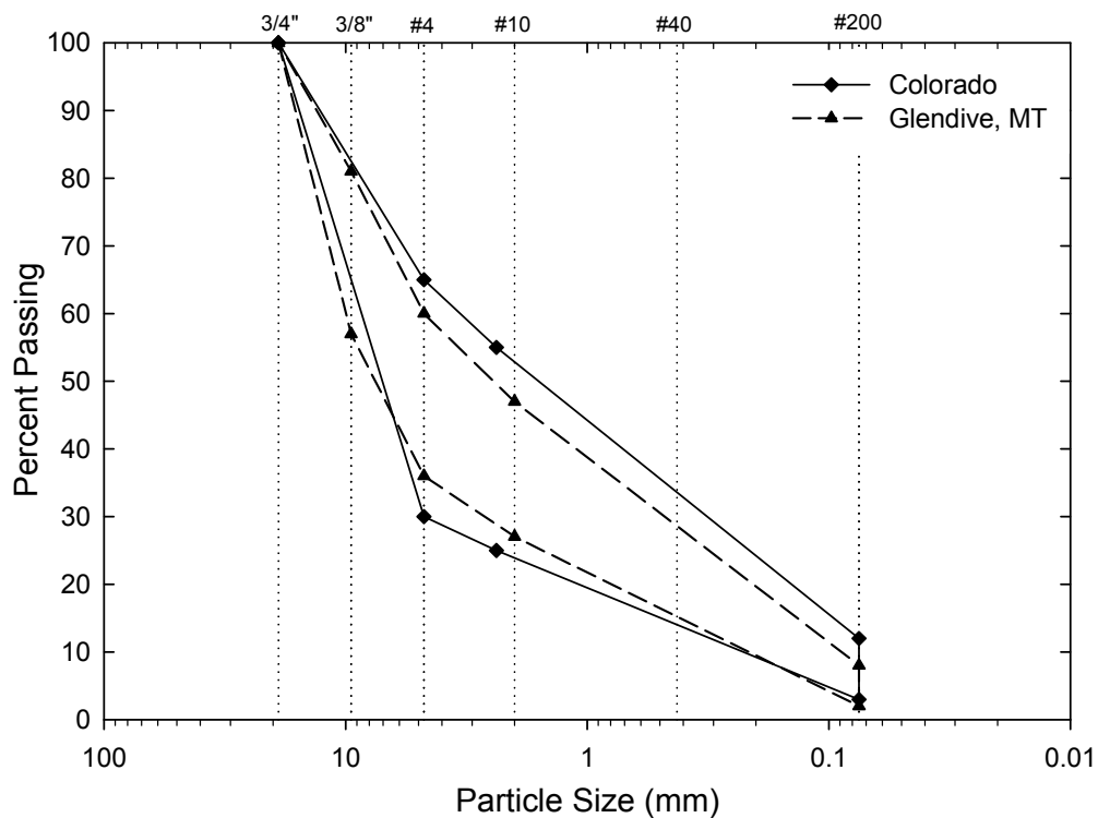
Figure 26: 3/4-inch minus specifications for Colorado and Glendive, MT.
