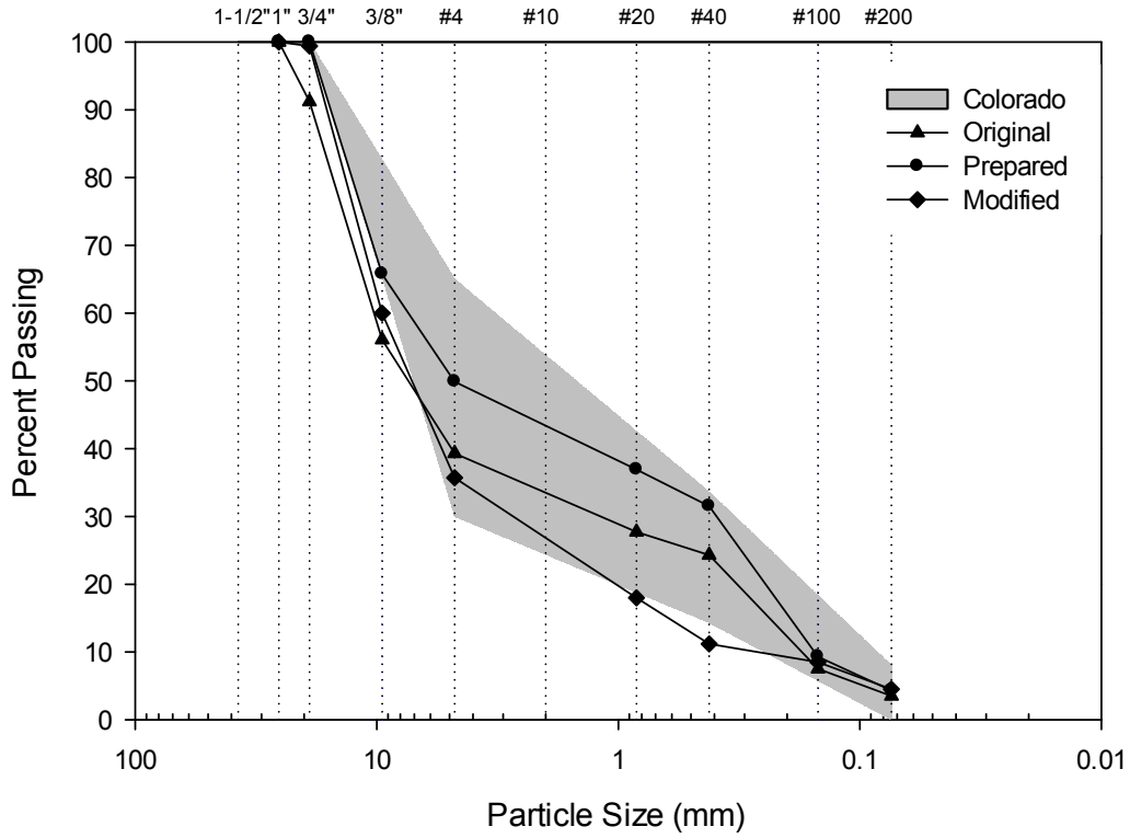
Figure B-5: Grain-size distribution of Source E gradations compared to Colorado specification.
