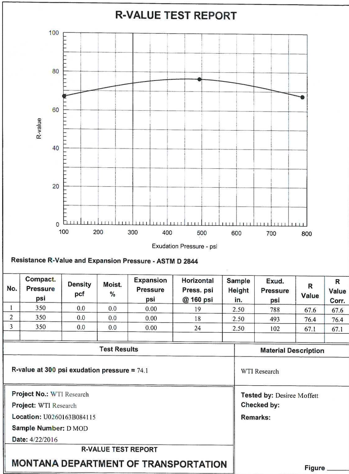
Figure D-15: R-value test report for Source D Modified gradation.
