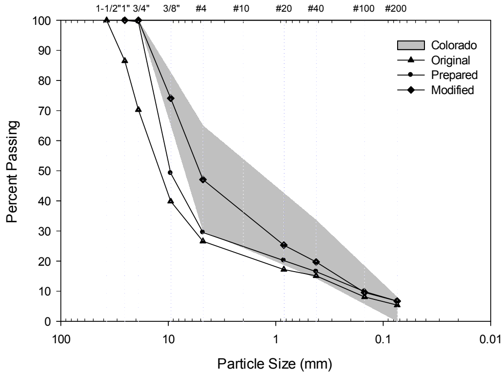
Figure B-2: Grain-size distribution of Source B gradations compared to Colorado specification.
