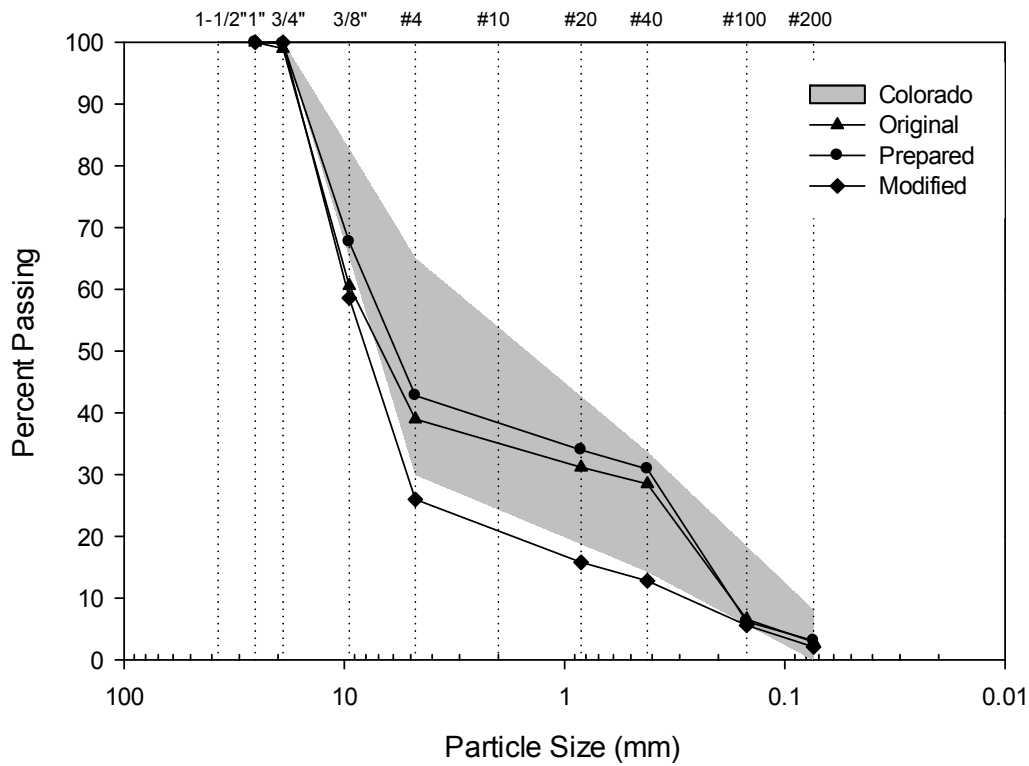
Figure B-4: Grain-size distribution of Source D gradations compared to Colorado specification.
