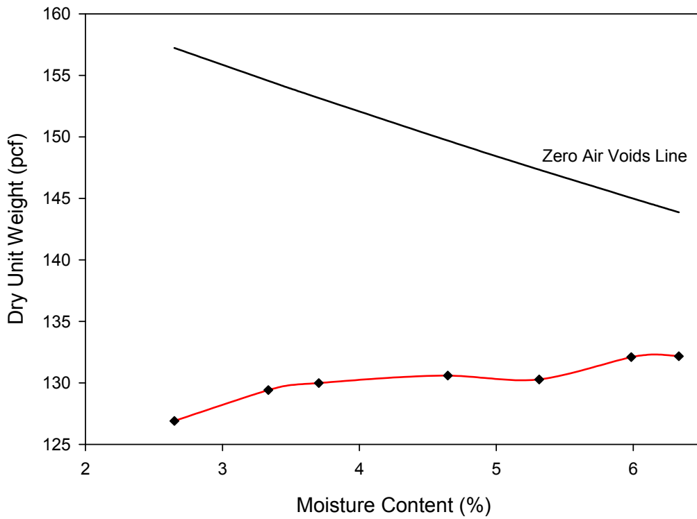
Figure C-8: Modified Proctor results for Source D Modified gradation.
