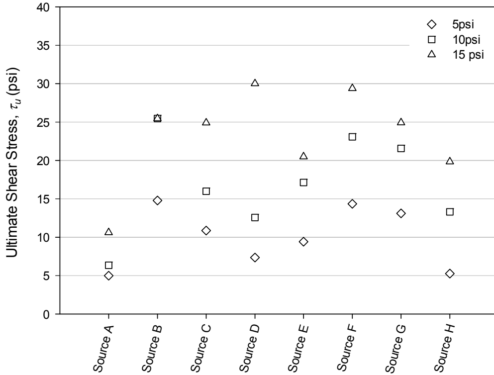
Figure 19: Ultimate shear strength ( \tau_u ) results for the Prepared gradations.
