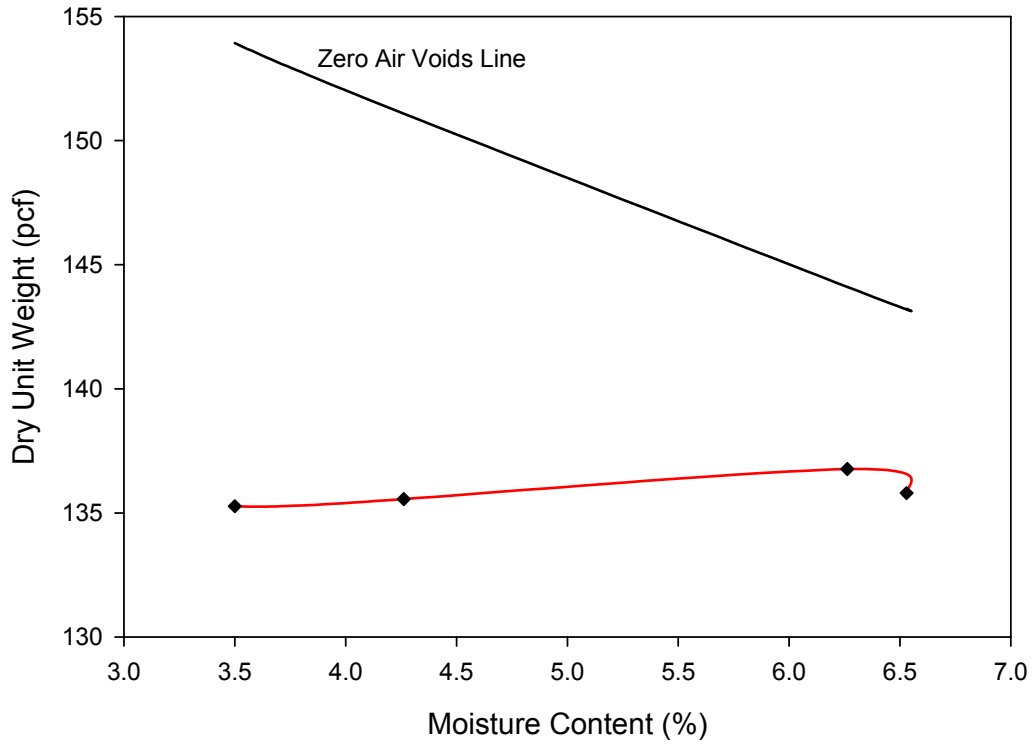
Figure C-15: Modified Proctor results for Source H Prepared gradation.
