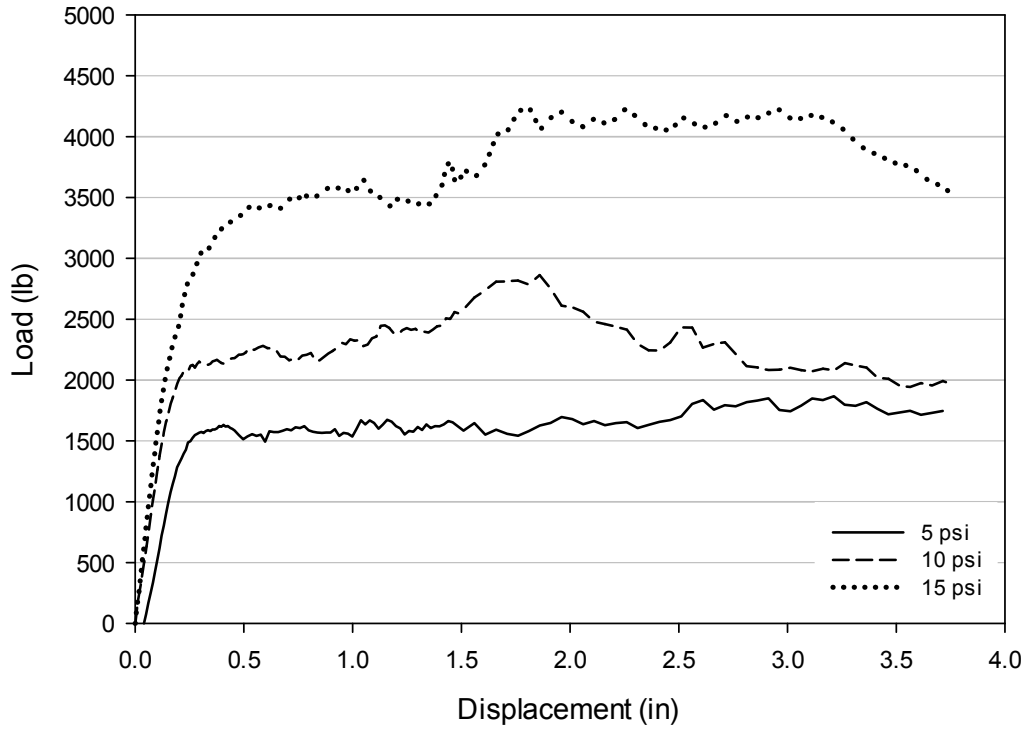
Figure E-5: Load-displacement plots from direct shear tests on Source C Prepared gradation.
