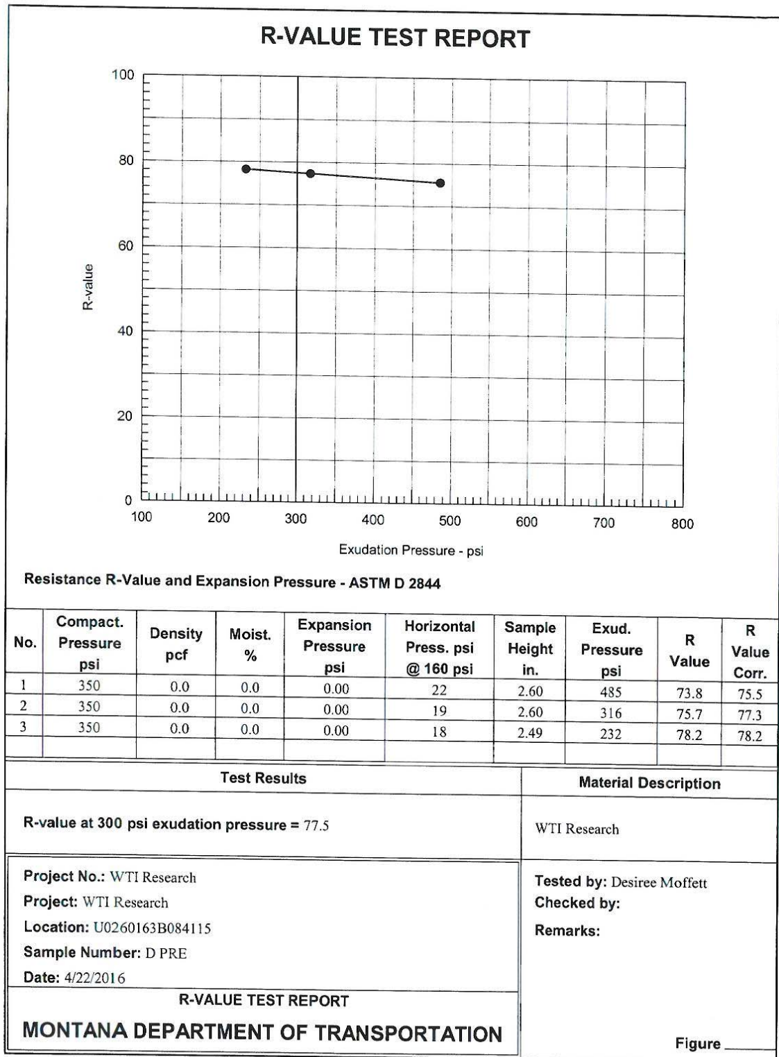
Figure D-13: R-value test report for Source D Prepared gradation.
