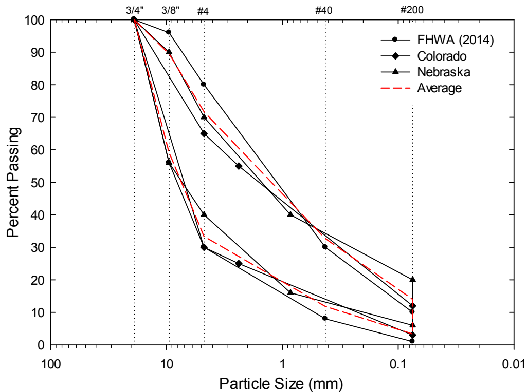
Figure 2: 2014 FHWA, Colorado, Nebraska, and average base course specifications.
