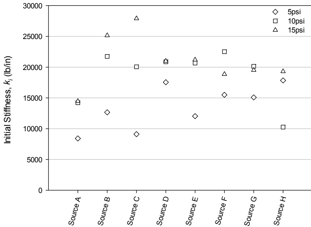
Figure 16: Initial stiffness ( k_i ) results for the Modified gradations.
