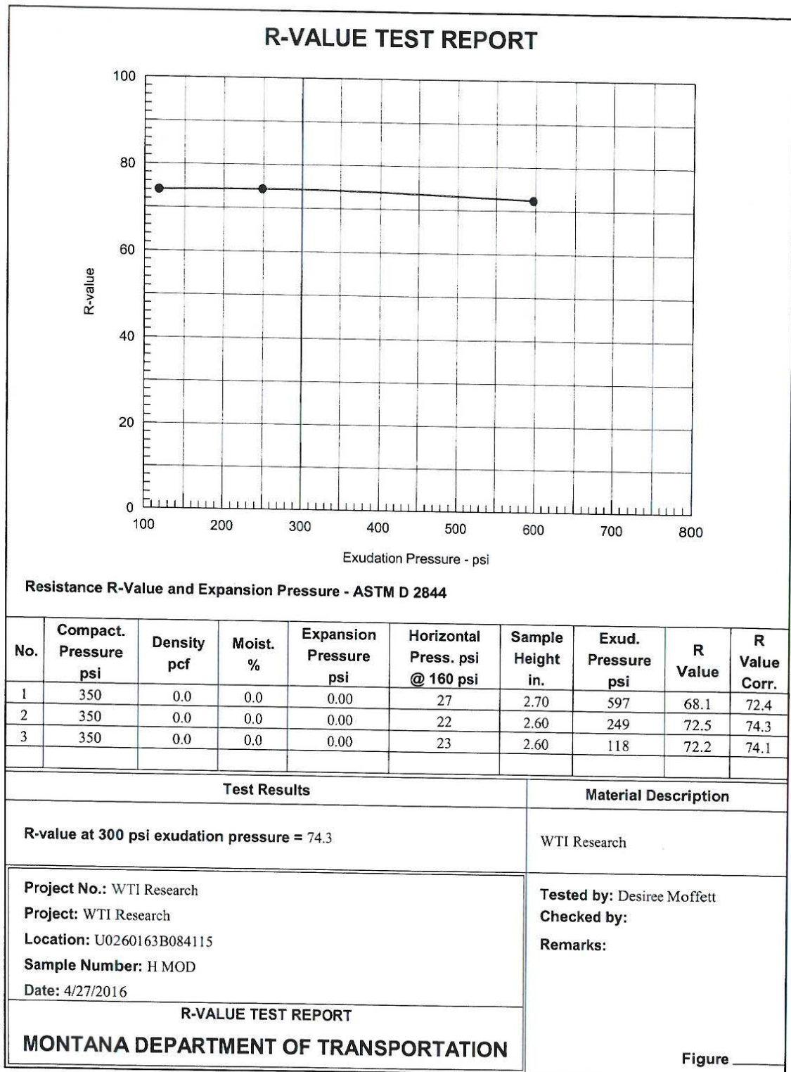
Figure D-31: R-value test report for Source H Modified gradation.
