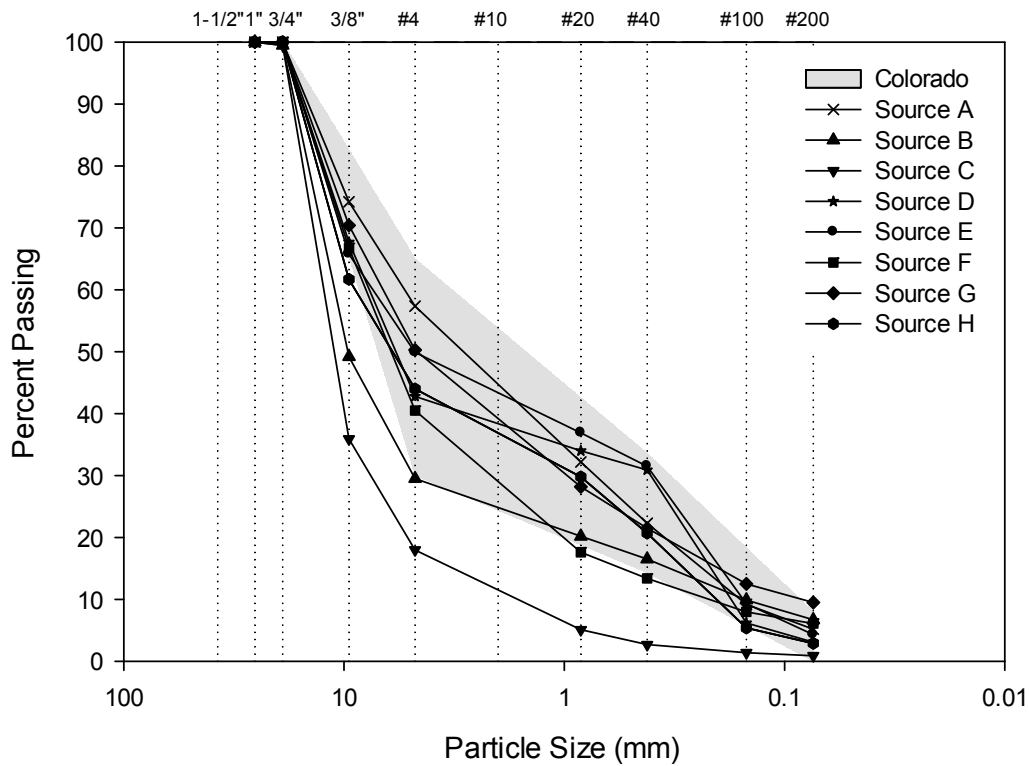
Figure 6: Sieve analysis results of Prepared gradations with respect to Colorado specification limits.
