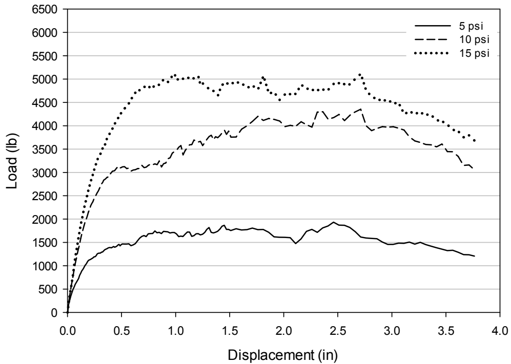
Figure E-8: Load-displacement plots from direct shear tests on Source D Modified gradation.
