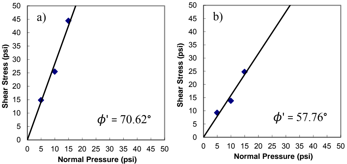
Figure F-2: Friction angle plots for Source B a) Prepared gradation and b) Modified gradation.
