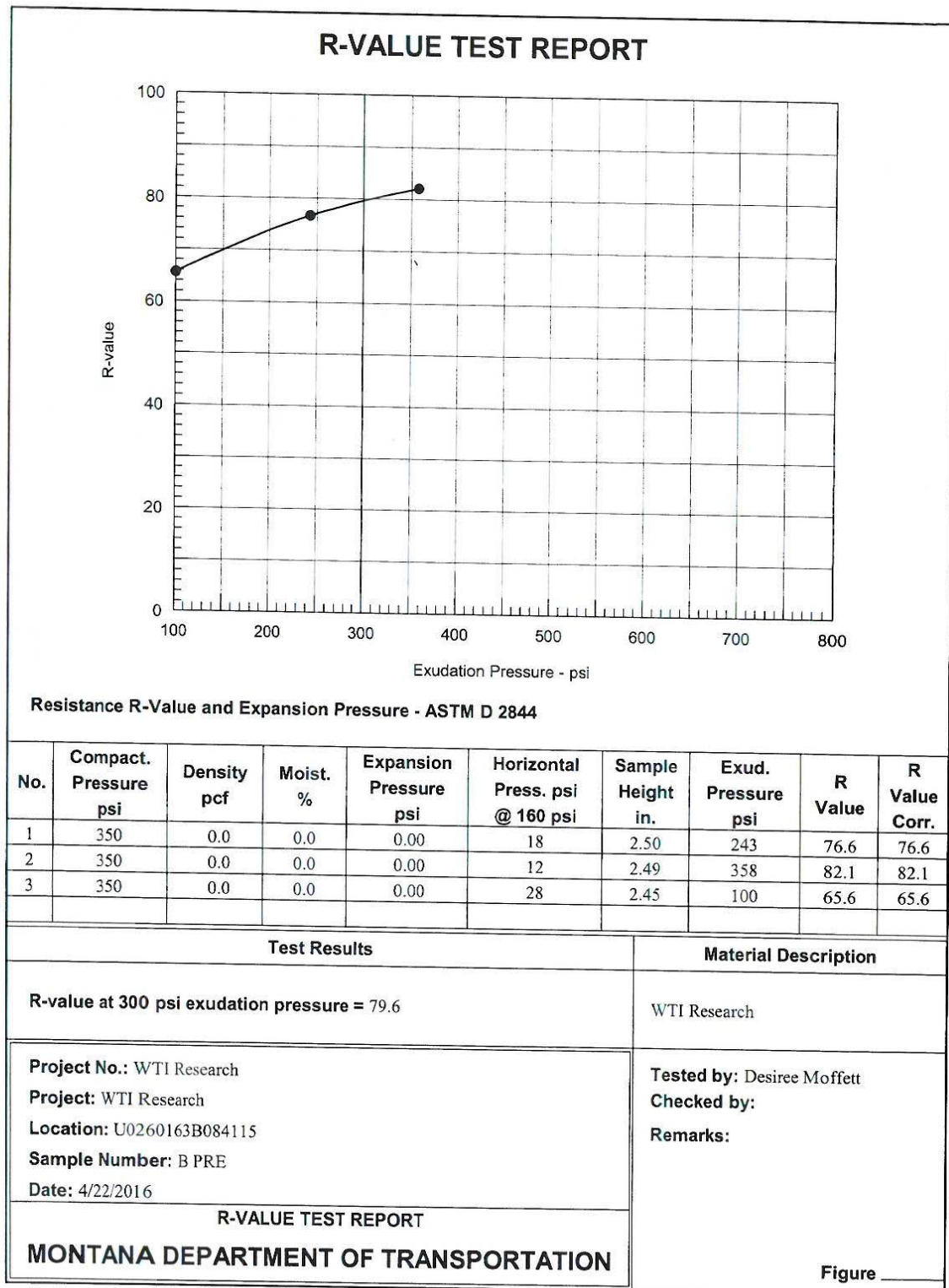
Figure D-5: R-value test report for Source B Prepared gradation.
