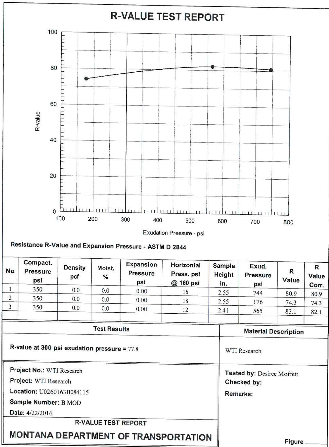
Figure D-7: R-value test report for Source B Modified gradation.
