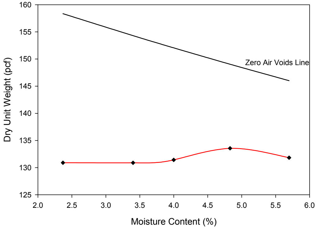
Figure C-1: Modified Proctor results for Source A Prepared gradation.
