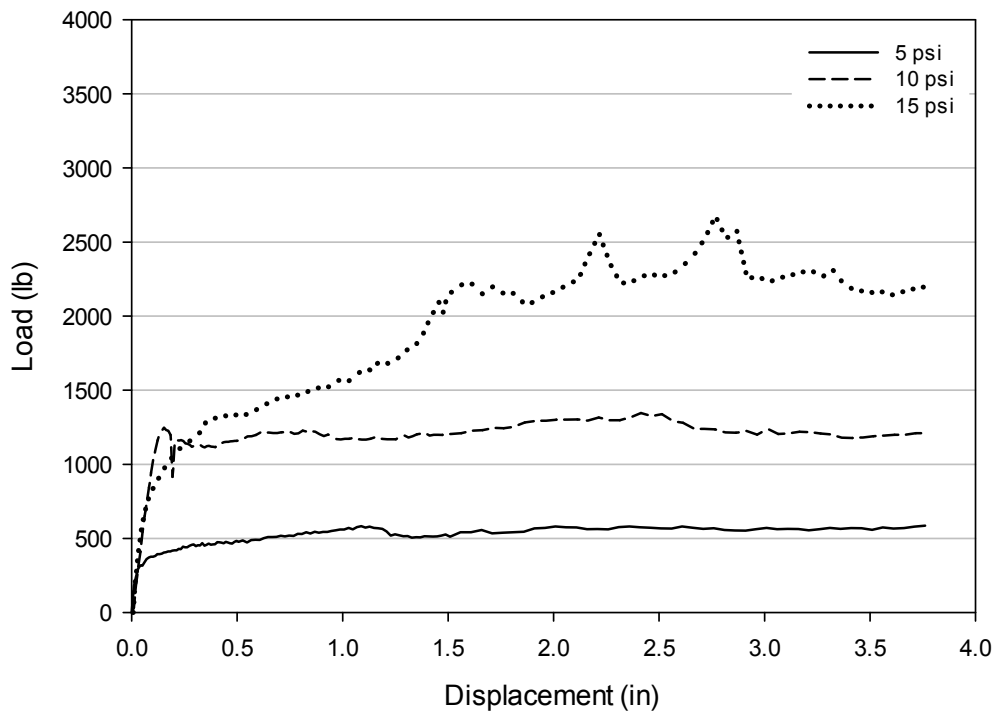
Figure E-16: Load-displacement plots from direct shear tests on Source H Modified gradation.
