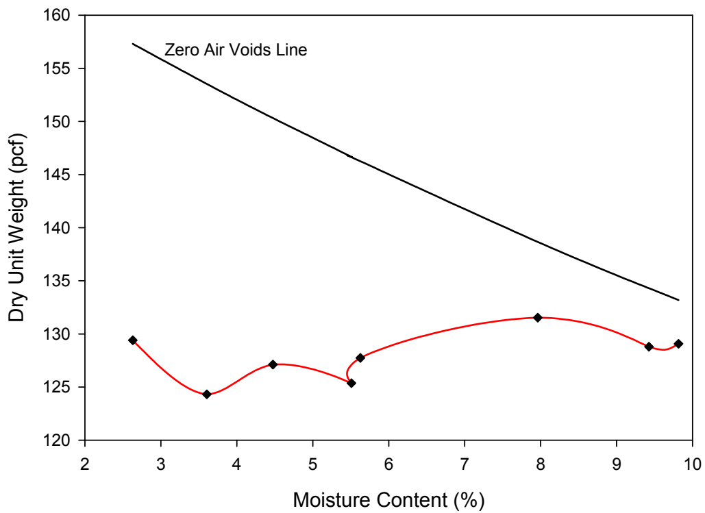
Figure C-16: Modified Proctor results for Source H Modified gradation.
