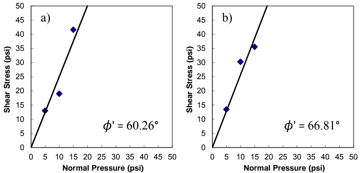
Figure F-4: Friction angle plots for Source D a) Prepared gradation and b) Modified gradation.
