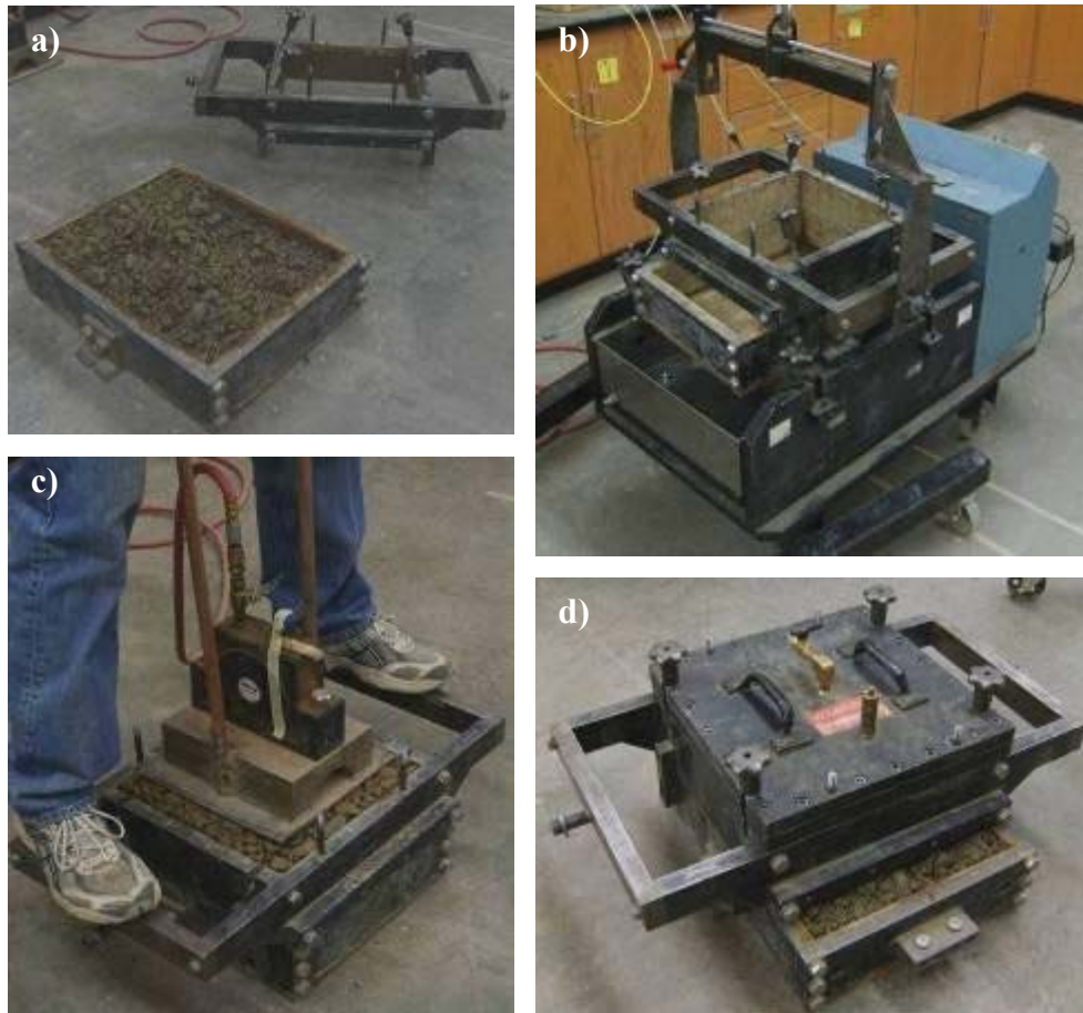
Figure 12: Direct shear testing apparatus a) mold halves, b) mold placed in load frame, c) vibratory compactor, and d) assembled mold halves with air bladder and cover plate attached to top.
