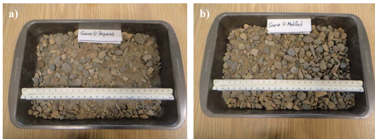
Figure A-4: Photo of Source D a) Prepared gradation and b) Modified gradation.
