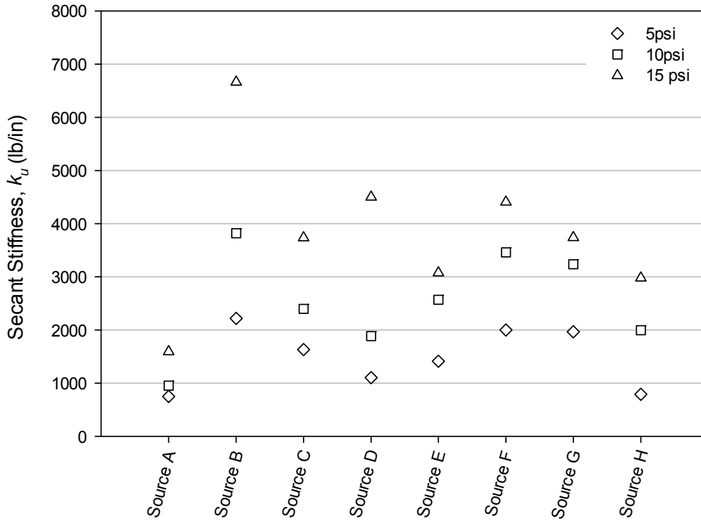
Figure 17: Ultimate secant stiffness ( k_u ) results for the Prepared gradations.
