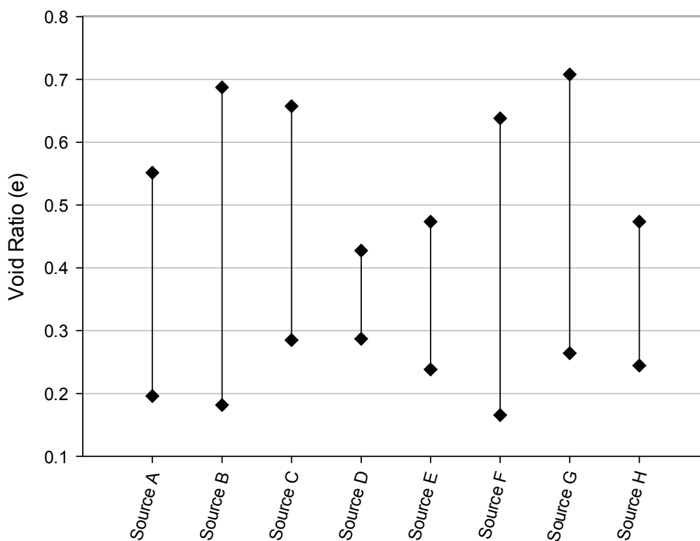
Figure 9: Relative densities of Modified gradations in terms of void ratio.
