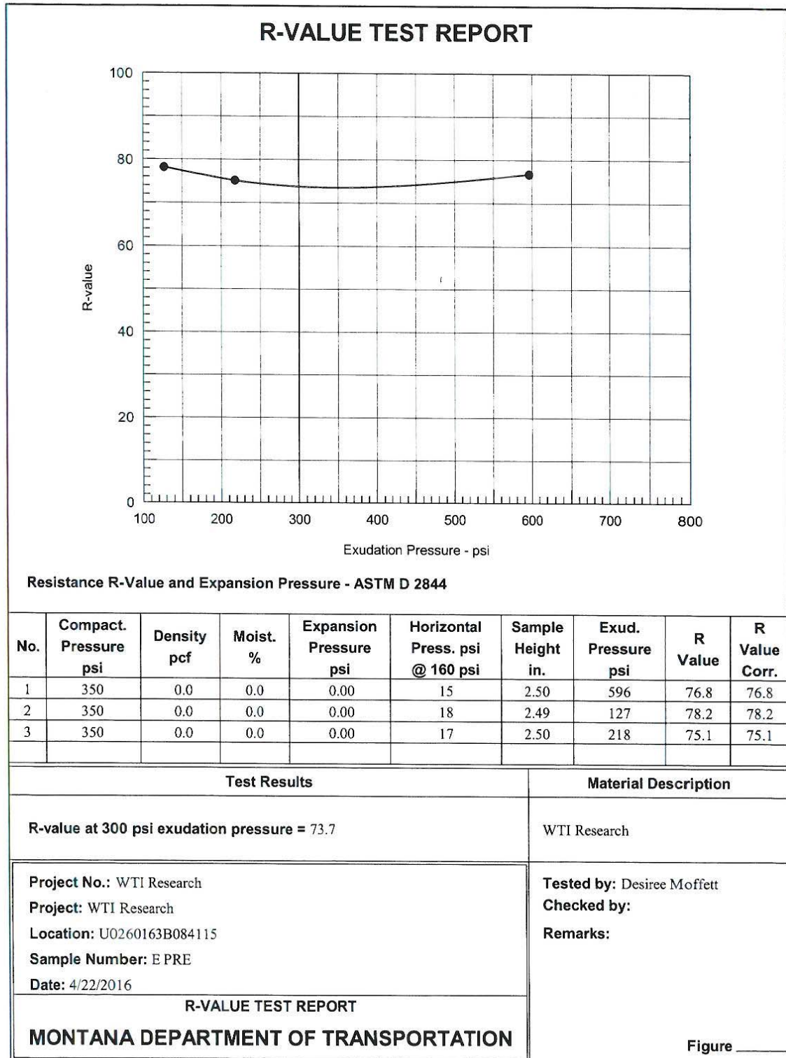
Figure D-17: R-value test report for Source E Prepared gradation.
