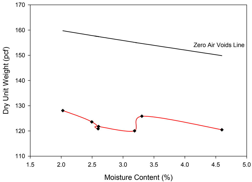
Figure C-6: Modified Proctor results for Source C Modified gradation.
