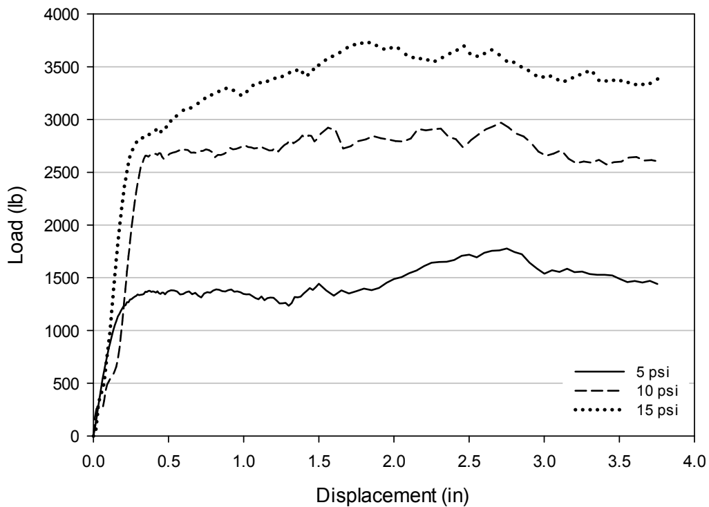
Figure E-2: Load-displacement plots from direct shear tests on Source A Modified gradation.
