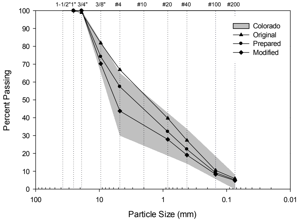
Figure B-1: Grain-size distribution of Source A gradations compared to Colorado specification.
