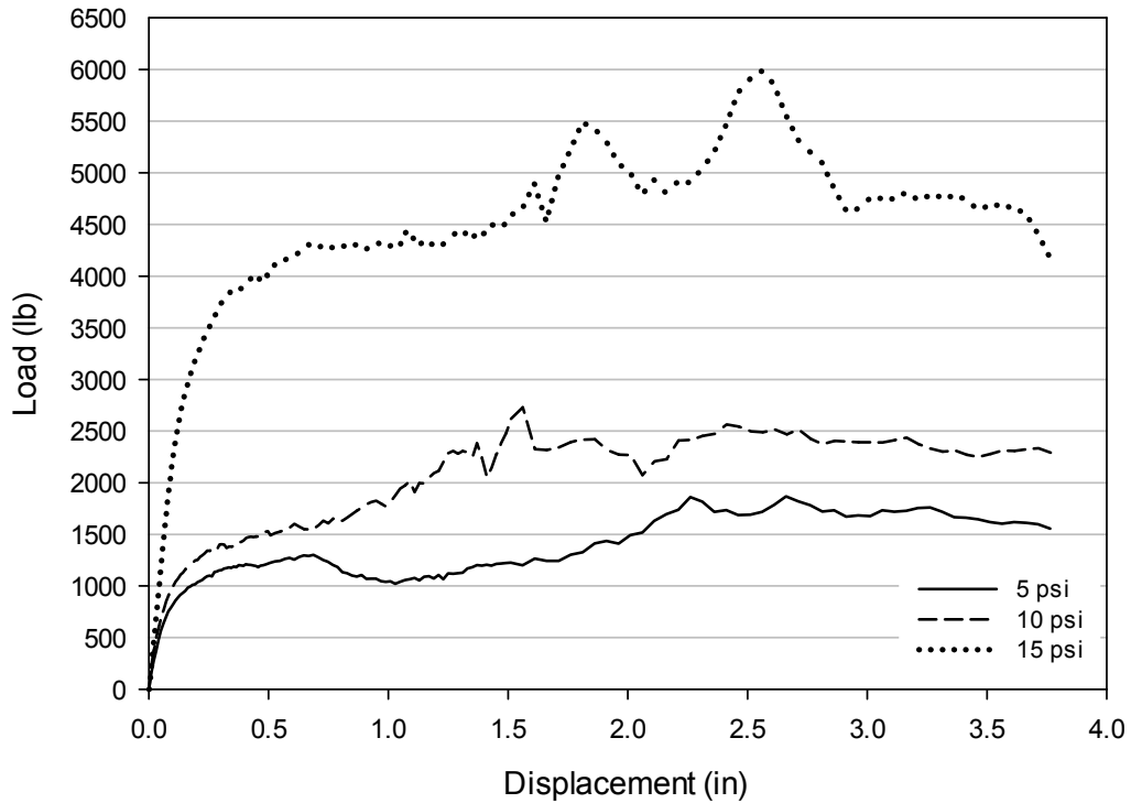
Figure E-7: Load-displacement plots from direct shear tests on Source D Prepared gradation.
