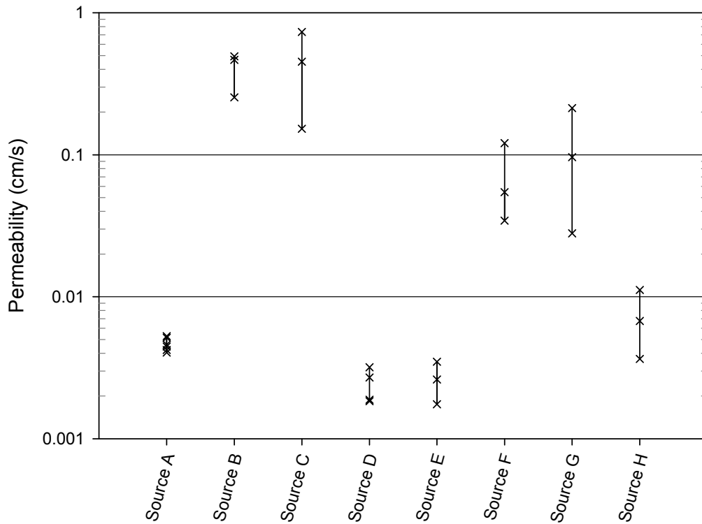
Figure 24: Permeability results of Prepared gradations.
