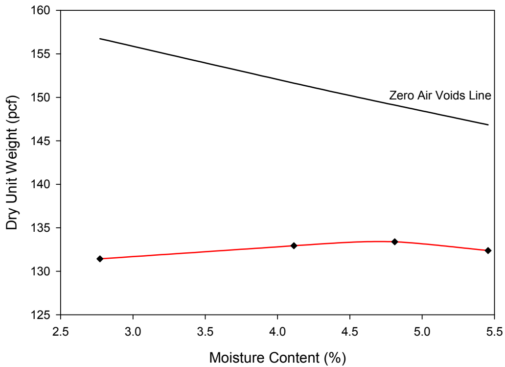
Figure C-2: Modified Proctor results for Source A Modified gradation.
