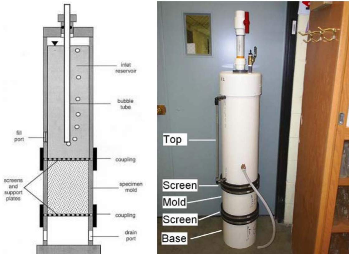
Figure 21: Schematic and photograph of permeameter.
