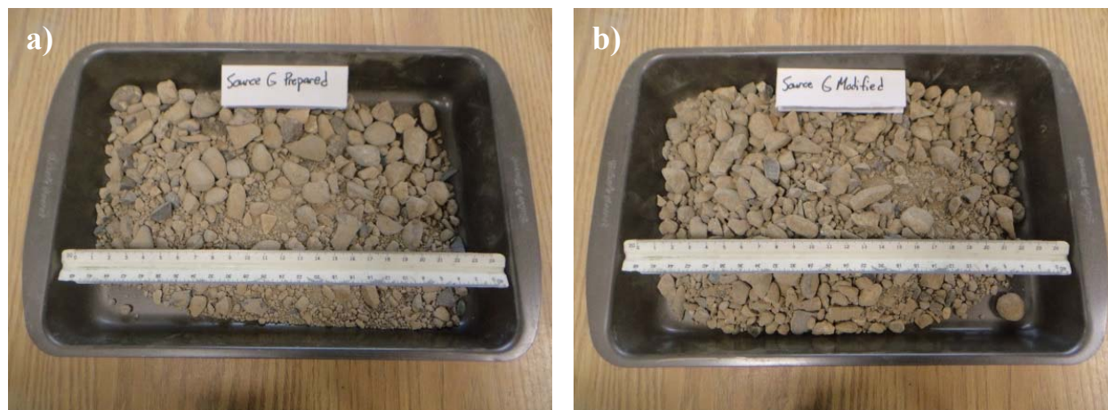
Figure A-7: Photo of Source G a) Prepared gradation and b) Modified gradation.
