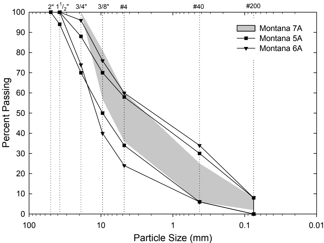
Figure 27: Final suggested 3/4-inch minus specifications (MT 7A) as compared to MT 6A and 5A.
