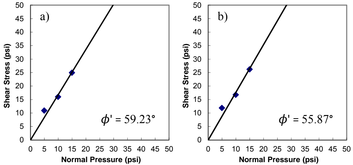
Figure F-3: Friction angle plots for Source C a) Prepared gradation and b) Modified gradation.
