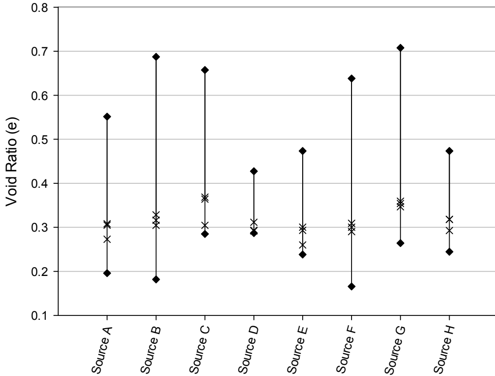
Figure 23. Densities of permeability samples for Modified gradations.
