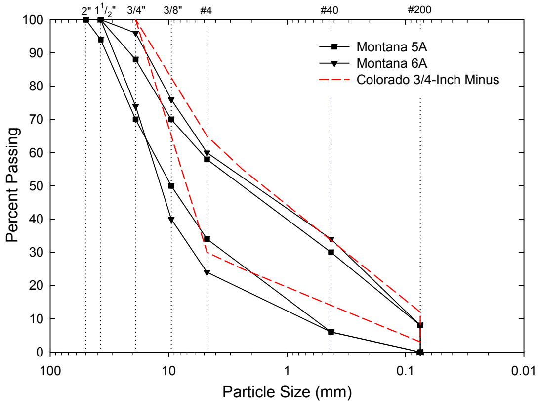
Figure 3: Montana 5A and 6A specifications compared to Colorado 3/4-inch minus specification.
