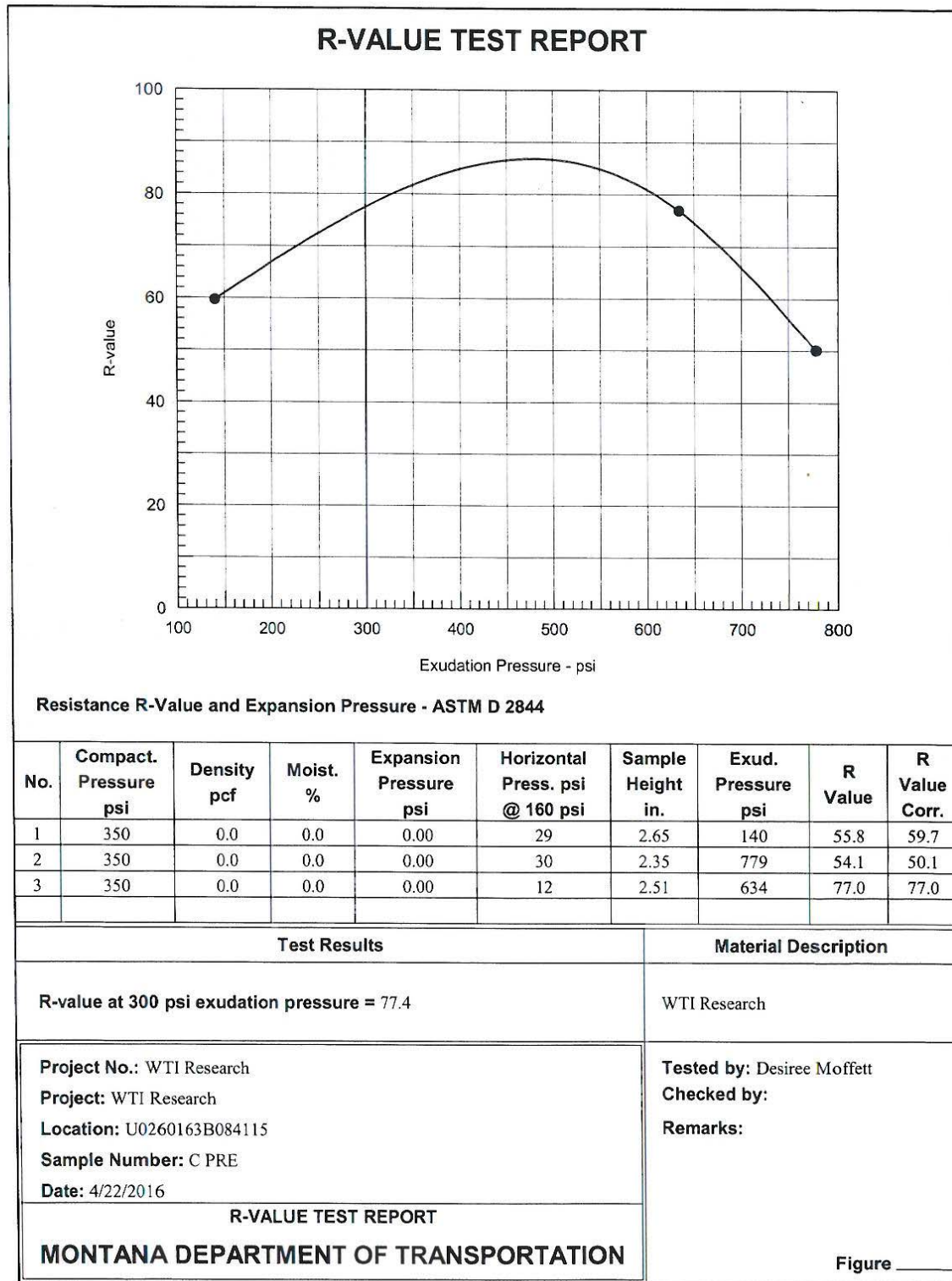
Figure D-9: R-value test report for Source C Prepared gradation.
