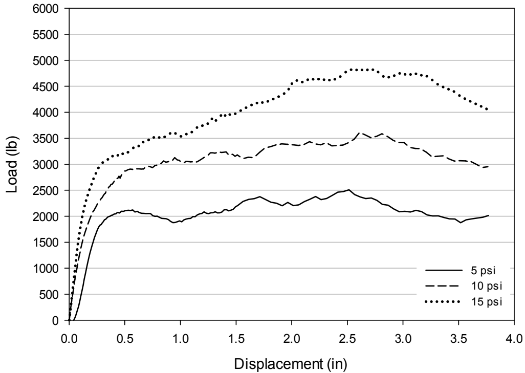
Figure E-13: Load-displacement plots from direct shear tests on Source G Prepared gradation.
