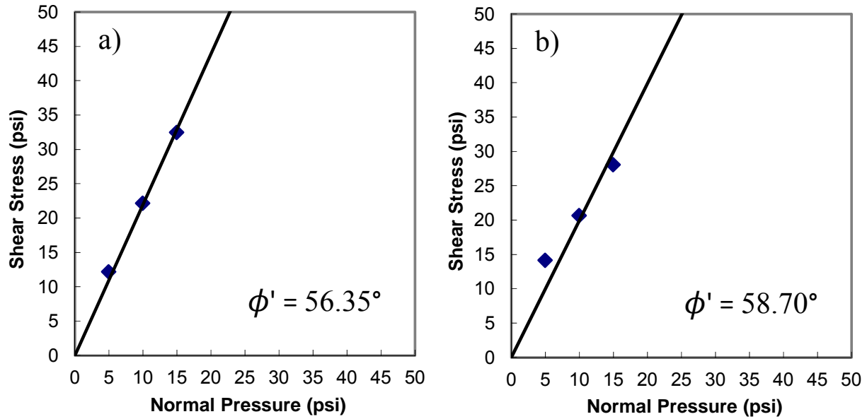
Figure F-5: Friction angle plots for Source E a) Prepared gradation and b) Modified gradation.
