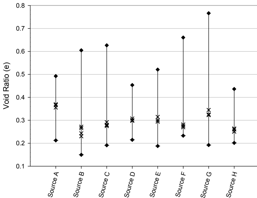
Figure 13: Direct shear densities for Prepared gradations.
