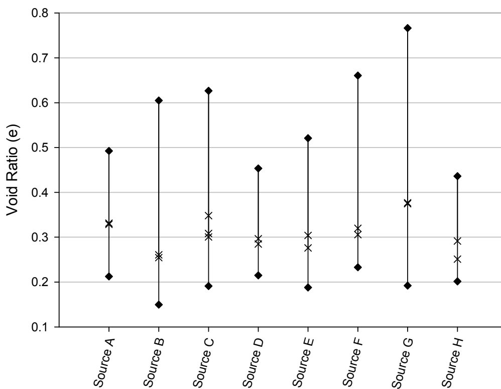
Figure 22. Densities of permeability samples for Prepared gradations.
