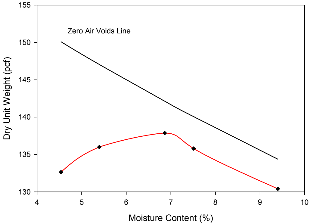
Figure C-9: Modified Proctor results for Source E Prepared gradation.
