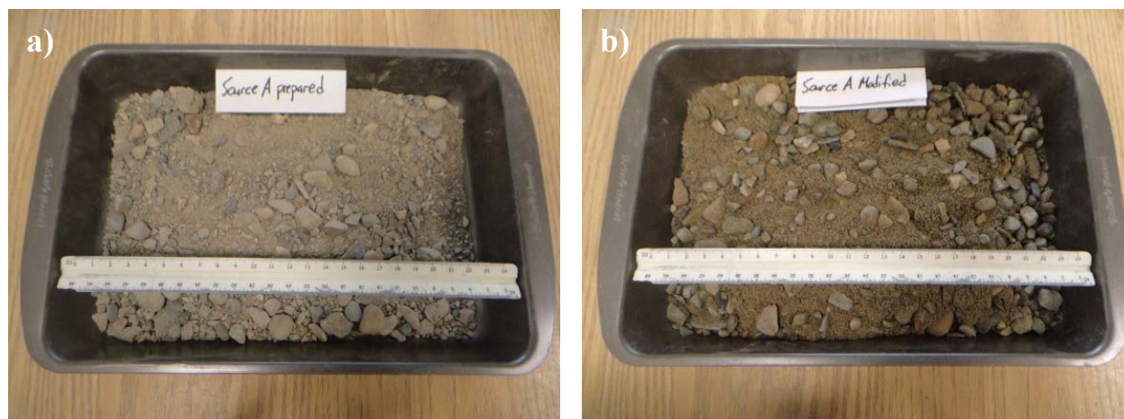
Figure A-1: Photo of Source A a) Prepared gradation and b) Modified gradation.
