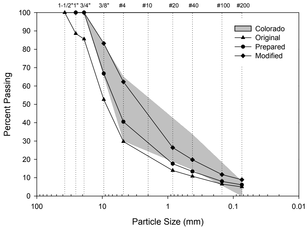
Figure B-6: Grain-size distribution of Source F gradations compared to Colorado specification.
