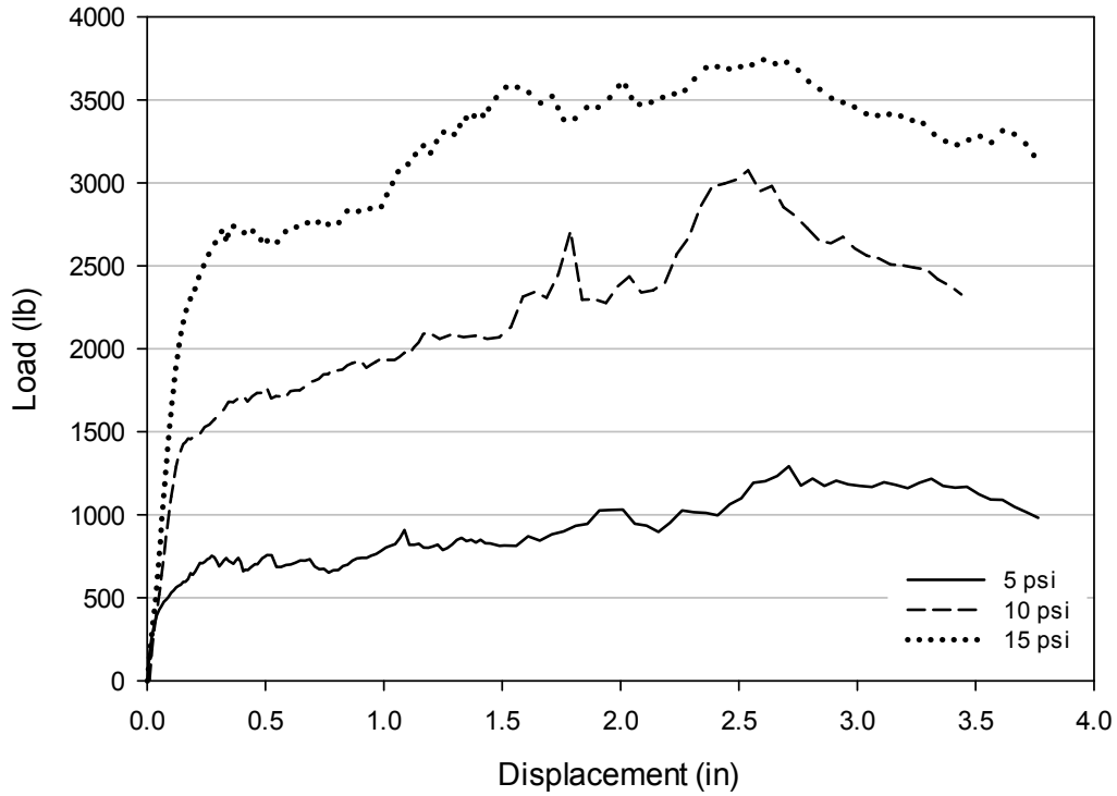
Figure E-15: Load-displacement plots from direct shear tests on Source H Prepared gradation.
