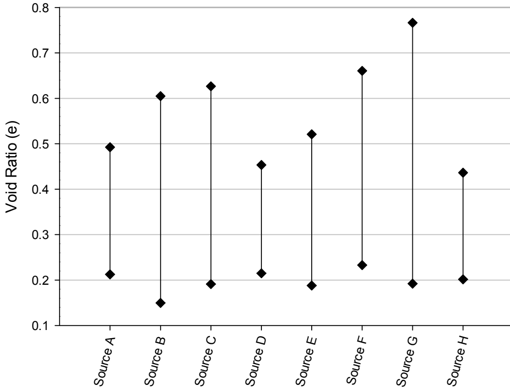
Figure 8: Relative density of Prepared gradations in terms of void ratio.
