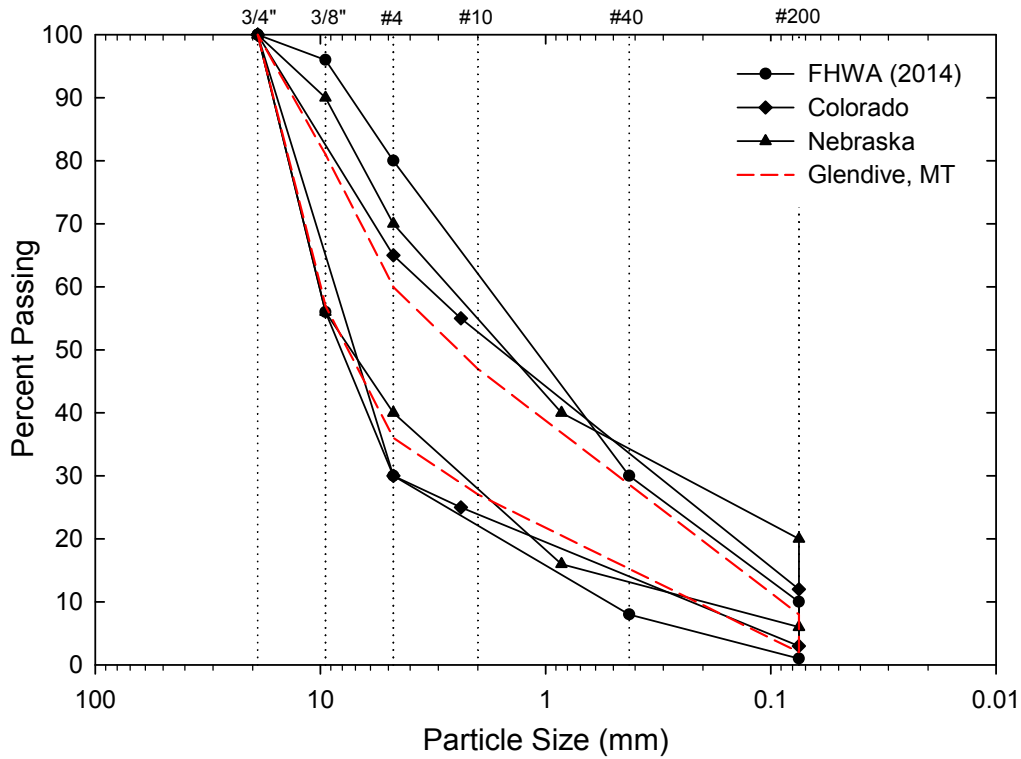
Figure 4: Montana Glendive specification compared to CO, NE and 2014 FHWA.
