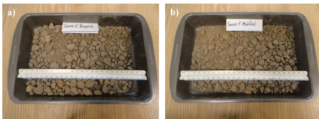
Figure A-6: Photo of Source F a) Prepared gradation and b) Modified gradation.
