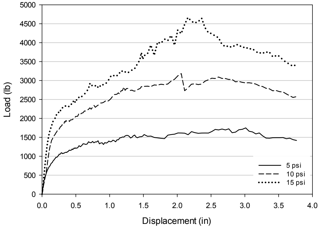
Figure E-9: Load-displacement plots from direct shear tests on Source E Prepared gradation.
