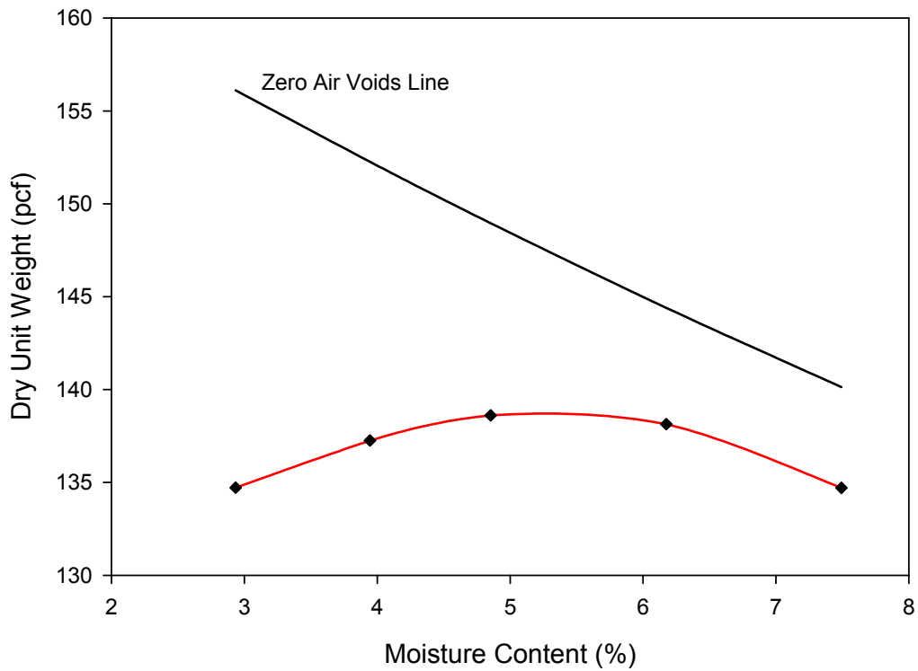
Figure C-12: Modified Proctor results for Source F Modified gradation.
