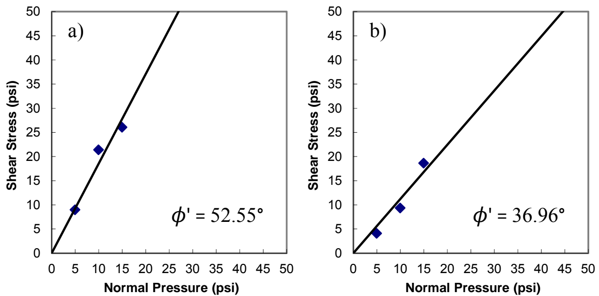
Figure F-8: Friction angle plots for Source H a) Prepared gradation and b) Modified gradation.
