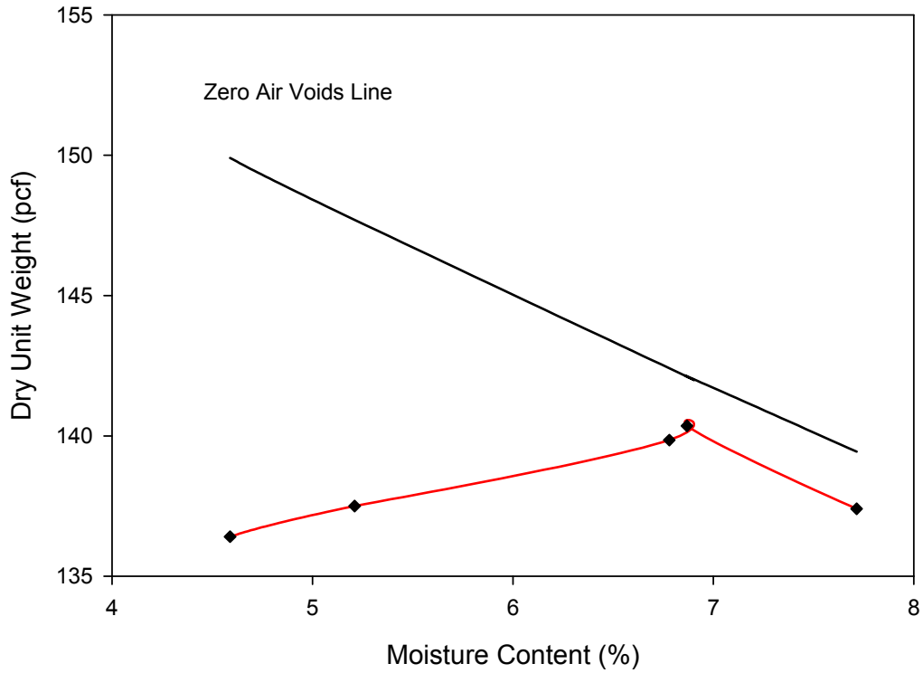
Figure C-13: Modified Proctor results for Source G Prepared gradation.
