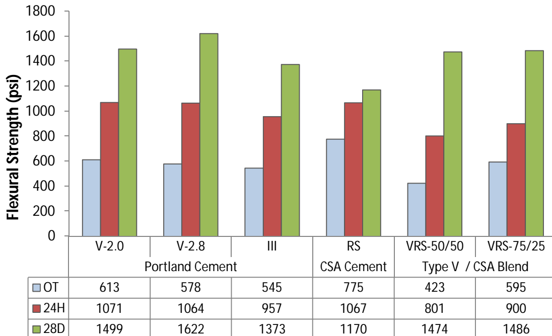
Figure 7-3: Flexural Strength of the Selected HES Concretes
