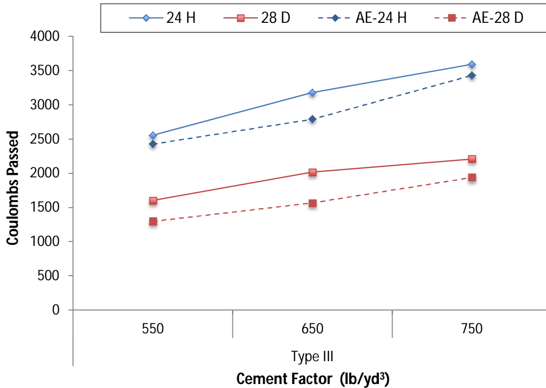
Figure 5-5: Passing Charge of Type III-HES Concretes
