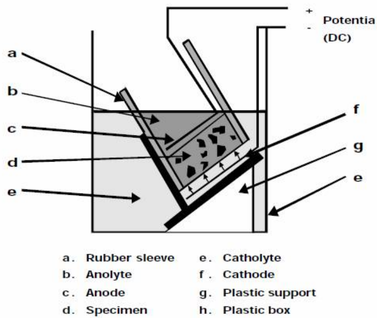
Figure 2-13: RMT Set-Up and Schematic
