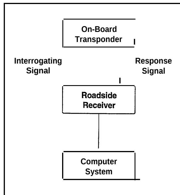
Figure 4-5.AVI block diagram.
