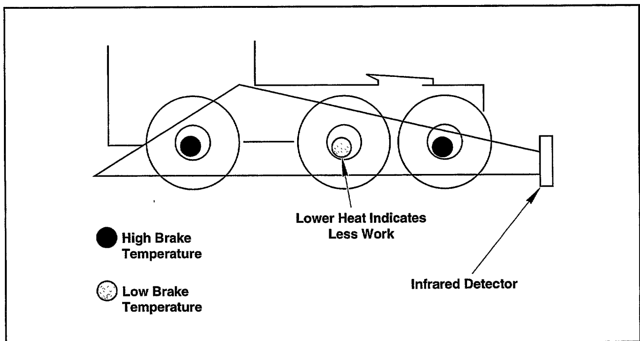
Figure 4-3. Infrared test schematic.
