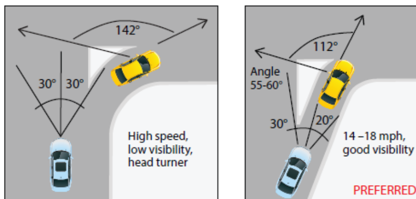
Figure 33. Right-Turn Channelization Design
