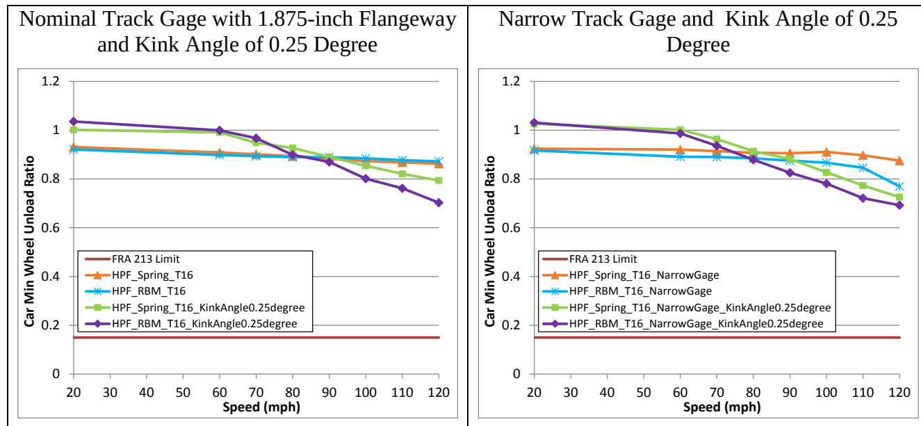
Figure 55. Minimum wheel unload ratio under the T16 passenger car - kink angle of 0.25 degree with nominal track gage (left) and narrow track gage (right)
