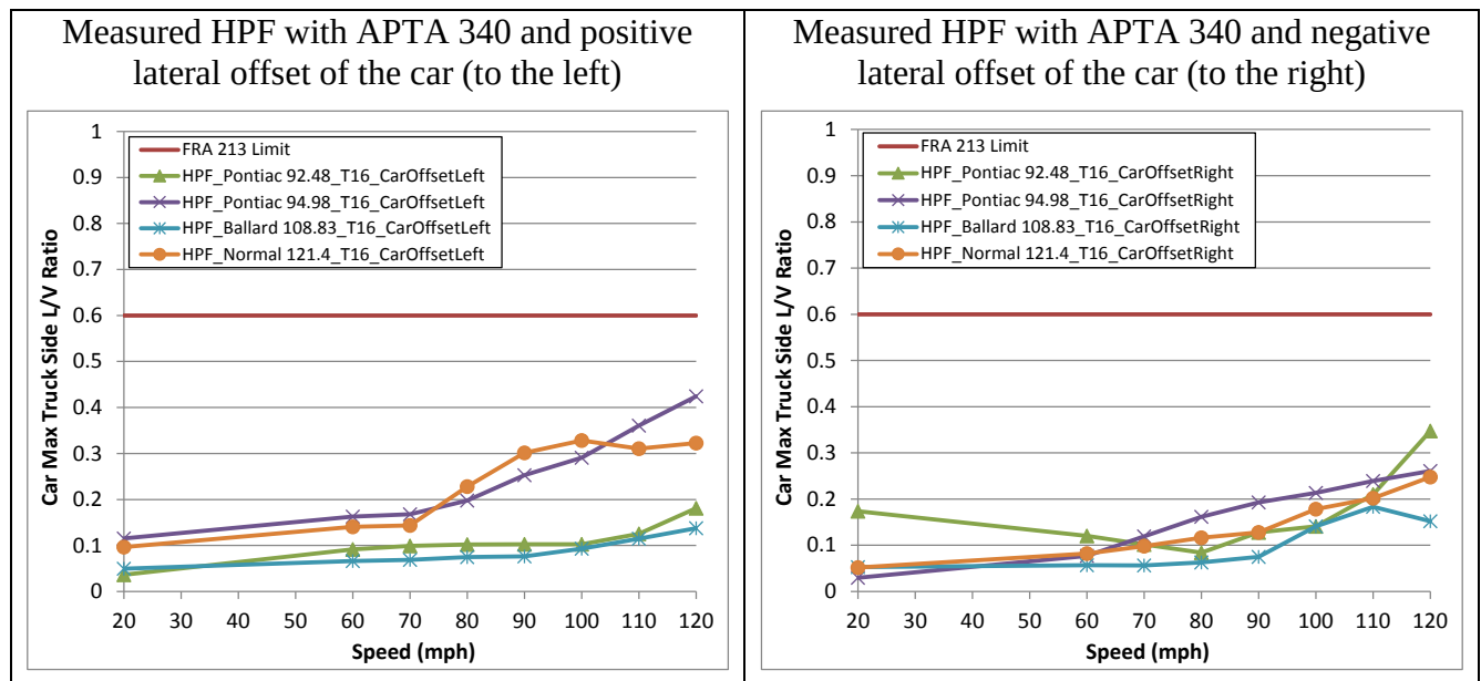
Figure 106. Maximum truck side L/V ratio under the T16 passenger car - measured HPFs with positive car offset (left) and negative car offset (right)
