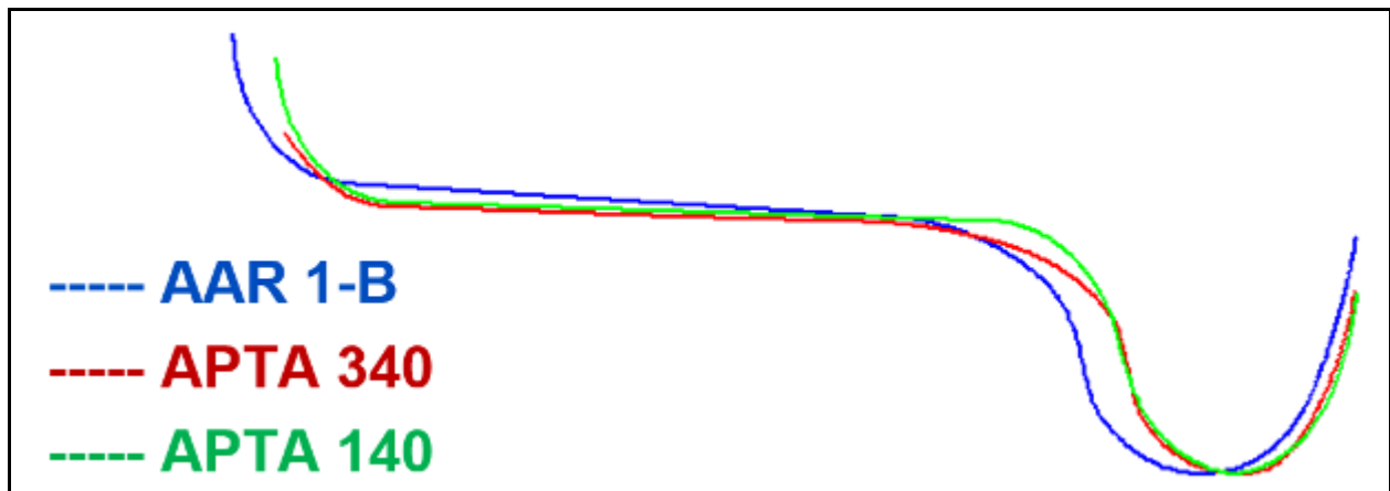
Figure 3. Wheel profiles
