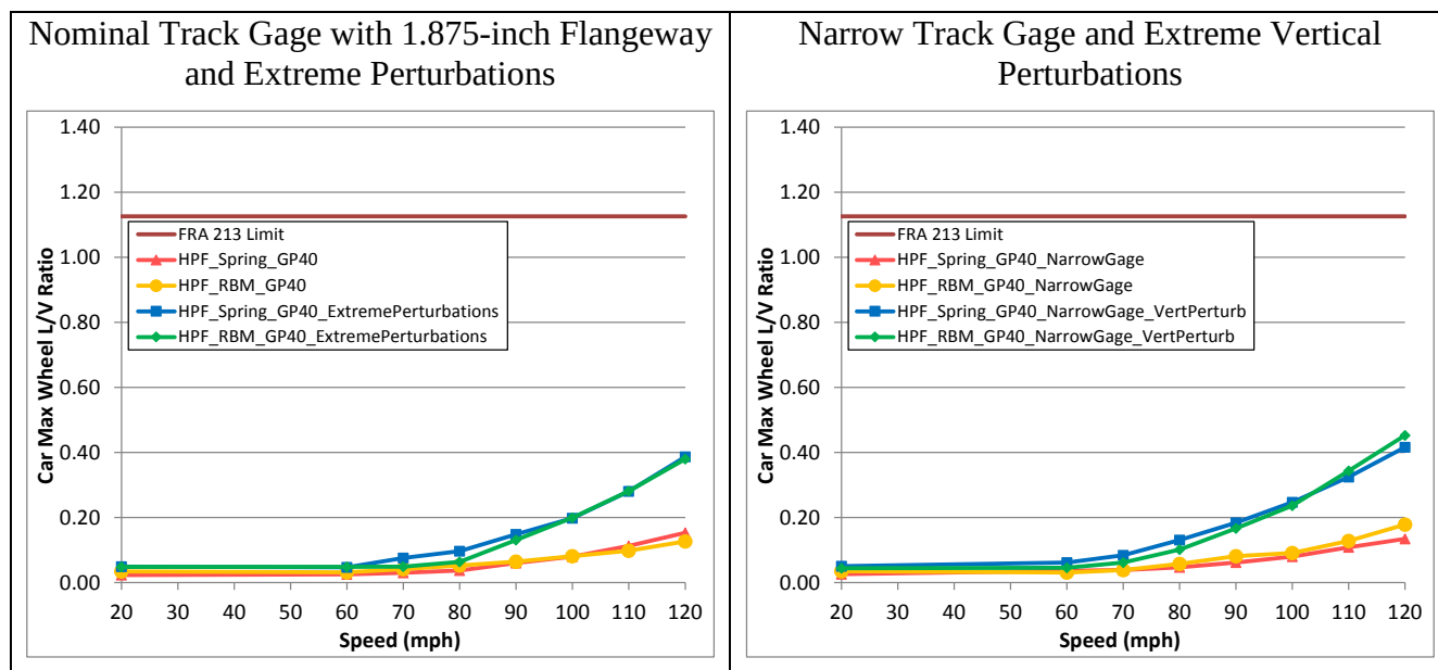
Figure 72. Single-wheel maximum L/V ratio under the GP40 passenger locomotive - nominal track gage (left) and narrow track gage (right)
