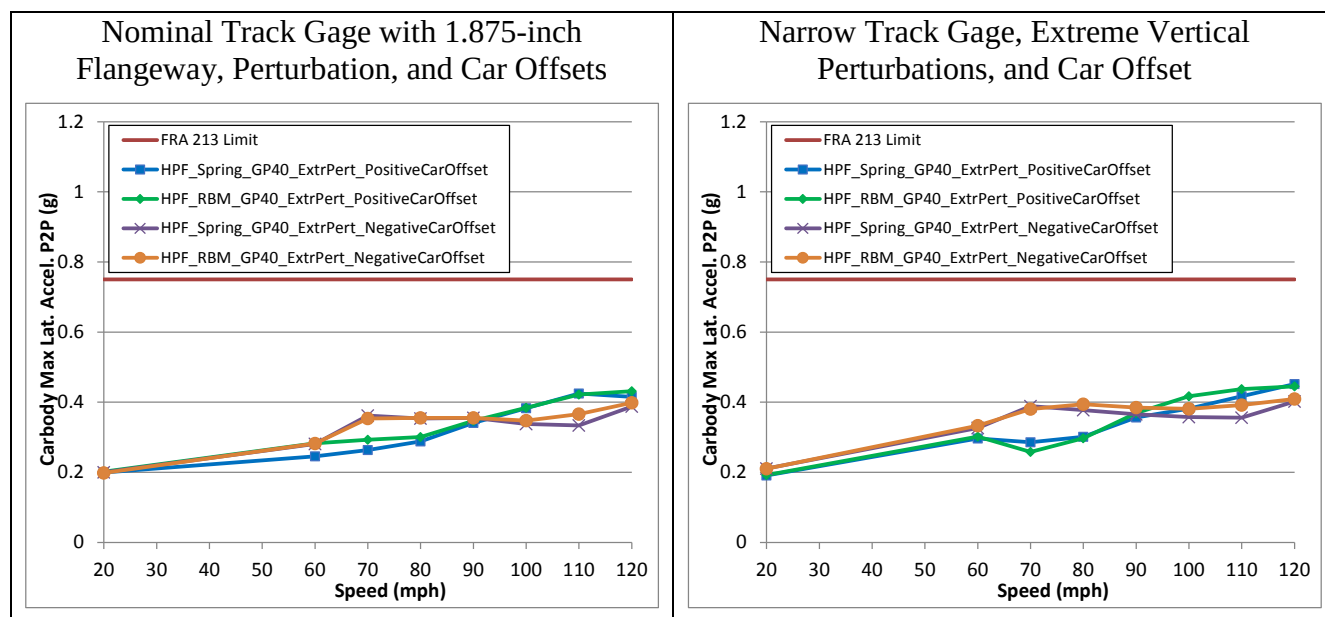
Figure 33. Carbody maximum lateral acceleration on the GP40 passenger locomotive - car offsets with nominal track gage (left) and narrow track gage (right)
