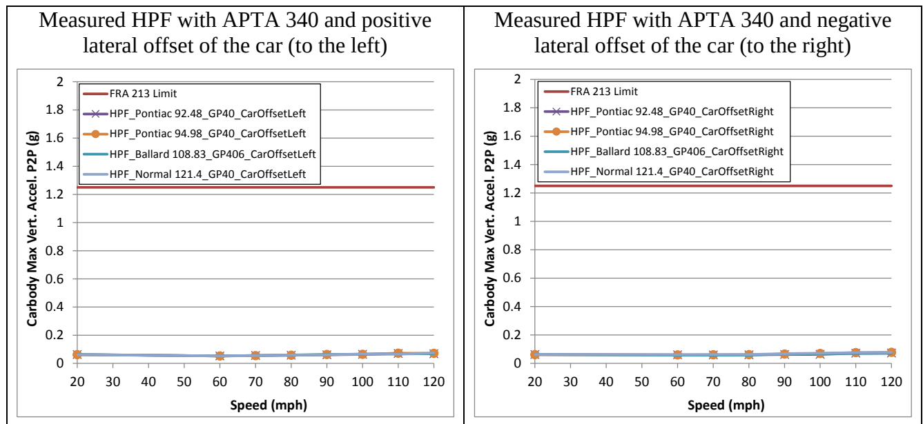
Figure 52. Carbody maximum vertical acceleration on the GP40 passenger locomotive - measured HPFs with positive car offset (left) and negative car offset (right) Single Wheel Vertical Load Ratio
