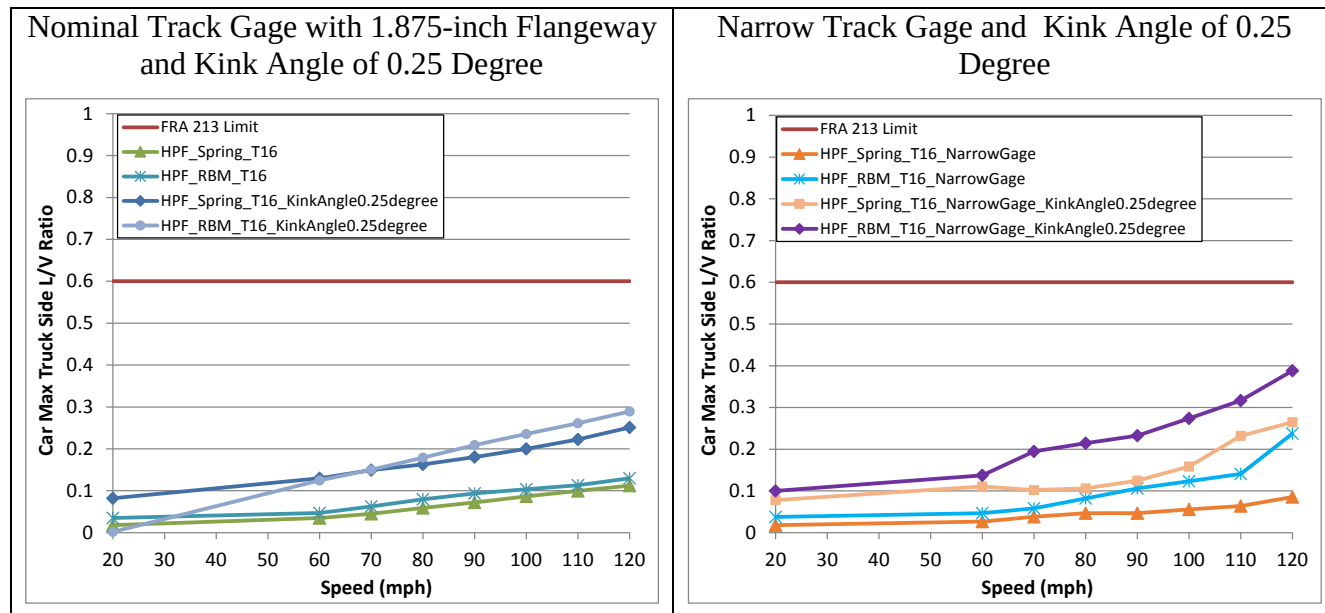
Figure 97. Maximum truck side L/V ratio under the T16 passenger car - kink angle of 0.25 degree with nominal track gage (left) and narrow track gage (right)
