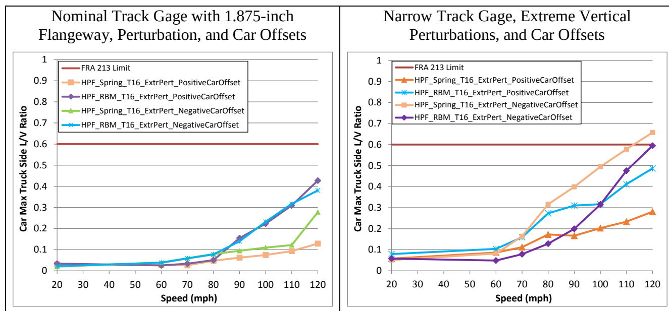
Figure 98. Maximum truck side L/V ratio under the T16 passenger car - car offsets with nominal track gage (left) and narrow track gage (right)
