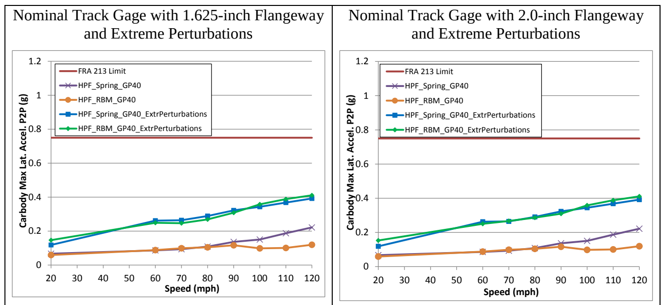
Figure 31. Carbody maximum lateral acceleration on the GP40 passenger locomotive - nominal track gage with 1.625-inch flangeway (left) and 2.0-inch flangeway (right)
