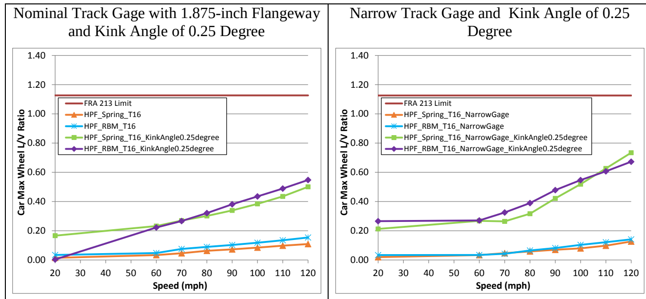
Figure 69. Single-wheel maximum L/V ratio under the T16 passenger car - kink angle of 0.25 degree with nominal track gage (left) and narrow track gage (right)
