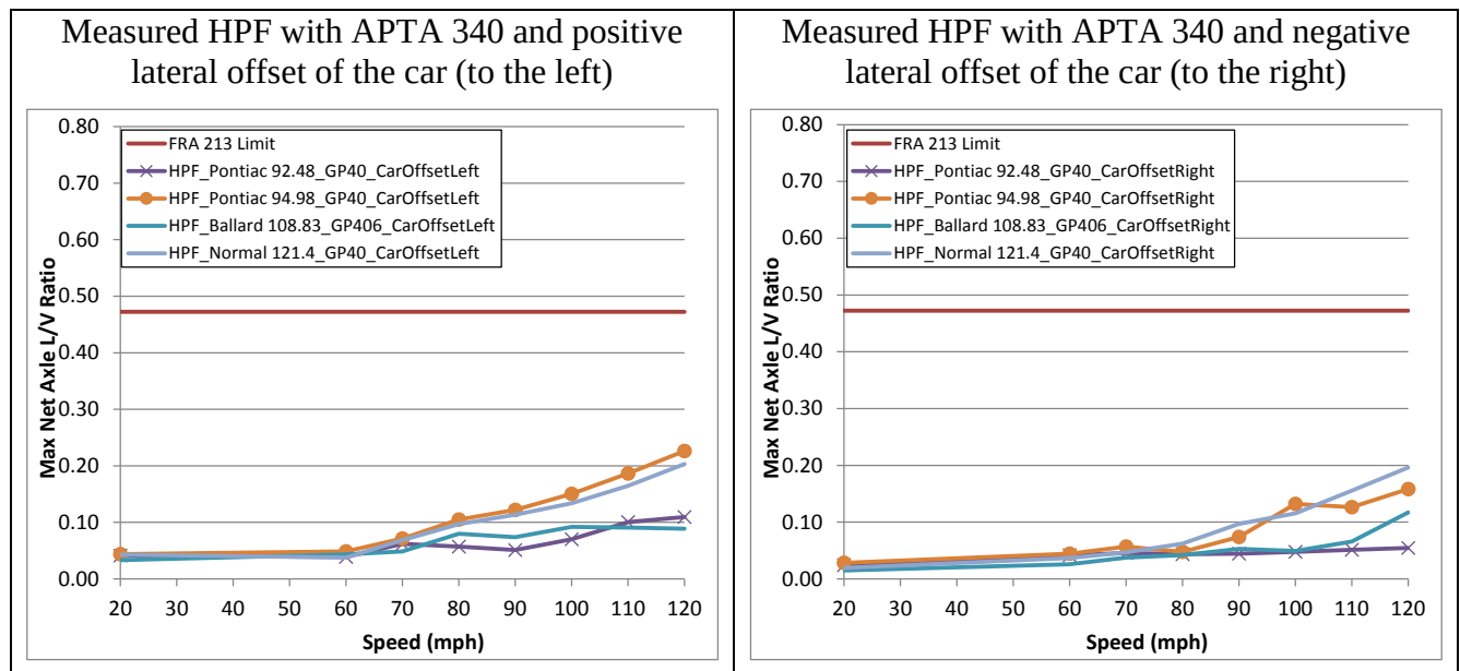
Figure 94. Maximum net axle lateral L/V ratio under the GP40 passenger locomotive - Measured HPFs with positive car offset (left) and negative car offset (right)
