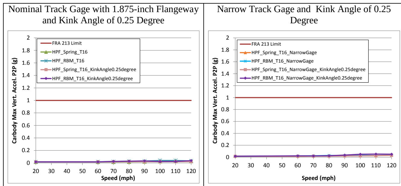
Figure 41. Carbody maximum vertical acceleration on the T16 passenger car - kink angle of 0.25 degree with nominal track gage (left) and narrow track gage (right)
