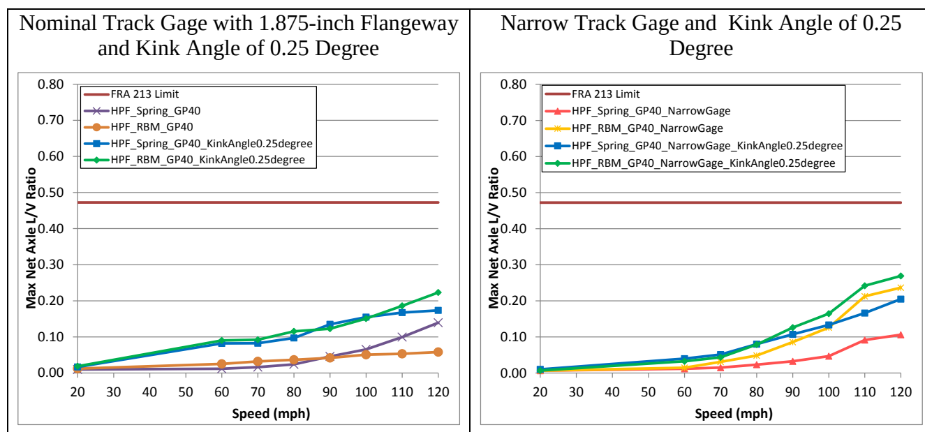
Figure 88. Maximum net axle lateral L/V ratio under the GP40 passenger locomotive - kink angle of 0.25 degree with nominal track gage (left) and narrow track gage (right)
