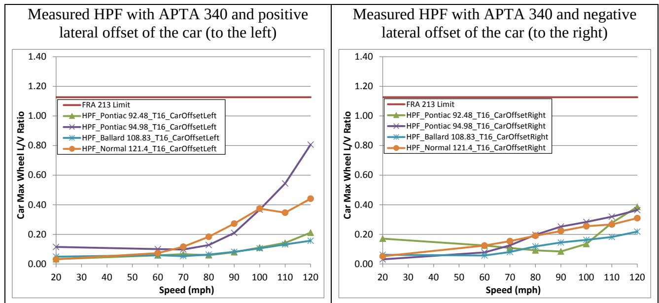
Figure 78. Single-wheel maximum L/V ratio under the T16 passenger car - measured HPFs with positive car offset (left) and negative car offset (right)
