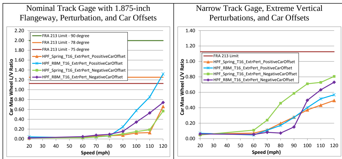
Figure 70. Single-wheel maximum L/V ratio under the T16 passenger car - car offsets with nominal track gage (left) and narrow track gage (right)
