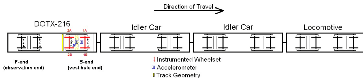
Figure 109. Train consist for IWS test
