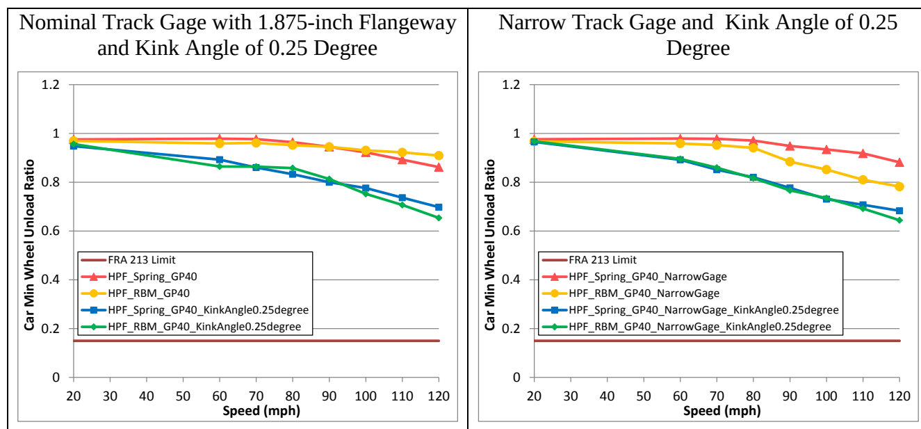
Figure 60. Minimum wheel unload ratio under the GP40 passenger locomotive - kink angle of 0.25 degree with nominal track gage (left) and narrow track gage (right)
