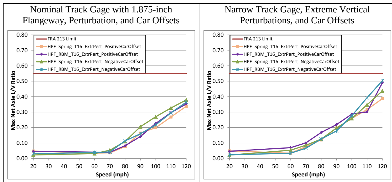
Figure 84. Maximum net axle lateral L/V ratio under the T16 passenger car - car offsets with nominal track gage (left) and narrow track gage (right)
