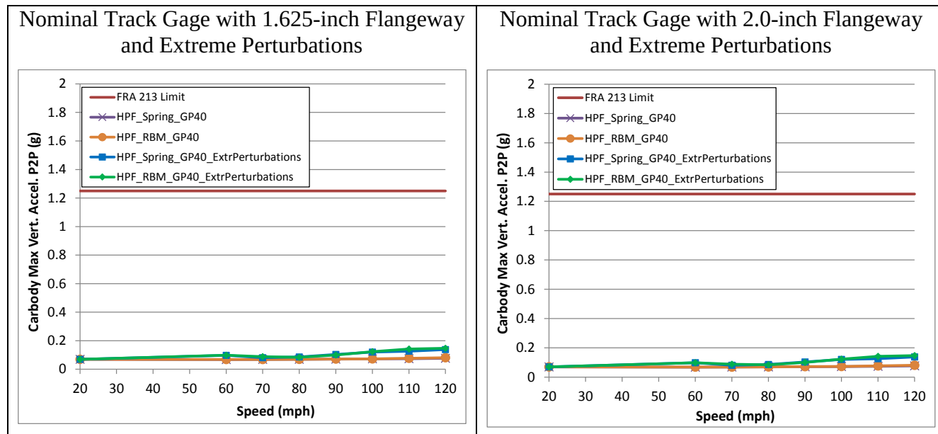
Figure 45. Carbody maximum vertical acceleration on the GP40 passenger locomotive - nominal track gage with 1.625-inch flangeway (left) and 2.0-inch flangeway (right)
