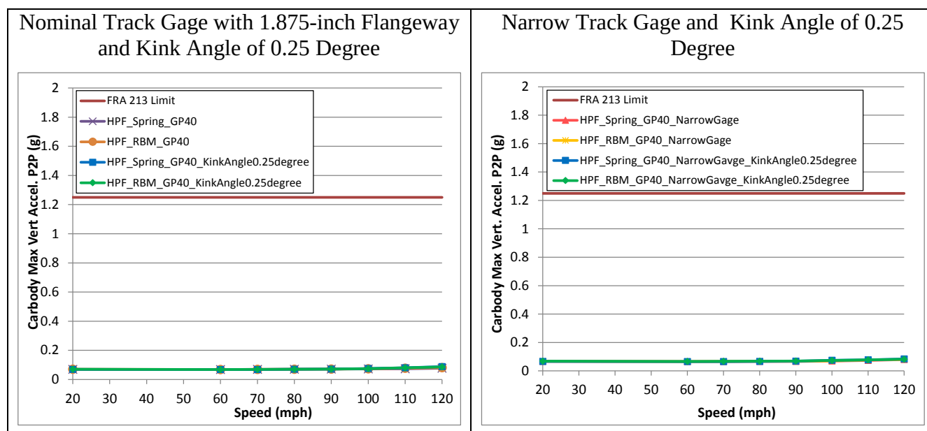
Figure 46. Carbody maximum vertical acceleration on the GP40 passenger locomotive - kink angle of 0.25 degree with nominal track gage (left) and narrow track gage (right)
