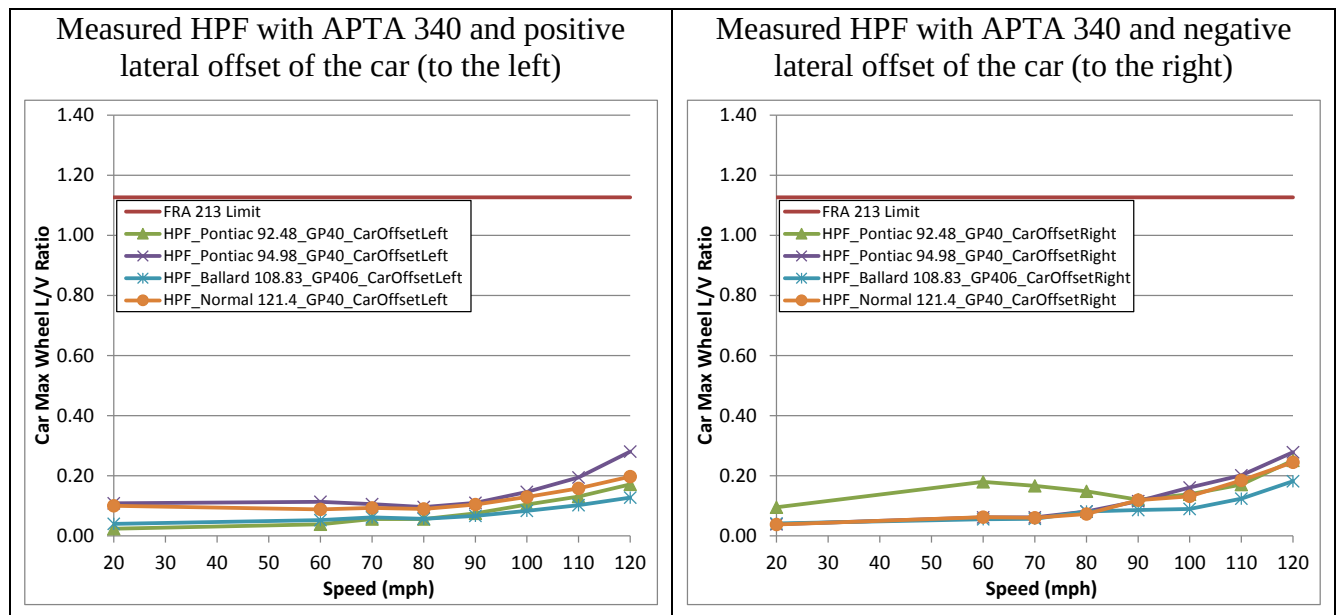
Figure 80. Single-wheel maximum L/V ratio under the GP40 passenger locomotive - measured HPFs with positive car offset (left) and negative car offset (right)
