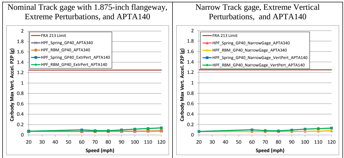
Figure 48. Carbody maximum vertical acceleration on the GP40 passenger locomotive - APTA140 with nominal track gage (left) and narrow track gage (right)
