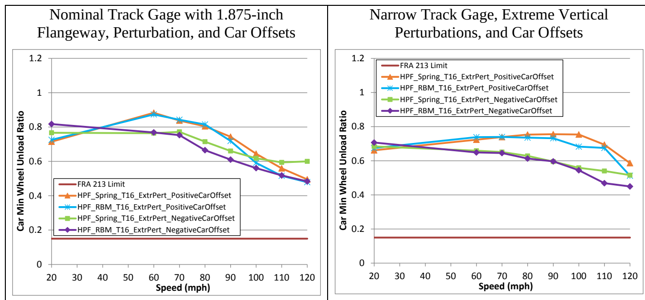
Figure 56. Minimum wheel unload ratio under the T16 passenger car - car offsets with nominal track gage (left) and narrow track gage (right)
