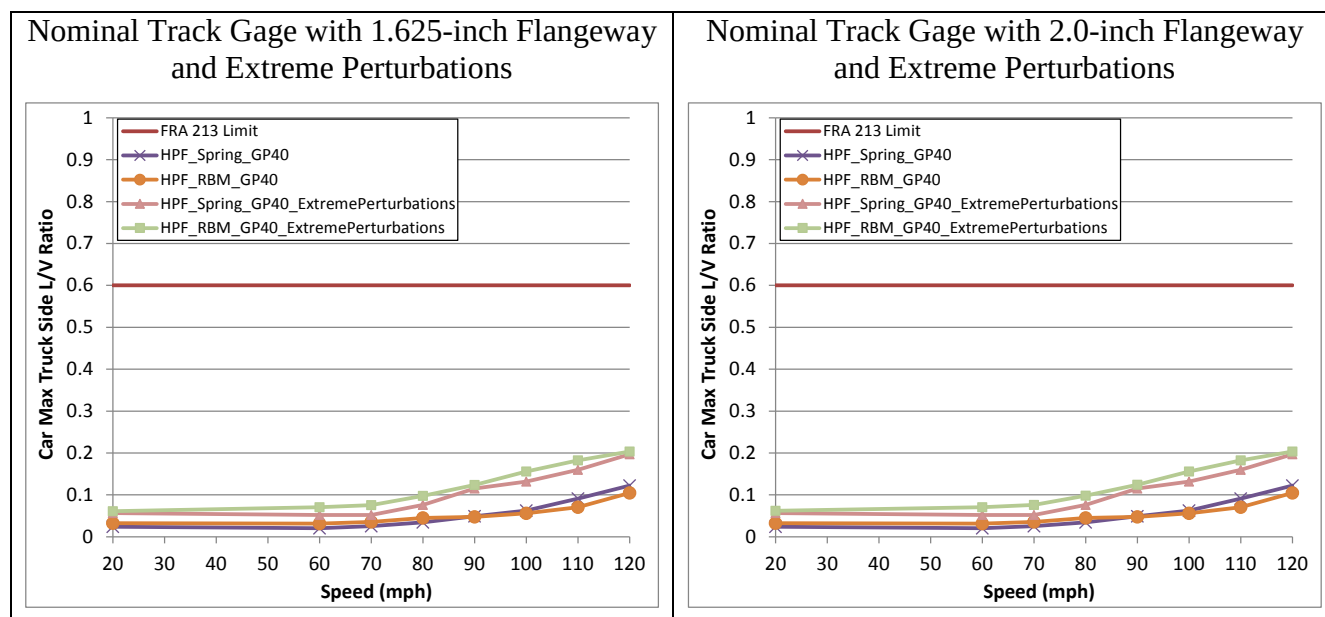
Figure 101. Maximum truck side L/V ratio under the GP40 passenger locomotive - nominal track gage with 1.625-inch flangeway (left) and 2.0-inch flangeway (right)
