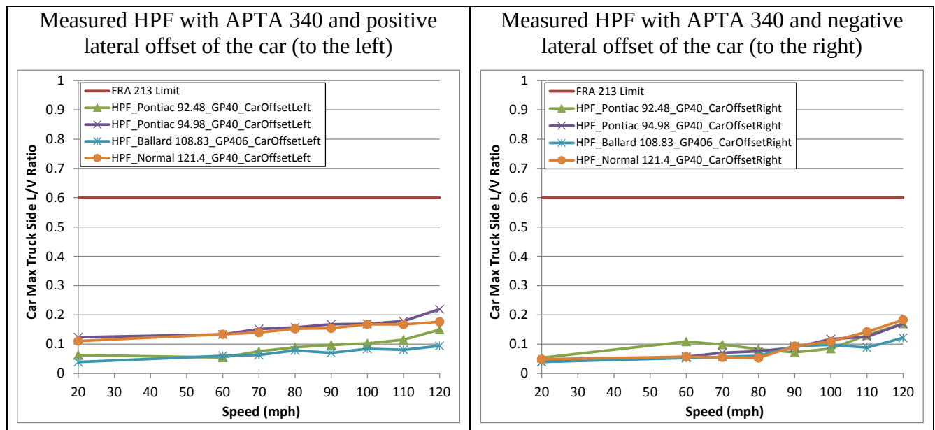
Figure 108. Maximum truck side L/V ratio under the GP40 passenger locomotive - measured HPFs with positive car offset (left) and negative car offset (right)
