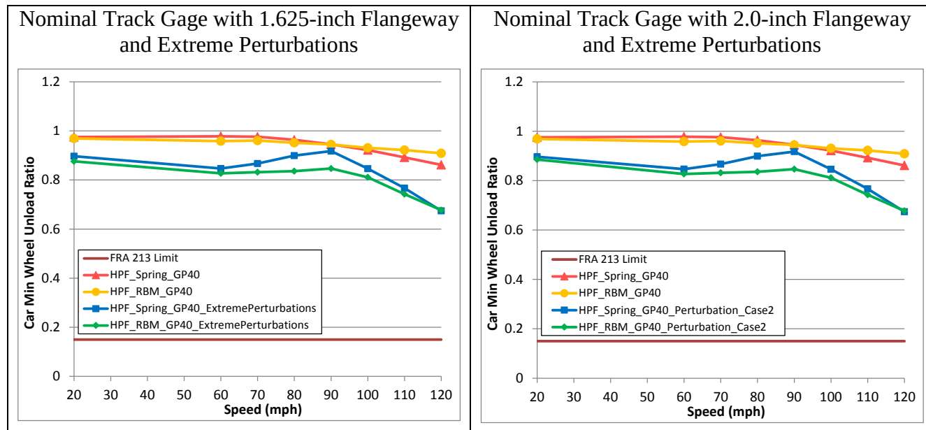
Figure 59. Minimum wheel unload ratio under the GP40 passenger locomotive - nominal track gage with 1.625-inch flangeway (left) and 2.0-inch flangeway (right)
