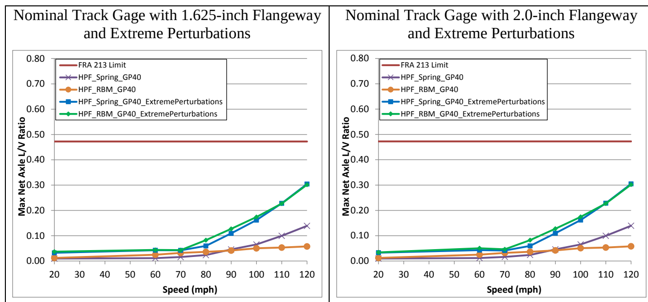
Figure 87. Maximum net axle lateral L/V ratio under the GP40 passenger locomotive - nominal track gage with 1.625-inch flangeway (left) and 2.0-inch flangeway (right)
