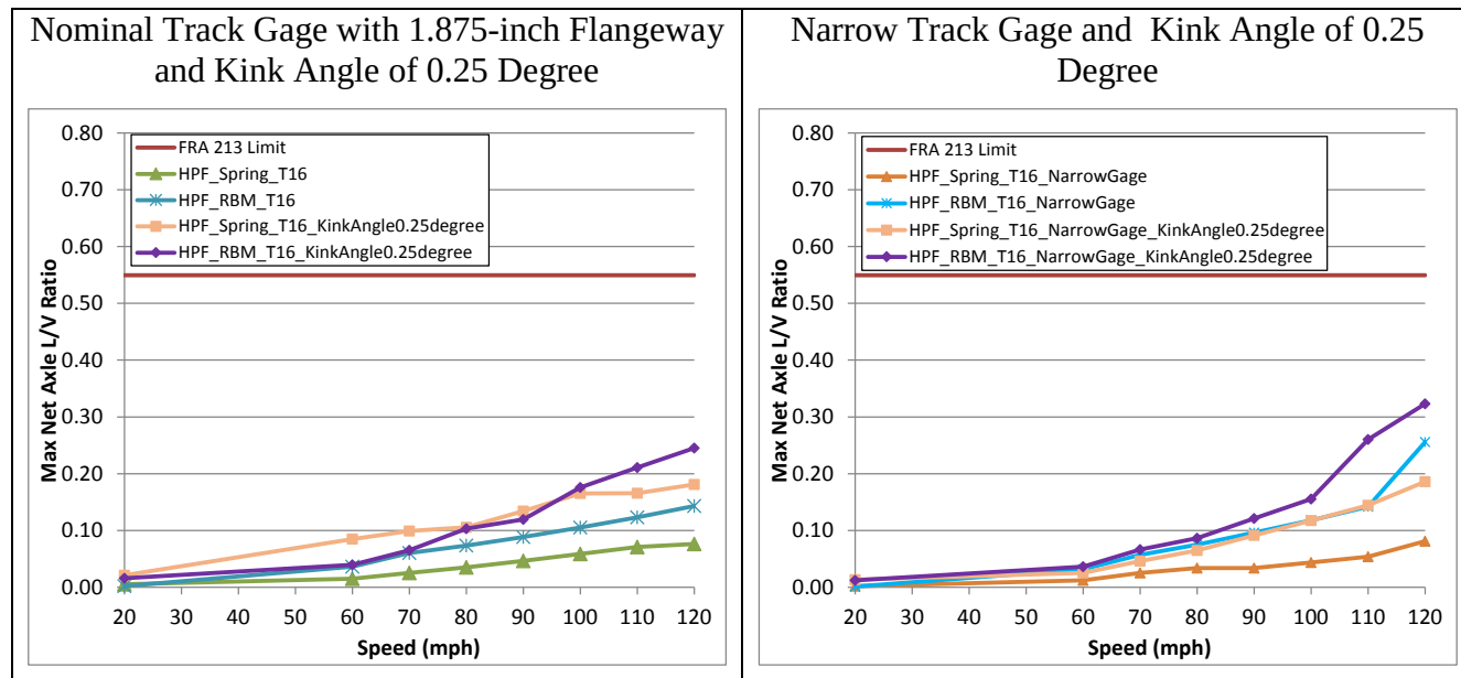
Figure 83. Maximum net axle lateral L/V ratio under the T16 passenger car - kink angle of 0.25 degree with nominal track gage (left) and narrow track gage (right)
