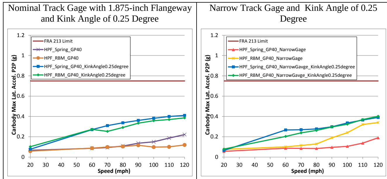
Figure 32. Carbody maximum lateral acceleration on the GP40 passenger locomotive - kink Angle of 0.25 degree with nominal track gage (left) and narrow track gage (right)
