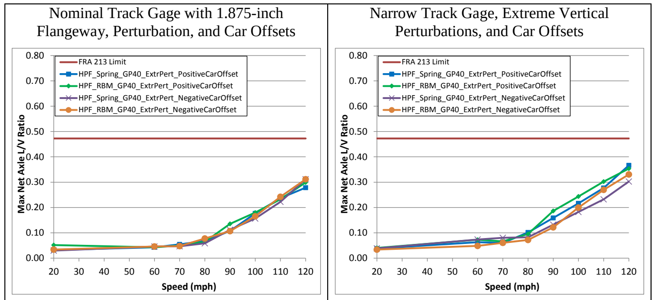
Figure 89. Maximum net axle lateral L/V ratio under the GP40 passenger locomotive - car offsets with nominal track gage (left) and narrow track gage (right)
