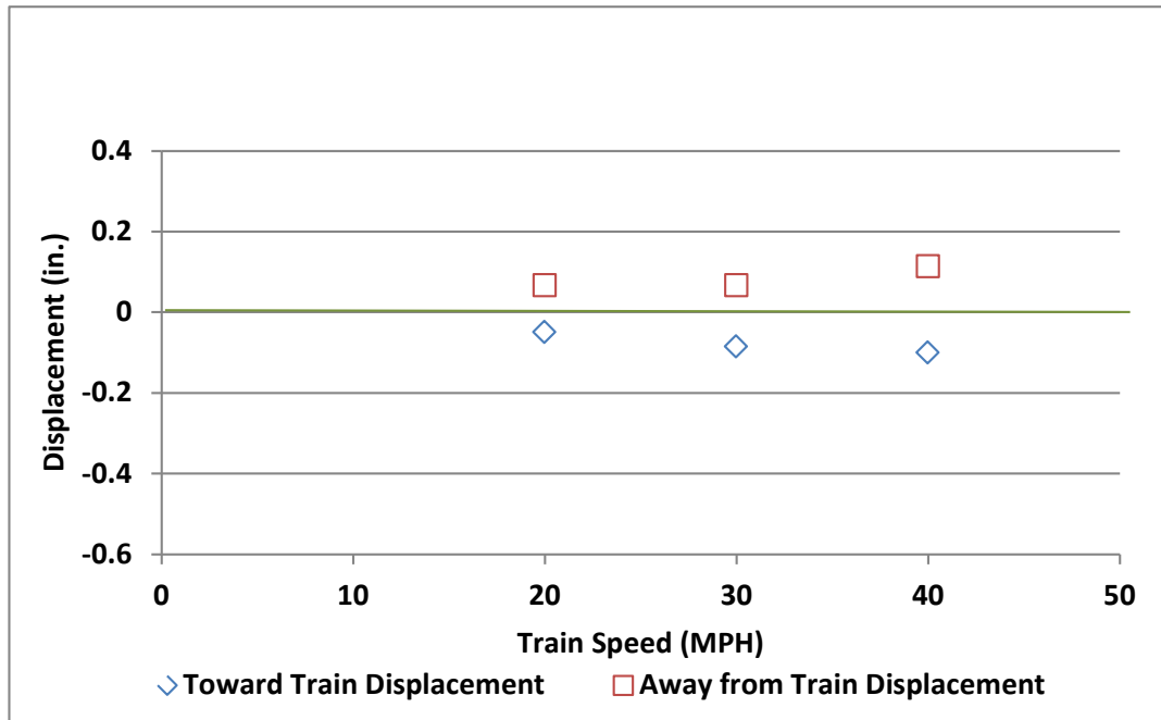
Figure 82. Each speed dataset represents the maximum longitudinal displacement measured in each direction under the entire train at the given speed
