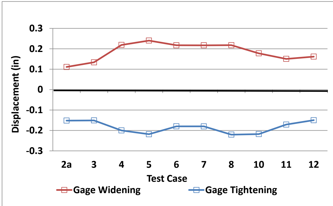
Figure 87. Lateral displacement of the outside corner in gage widening and gage tightening direction at 40 mph
