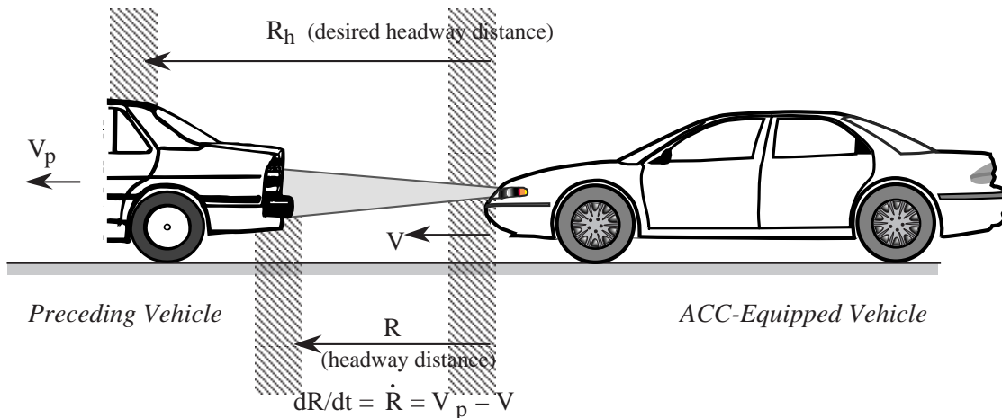
Figure 7. Headway control
