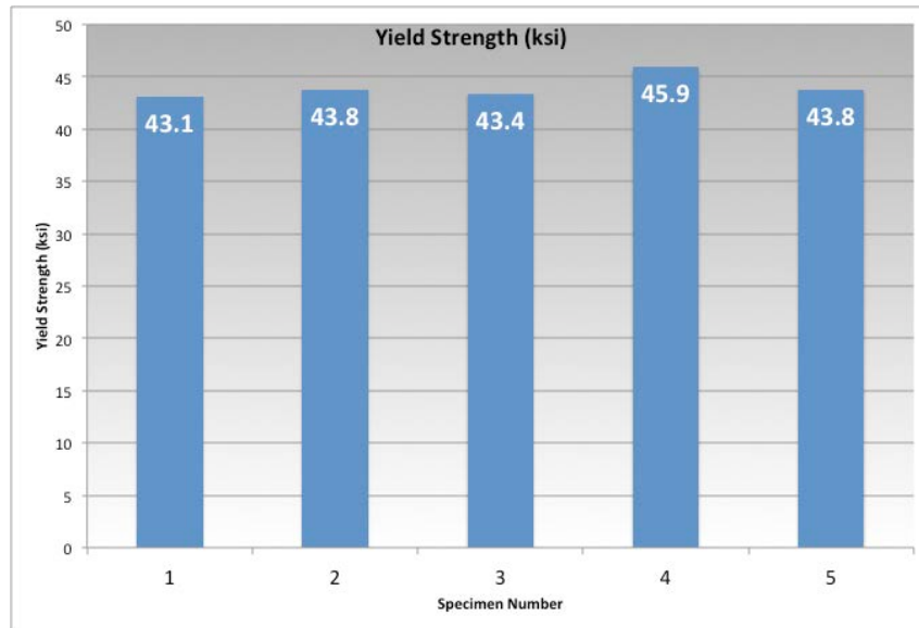
Figure 22. Material properties per sample — yield strength.
