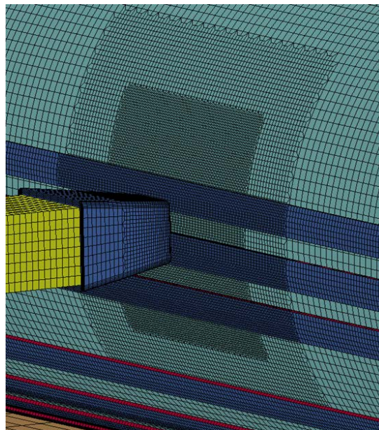
Figure 29. Impact zone of shell based tank in global response model.
