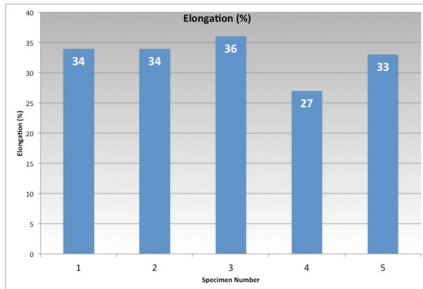
Figure 23. Material properties per sample — elongation at failure.
