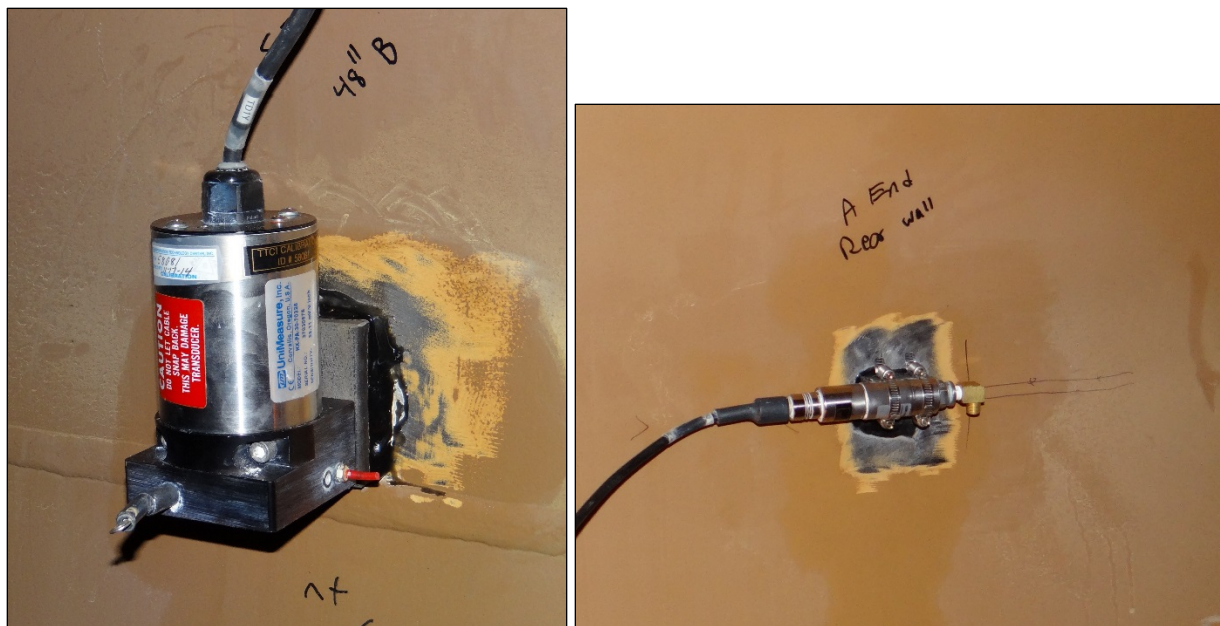
Figure A-5. Typical Mounting of String Potentiometer and Pressure Gauges (Tank Interior)
