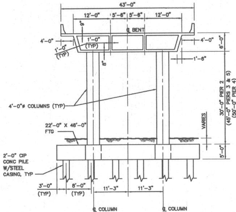
Figure 6.4 LRFD Example Bridge cross-section at an intermediate pier (ATC/MCEER 2003a).
