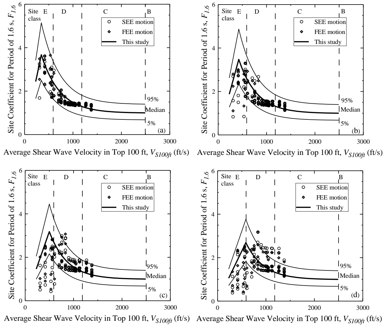
Figure G.5 Site coefficient for 1.6 s spectral period with S_{1.6} equal to (a) 0.02 g, (b) 0.05 g, (c) 0.1 g, and (d) 0.2 g for Lake Marion.
