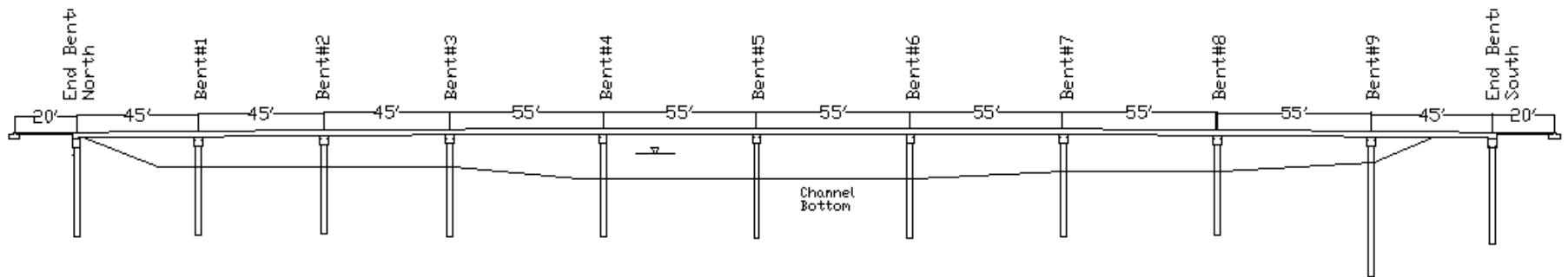
Figure 6.17 Schematic diagram of Russell Creek Bridge.
