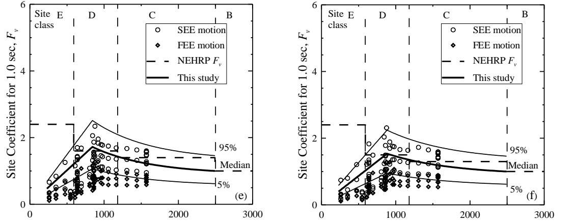
Average Shear Wave Velocity in Top 100 ft, V_{S100ft} (ft/s) Average Shear Wave Velocity in Top 100 ft, V_{S100ft} (ft/s)
