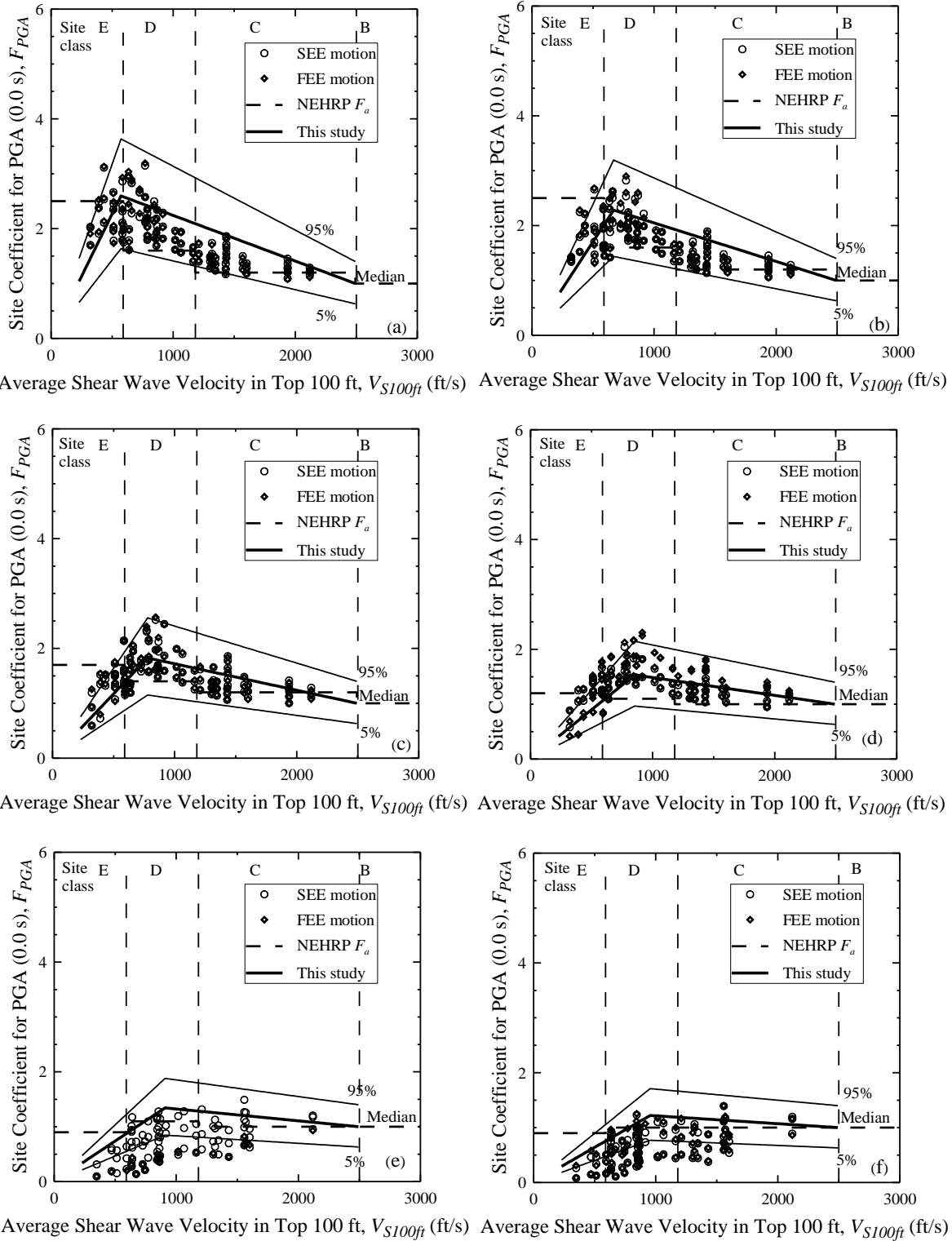
Figure 3.11 Site coefficients for 0.0 s spectral period (free-field) with PGA_{oucrop} equal to (a) 0.05 g, (b) 0.1 g, (c) 0.2 g, (d) 0.3 g, (e) 0.4 g, and (f) 0.5 g based on V_S profiles shown in Figure 3.3b for Myrtle Beach.
