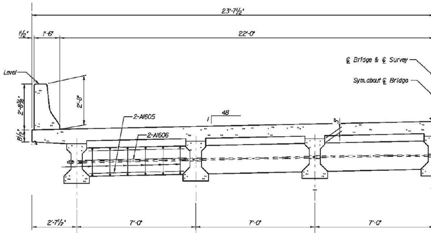
Figure 6.18 Russell Creek Bridge deck cross-section at an interior bent.
