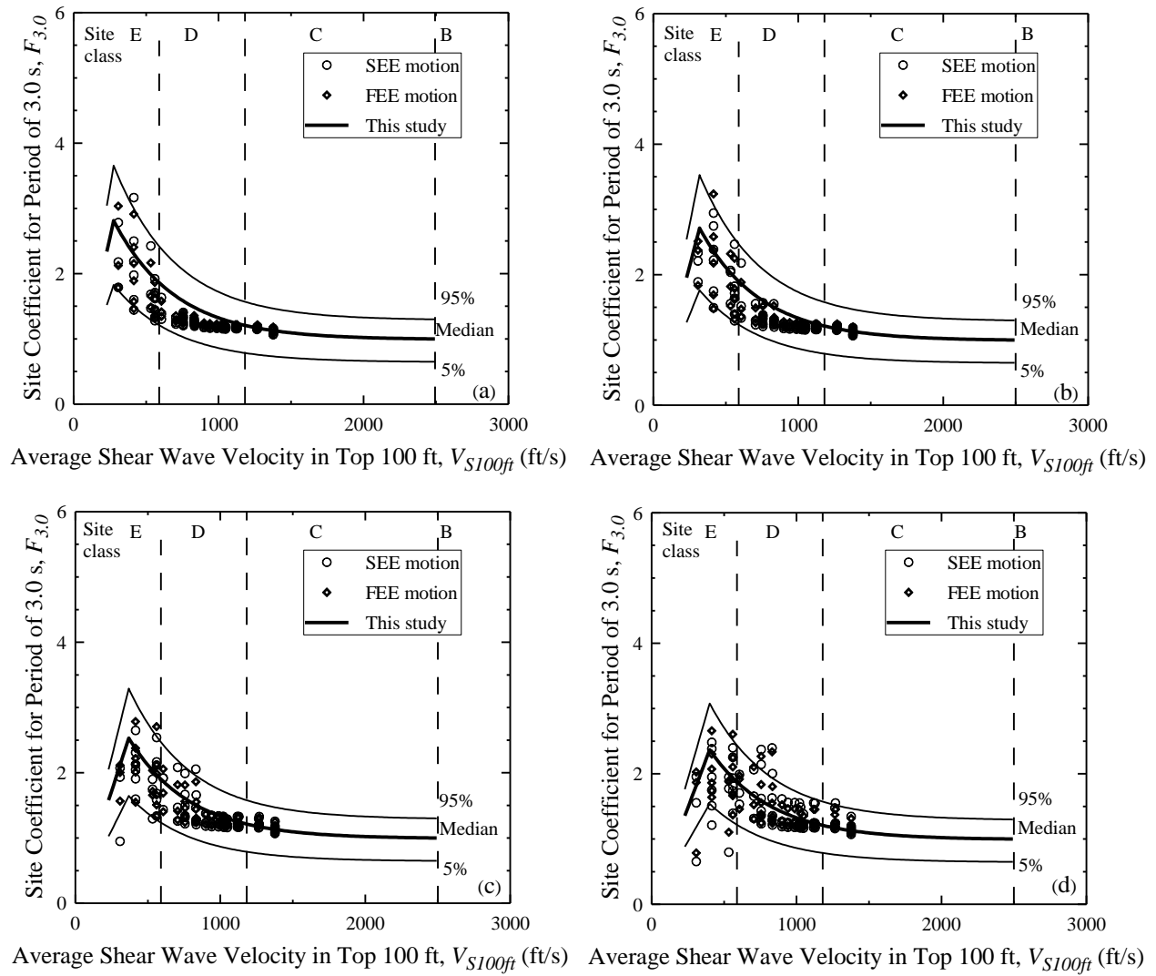
Figure G.6 Site coefficient for 3.0 s spectral period with S_{3.0} equal to (a) 0.01 g, (b) 0.02 g, (c) 0.04 g, and (d) 0.06 g for Lake Marion.
