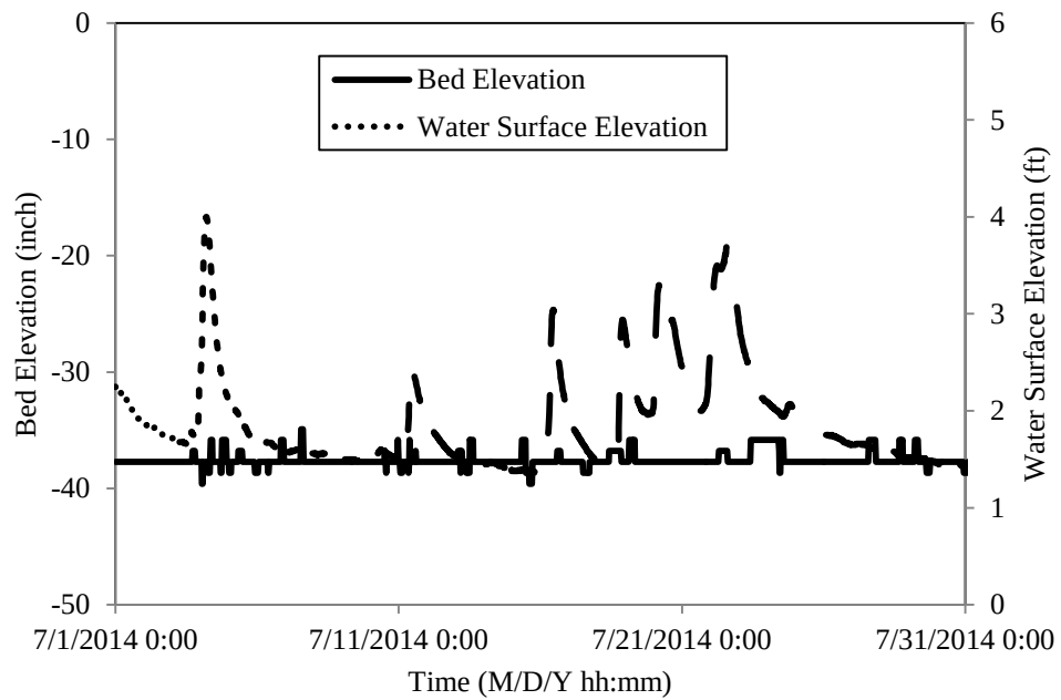
Figure 6.37: Bed elevation from TDR in July 2014.
