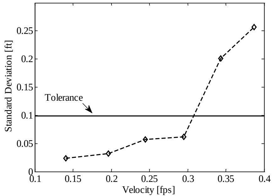
Figure 5.15: Average standard deviation of sonar readings based on Figure 5.14.
