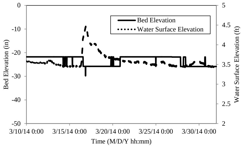
Figure 6.17: Bed elevation from VTP in March 2014.
