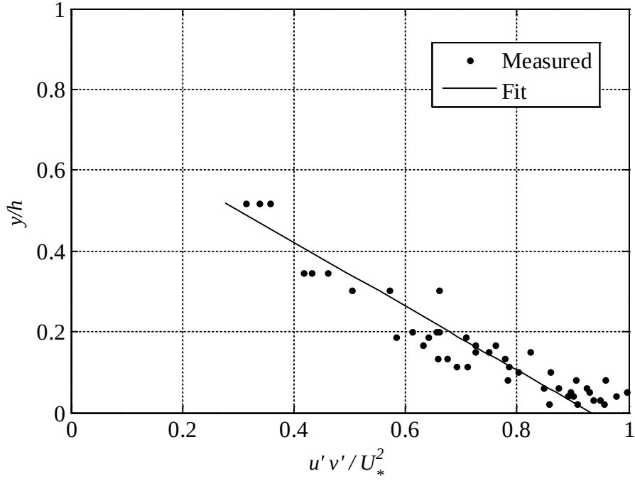
Figure 4.7: Distribution of u'v' as a function of depth in the channel for run 1.
