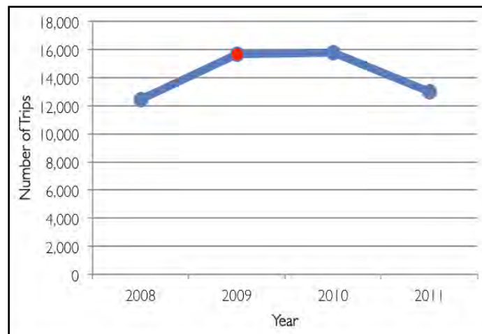
Figure 35. Paratransit Ridership
