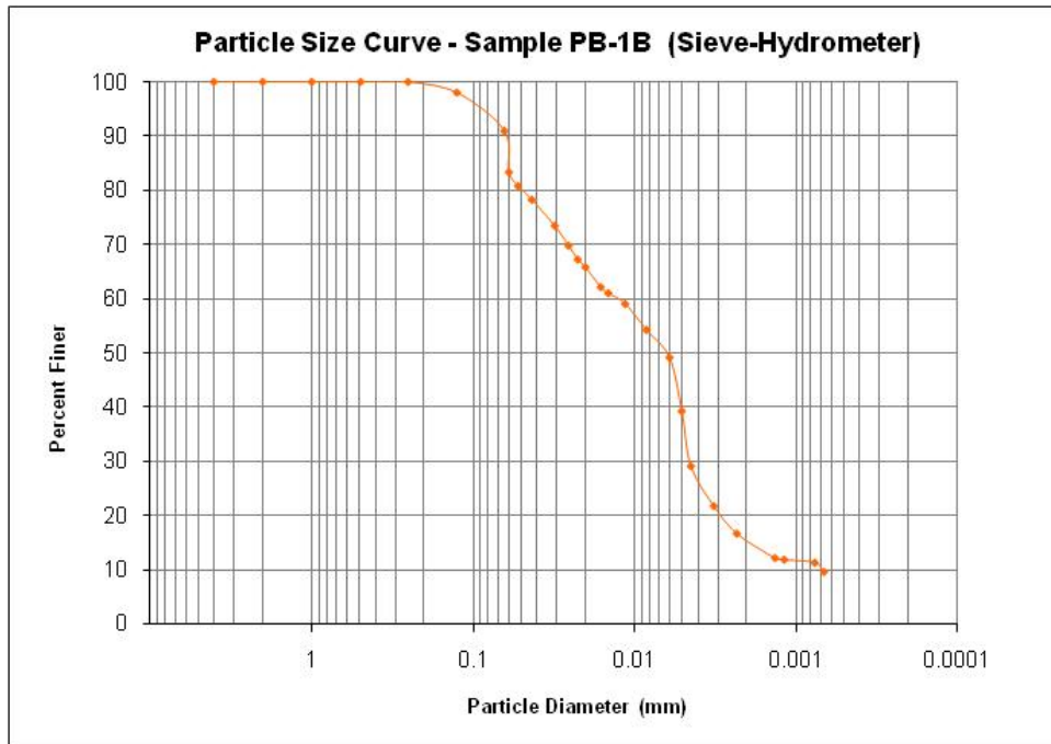
Figure 23 Gradation of PB-1B (Hydrometer)
