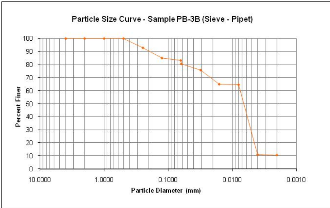
Figure 22 Gradation of PB-3B (Pipette)
