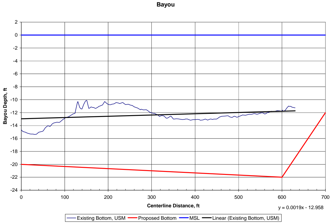
Figure 32 Sediment Trap Profile for Bayou
