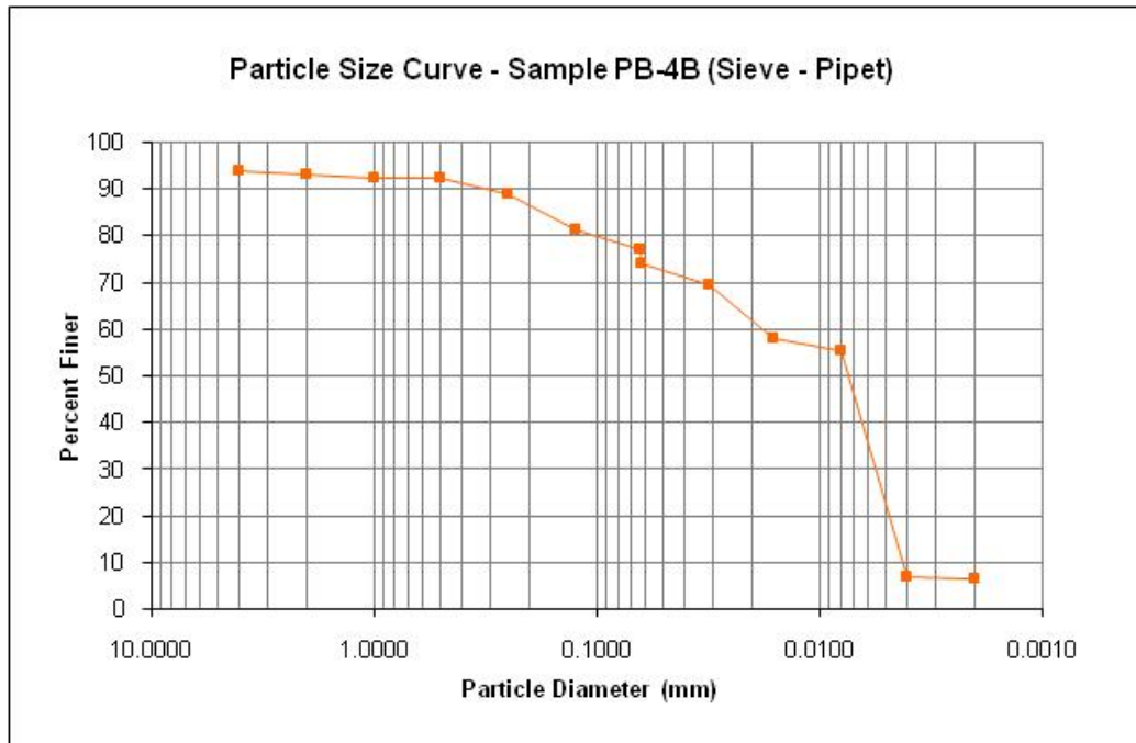
Figure 24 Gradation of PB-4B (Pipette)
