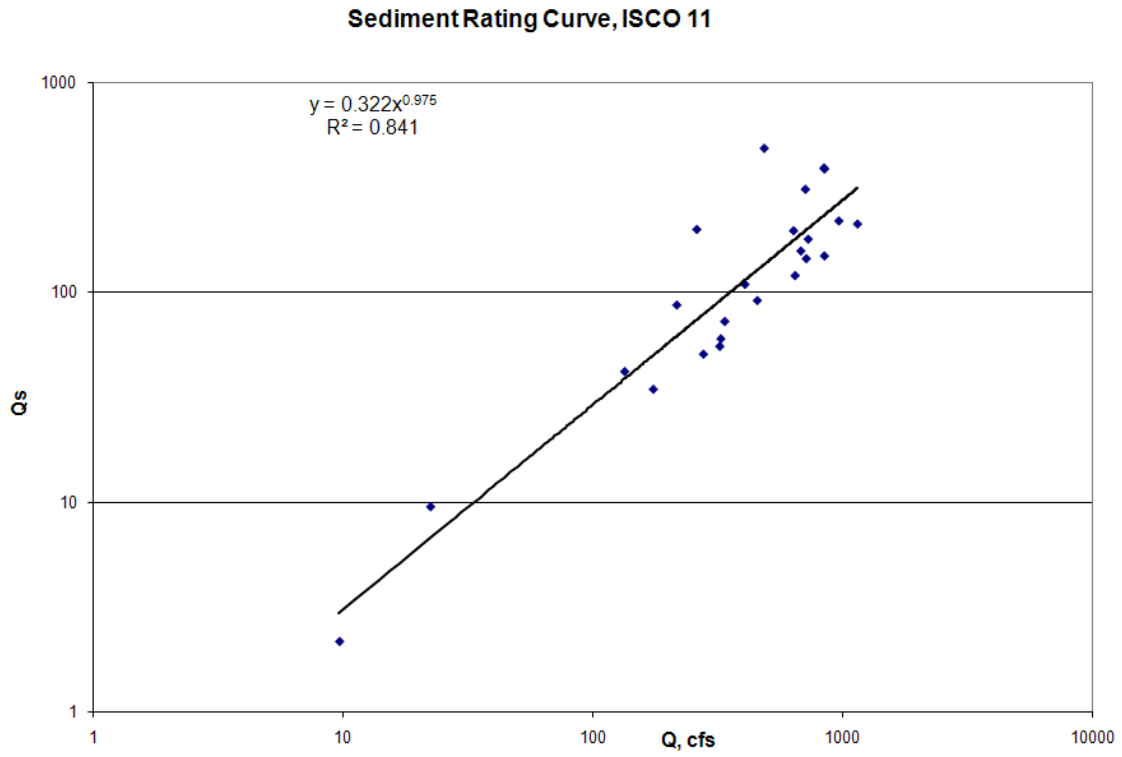
Figure 27 Sediment Rating Curve ISCO 11
