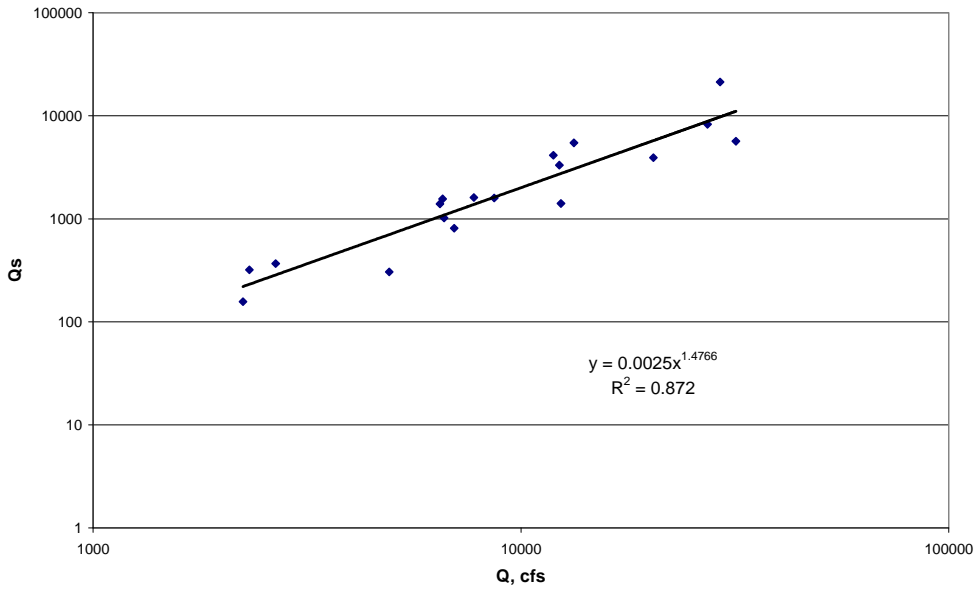
Figure 14 Sediment Rating Curves for the Lower Pearl HUC
