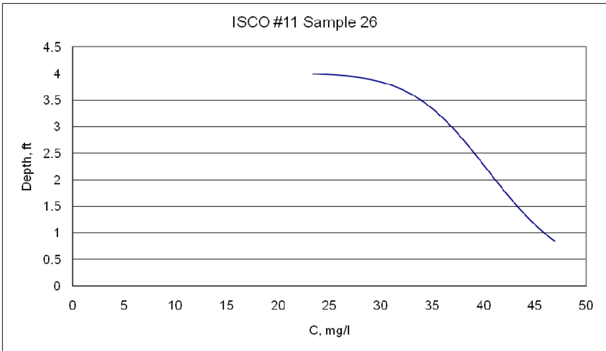
Figure 26 Typical Rouse Profiles for ISCO Samples
