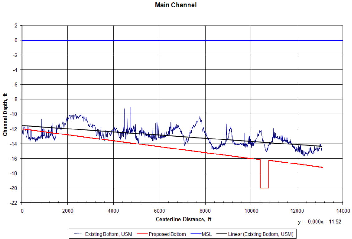
Figure 30 Sediment Trap Profile for Main Channel
