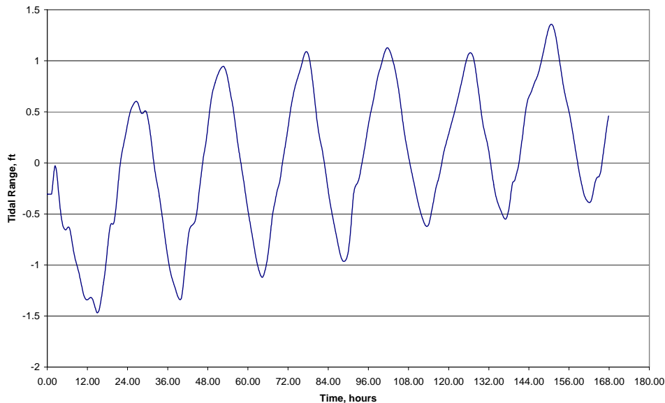
Port Bienville Entrance, ADH Model Tide for Flux Calculator
