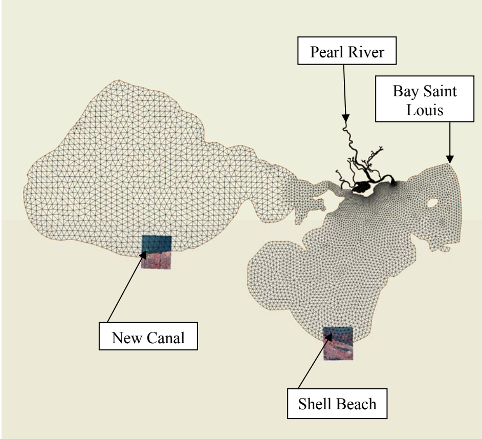
Figure 8 Bienville ADH Mesh with Tidal Station and Boundary Conditions
