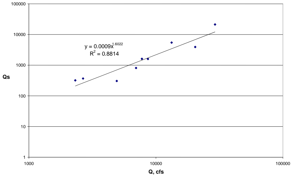
Figure 13 Sediment Rating Curve for the USGS Station 02489500
