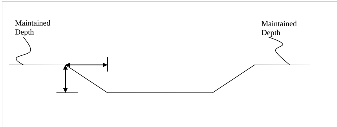
Figure 7-2 - Profile View of Sediment Trap
