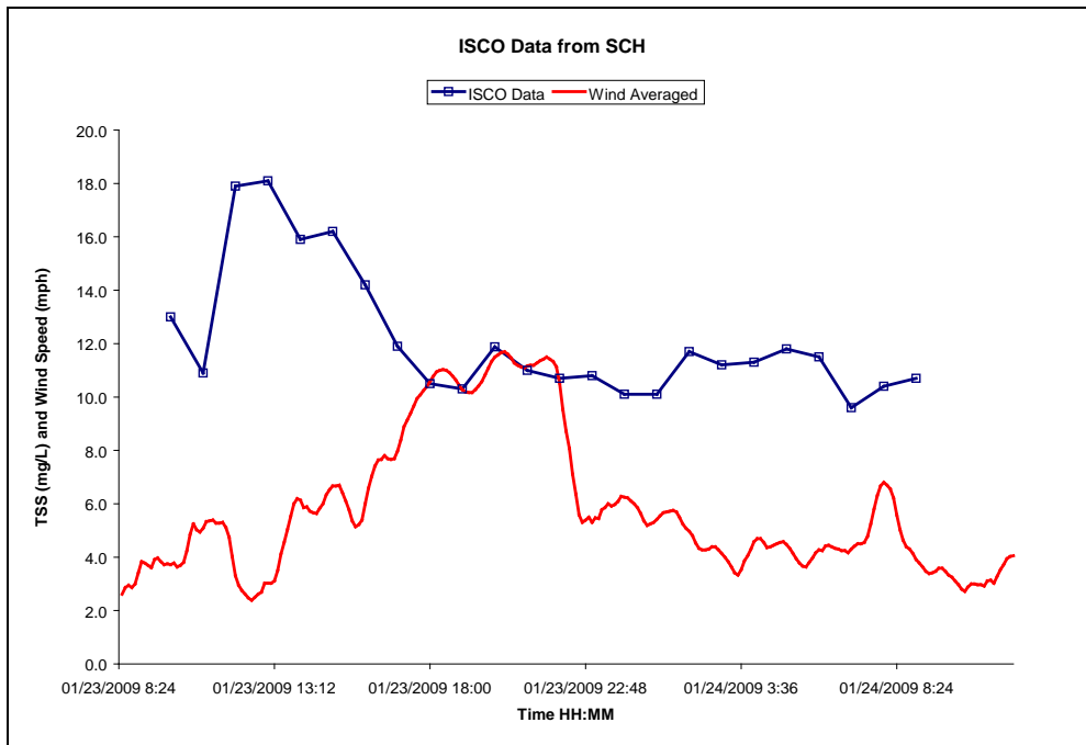
Figure 6: Total suspended solids and wind speed over 24 hours.
