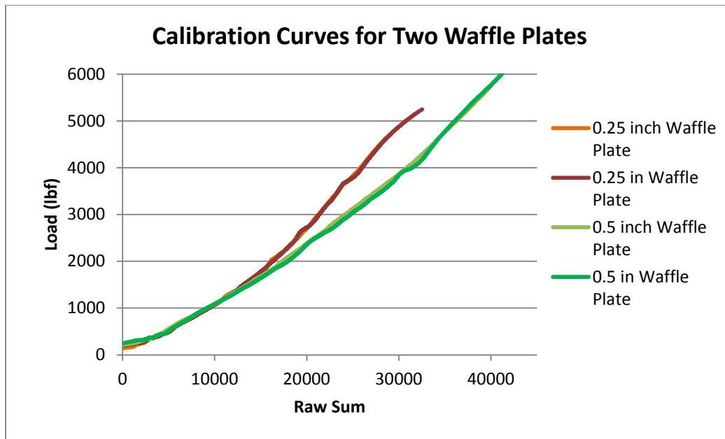
FIGURE 11 Calibration curves for two different waffle plates.
