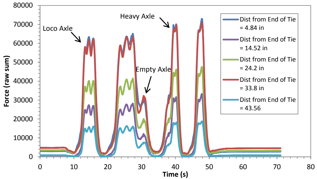
Figure 7.8 – A force vs. time plot for Test 31
