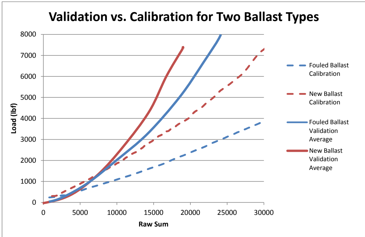
7 FIGURE 10 Validation vs. calibration for two ballast types.
