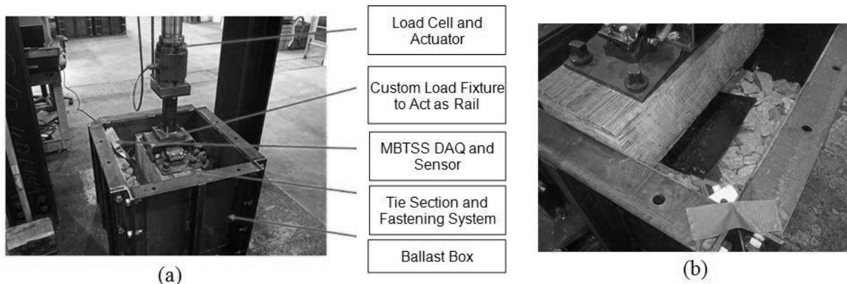
FIGURE 4 (a) Laboratory ballast box test configuration and (b) MBTSS/protection.
