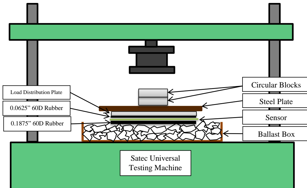
20 21 22 23 24 25 26 27 28 29 30 31 32 33 34 35 36 37 38 FIGURE 8 Validation testing setup. 39
