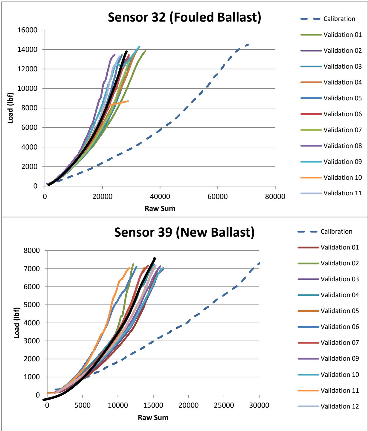
FIGURE 9 Validation tests on a fouled ballast and a new ballast.
