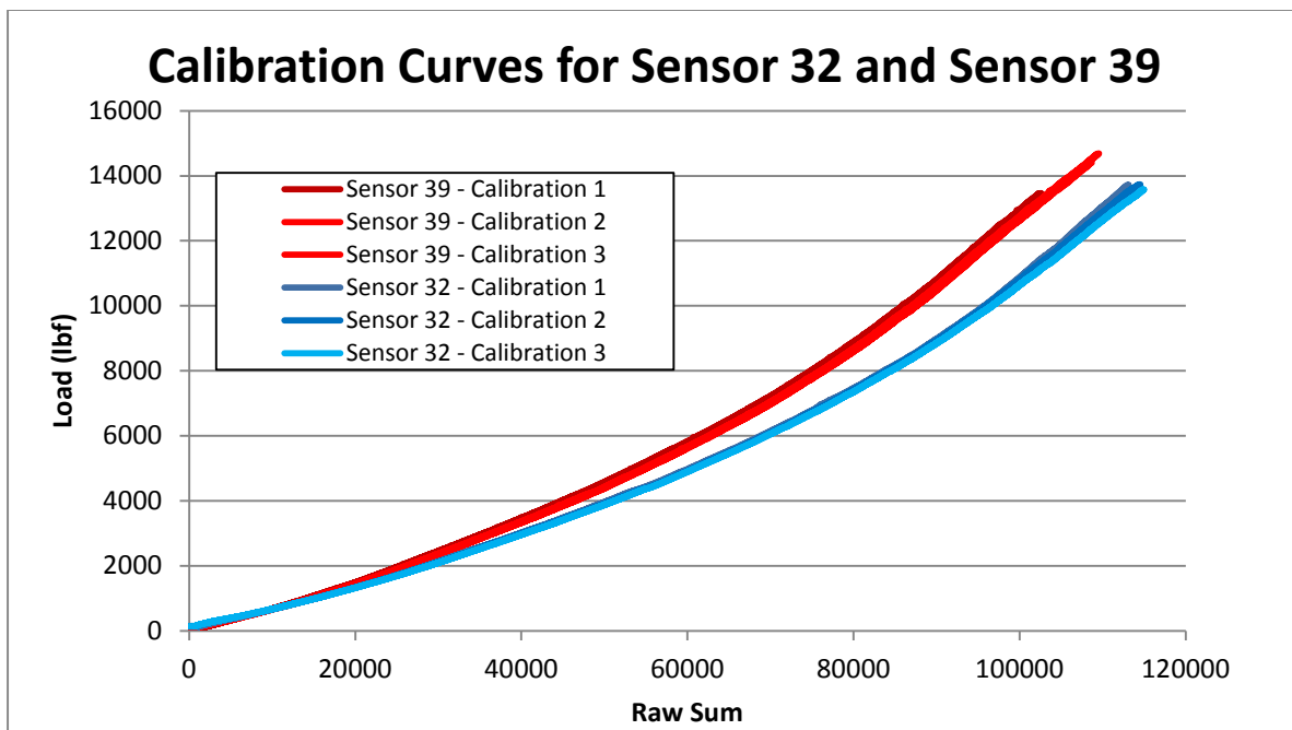
FIGURE 7 Calibration curves for two MBTSS sensors.
