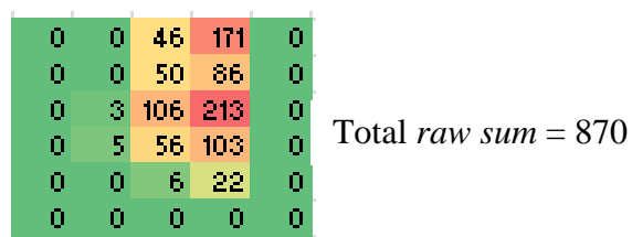
Figure 6.3 – A sample 6x5 pressure distribution with forces shown in raw sum
