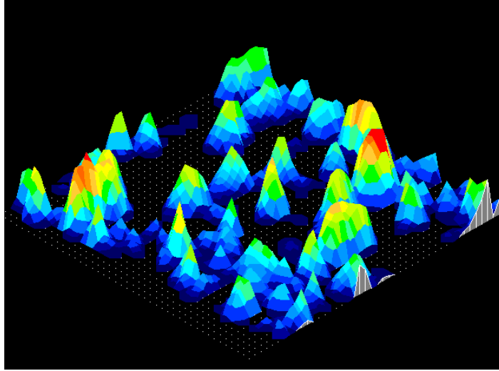
FIGURE 2 A typical ballast-tie pressure distribution.
