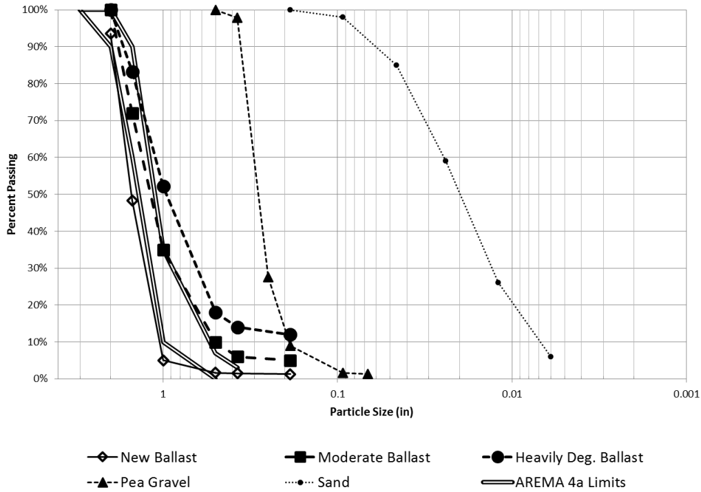
FIGURE 3 Granular material gradations for laboratory testing. (AREMA 4a limits shown for reference)
