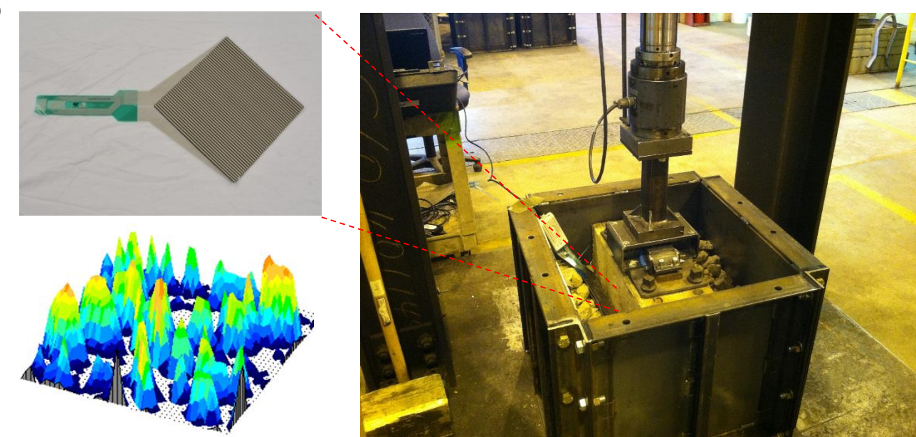
Ballast box testing at TTC
