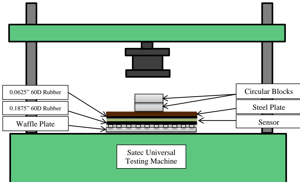
FIGURE 4 Calibration testing setup.
