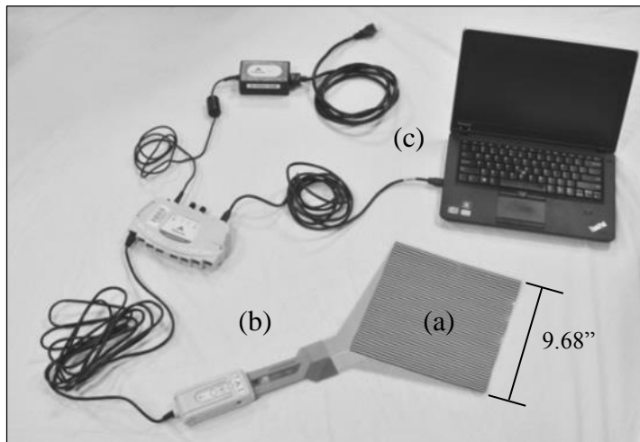
23 24 FIGURE 2 MBTSS system components.
