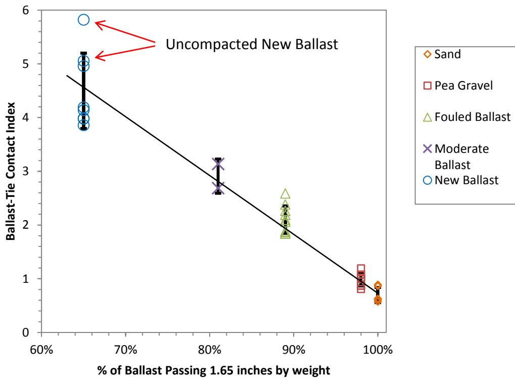
Figure 6.8 BTCI vs. Percent of ballast material passing 1.65 inches for the ballast box laboratory testing at an applied load of 20 kip.
