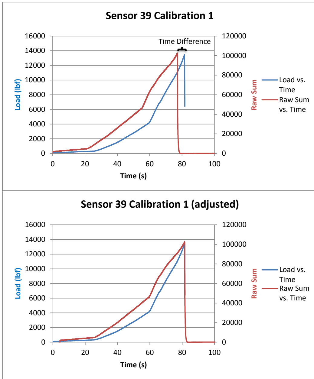
FIGURE 5 Synchronization of MBTSS and load frame data.
