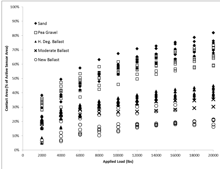
6 FIGURE 6 Contact area versus applied load for the five granular materials.
