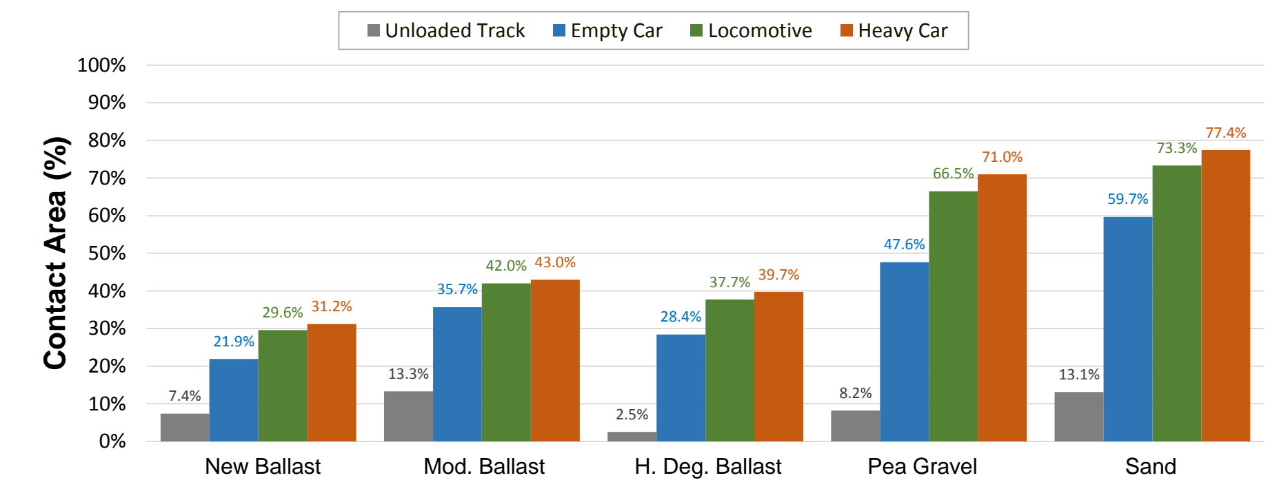
Average contact area in each zone for each applied load
