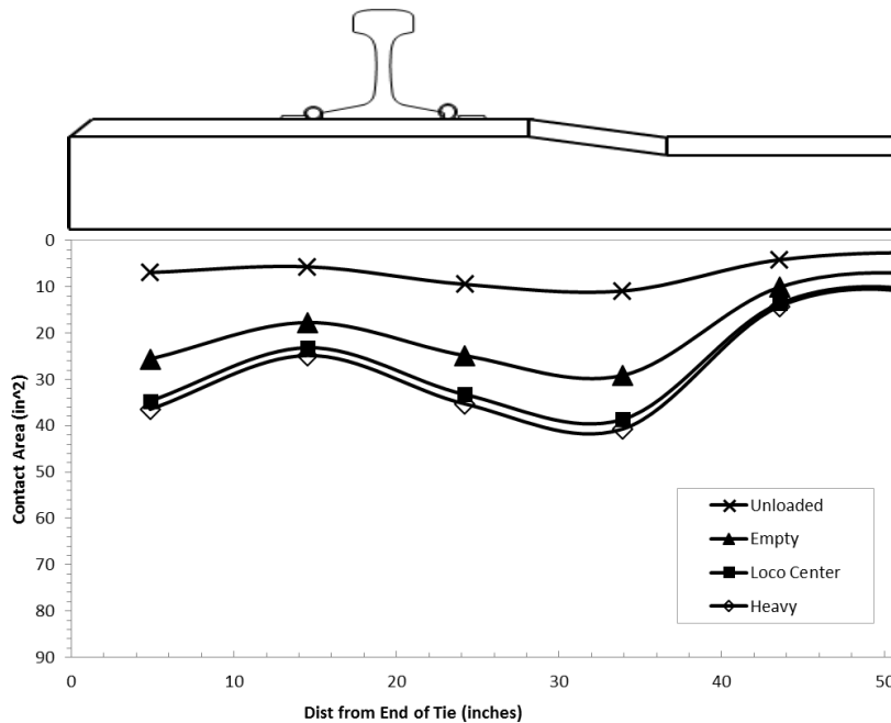
7 8 FIGURE 12 Contact area at each sensor along the length of Tie 40 (new ballast surface). 9
