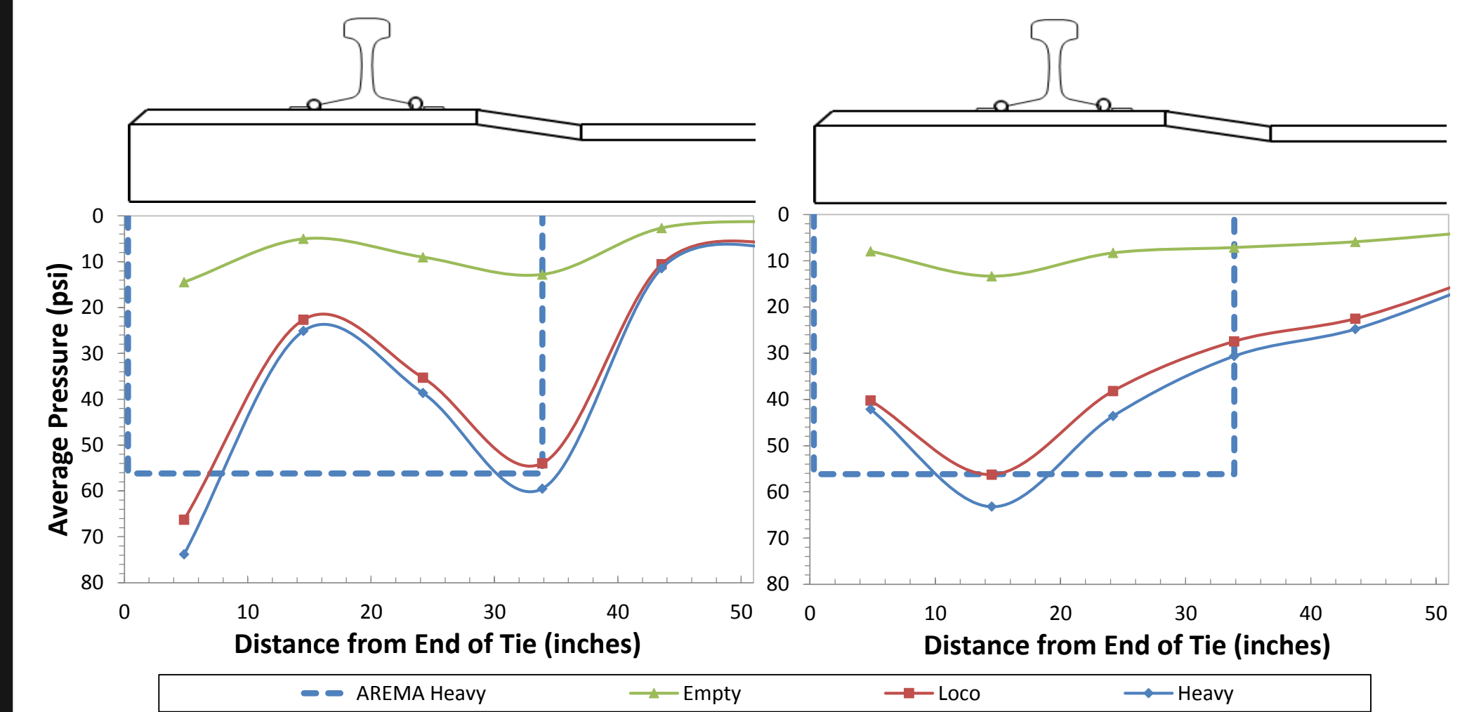
Average pressure distribution for Tie 39 and Tie 3 showing variability in support
