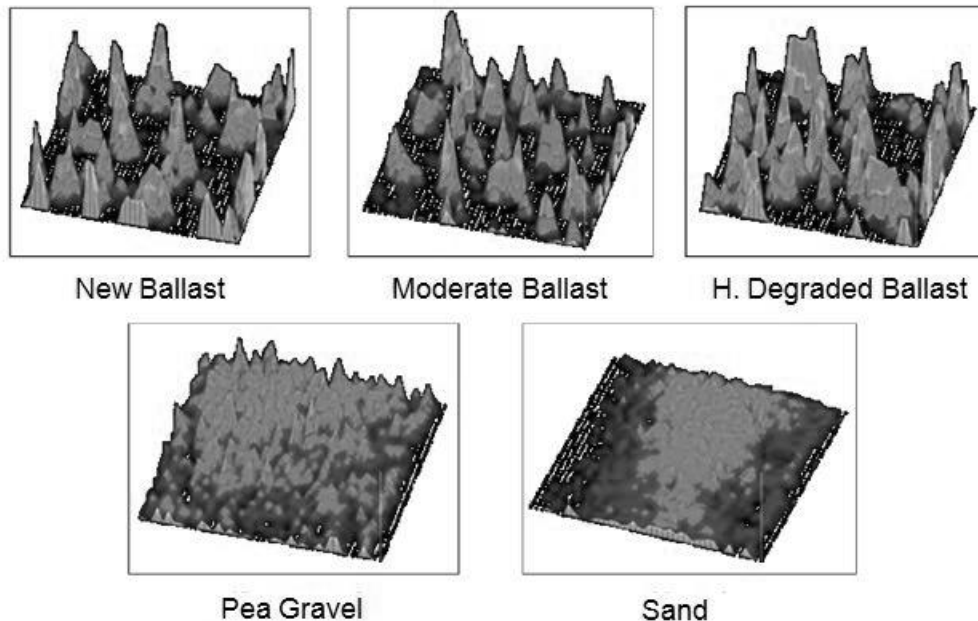
26 27 28 FIGURE 5 A typical qualitative pressure distribution for each of the five granular 29 material reaction surfaces. 30
