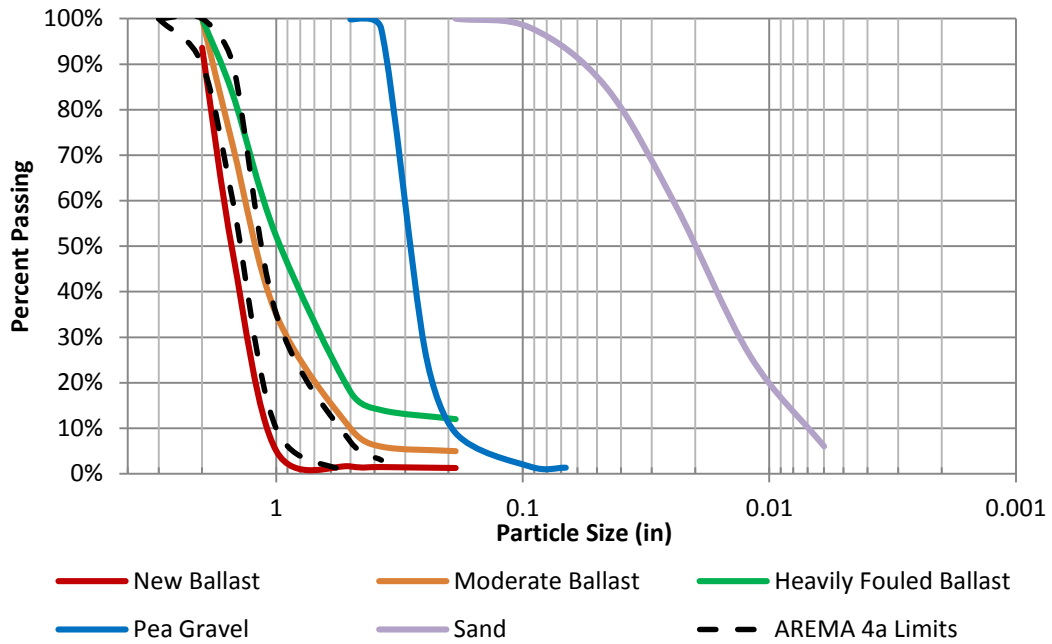
Figure 5.1 Gradations of the five ballasts used in the laboratory ballast box tests After being filled with ballast, the ballast box was installed in the load frame using a fork lift. Figure 5.2 shows a ballast box and buckets of ballast.
