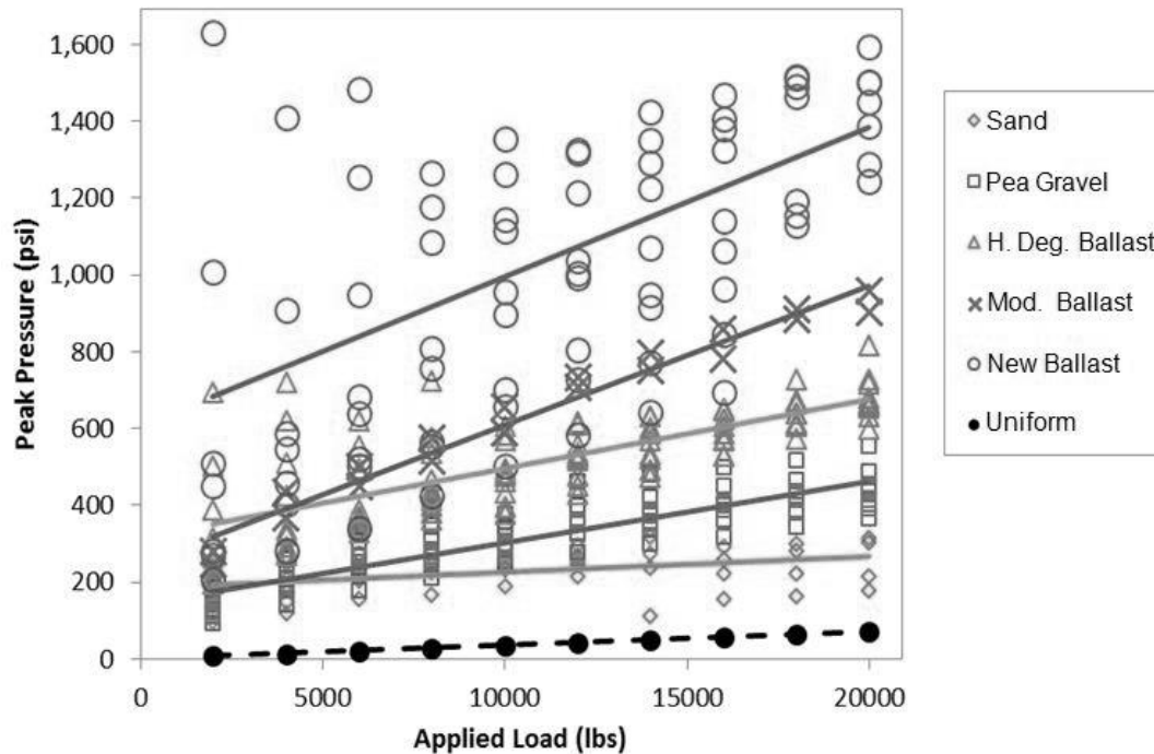
FIGURE 7 Peak pressure versus applied load for the five granular materials.
