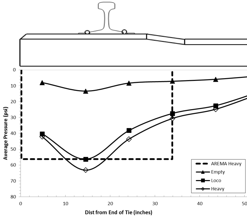
FIGURE 13 Average pressure distribution under Tie 3 (moderately degraded existing ballast) for 3 axle loads.
