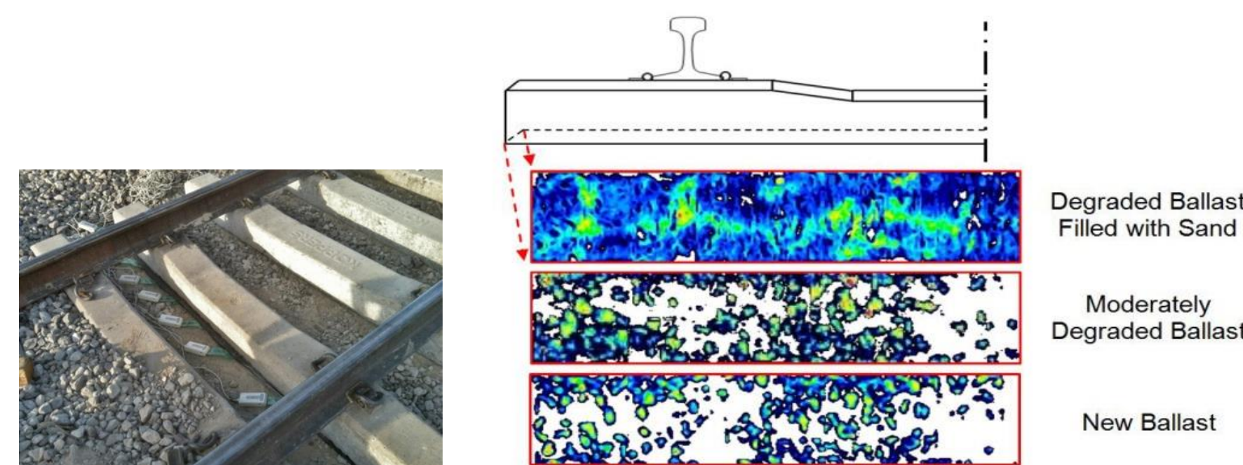
Pressure distributions along the length of three ties for three different ballast surfaces
