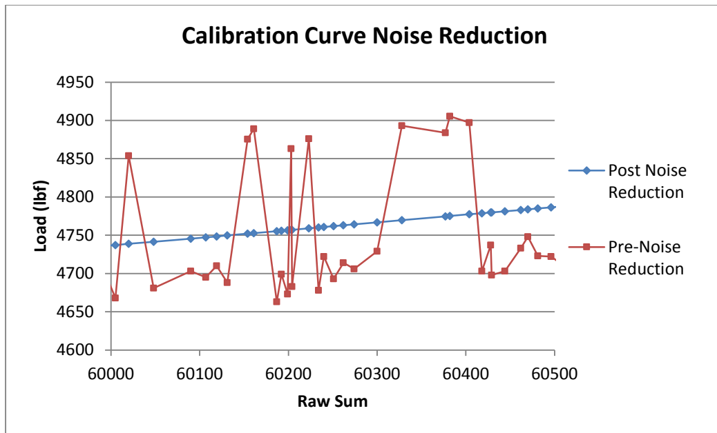
FIGURE 6 Calibration curve noise reduction
