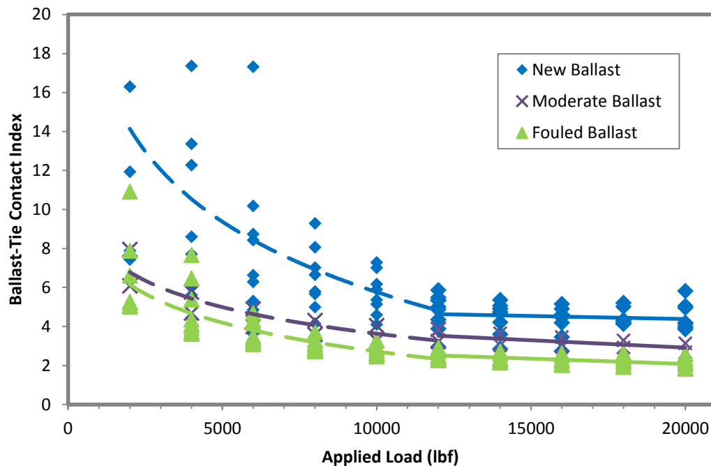
Figure 6.9 BTCI vs. applied load for new ballast, moderate ballast, and fouled ballast and
