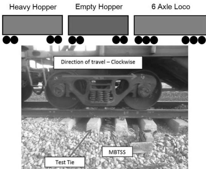
FIGURE 9 Test consist showing a clockwise pass.
