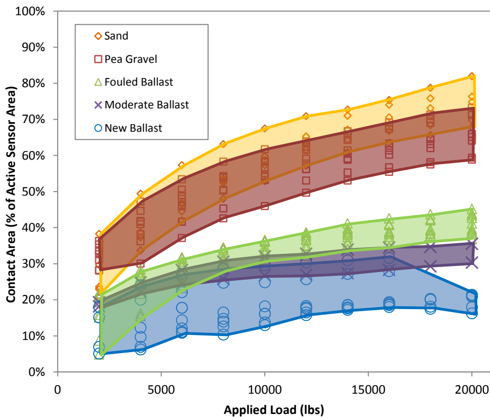
Figure 5.10 Contact area vs. applied load for the five ballast materials used in laboratory testing
