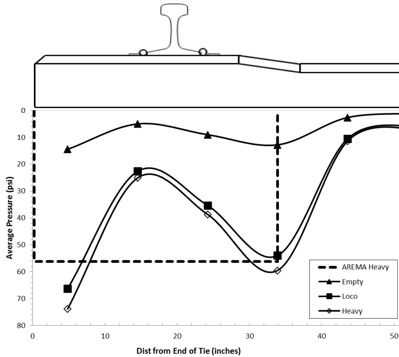
FIGURE 14 Average pressure distribution under Tie 39 (new ballast) for 3 axle loads.
