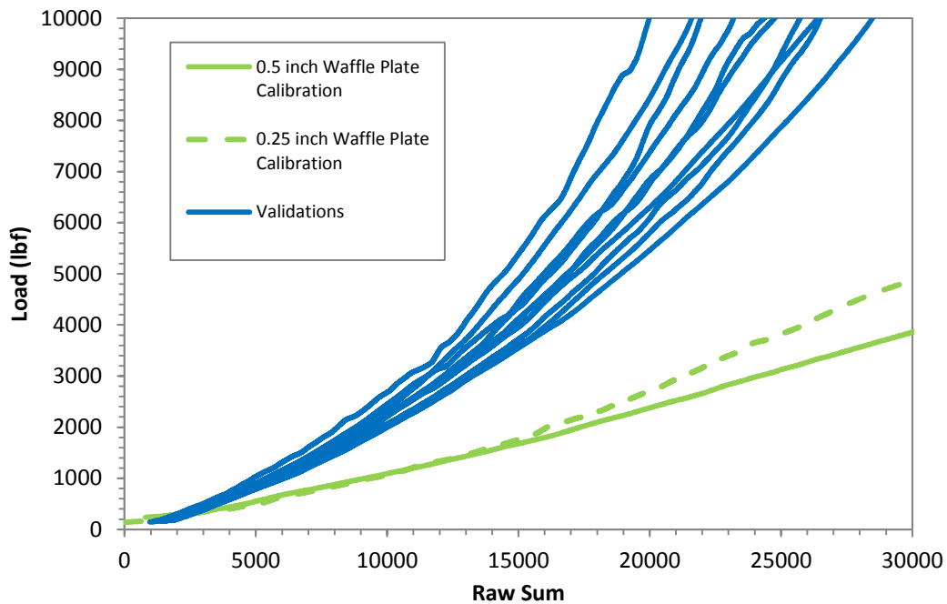
Figure 4.9 The 0.5 inch waffle plate calibration and 0.25 inch waffle plate calibration curves compared to validation curves for fouled ballast.
