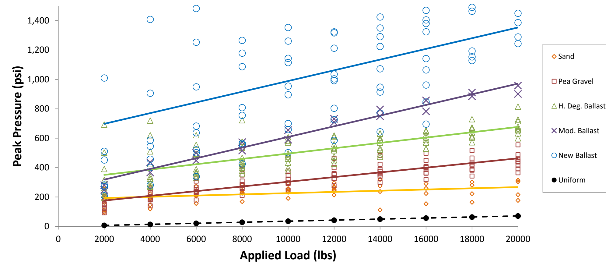
Peak pressure versus applied load for the five different laboratory ballast types
