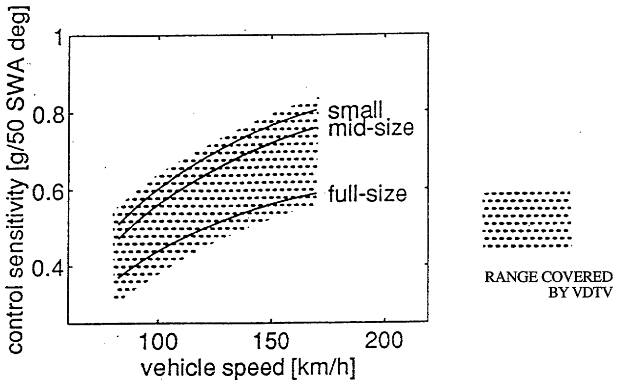
Figure 2. Example of VDTV Lateral Dynamics Emulation Capability
