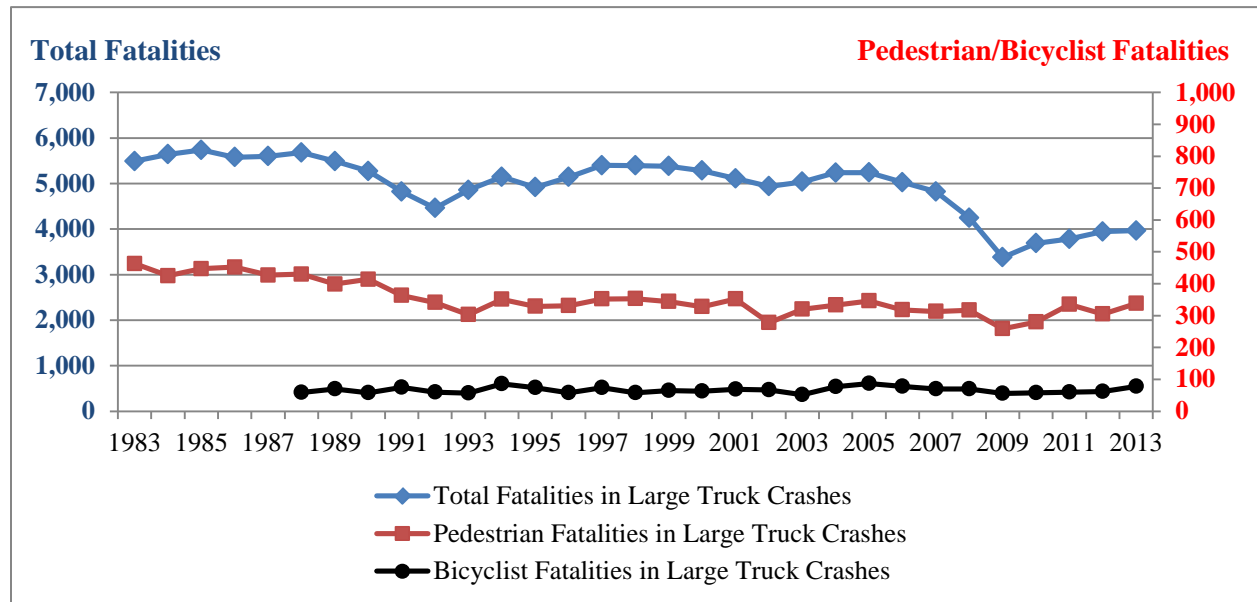
Figure 4. Line graph. Fatality trends in large truck crashes, 1983–2013.
