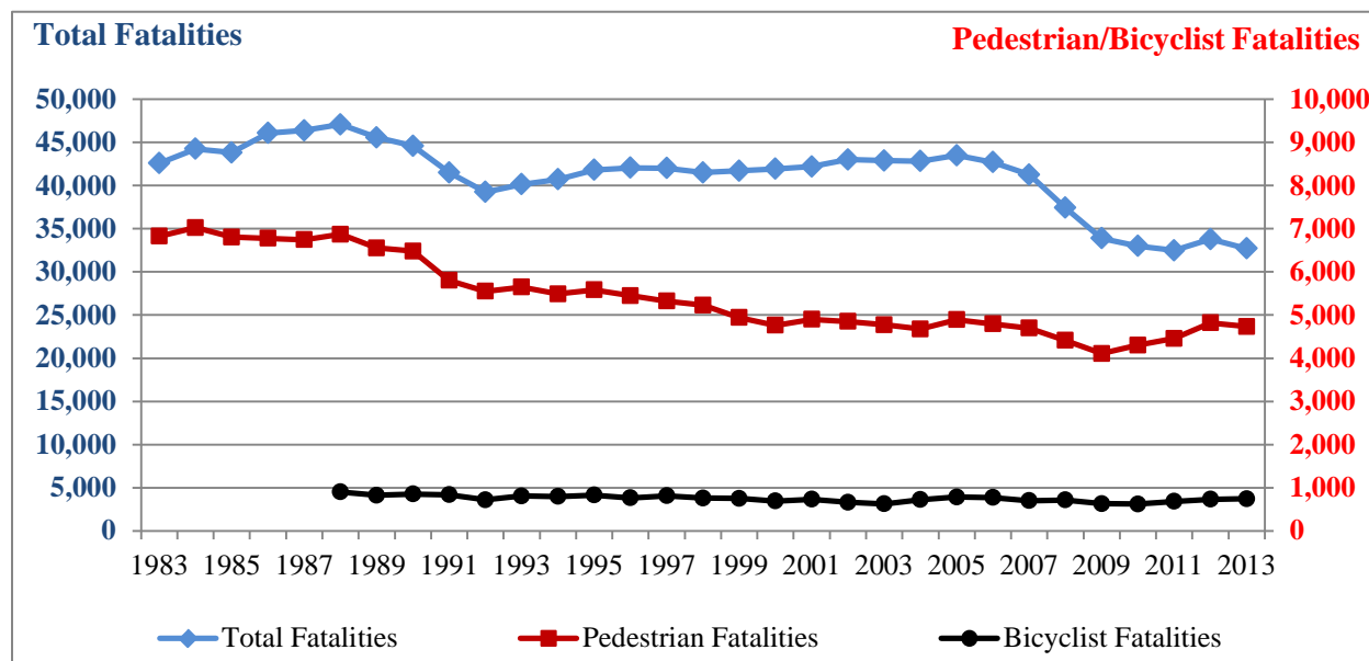
Figure 1. Line graph. Fatality trends in all crashes, 1983–2013.
