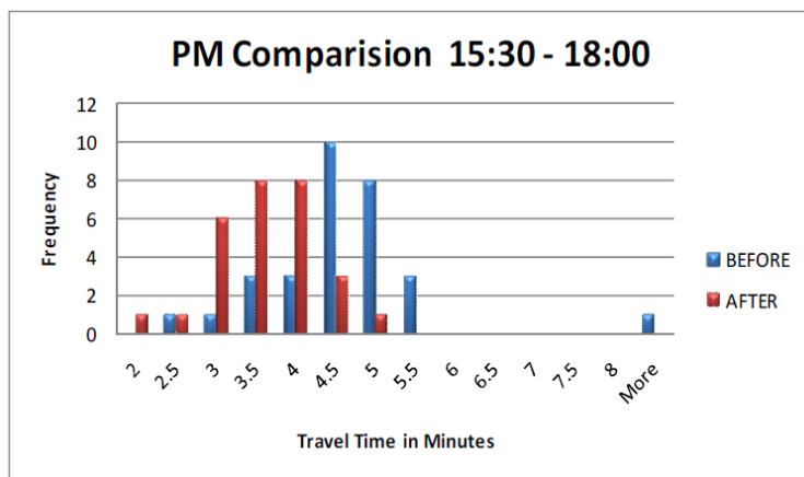
Figure 5 Before and after travel-time histograms for northbound MD 24
