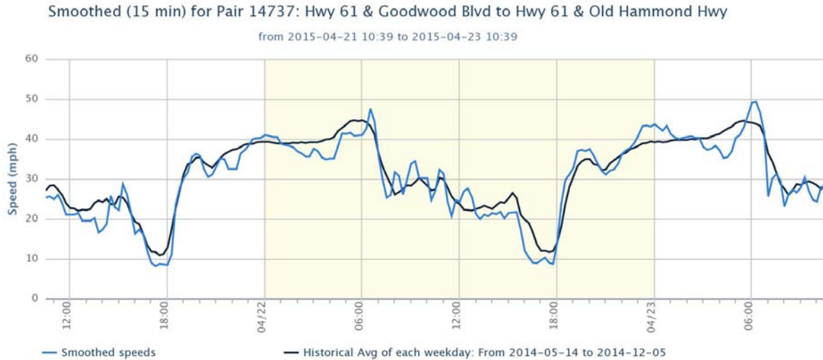
Figure 26 Smoothed speed for segment between Goodwood Blvd and Old Hammond
