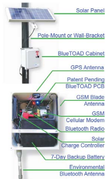
Figure 2 A self-enclosed Bluetooth traffic monitoring device (TrafficCast)
