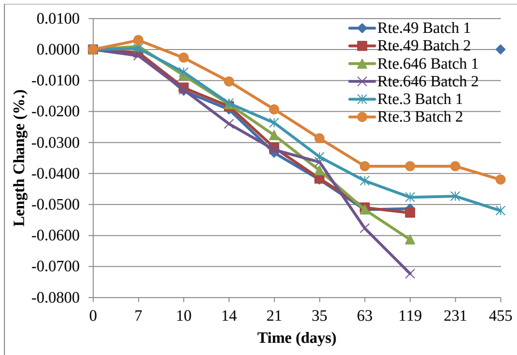
Figure 5. Drying Shrinkage Results for Route 646 Nokesville, Route 49 Crewe, and Route 3 Mathews County
