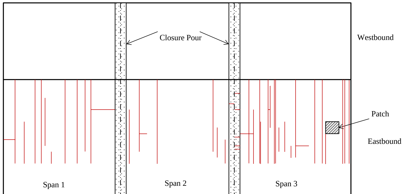
Figure 8. Crack Survey Plots for Route 646 Nokesville (not to scale)
