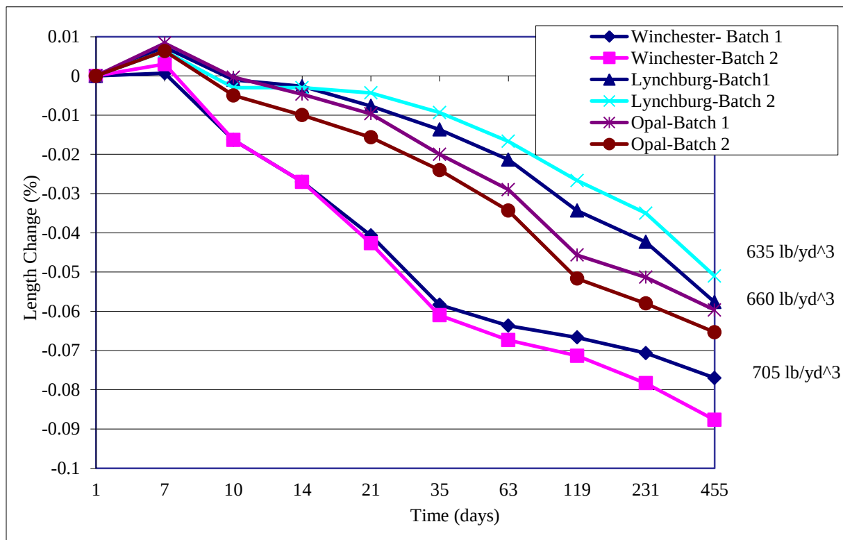
Figure 4. Drying Shrinkage Results for Route 657 Winchester, Route 128 Lynchburg, and Route 15 Opal
