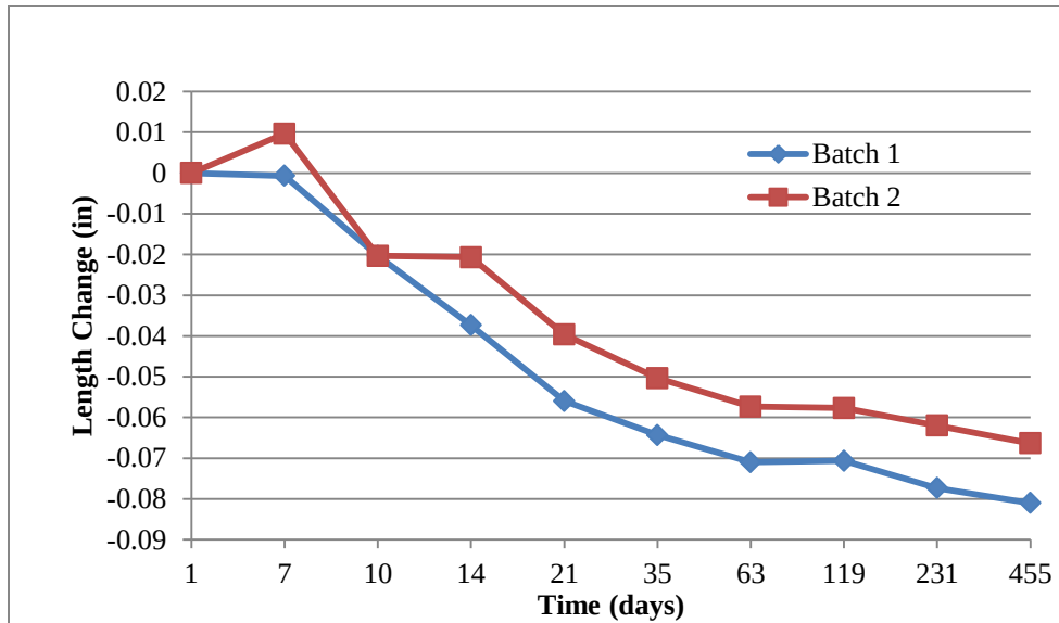
Figure 6. Drying Shrinkage Results for I-95 HOV Lane Stafford
