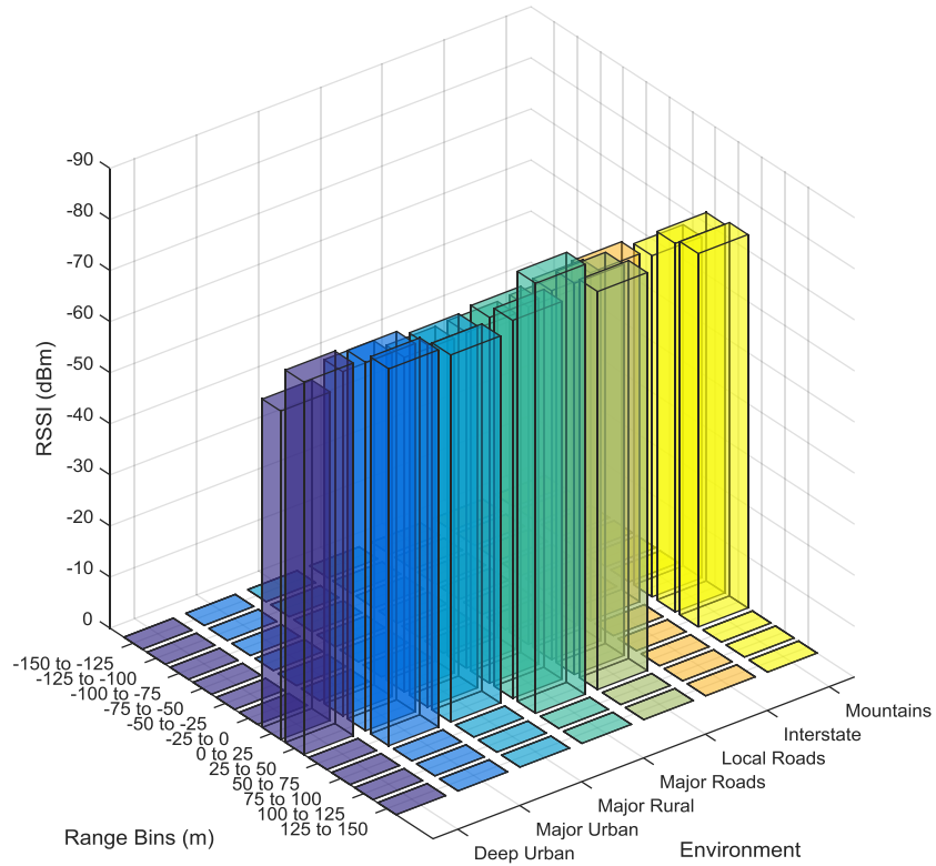
New River Valley Test: RSSI (dBm) Rear Antenna Communicating with Behind Vehicle (No Rider Occlusion) Vehicle Positions: 4-3
