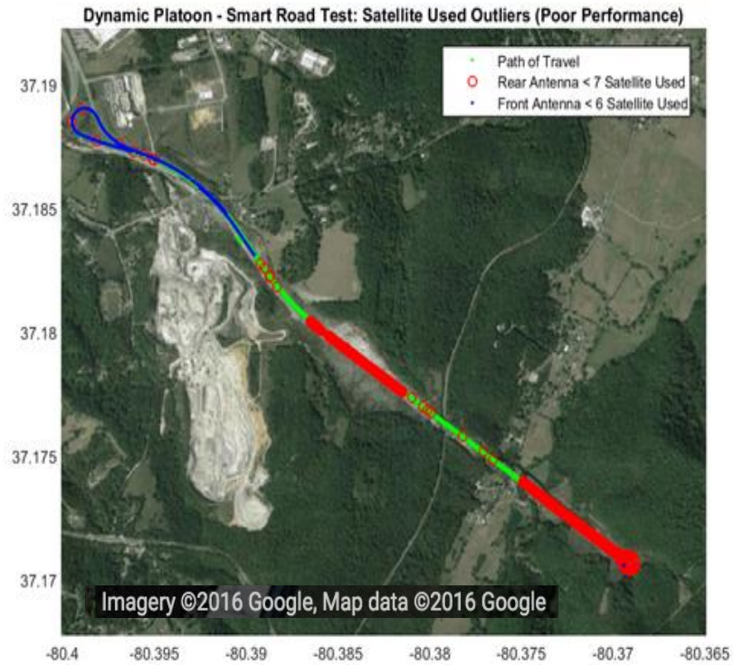
Figure 33. Dynamic platoon in Smart Road – Position performance antenna comparison map.
