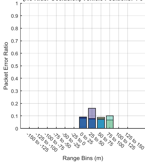
New River Valley Test: Packet Error Ratio vs Range (m) Rear Antenna Communicating with Behind Vehicle (No Rider Occlusion) Vehicle Positions: 4-3
