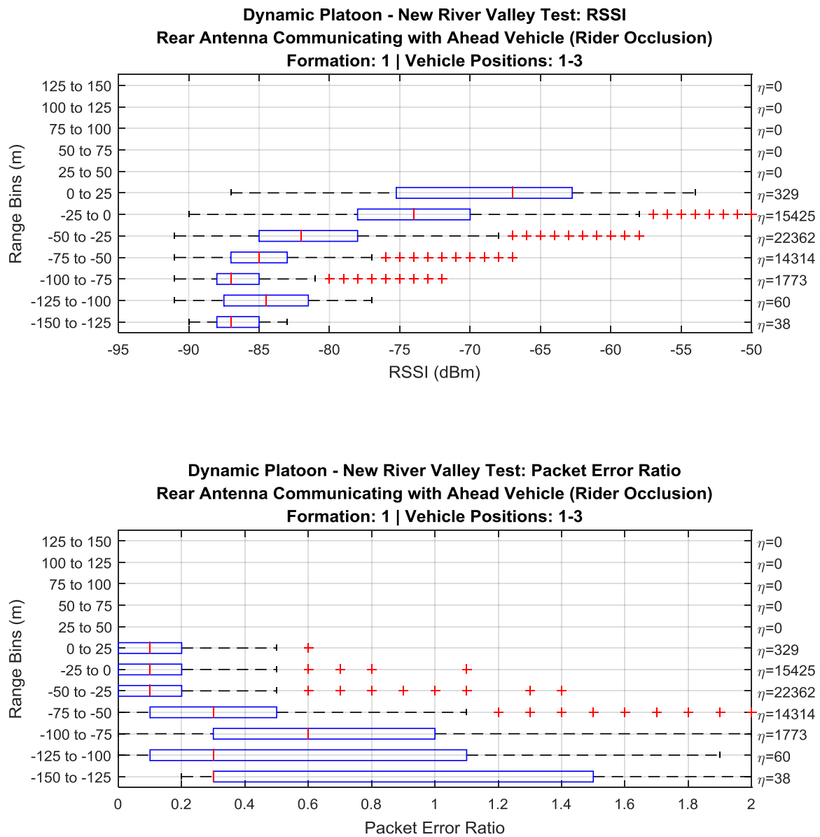
Figure 47. Dynamic platoon in New River Valley – Communication (example).
