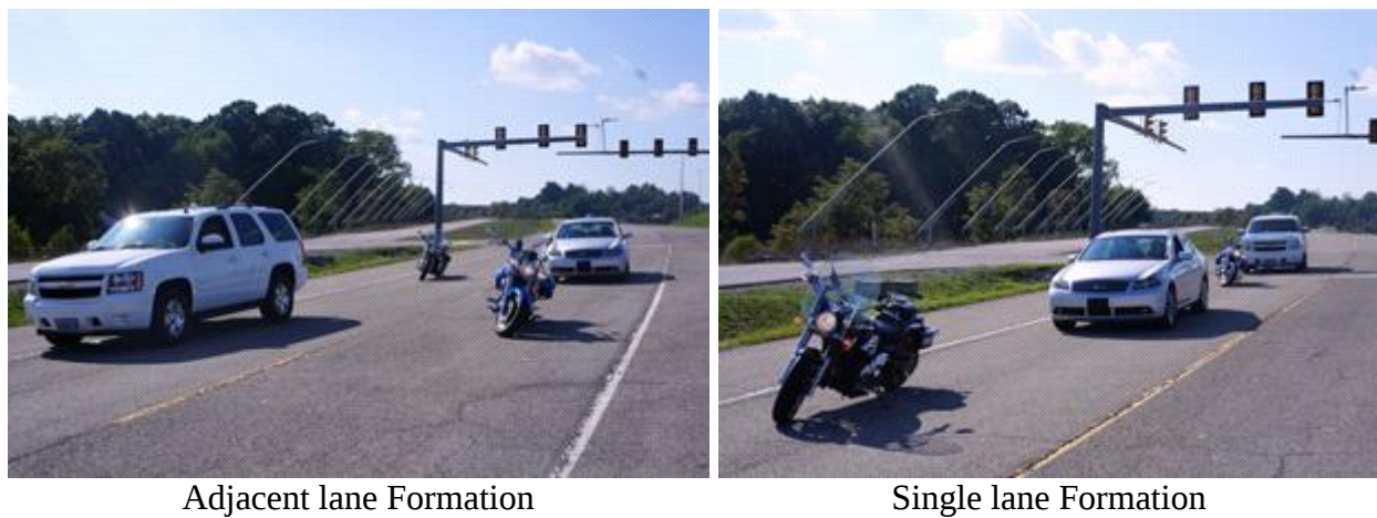
Figure 16. Static dwell test formations on the Virginia Smart Road.
