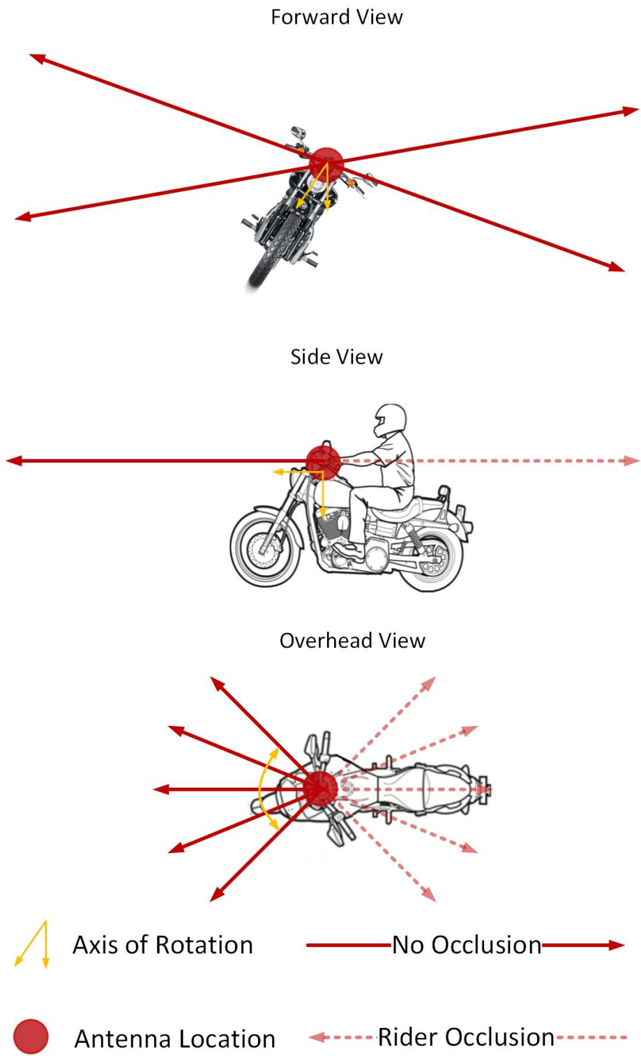
Figure 6. Forward antenna.
