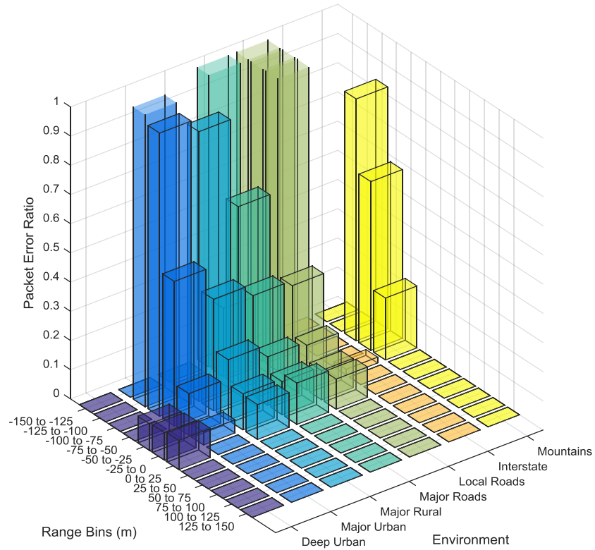
New River Valley Test: Packet Error Ratio Rear Antenna Communicating with Ahead Vehicle (Rider Occlusion) Vehicle Positions: 1-3
