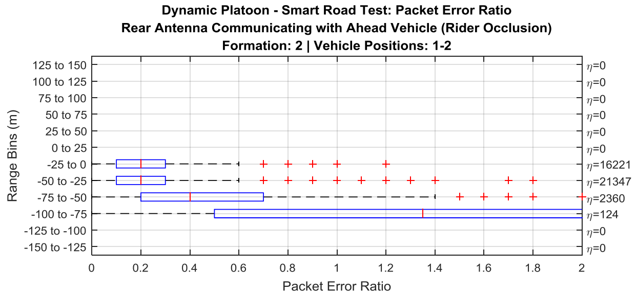
Figure 37. Dynamic platoon in Smart Road – Communication (selected plots).
