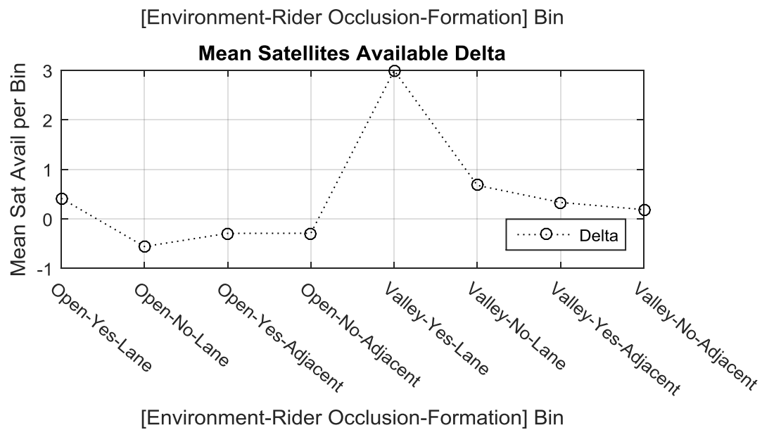
Figure 25. Static dwell test comparison – Satellites available.
