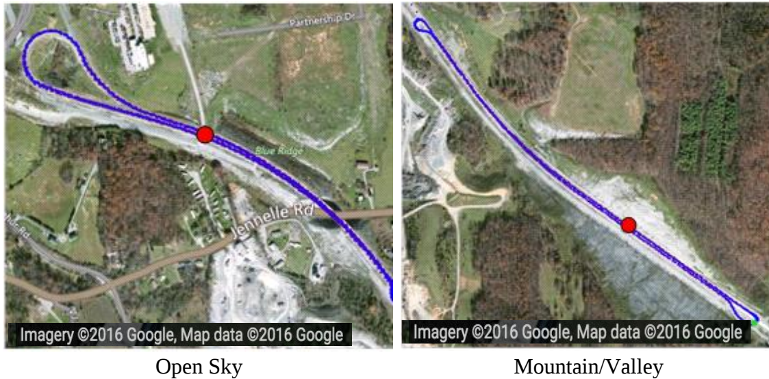
Figure 18. Dynamic range test locations (red dot signifies static vehicle location, blue points signify motorcycle route).
