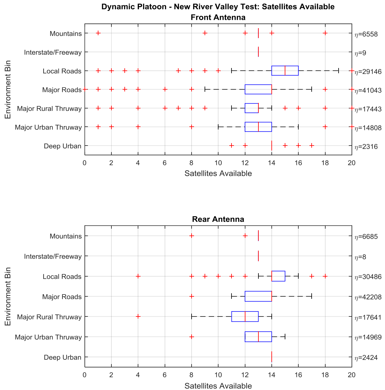
Figure 43. New River Valley Position performance – Satellites available.
