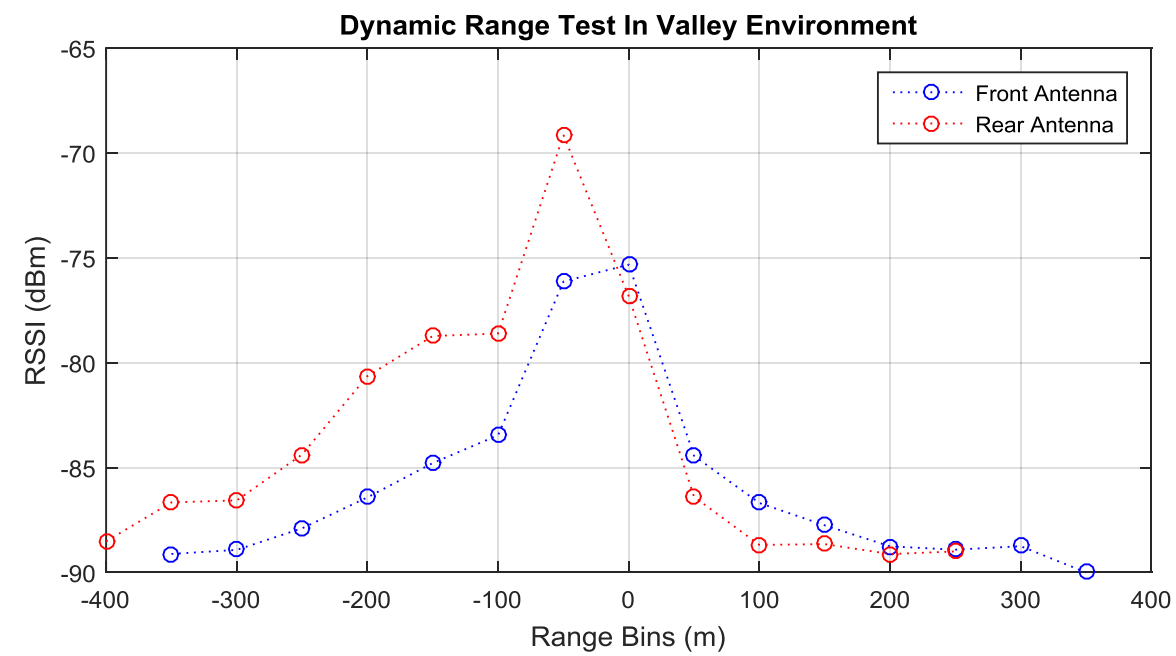
Figure 31. Dynamic ranging communication performance - Antenna comparison.
