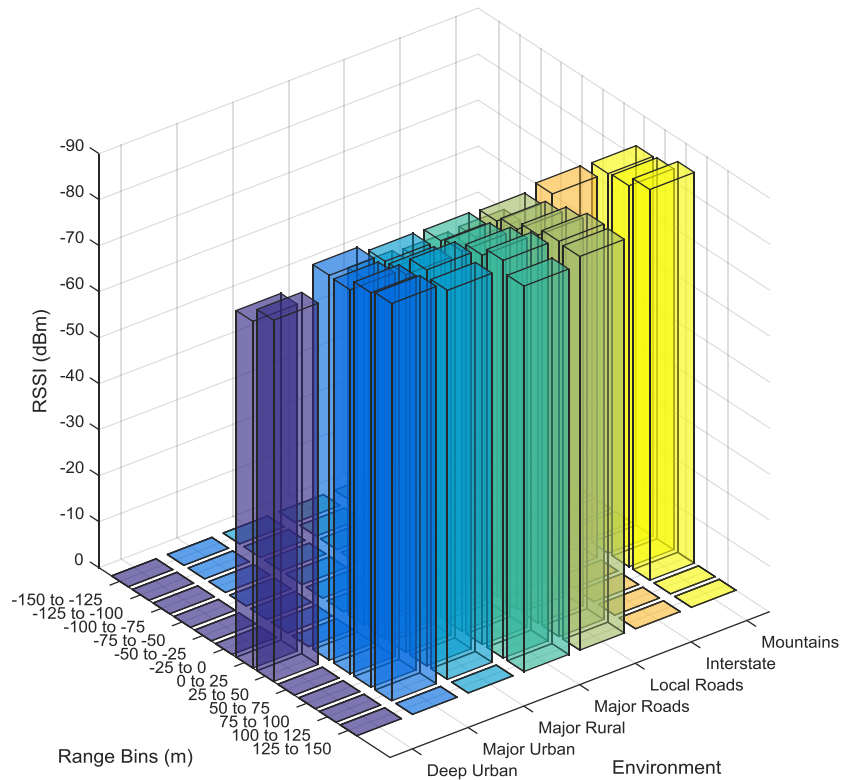
New River Valley Test: RSSI (dBm) Front Antenna Communicating with Behind Vehicle (Rider Occlusion) Vehicle Positions: 4-2
