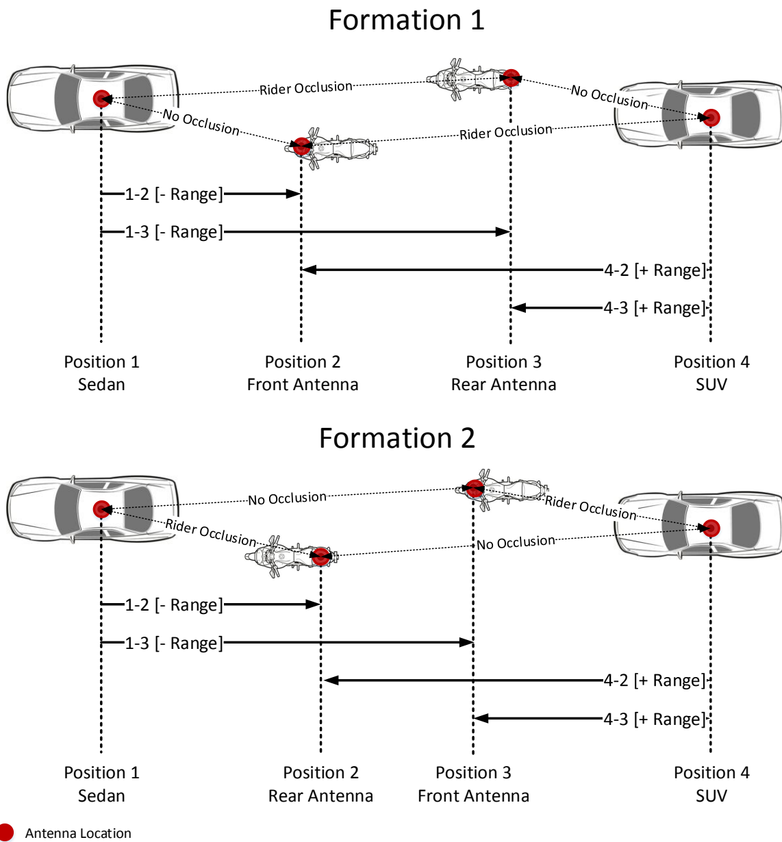
Figure 19. Hypothesized antenna occlusion in platoon.
