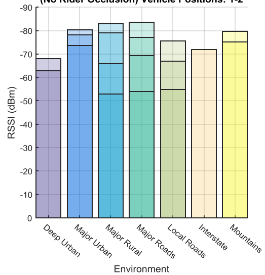
New River Valley Test: RSSI (dBm) vs Environment Front Antenna Communicating with Ahead Vehicle (No Rider Occlusion) Vehicle Positions: 1-2
