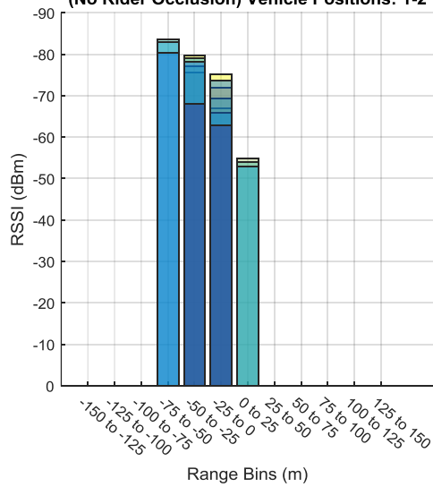
New River Valley Test: RSSI (dBm) vs Range (m) Front Antenna Communicating with Ahead Vehicle (No Rider Occlusion) Vehicle Positions: 1-2
