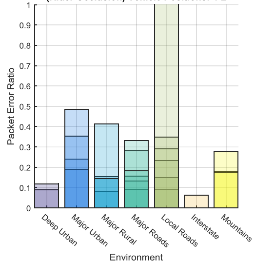
New River Valley Test: Packet Error Ratio vs Environment Front Antenna Communicating with Behind Vehicle (Rider Occlusion) Vehicle Positions: 4-2
