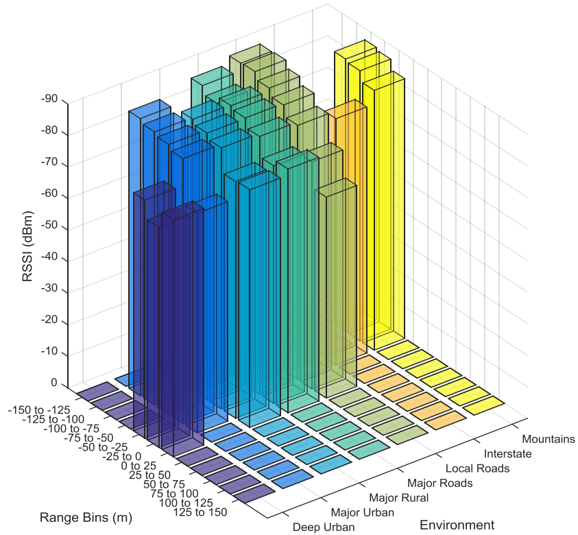
New River Valley Test: RSSI (dBm) Rear Antenna Communicating with Ahead Vehicle (Rider Occlusion) Vehicle Positions: 1-3
