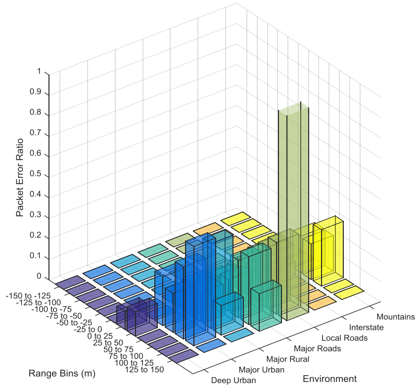
New River Valley Test: Packet Error Ratio Front Antenna Communicating with Behind Vehicle (Rider Occlusion) Vehicle Positions: 4-2
