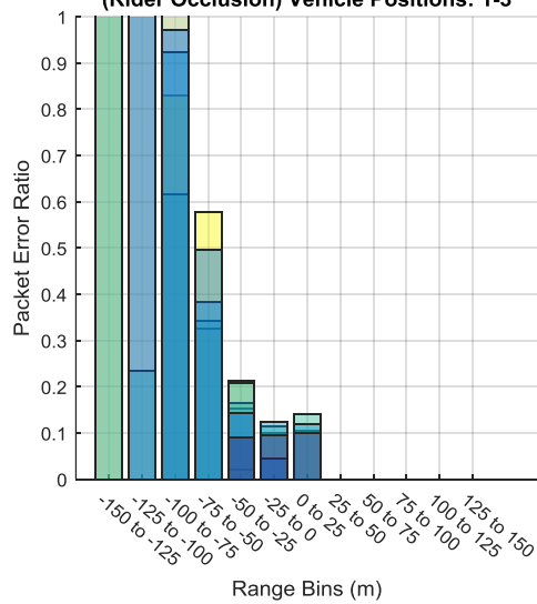
New River Valley Test: Packet Error Ratio vs Range (m) Rear Antenna Communicating with Ahead Vehicle (Rider Occlusion) Vehicle Positions: 1-3
