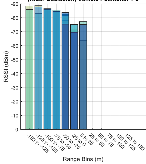
New River Valley Test: RSSI (dBm) vs Range (m) Rear Antenna Communicating with Ahead Vehicle (Rider Occlusion) Vehicle Positions: 1-3
