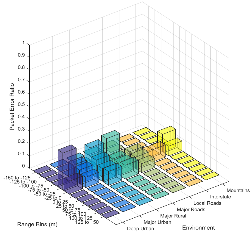
New River Valley Test: Packet Error Ratio Front Antenna Communicating with Ahead Vehicle (No Rider Occlusion) Vehicle Positions: 1-2
