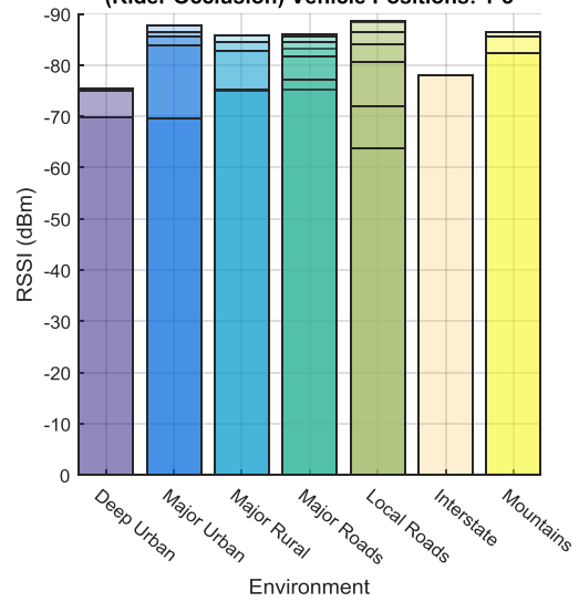
New River Valley Test: RSSI (dBm) vs Environment Rear Antenna Communicating with Ahead Vehicle (Rider Occlusion) Vehicle Positions: 1-3
