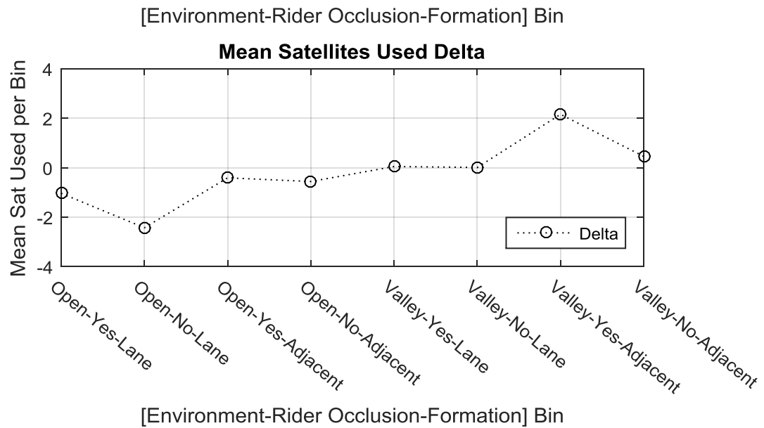
Figure 24. Static dwell test comparison – Satellites used.
