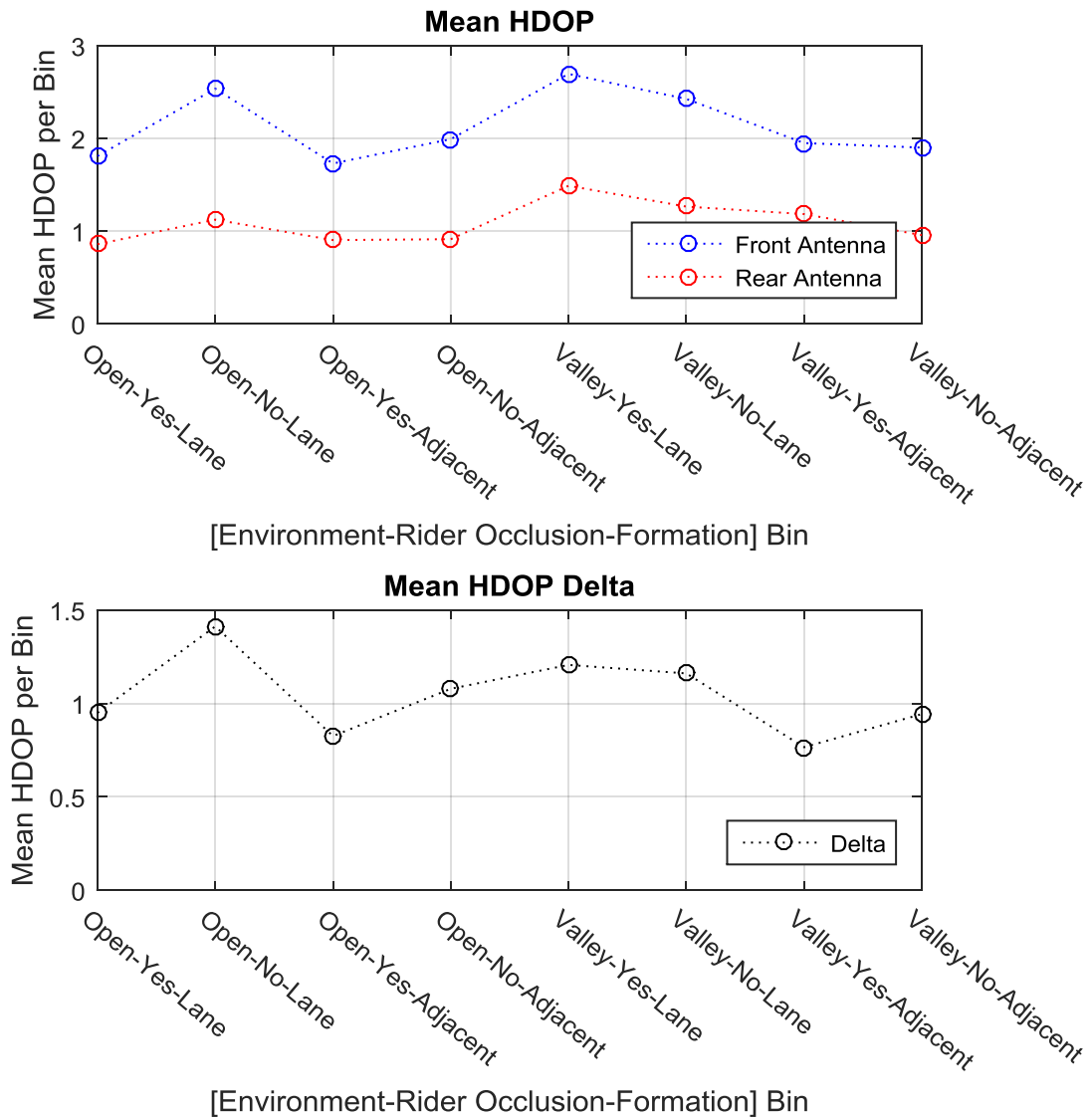
Figure 23. Static dwell test comparison – HDOP.
