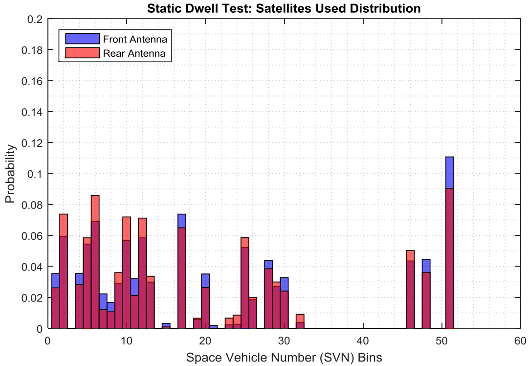
Figure 26. Static dwell test – Space vehicles used distribution.
