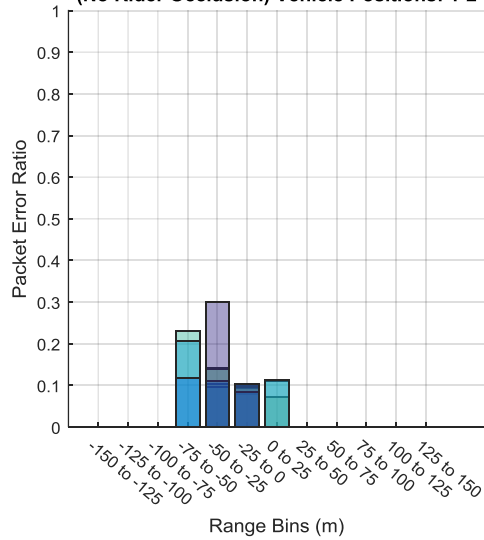
New River Valley Test: Packet Error Ratio vs Range (m) Front Antenna Communicating with Ahead Vehicle (No Rider Occlusion) Vehicle Positions: 1-2
