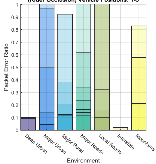
New River Valley Test: Packet Error Ratio vs Environment Rear Antenna Communicating with Ahead Vehicle (Rider Occlusion) Vehicle Positions: 1-3
