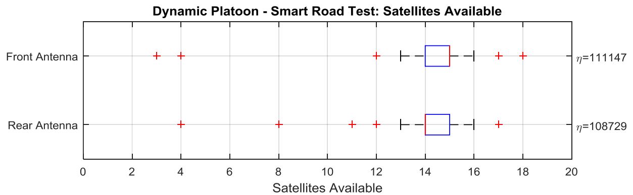
Figure 32. Dynamic platoon in Smart Road – Position performance antenna comparison box plot.
