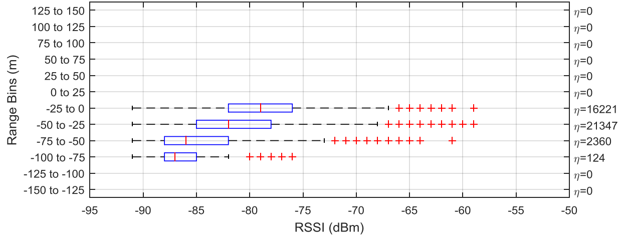
Dynamic Platoon - Smart Road Test: RSSI Rear Antenna Communicating with Ahead Vehicle (Rider Occlusion) Formation: 2 | Vehicle Positions: 1-2
