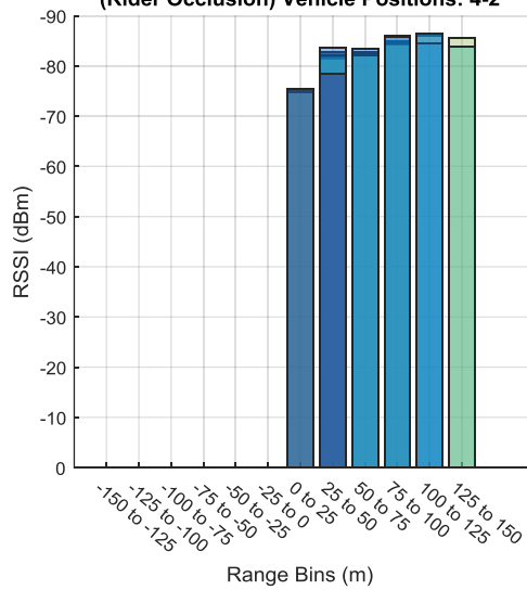
New River Valley Test: RSSI (dBm) vs Range (m) Front Antenna Communicating with Behind Vehicle (Rider Occlusion) Vehicle Positions: 4-2
