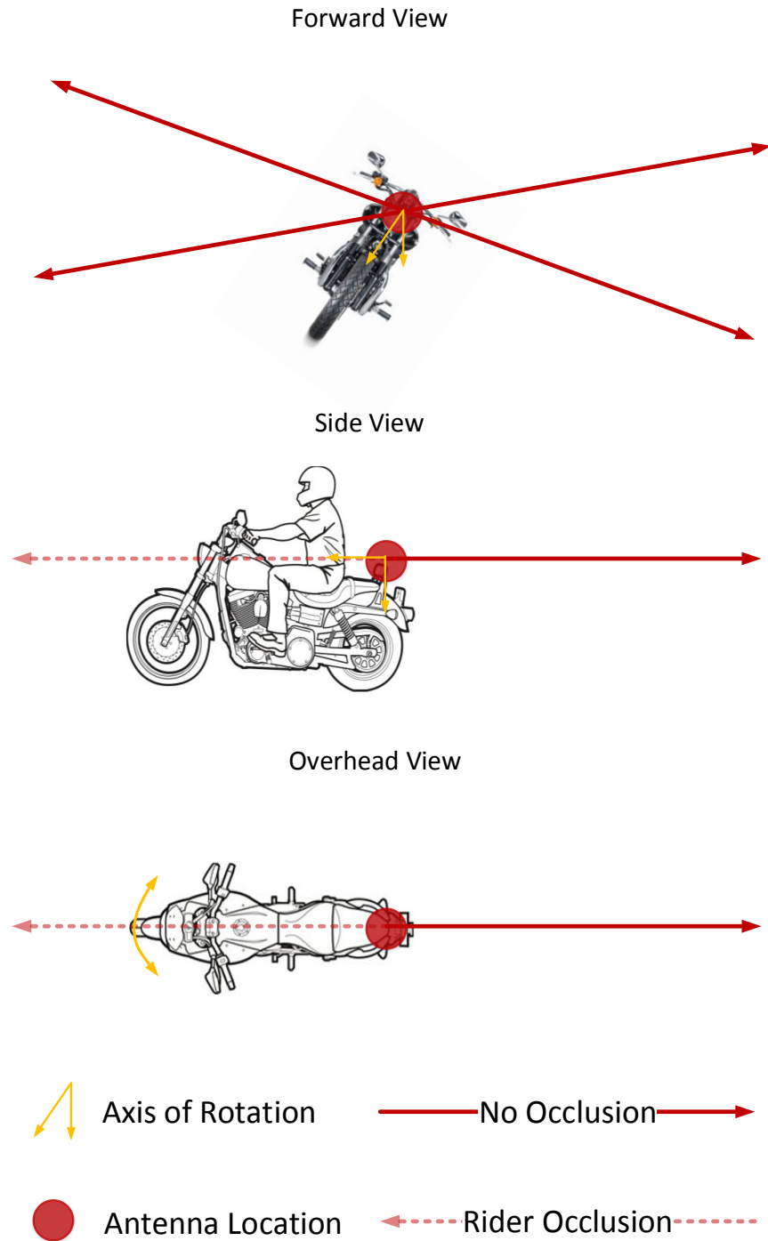
Figure 7. Rear Antenna.
