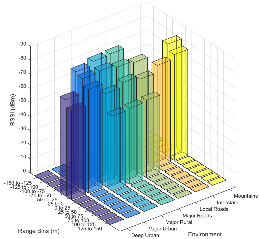
New River Valley Test: RSSI (dBm) Front Antenna Communicating with Ahead Vehicle (No Rider Occlusion) Vehicle Positions: 1-2
