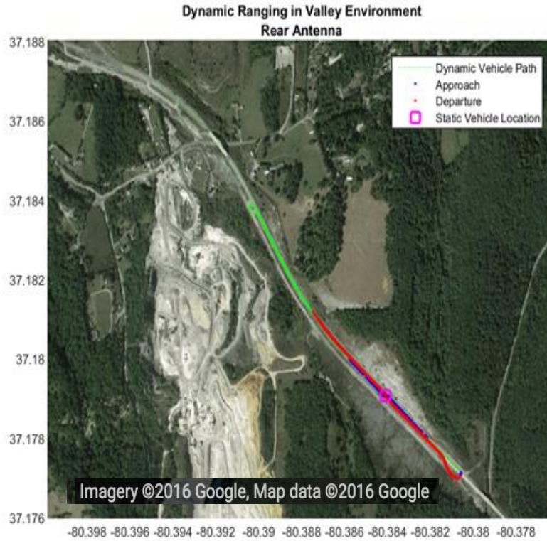
Figure 28. Dynamic ranging maps – Valley environment.
