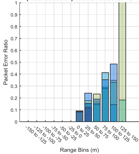
New River Valley Test: Packet Error Ratio vs Range (m) Front Antenna Communicating with Behind Vehicle (Rider Occlusion) Vehicle Positions: 4-2
