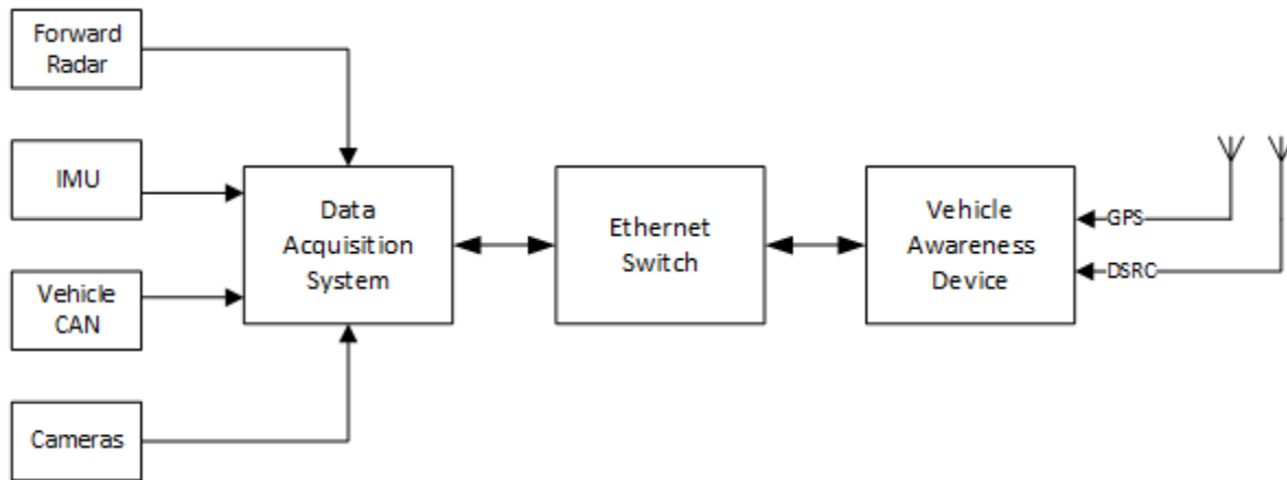
Figure 3. Test vehicle equipment diagram.
