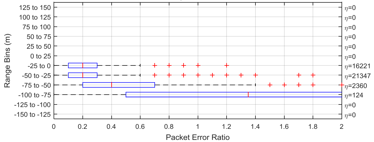
Dynamic Platoon - Smart Road Test: Packet Error Ratio Rear Antenna Communicating with Ahead Vehicle (Rider Occlusion) Formation: 2 | Vehicle Positions: 1-2
