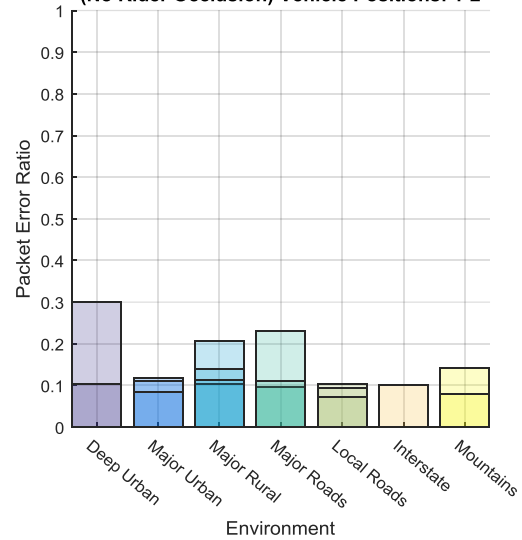
New River Valley Test: Packet Error Ratio vs Environment Front Antenna Communicating with Ahead Vehicle (No Rider Occlusion) Vehicle Positions: 1-2
