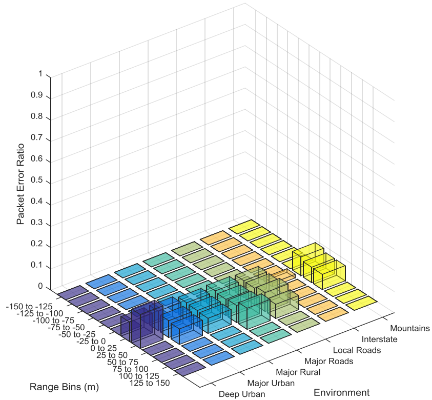
New River Valley Test: Packet Error Ratio Rear Antenna Communicating with Behind Vehicle (No Rider Occlusion) Vehicle Positions: 4-3
