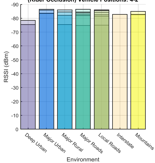
New River Valley Test: RSSI (dBm) vs Environment Front Antenna Communicating with Behind Vehicle (Rider Occlusion) Vehicle Positions: 4-2
