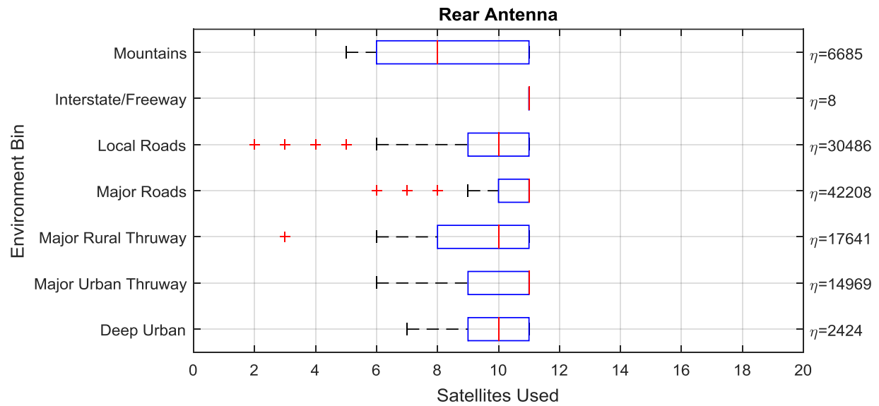
Figure 42. New River Valley Position performance – Satellites used.
