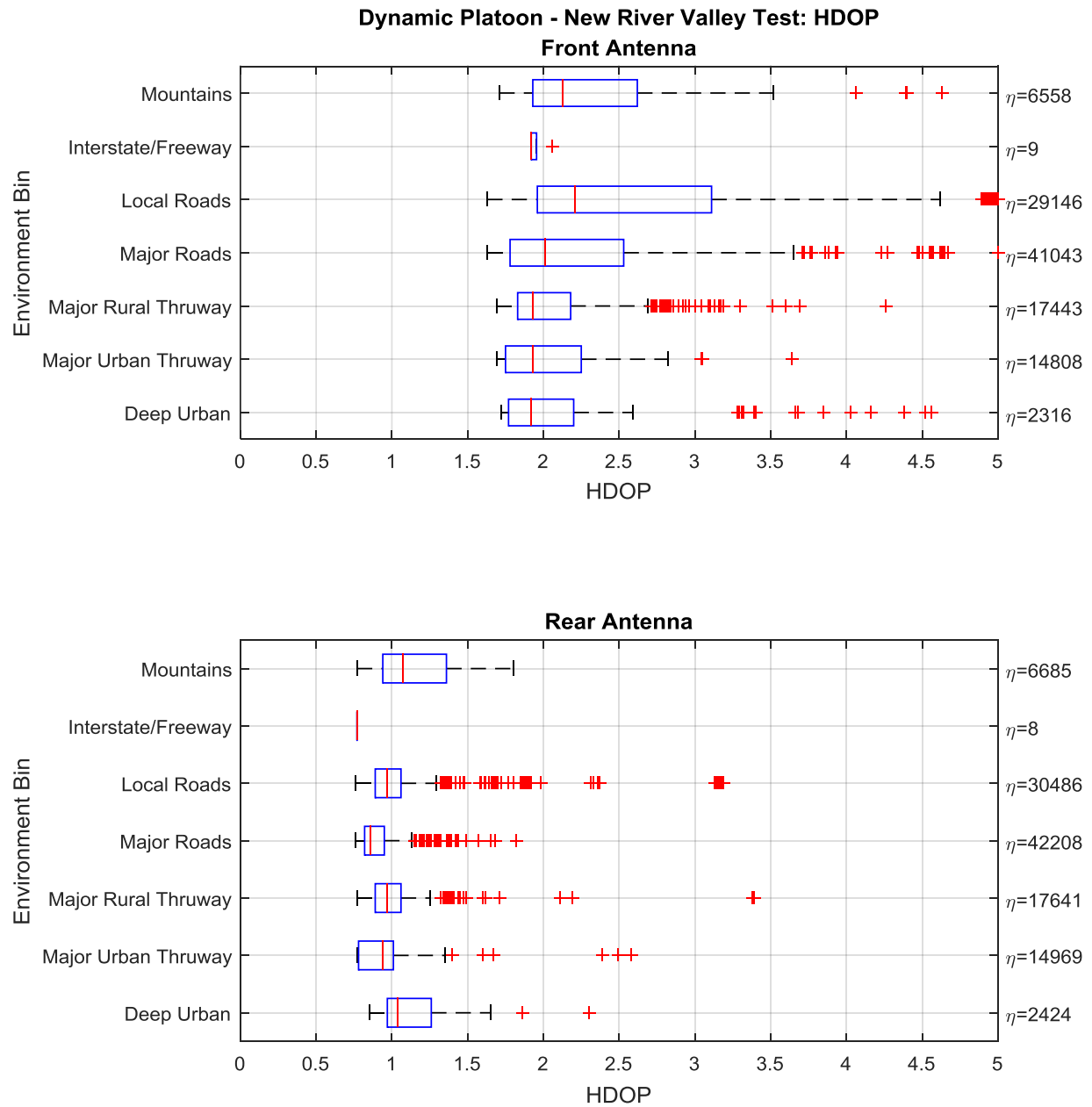
Figure 41. New River Valley Position performance – HDOP.
