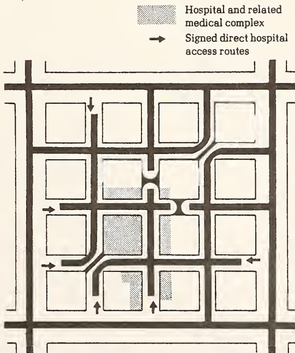
Figure 15. MAZE SYSTEM WITH INTERNAL SPECIAL GENERATOR (HOSPITAL)
