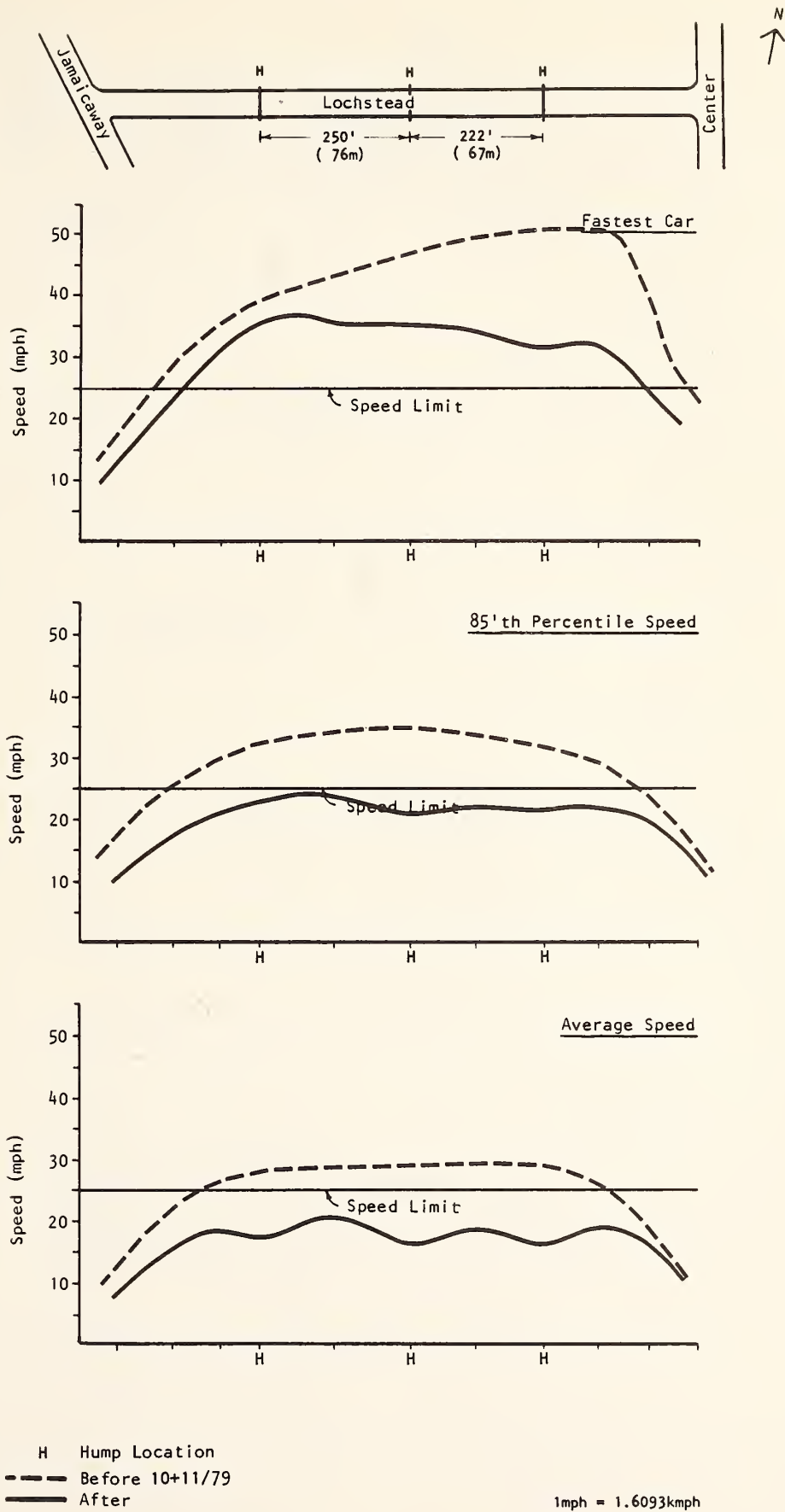
Figure 29. LOCHSTEAD SPEED STUDY - WESTBOUND
