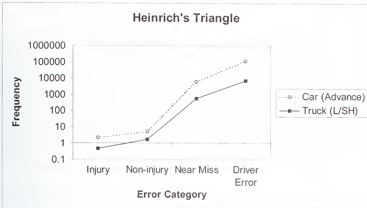
Figure 30. Comparison of car and L/SH data by Heinrich's Triangle categories.
