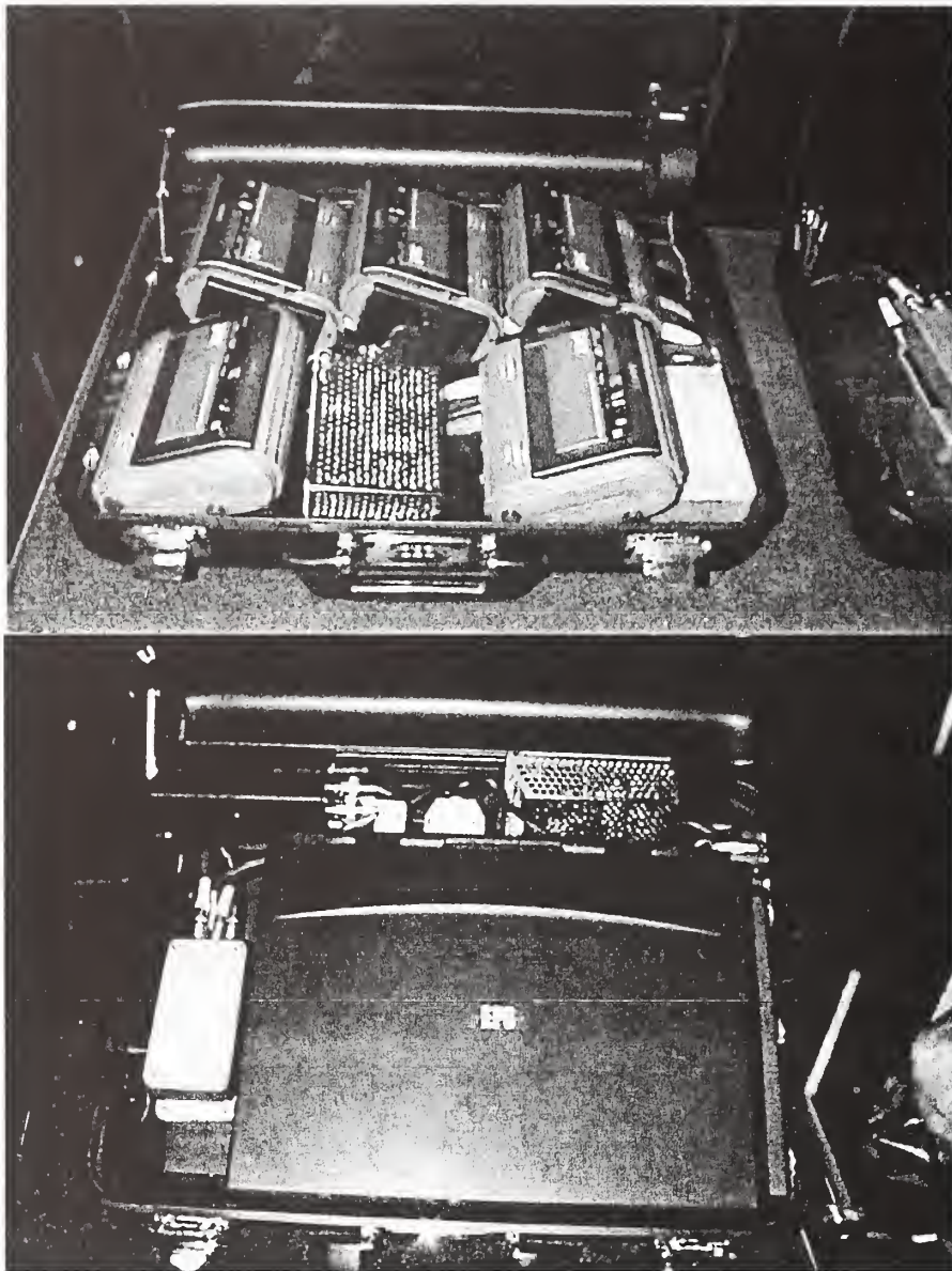
Figure 8. One of the black box data collection systems that were installed in L/SH trucks.
