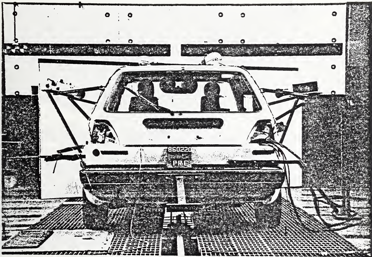
Figure 7. PRE-TEST VEHICLE REAR
