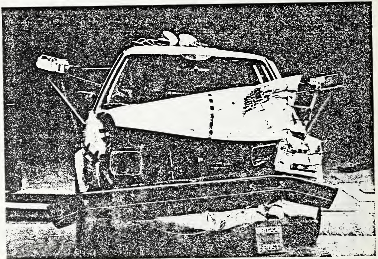
Figure 6. POST-TEST VEHICLE FRONT
