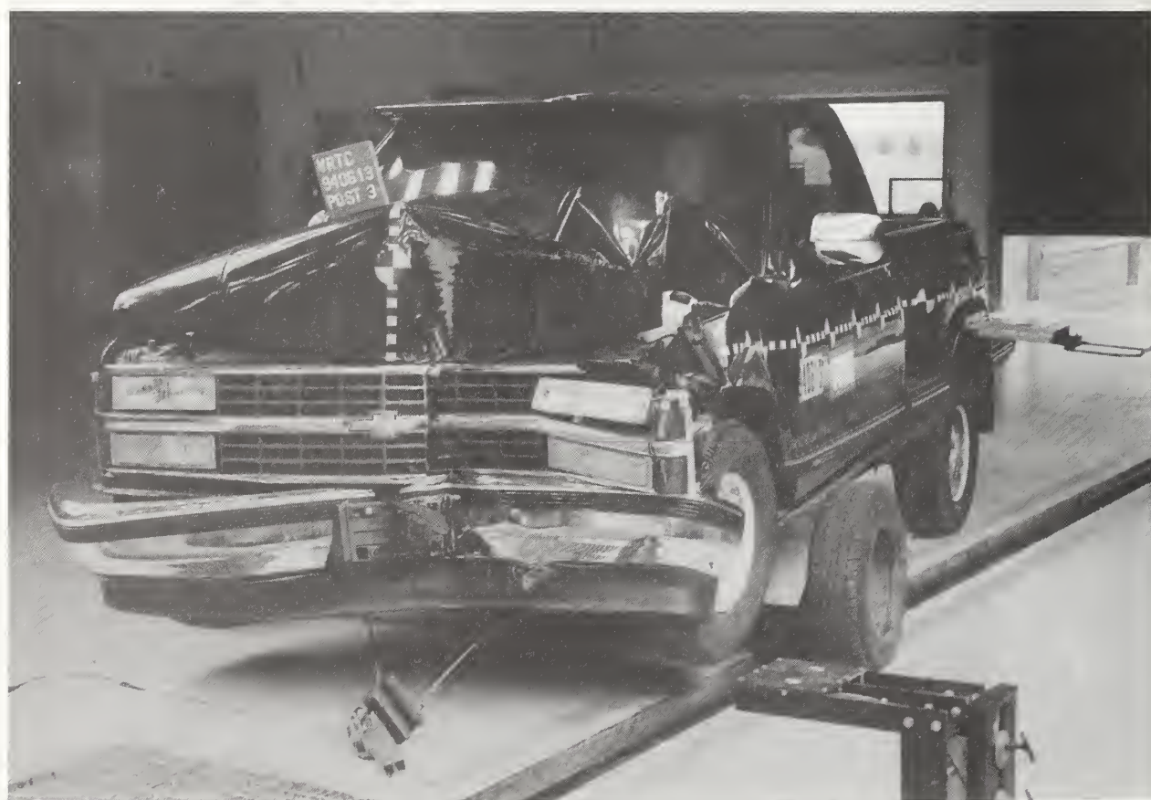
Figure A-22 Post-Test Left Front Three-Quarter View
