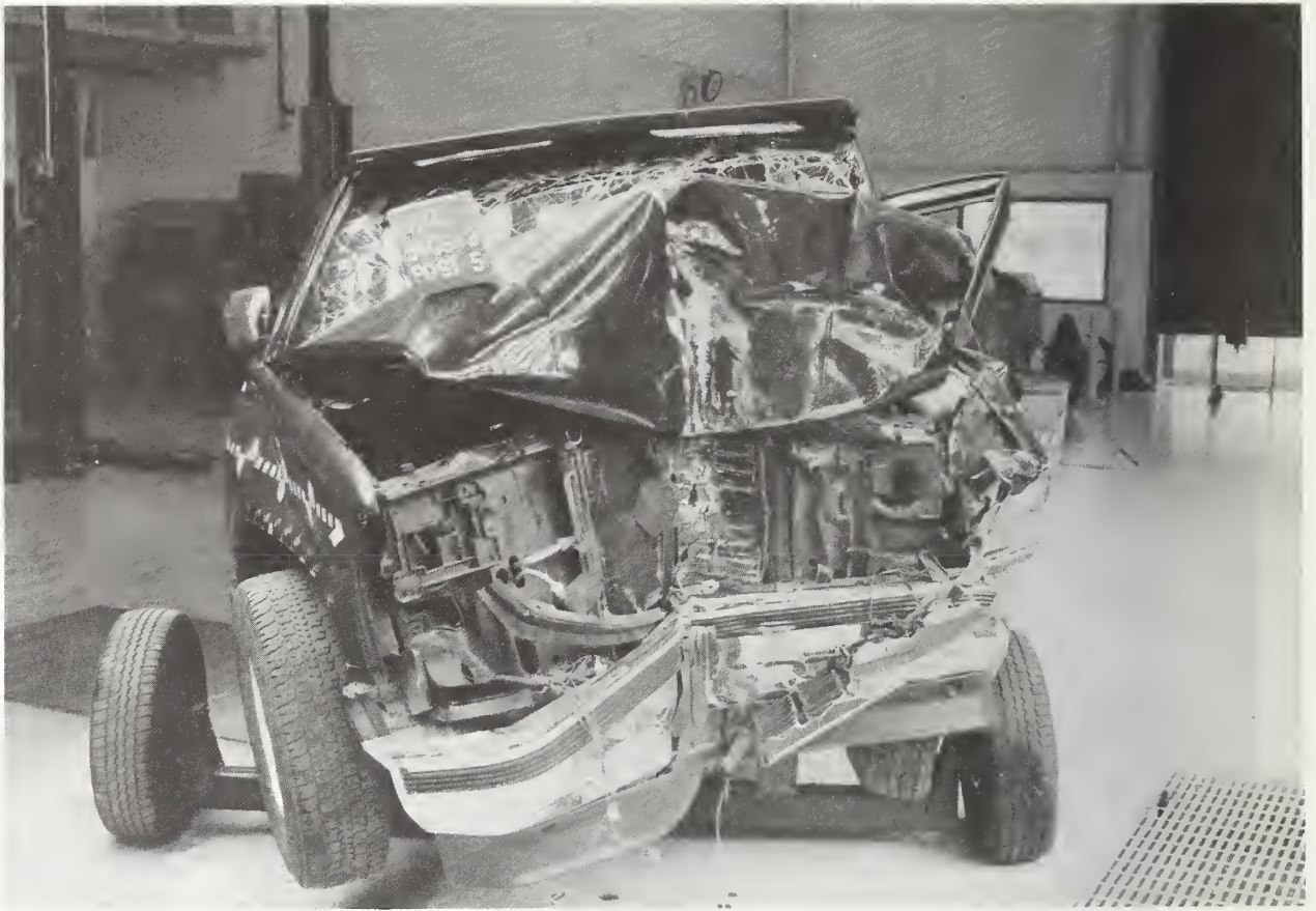
Figure A-33 Post-Test Front View
