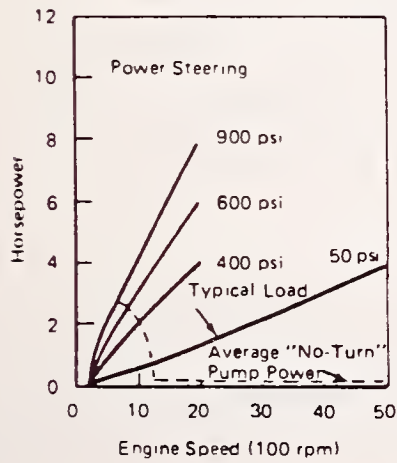
FIGURE 3-3. POWER REQUIREMENTS FOR ACCESSORIES IN STANDARD-SIZE CAR (Ref. 3-16)
