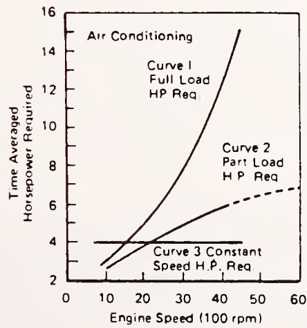
FIGURE 3-3. POWER REQUIREMENTS FOR ACCESSORIES IN STANDARD-SIZE CAR (Ref. 3-16)
