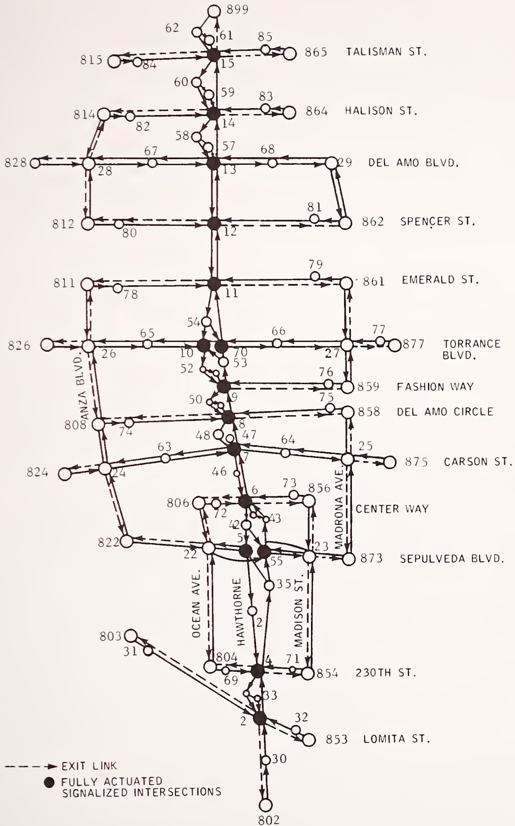
FIGURE 3-24. PRE-TIMED AND FULLY ACTUATED SIGNAL SYSTEMS (PORTION OF HAWTHORNE BLVD. ARTERIAL, LOS ANGELES) (Ref. 3-92)
