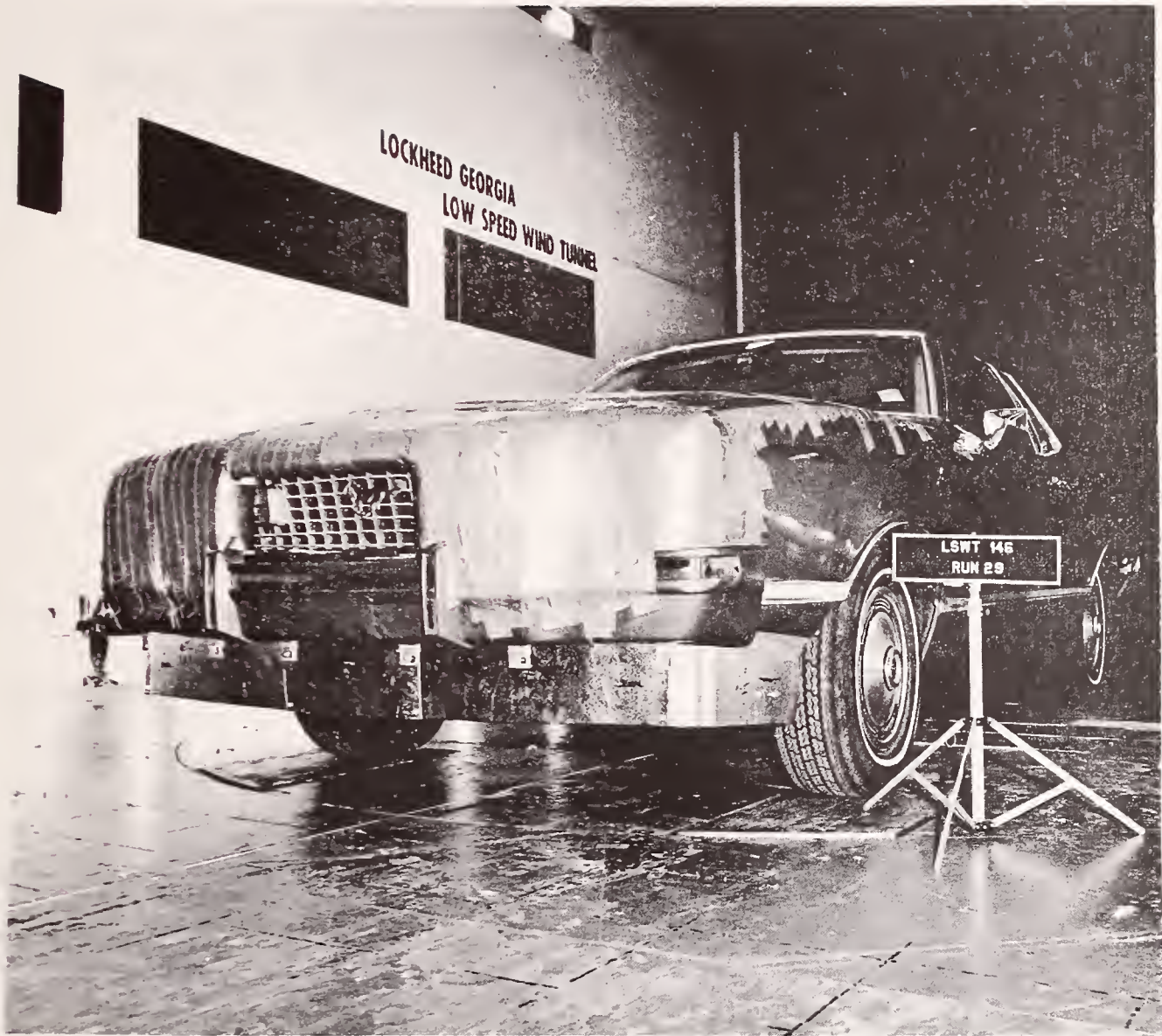
FIGURE 3-18. JPL FRONT AIR DAM ON 1974 MUSTANG II (Ref. 3-55)
