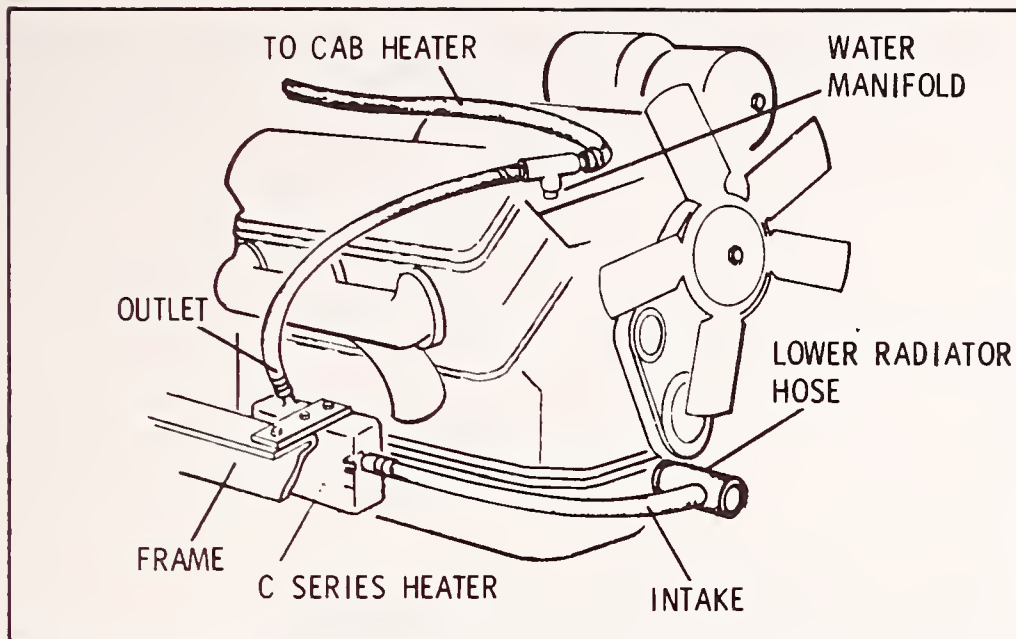
FIGURE 3-8. ENGINE PREHEATER INSTALLATION (Ref. 3-35)
