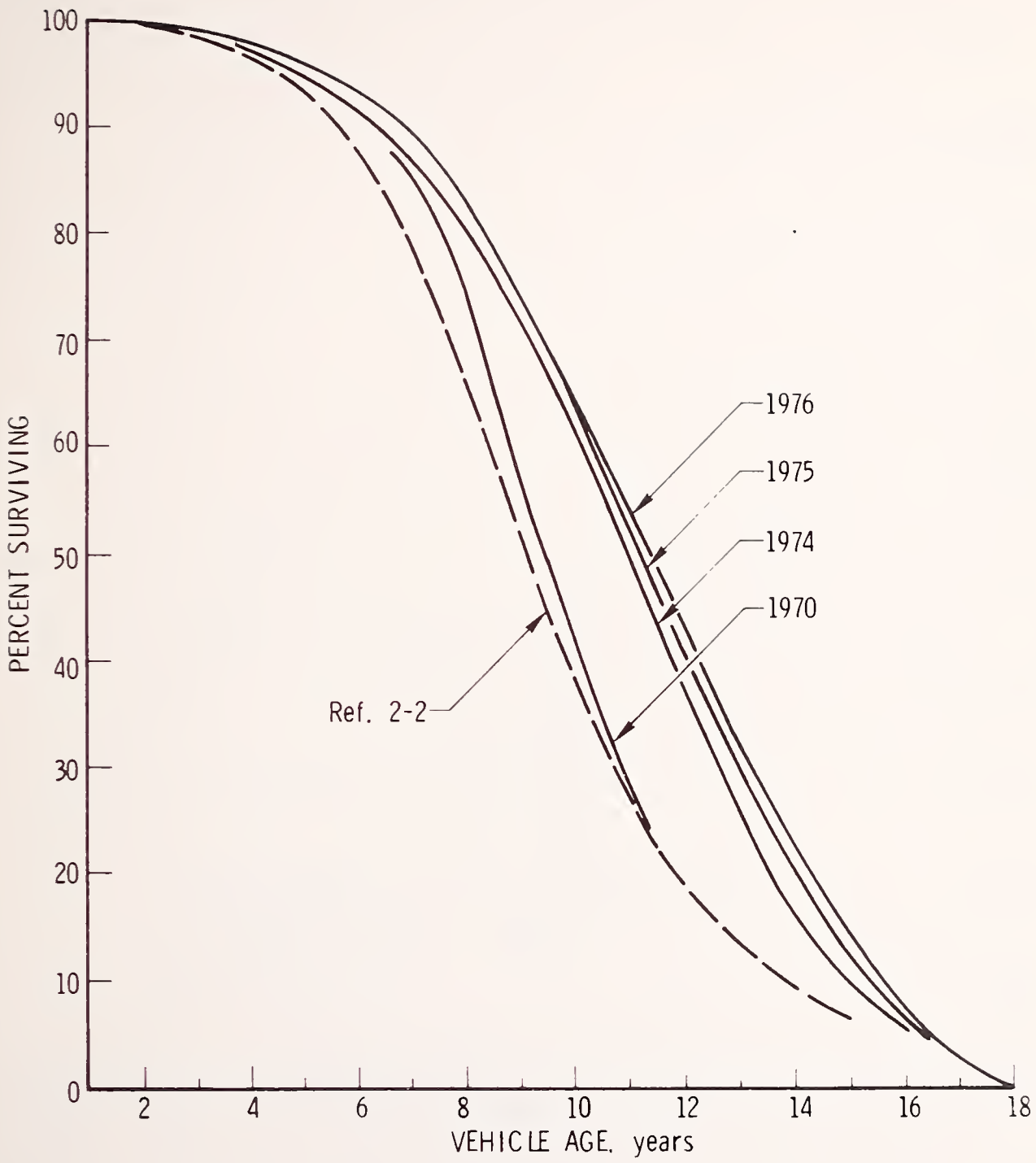
FIGURE 2-1. SURVIVABILITY CHARACTERISTICS FOR PASSENGER CARS
