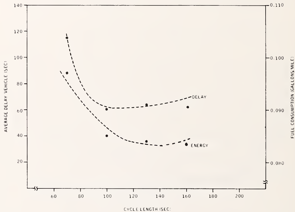
FIGURE 3-26. FUEL CONSUMPTION AND DELAY AS A FUNCTION OF CYCLE LENGTH FOR HAWTHORNE BLVD. NETWORK (Ref. 3-92)
