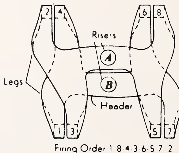
FIGURE 3-5. V-8 INTAKE MANIFOLD (Ref. 3-23)
