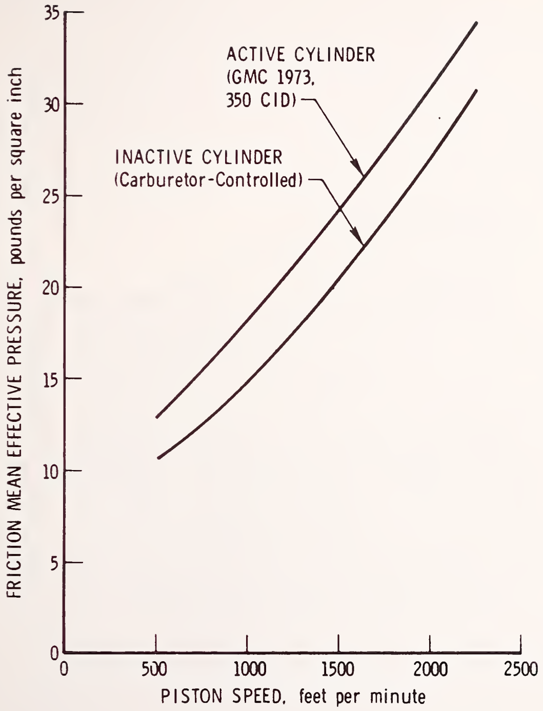
FIGURE 3-6. VARIABLE-CYLINDER ENGINE FRICTION AND PUMPING LOSSES (Ref. 3-28)
