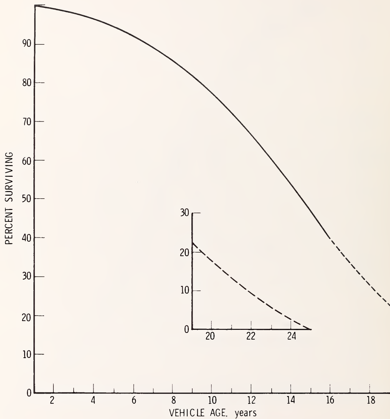
FIGURE 2-2. SURVIVABILITY CHARACTERISTICS FOR LIGHT DUTY TRUCKS (CLASS I AND II)
