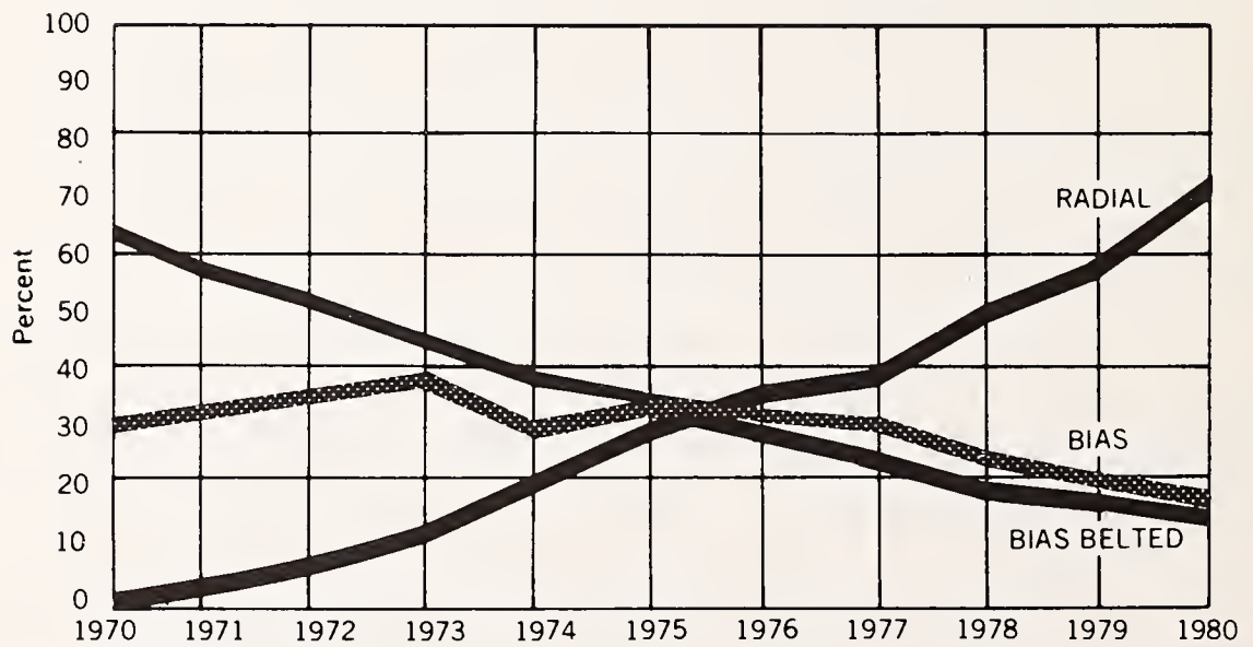
FIGURE 3-16. AFTERMARKET TIRE TRENDS (PASSENGER CARS) (Ref. 3-48)
