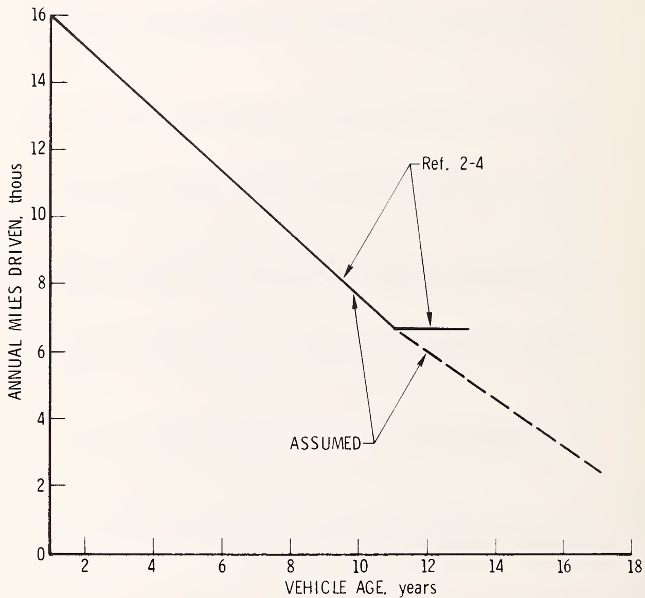
FIGURE 2-3. AVERAGE ANNUAL MILES DRIVEN BY VEHICLE AGE (PASSENGER CARS)
