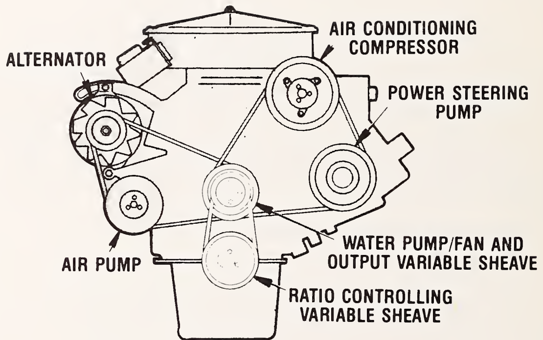
FIGURE 3-2. VARIABLE RATIO BELT DRIVE SYSTEM (Ref. 3-15)
