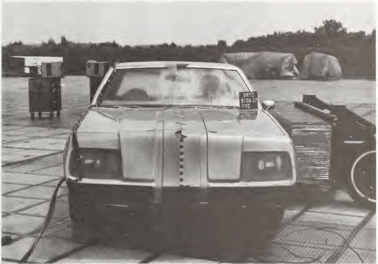
Figure A-1. PRE-TEST VEHICLE FRONT AND BARRIER VIEW
