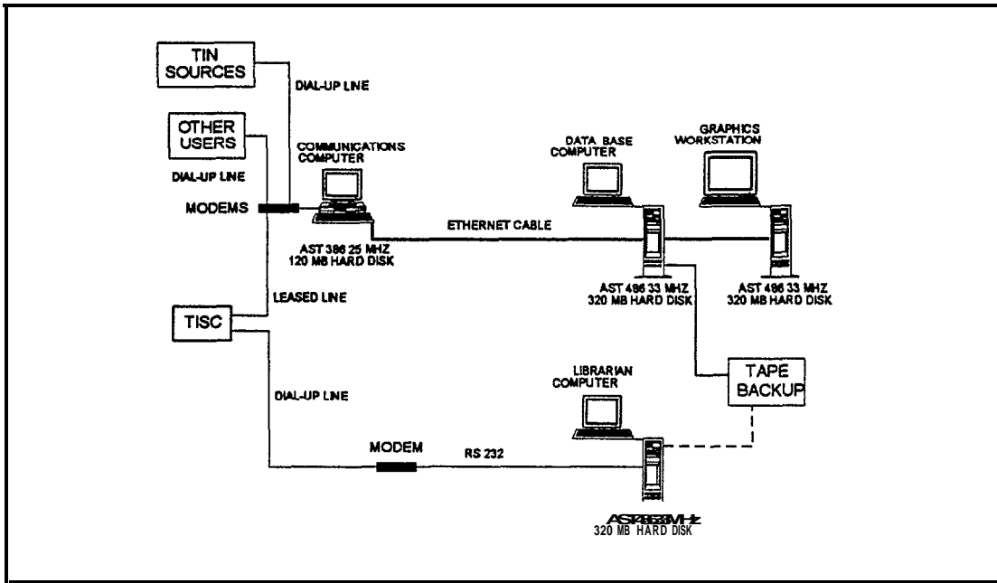
Figure 15. TMC computer configuration. (I)
