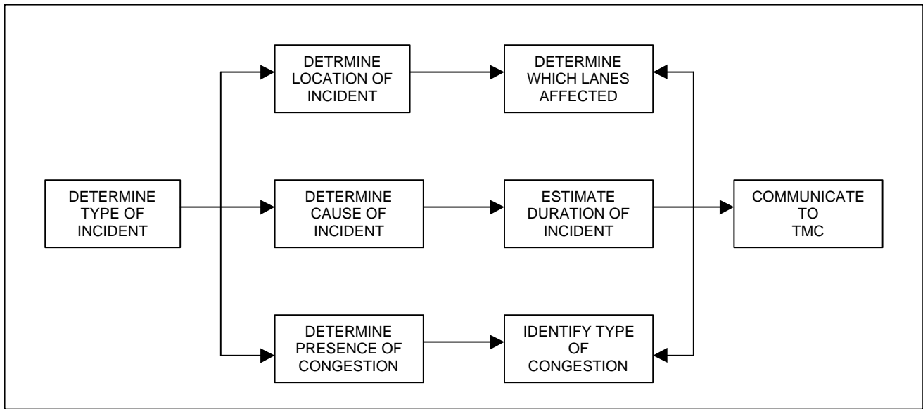
Figure 9. Functional diagram of incident/congestion reporting task
