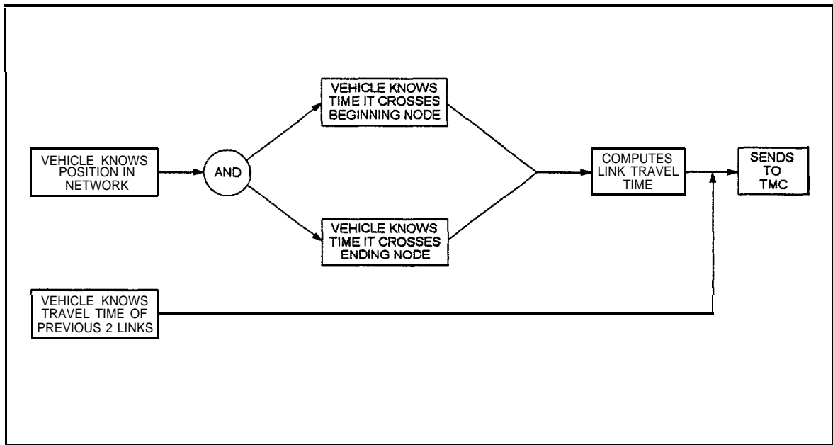
Figure 41. Vehicle probe function.
