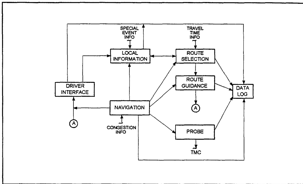
Figure 29. Interactions between TravTek vehicle functions.
