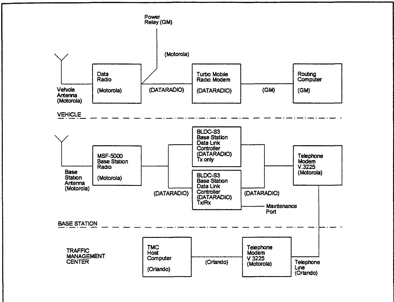
Figure 22. TMC/vehicle data radio system. (12)
