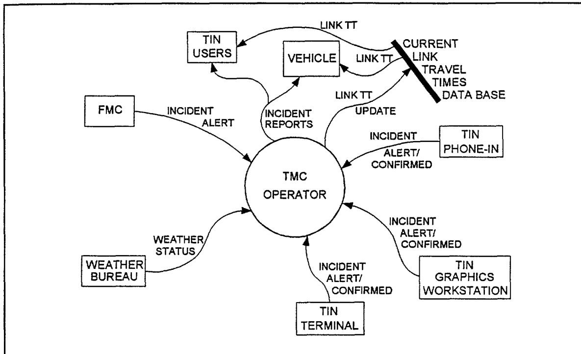
Figure 26. TMC operator interaction process data flow.
