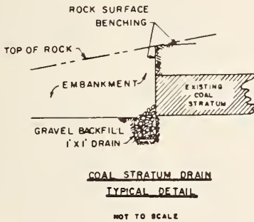
a. Sidehill embankment benching and drainage
