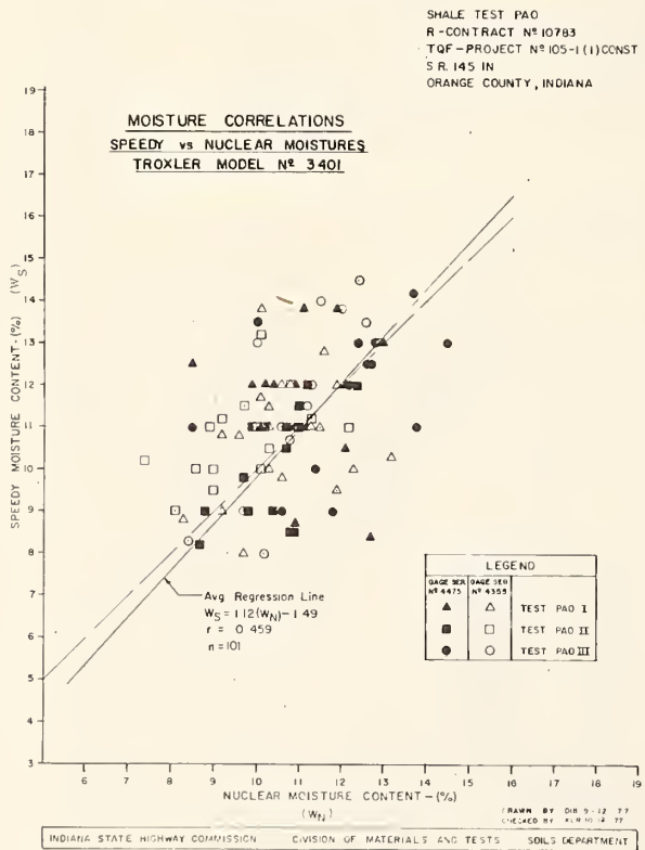
Figure 67. Example of inherent scatter in moisture and density data for a carefully conducted shale test pad program (courtesy Indiana State Highway Commission)
