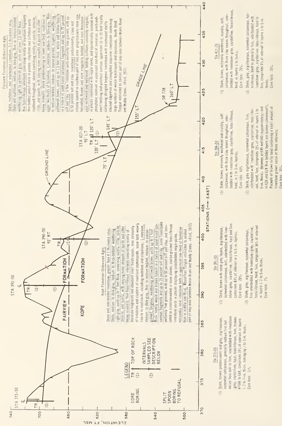
Figure 6. Example of geologic profile using existing quadrangle geology and boring logs (discussed subsequently). (Boring log description courtesy of Ohio Department of Transportation)
