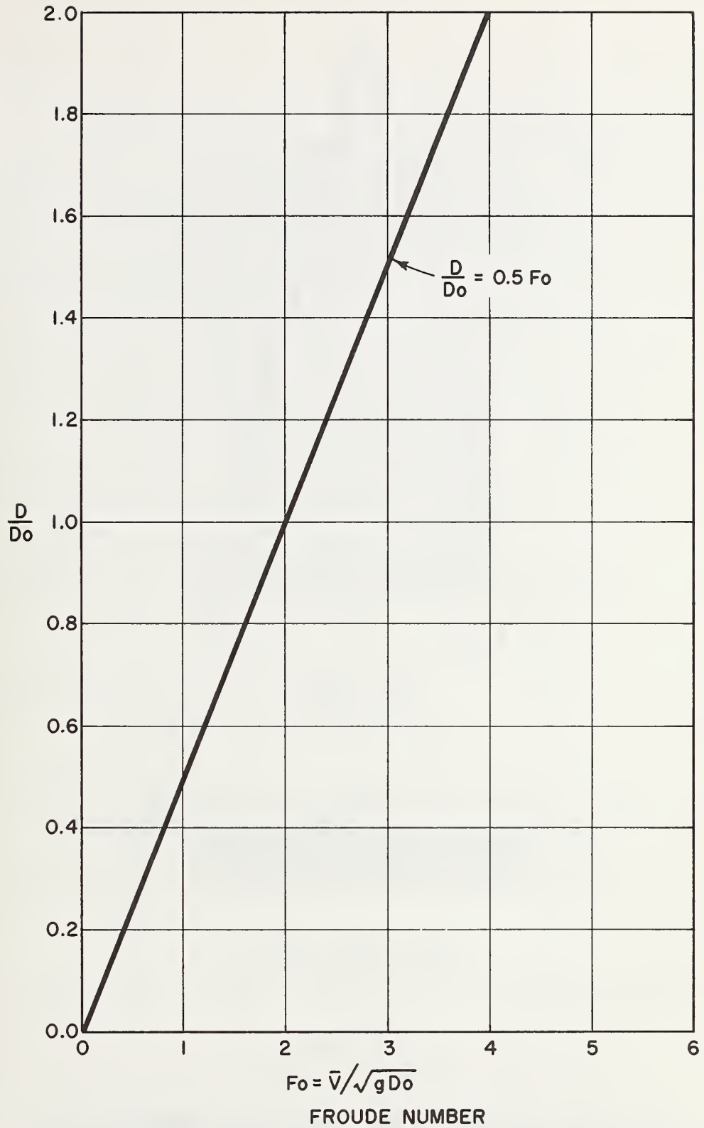
FIGURE 3. HORIZONTAL RIPRAP THICKNESS (MIN. TAILWATER) U.S. ARMY WATERWAYS EXPERIMENT STATION ROCK BASINS
