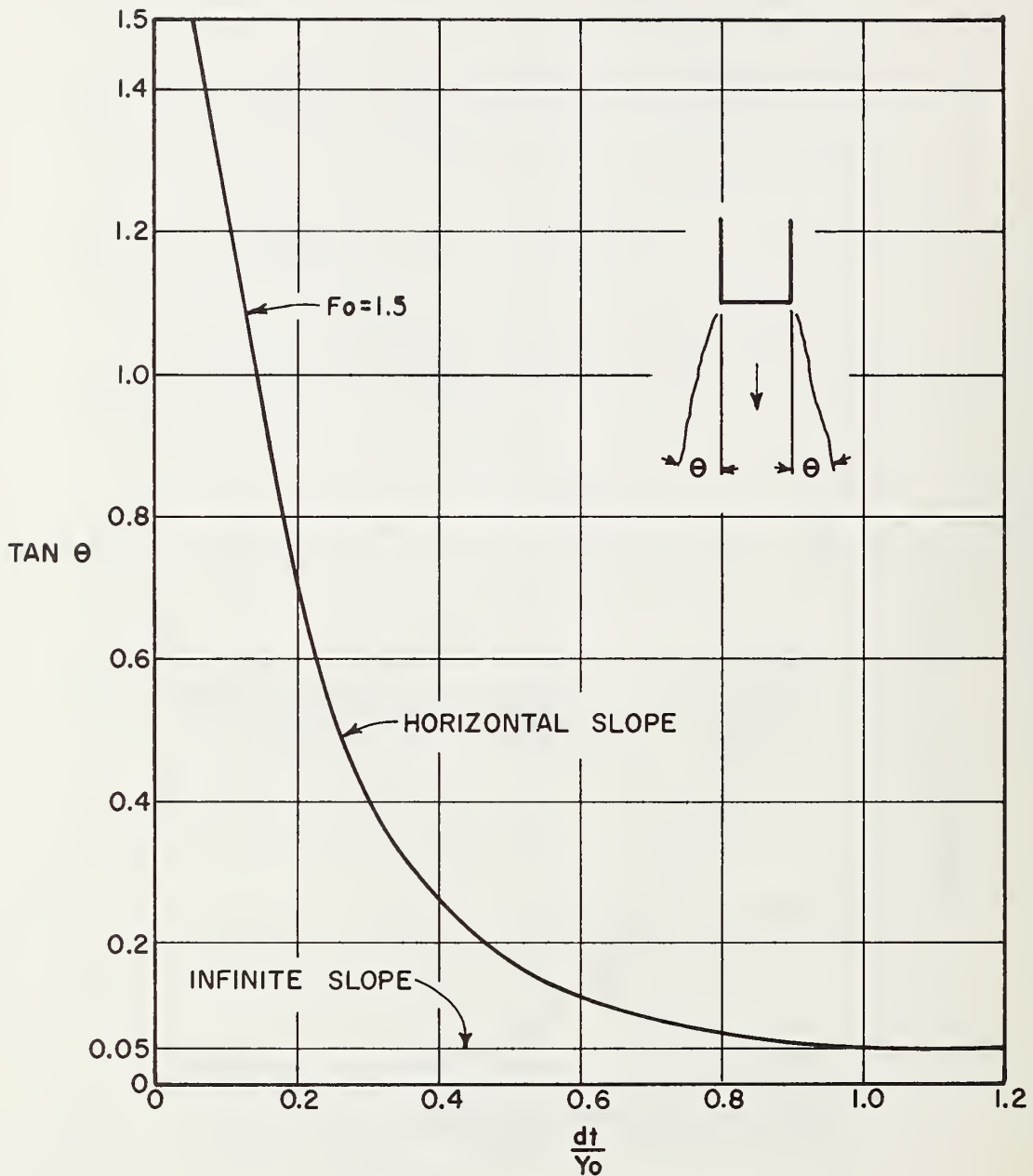
FIGURE 20. AN ESTIMATE OF THE ANGLE OF LATERAL EXPANSION FOR HORIZONTAL AND MILD SLOPING CIRCULAR CULVERTS COLORADO STATE UNIVERSITY ROCK RIPRAPED BASINS
