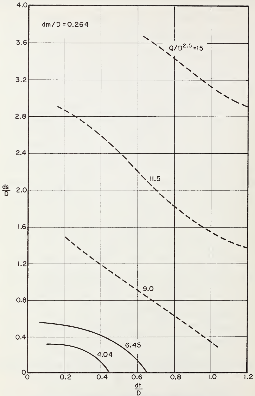
FIGURE 18. SCOUR: PLAIN CIRCULAR OUTLET COLORADO STATE UNIVERSITY ROCK RIPRAPPED BASINS
