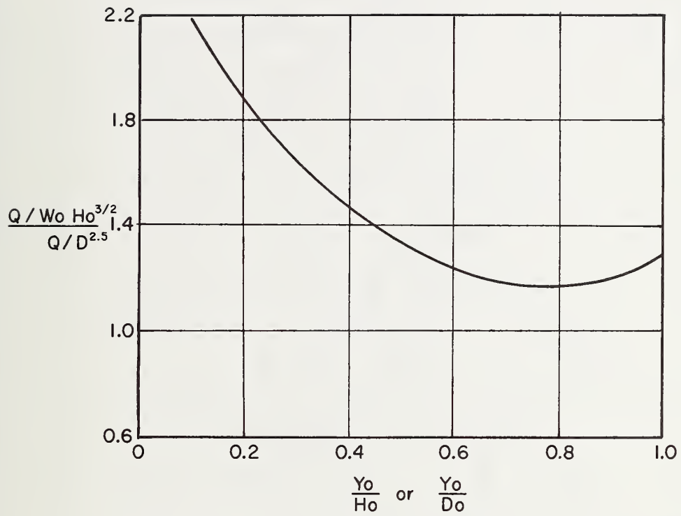
FIGURE 13. DISCHARGE RATIOS FOR THE TWO-DIMENSIONAL FLOW APPROXIMATION COLORADO STATE UNIVERSITY ROCK RIPRAPED BASIN
