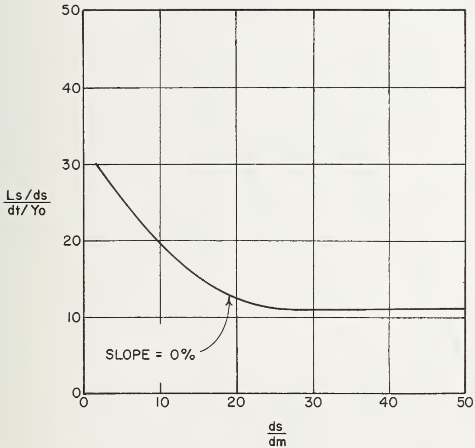
FIGURE 23. LENGTH OF SCOUR HOLE COLORADO STATE UNIVERSITY ROCK RIPRAPPED BASIN
