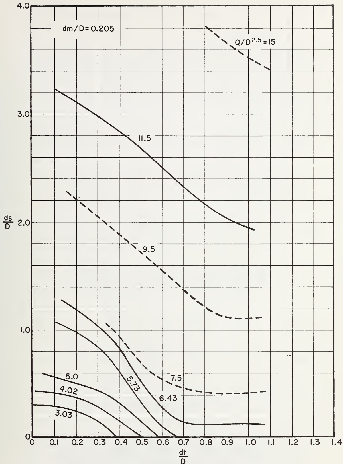
FIGURE 17. SCOUR: PLAIN CIRCULAR OUTLET COLORADO STATE UNIVERSITY ROCK RIPRAPPED BASIN
